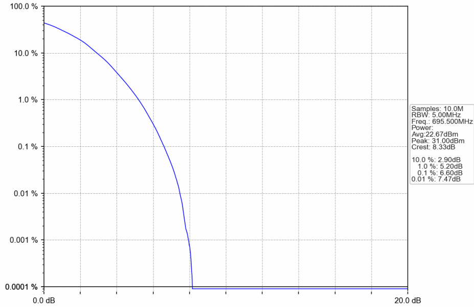
Band71_5MHz_64QAM_HCH_695.5MHz_RB_25_0_NTNV
