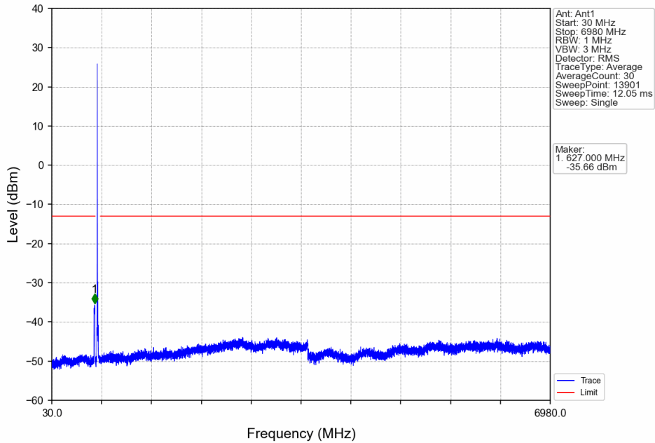
Band71_15MHz_16QAM_LCH_670.5MHz_RB_1_0_NTNV
