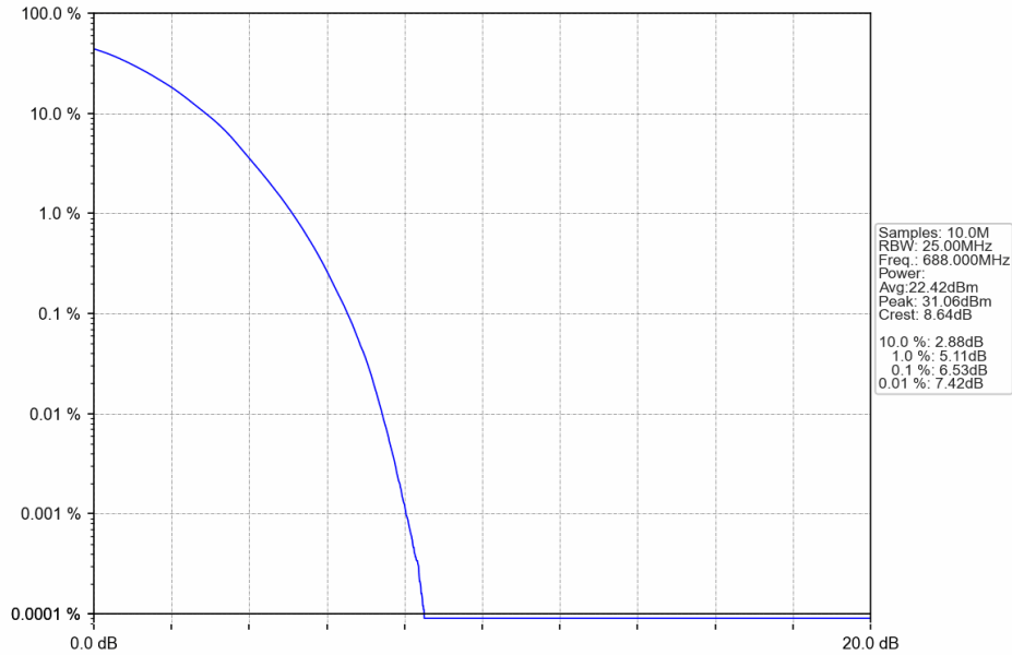
Band71_20MHz_64QAM_HCH_688MHz_RB_100_0_NTNV
