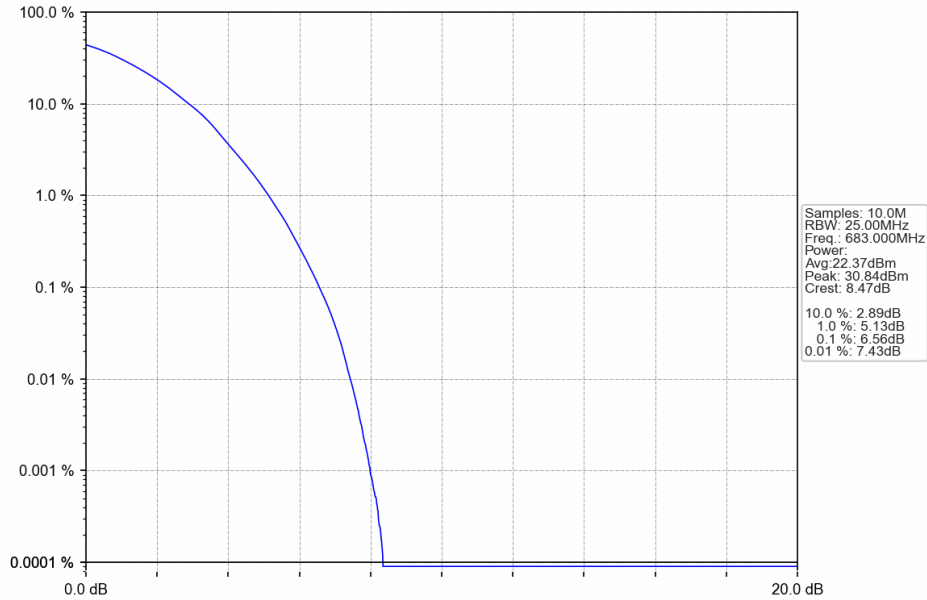
Band71_20MHz_64QAM_MCH_683MHz_RB_100_0_NTNV
