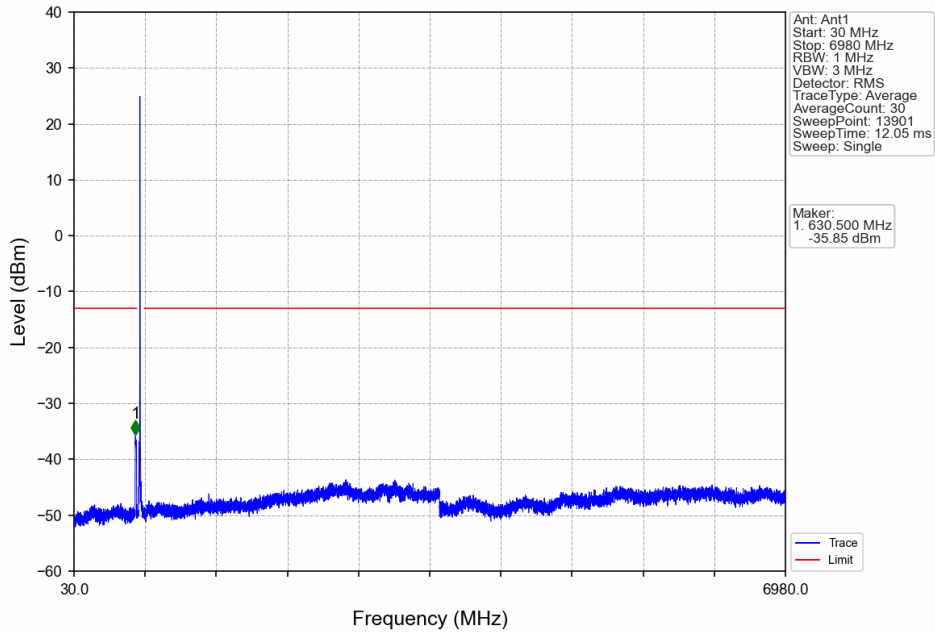
Band71_15MHz_16QAM_MCH_680.5MHz_RB_1_0_NTNV
