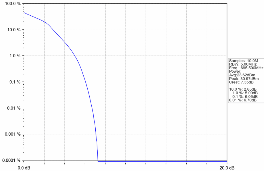
Band71_5MHz_16QAM_HCH_695.5MHz_RB_25_0_NTNV
