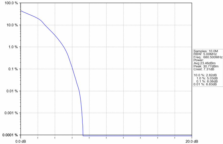
Band71_5MHz_16QAM_MCH_680.5MHz_RB_25_0_NTNV
