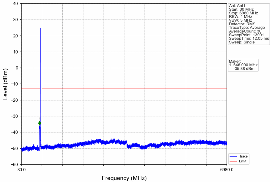
Band71_15MHz_64QAM_HCH_690.5MHz_RB_1_0_NTNV
