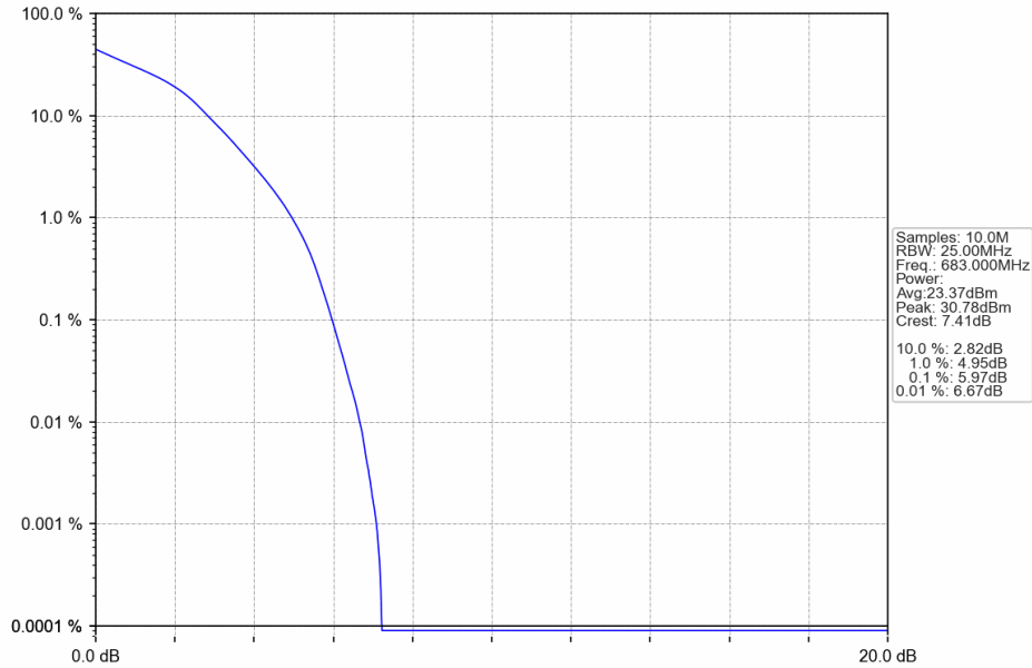
Band71_20MHz_16QAM_MCH_683MHz_RB_100_0_NTNV
