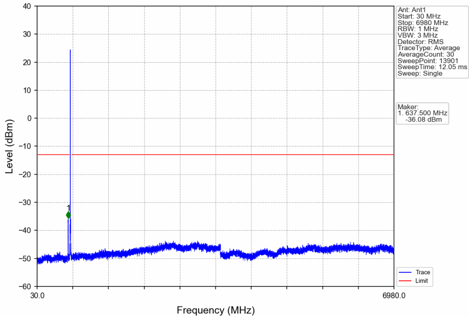
Band71_10MHz_16QAM_MCH_680.5MHz_RB_1_0_NTNV
