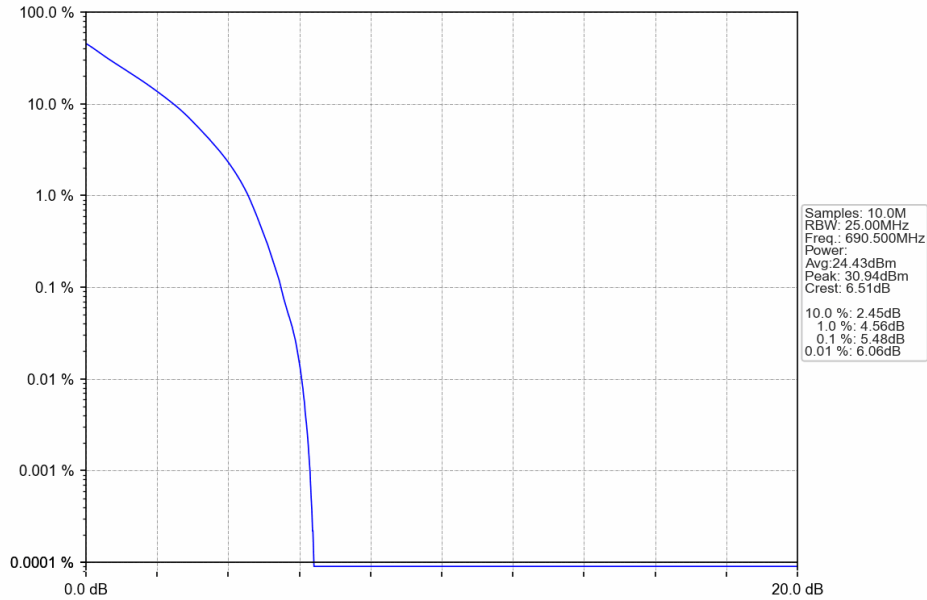
Band71_15MHz_QPSK_HCH_690.5MHz_RB_75_0_NTNV
