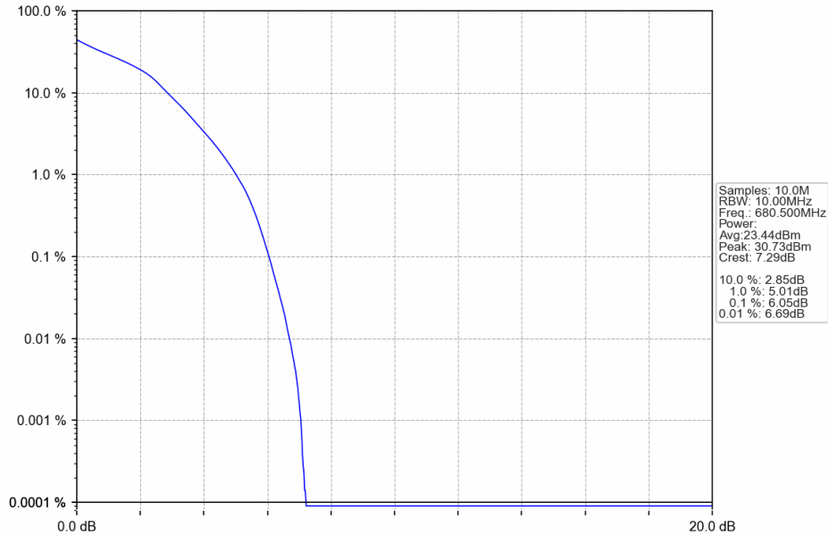
Band71_10MHz_16QAM_MCH_680.5MHz_RB_50_0_NTNV
