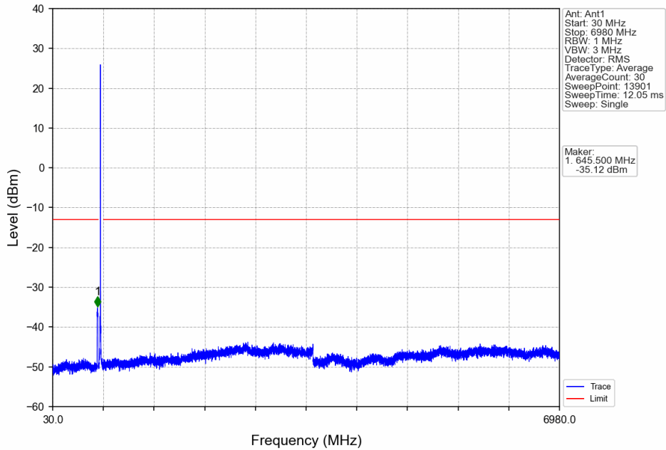
Band71_15MHz_16QAM_HCH_690.5MHz_RB_1_0_NTNV
