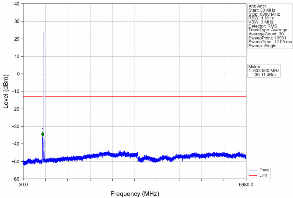
Band71_10MHz_64QAM_MCH_680.5MHz_RB_1_0_NTNV
