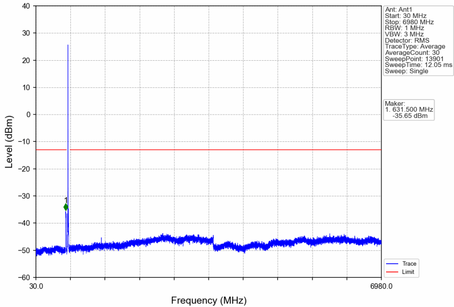
Band71_15MHz_QPSK_MCH_680.5MHz_RB_1_0_NTNV
