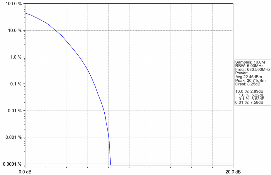
Band71_5MHz_64QAM_MCH_680.5MHz_RB_25_0_NTNV
