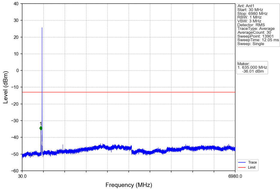
Band71_5MHz_QPSK_MCH_680.5MHz_RB_1_0_NTNV
