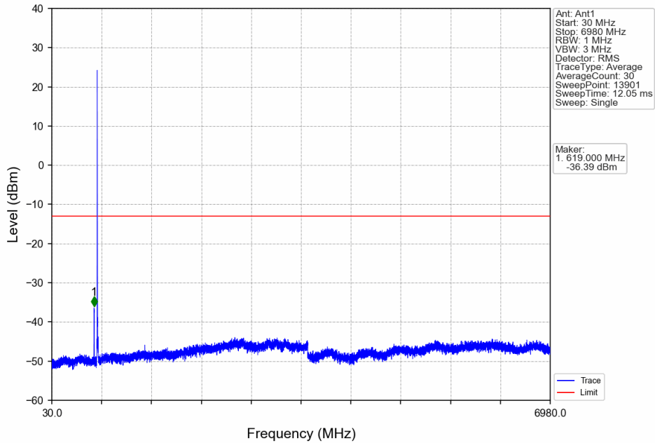
Band71_5MHz_64QAM_LCH_665.5MHz_RB_1_0_NTNV
