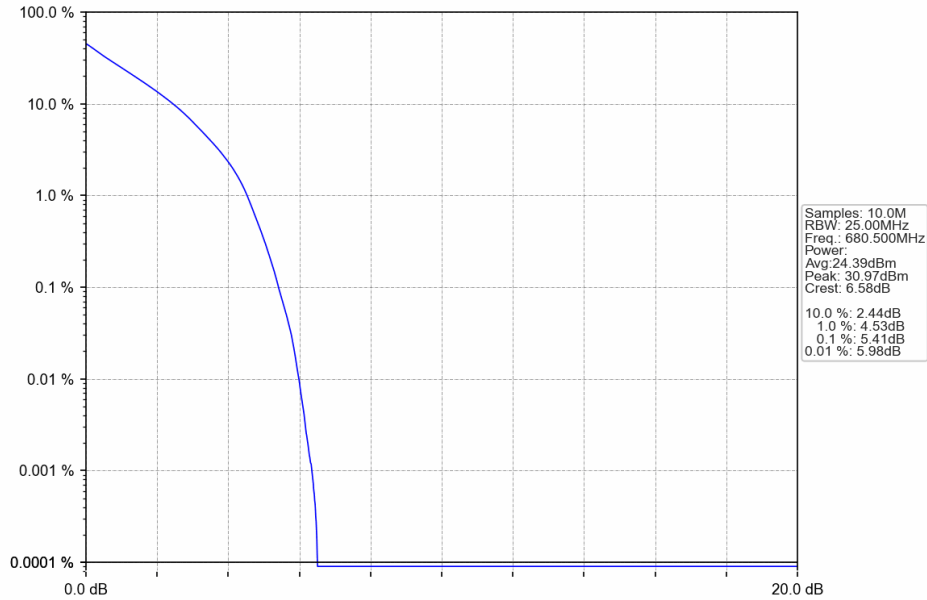
Band71_15MHz_QPSK_MCH_680.5MHz_RB_75_0_NTNV
