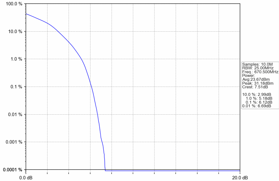
Band71_15MHz_16QAM_LCH_670.5MHz_RB_75_0_NTNV
