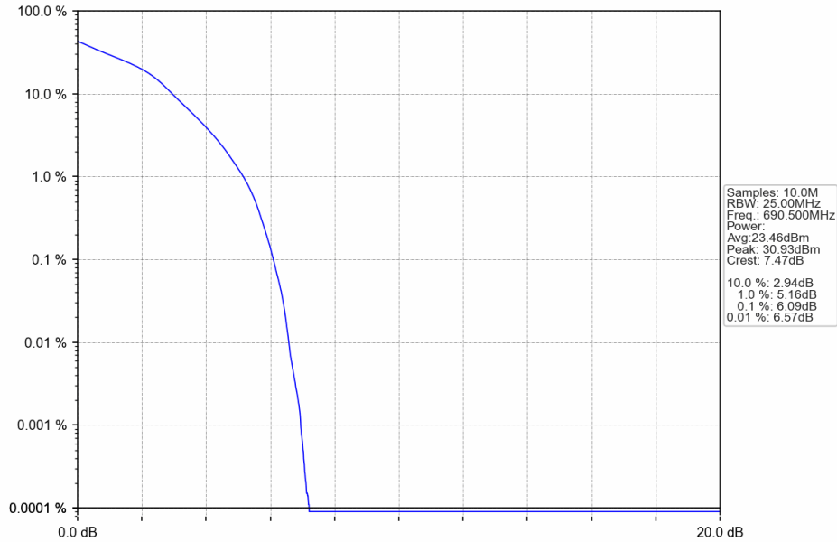
Band71_15MHz_16QAM_HCH_690.5MHz_RB_75_0_NTNV
