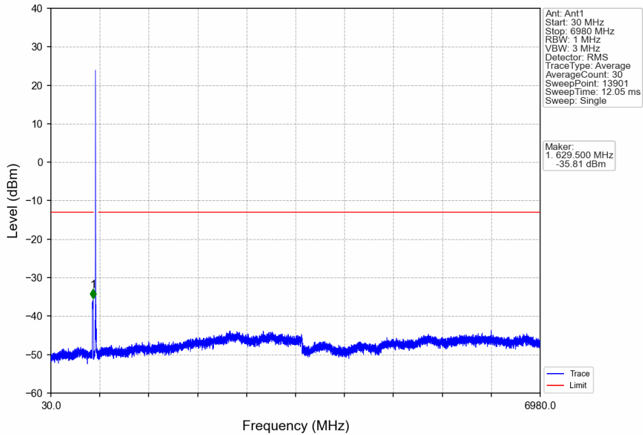
Band71_15MHz_64QAM_LCH_670.5MHz_RB_1_0_NTNV
