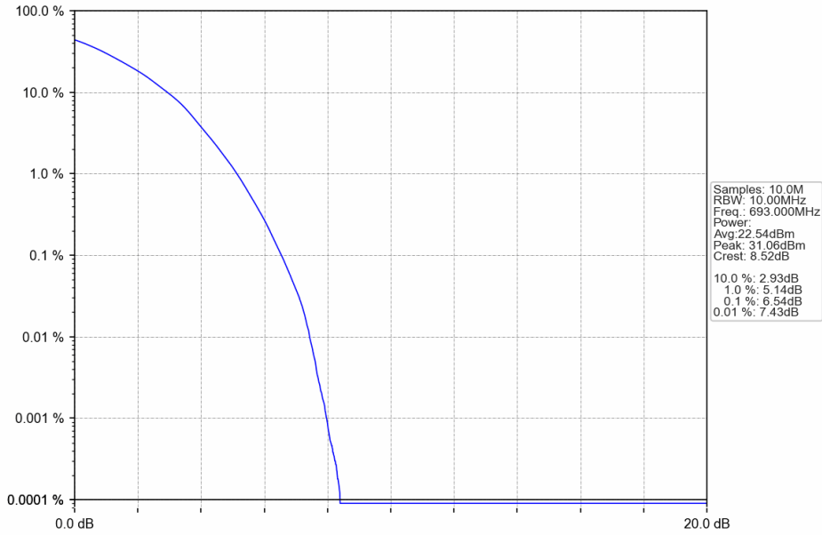
Band71_10MHz_64QAM_HCH_693MHz_RB_50_0_NTNV
