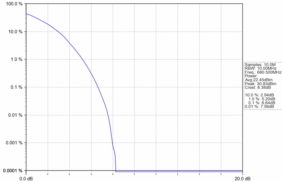
Band71_10MHz_64QAM_MCH_680.5MHz_RB_50_0_NTNV
