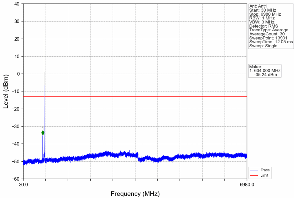
Band71_5MHz_16QAM_MCH_680.5MHz_RB_1_0_NTNV
