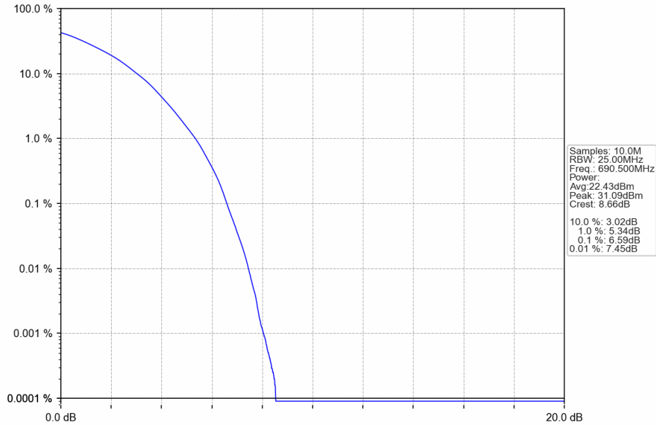
Band71_15MHz_64QAM_HCH_690.5MHz_RB_75_0_NTNV
