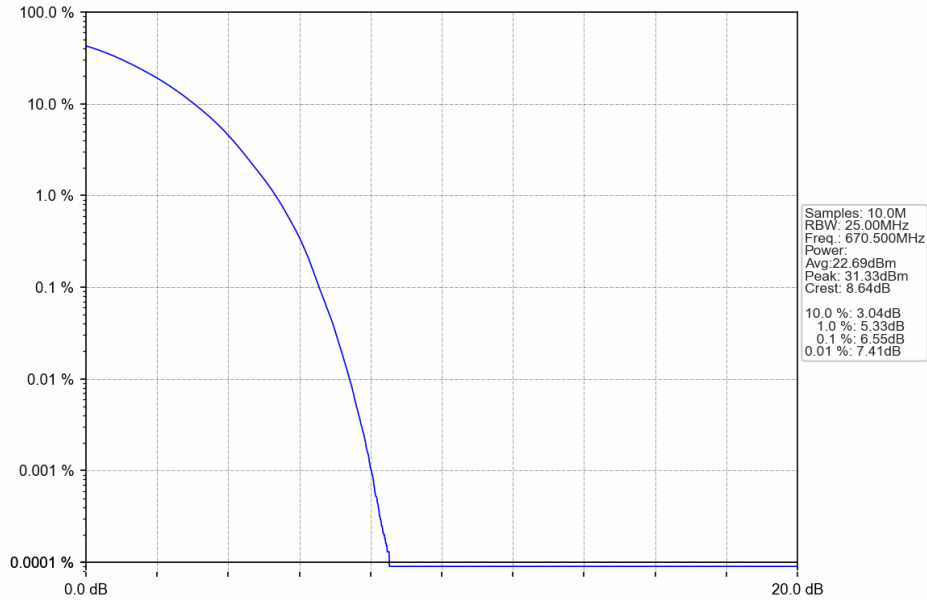
Band71_15MHz_64QAM_LCH_670.5MHz_RB_75_0_NTNV
