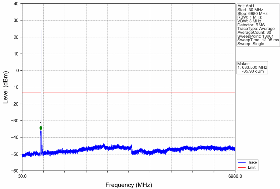
Band71_15MHz_64QAM_MCH_680.5MHz_RB_1_0_NTNV
