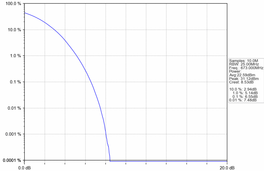
Band71_20MHz_64QAM_LCH_673MHz_RB_100_0_NTNV
