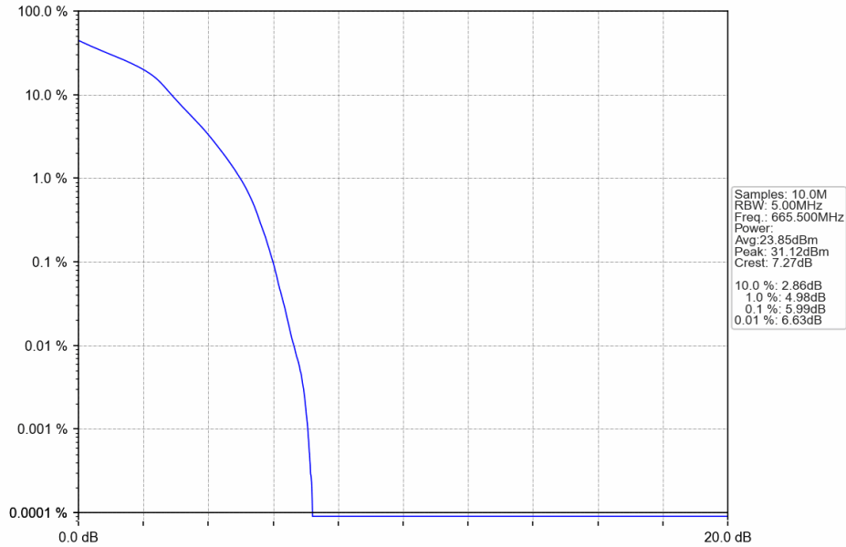
Band71_5MHz_16QAM_LCH_665.5MHz_RB_25_0_NTNV
