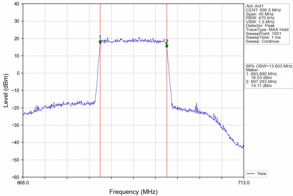
Band71_15MHz_16QAM_HCH_690.5MHz_RB_75_0_NTNV
