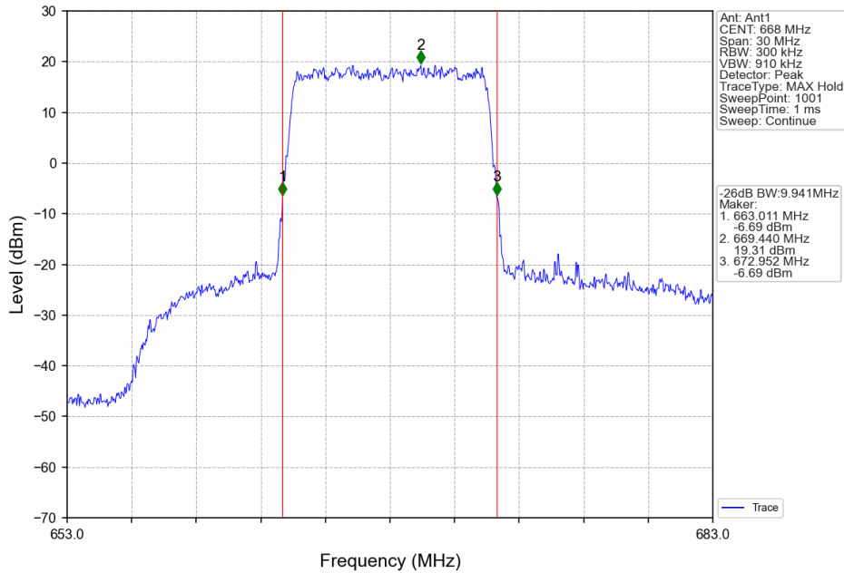
Band71_10MHz_64QAM_LCH_668MHz_RB_50_0_NTNV
