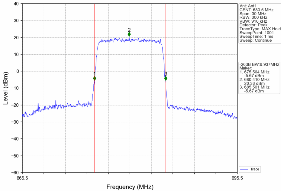
Band71_10MHz_16QAM_MCH_680.5MHz_RB_50_0_NTNV
