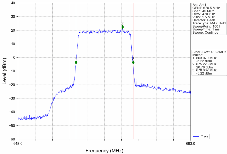
Band71_15MHz_16QAM_LCH_670.5MHz_RB_75_0_NTNV
