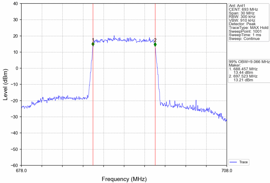
Band71_10MHz_64QAM_HCH_693MHz_RB_50_0_NTNV
