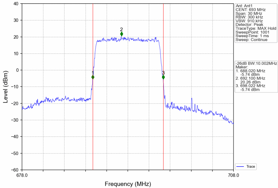
Band71_10MHz_16QAM_HCH_693MHz_RB_50_0_NTNV
