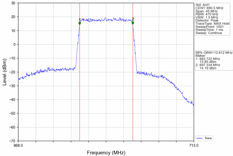
Band71_15MHz_64QAM_HCH_690.5MHz_RB_75_0_NTNV
