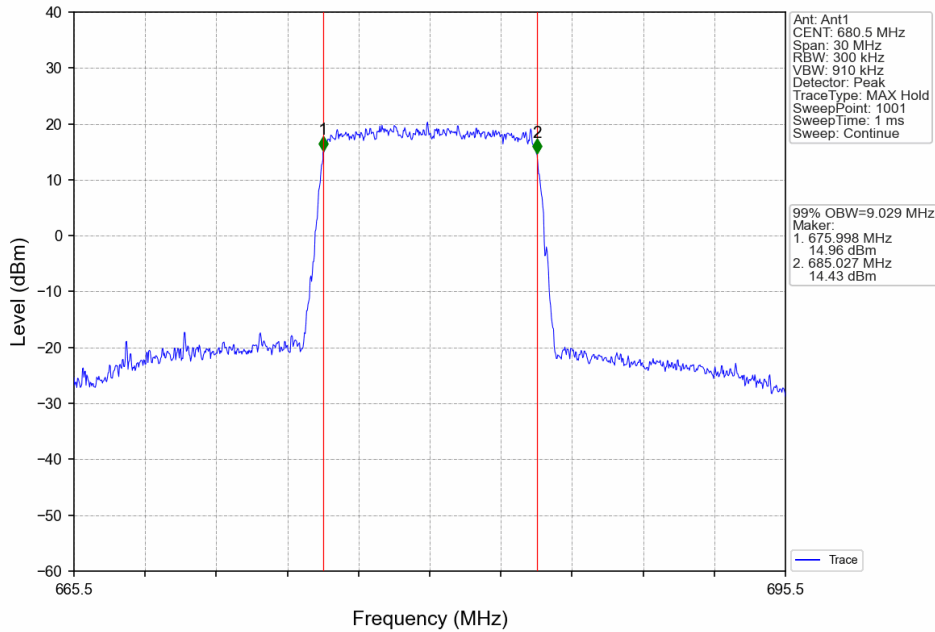
Band71_10MHz_16QAM_MCH_680.5MHz_RB_50_0_NTNV
