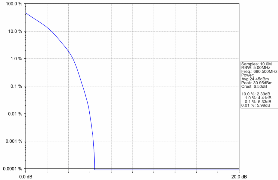
Band71_5MHz_QPSK_MCH_680.5MHz_RB_25_0_NTNV
