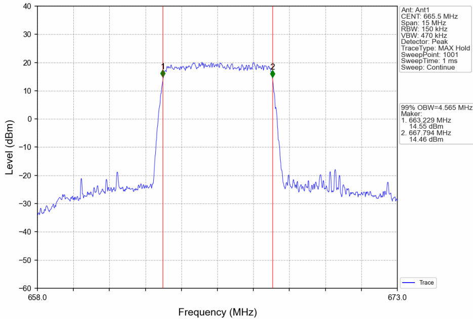
Band71_5MHz_16QAM_LCH_665.5MHz_RB_25_0_NTNV
