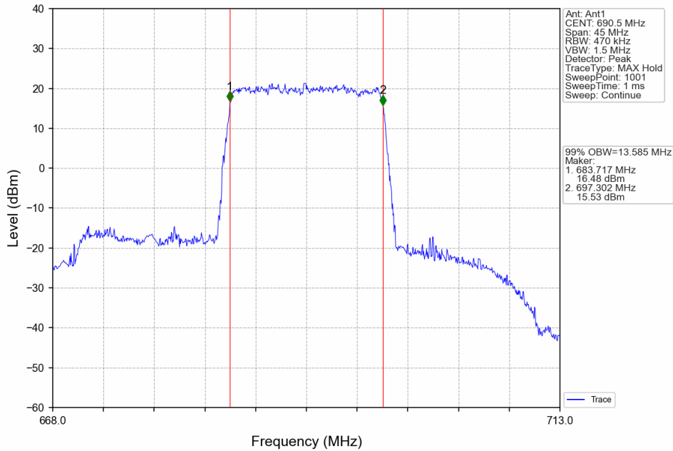
Band71_15MHz_QPSK_HCH_690.5MHz_RB_75_0_NTNV
