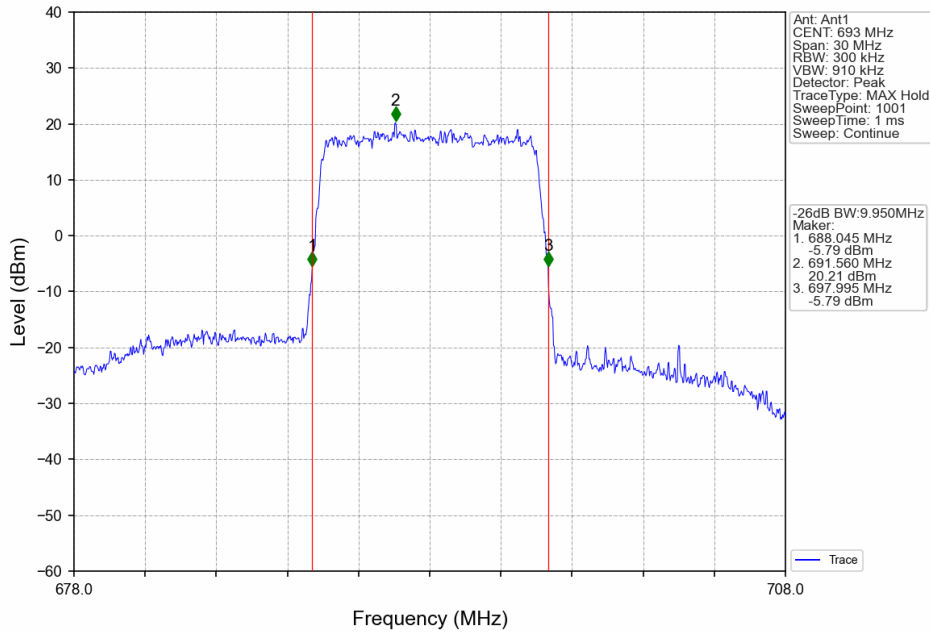
Band71_10MHz_64QAM_HCH_693MHz_RB_50_0_NTNV
