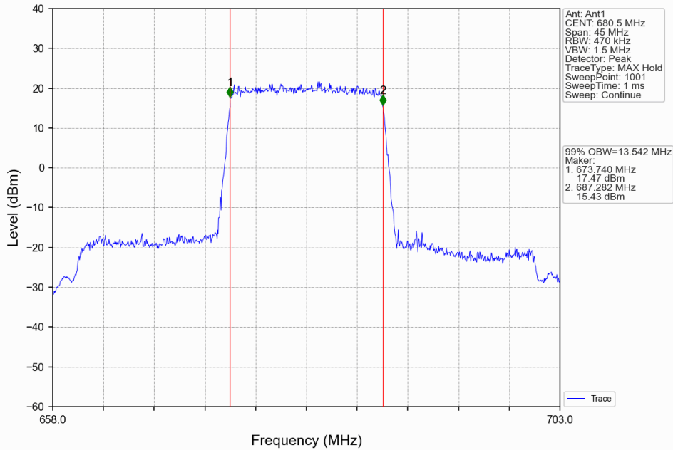
Band71_15MHz_QPSK_MCH_680.5MHz_RB_75_0_NTNV
