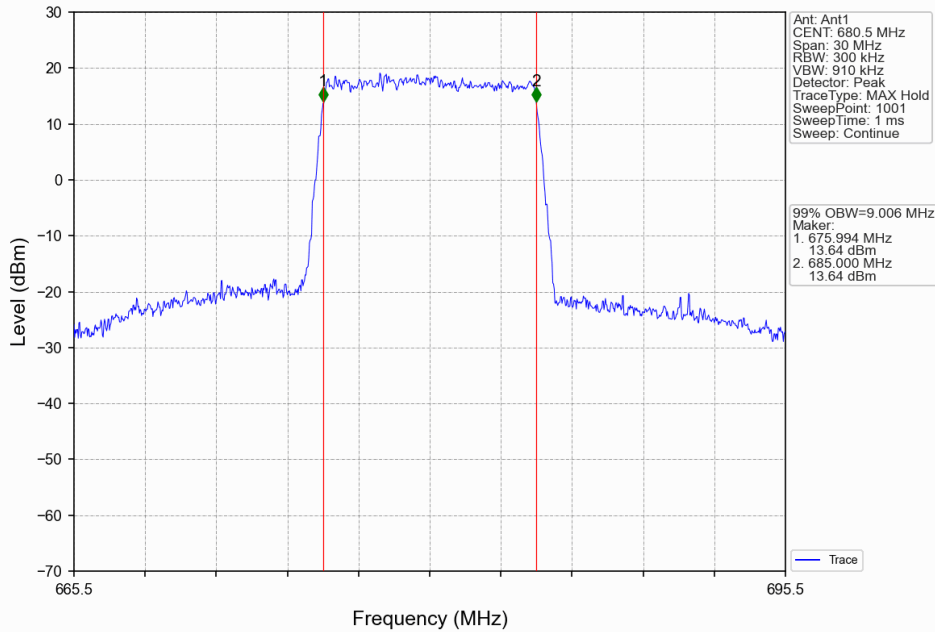
Band71_10MHz_64QAM_MCH_680.5MHz_RB_50_0_NTNV
