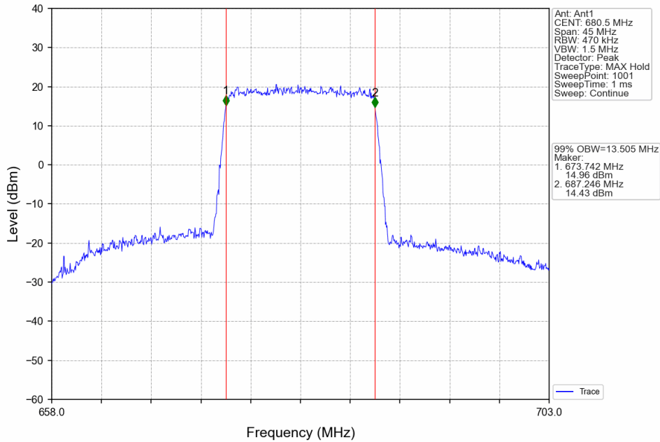
Band71_15MHz_16QAM_MCH_680.5MHz_RB_75_0_NTNV
