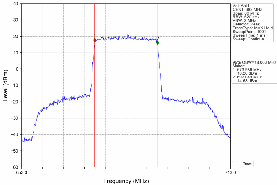
Band71_20MHz_16QAM_MCH_683MHz_RB_100_0_NTNV
