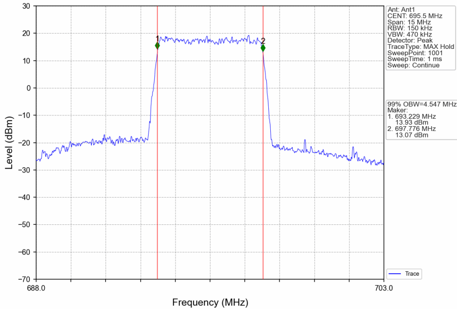
Band71_5MHz_64QAM_HCH_695.5MHz_RB_25_0_NTNV
