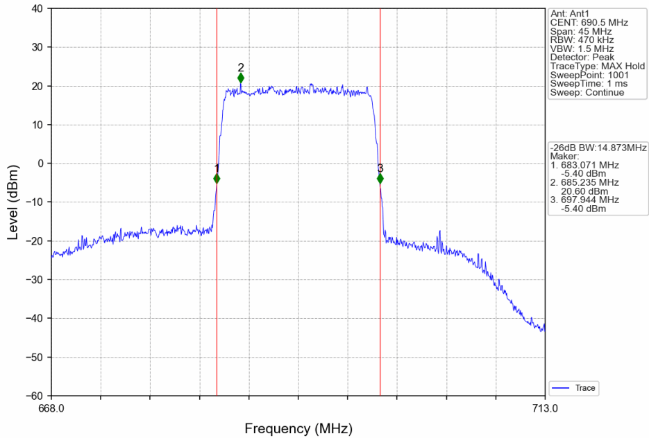
Band71_15MHz_16QAM_HCH_690.5MHz_RB_75_0_NTNV
