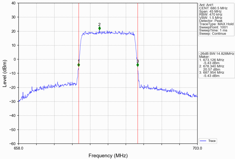
Band71_15MHz_16QAM_MCH_680.5MHz_RB_75_0_NTNV
