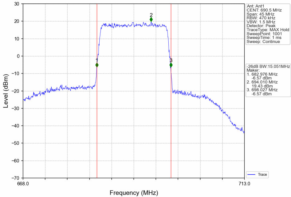
Band71_15MHz_64QAM_HCH_690.5MHz_RB_75_0_NTNV
