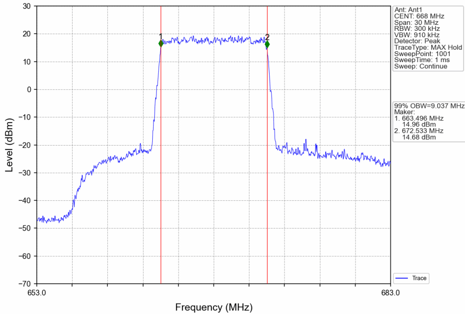
Band71_10MHz_64QAM_LCH_668MHz_RB_50_0_NTNV
