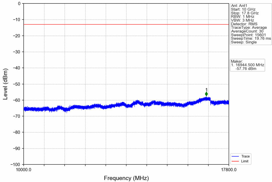
Band66_15MHz_64QAM_HCH_1772.5MHz_RB_1_0_NTNV
