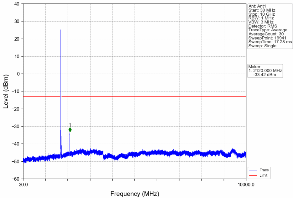
Band66_15MHz_QPSK_LCH_1717.5MHz_RB_1_0_NTNV
