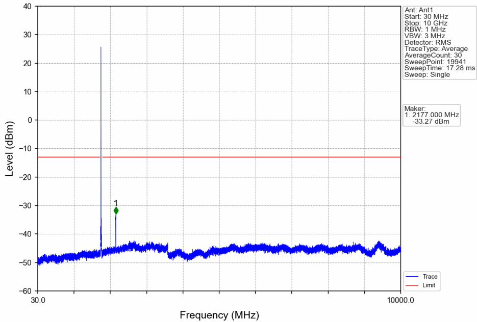
Band66_15MHz_QPSK_HCH_1772.5MHz_RB_1_0_NTNV
