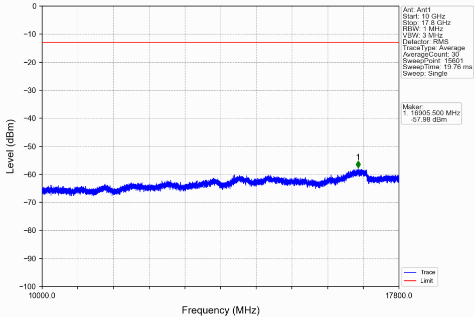
Band66_15MHz_QPSK_LCH_1717.5MHz_RB_1_0_NTNV
