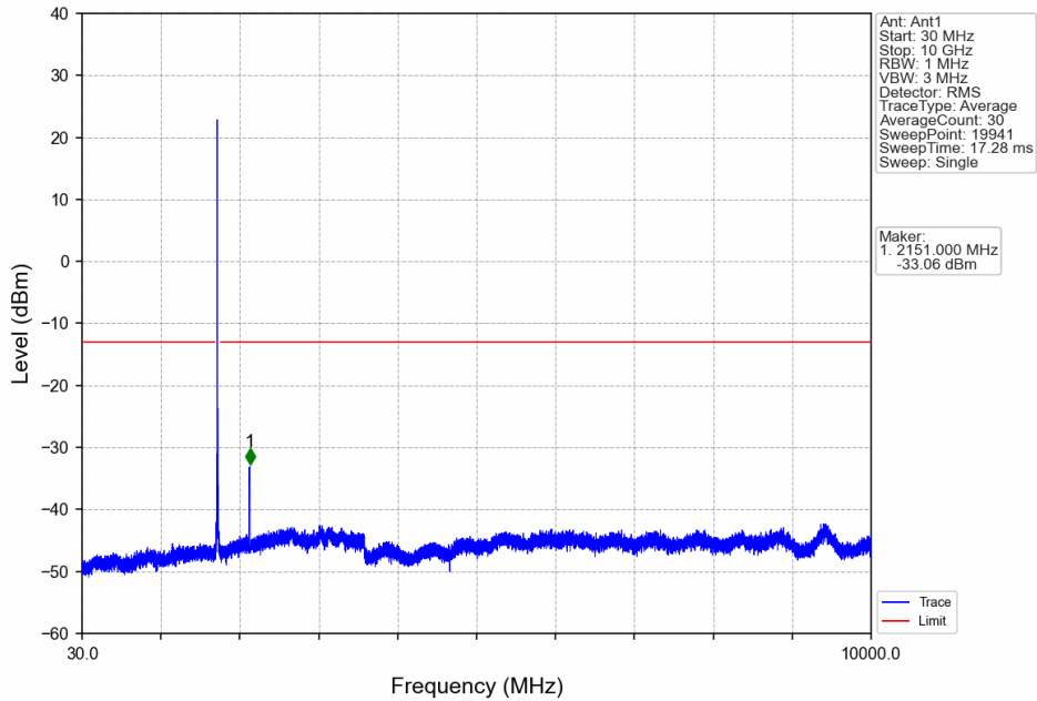
Band66_15MHz_64QAM_MCH_1745MHz_RB_1_0_NTNV
