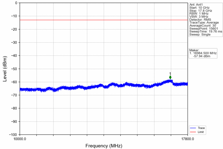
Band66_15MHz_16QAM_MCH_1745MHz_RB_1_0_NTNV
