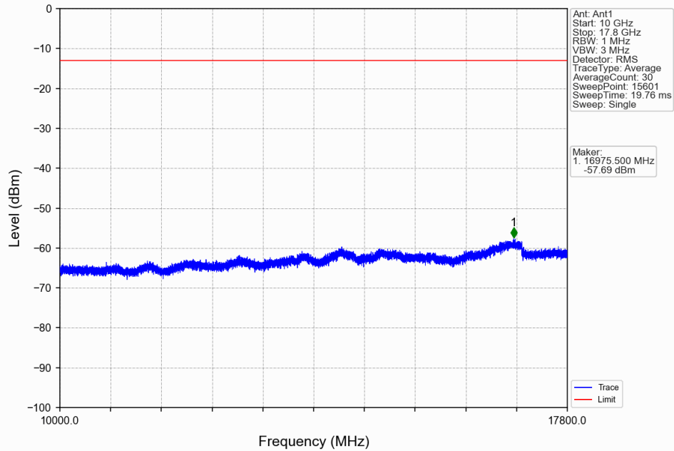
Band66_20MHz_64QAM_MCH_1745MHz_RB_1_0_NTNV
