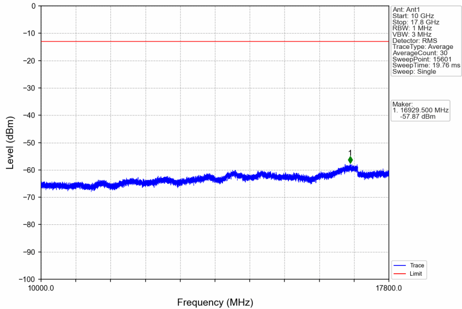
Band66_10MHz_64QAM_HCH_1775MHz_RB_1_0_NTNV
