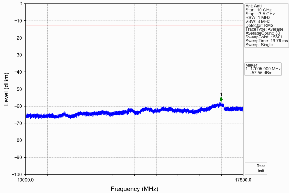
Band66_15MHz_64QAM_MCH_1745MHz_RB_1_0_NTNV
