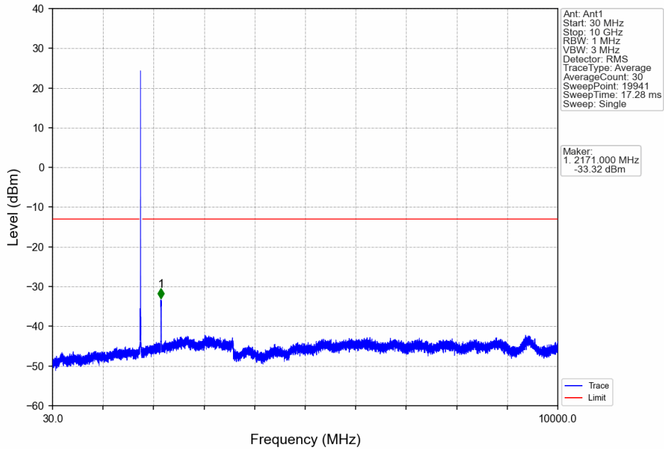
Band66_15MHz_64QAM_HCH_1772.5MHz_RB_1_0_NTNV
