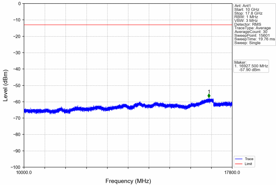
Band66_20MHz_64QAM_LCH_1720MHz_RB_1_0_NTNV
