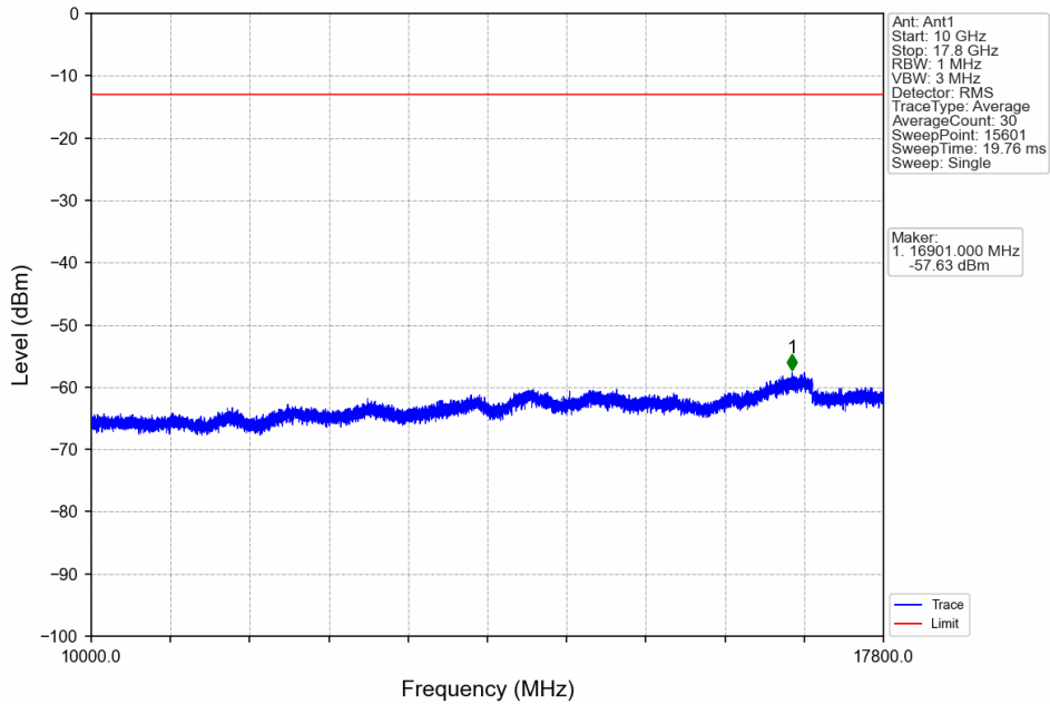
Band66_10MHz_16QAM_LCH_1715MHz_RB_1_0_NTNV
