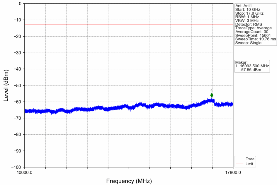
Band66_1.4MHz_64QAM_MCH_1745MHz_RB_1_0_NTNV
