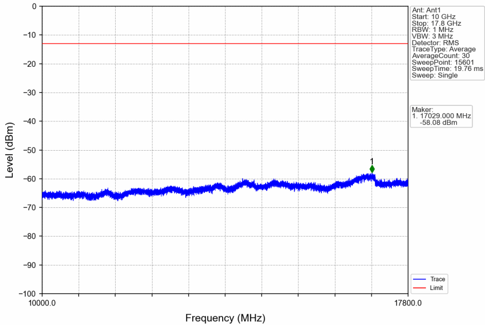
Band66_3MHz_64QAM_HCH_1778.5MHz_RB_1_0_NTNV
