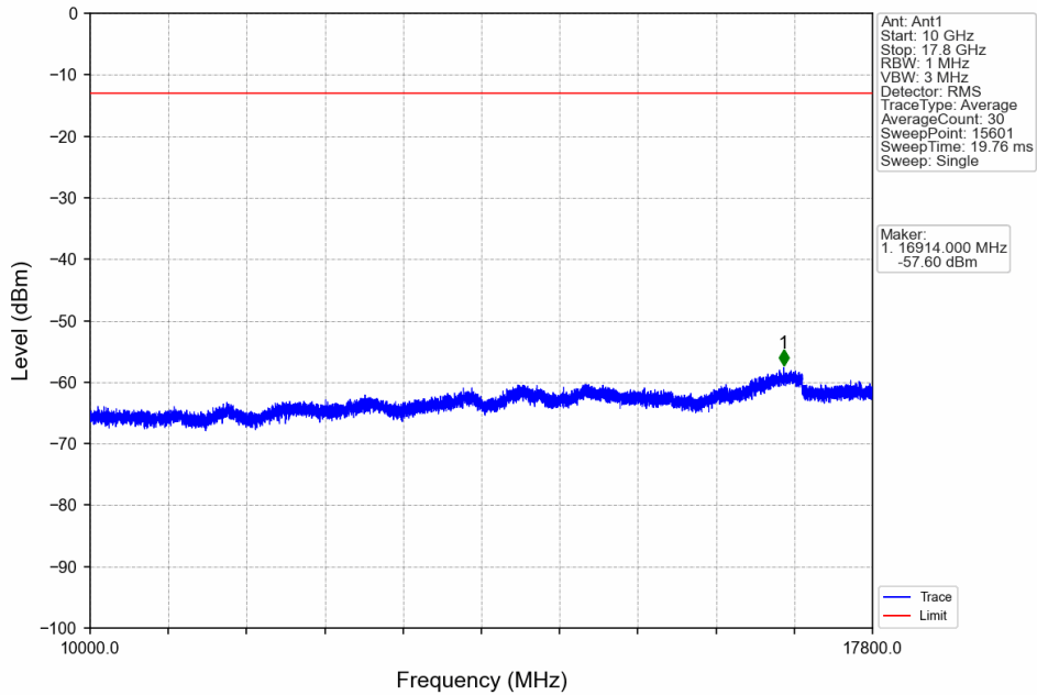
Band66_3MHz_64QAM_MCH_1745MHz_RB_1_0_NTNV
