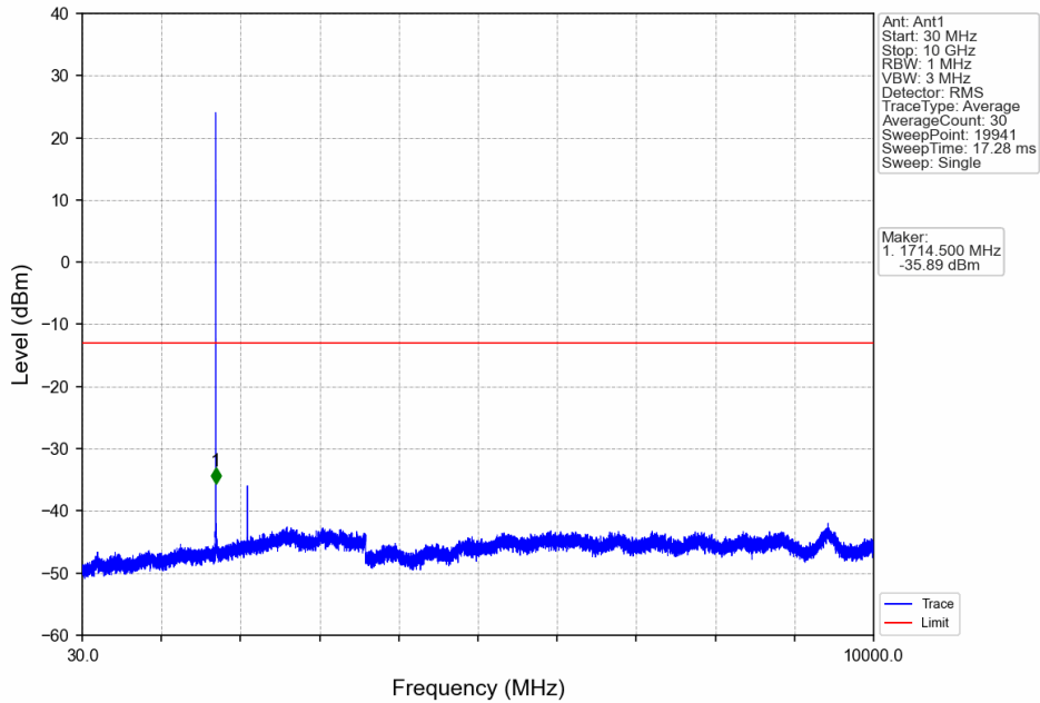
Band66_1.4MHz_64QAM_LCH_1710.7MHz_RB_1_0_NTNV
