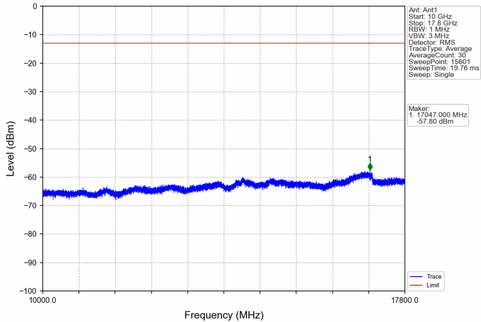
Band66_10MHz_16QAM_MCH_1745MHz_RB_1_0_NTNV
