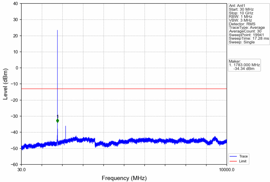
Band66_1.4MHz_64QAM_HCH_1779.3MHz_RB_1_0_NTNV
