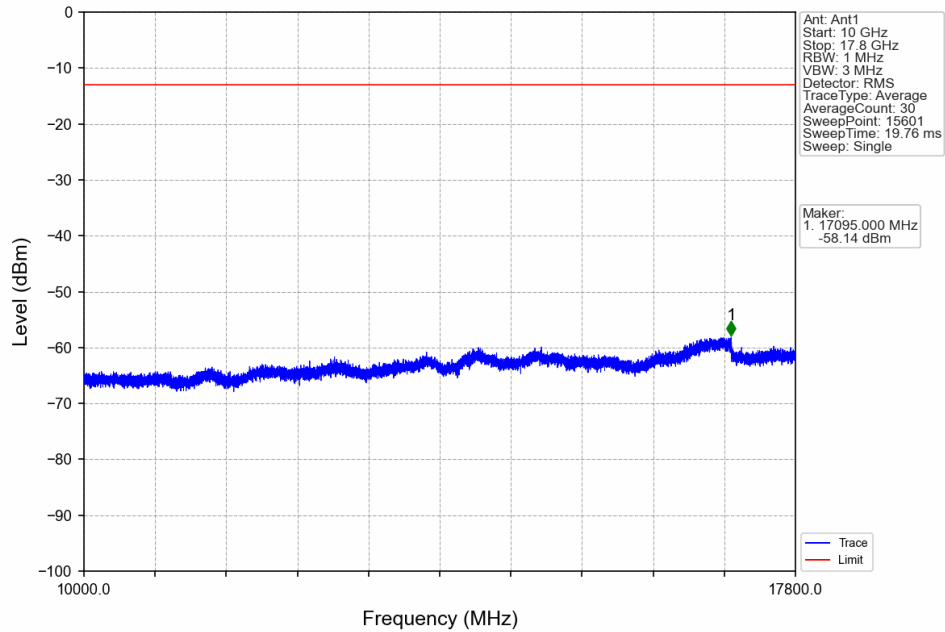
Band66_5MHz_QPSK_MCH_1745MHz_RB_1_0_NTNV
