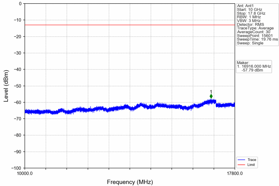
Band66_10MHz_64QAM_MCH_1745MHz_RB_1_0_NTNV
