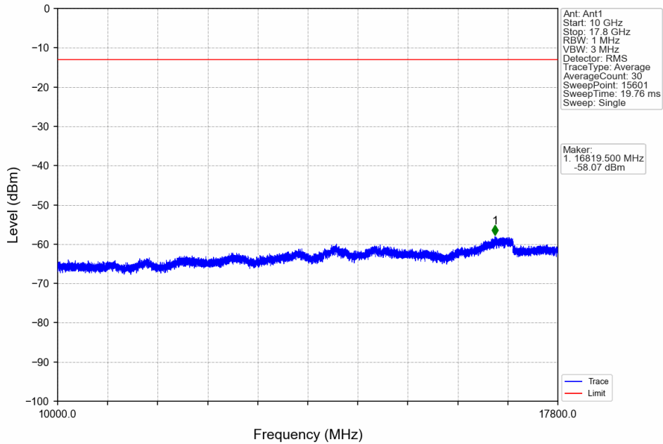
Band66_5MHz_16QAM_MCH_1745MHz_RB_1_0_NTNV
