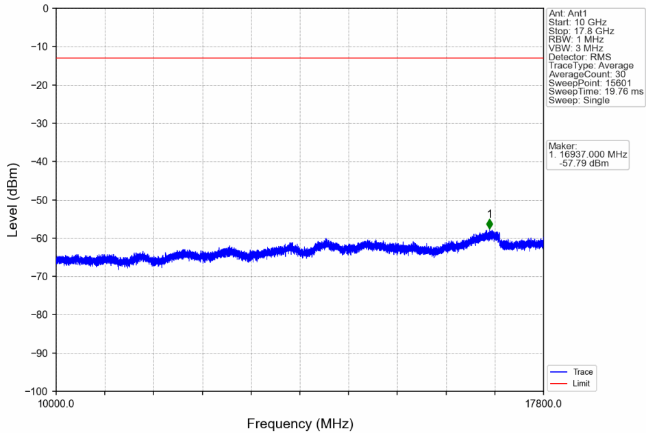
Band66_5MHz_64QAM_LCH_1712.5MHz_RB_1_0_NTNV
