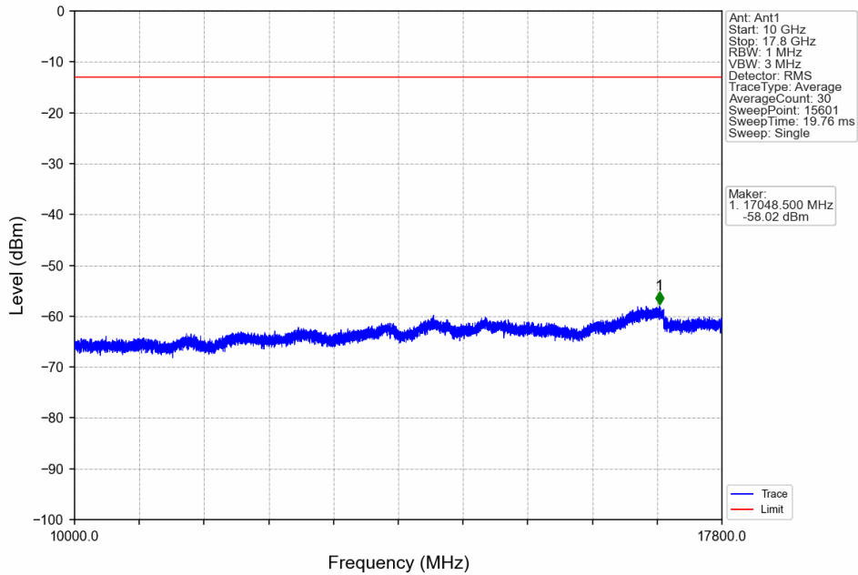
Band66_10MHz_64QAM_LCH_1715MHz_RB_1_0_NTNV
