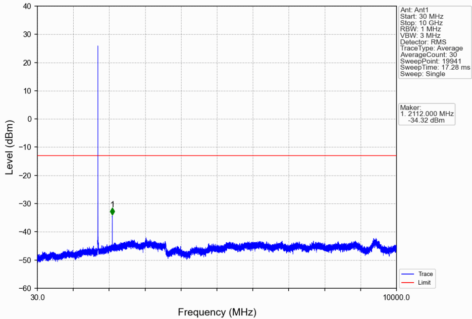
Band66_5MHz_QPSK_LCH_1712.5MHz_RB_1_0_NTNV
