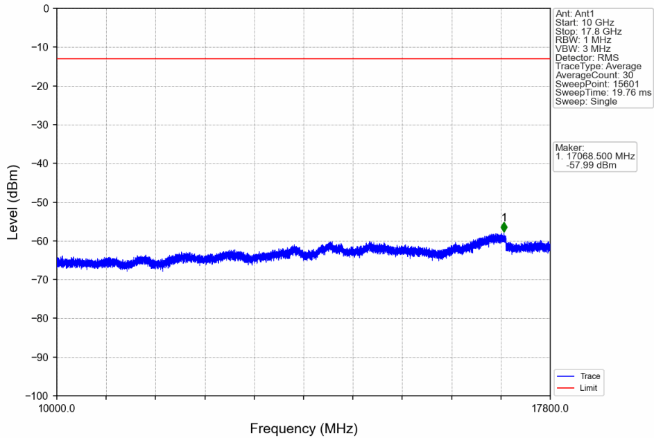
Band66_3MHz_QPSK_HCH_1778.5MHz_RB_1_0_NTNV
