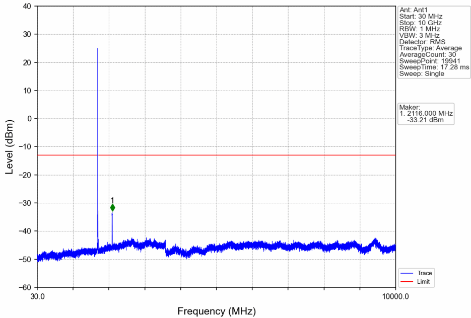
Band66_10MHz_QPSK_LCH_1715MHz_RB_1_0_NTNV
