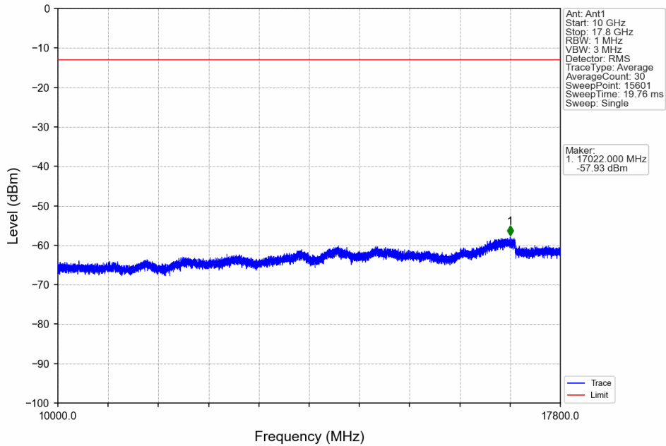
Band66_3MHz_16QAM_LCH_1711.5MHz_RB_1_0_NTNV
