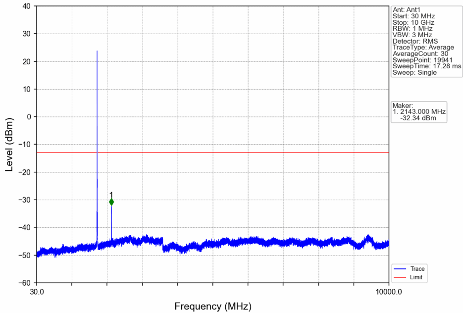
Band66_10MHz_16QAM_MCH_1745MHz_RB_1_0_NTNV
