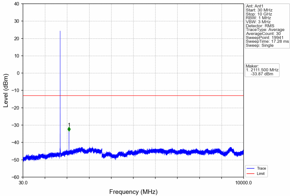
Band66_3MHz_16QAM_LCH_1711.5MHz_RB_1_0_NTNV
