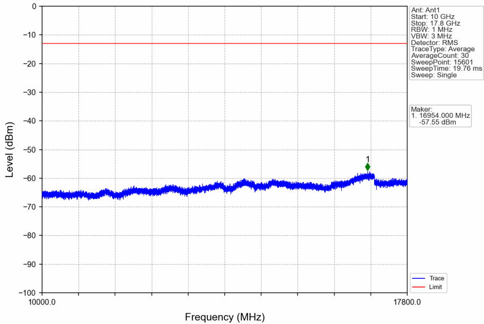
Band66_10MHz_QPSK_MCH_1745MHz_RB_1_0_NTNV
