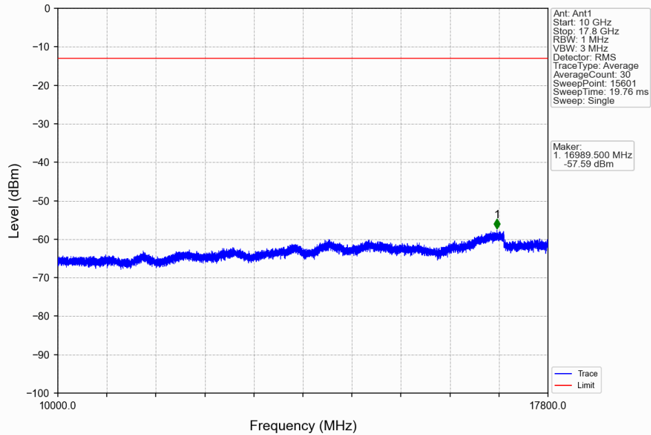
Band66_1.4MHz_64QAM_HCH_1779.3MHz_RB_1_0_NTNV
