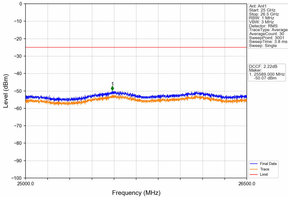
Band41_15MHz_16QAM_HCH_2682.5MHz_RB_1_0_NTNV
