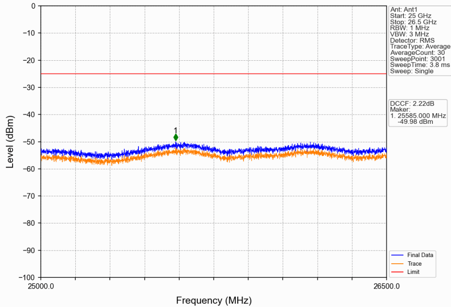
Band41_20MHz_16QAM_LCH_2506MHz_RB_100_0_NTNV
