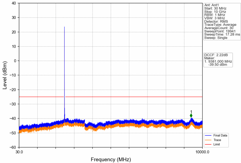
Band41_20MHz_64QAM_LCH_2506MHz_RB_1_0_NTNV
