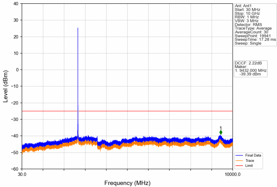
Band41_15MHz_16QAM_HCH_2682.5MHz_RB_1_0_NTNV
