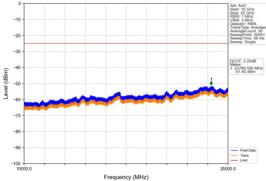
Band41_15MHz_64QAM_HCH_2682.5MHz_RB_1_0_NTNV
