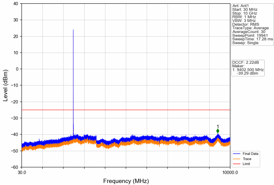
Band41_10MHz_64QAM_LCH_2501MHz_RB_1_0_NTNV
