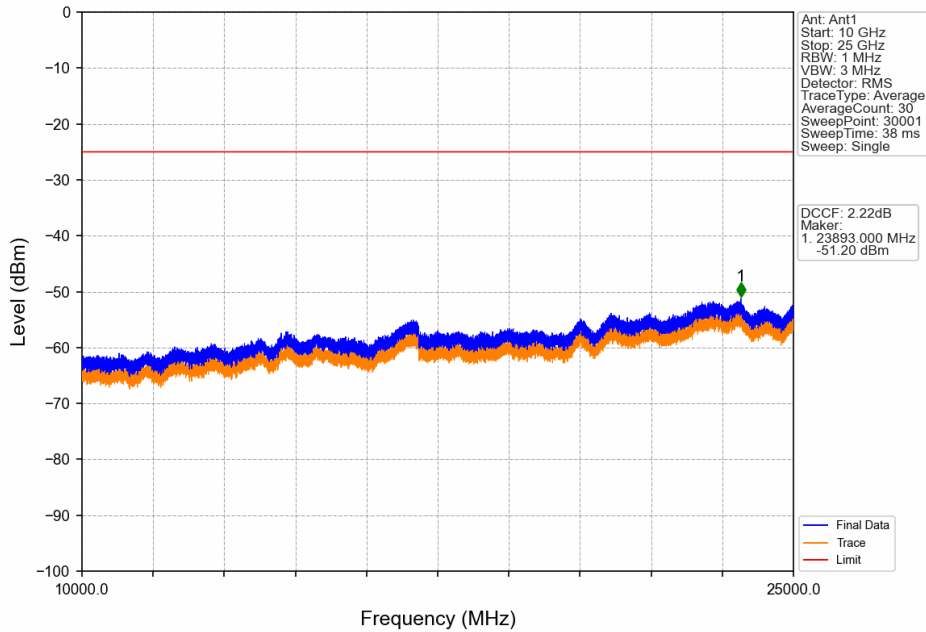
Band41_20MHz_16QAM_HCH_2680MHz_RB_1_0_NTNV
