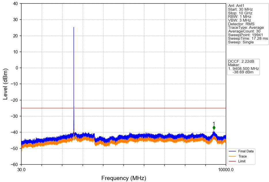
Band41_15MHz_16QAM_MCH_2593MHz_RB_1_0_NTNV
