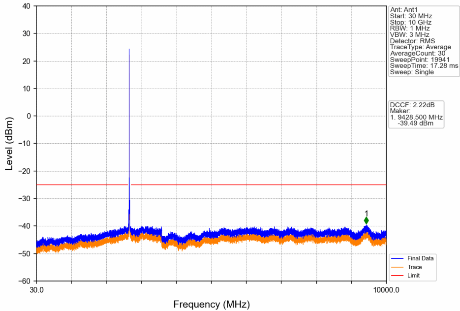
Band41_20MHz_16QAM_HCH_2680MHz_RB_1_0_NTNV
