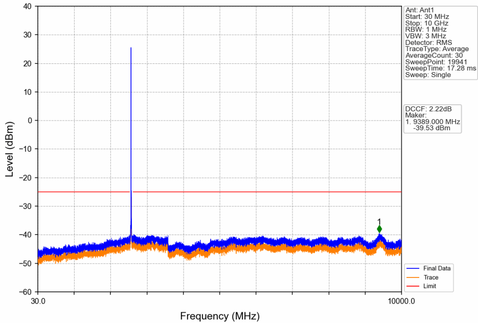
Band41_20MHz_64QAM_MCH_2593MHz_RB_1_0_NTNV
