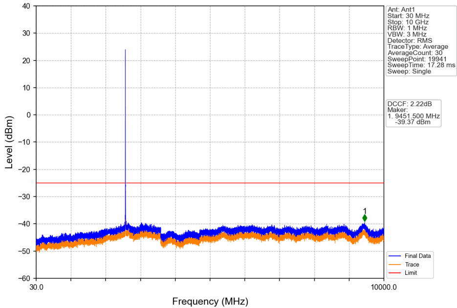
Band41_10MHz_64QAM_MCH_2593MHz_RB_1_0_NTNV
