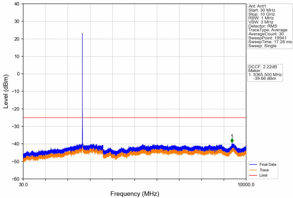
Band41_15MHz_64QAM_HCH_2682.5MHz_RB_1_0_NTNV
