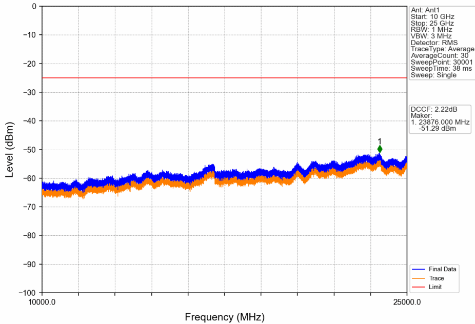
Band41_15MHz_64QAM_LCH_2503.5MHz_RB_1_0_NTNV
