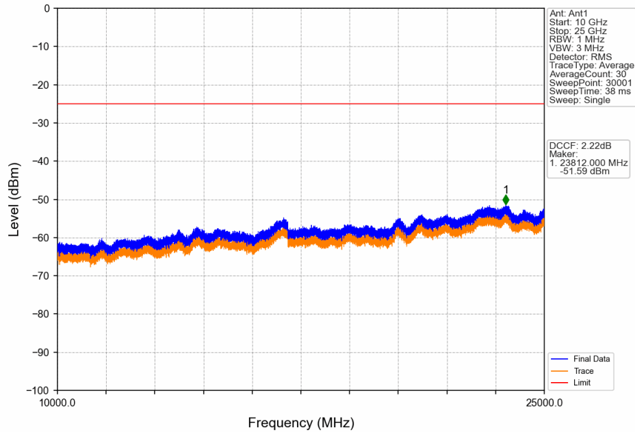
Band41_20MHz_64QAM_MCH_2593MHz_RB_1_0_NTNV
