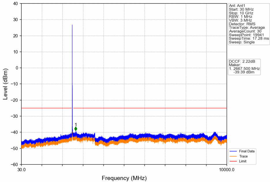
Band41_20MHz_16QAM_LCH_2506MHz_RB_1_0_NTNV
