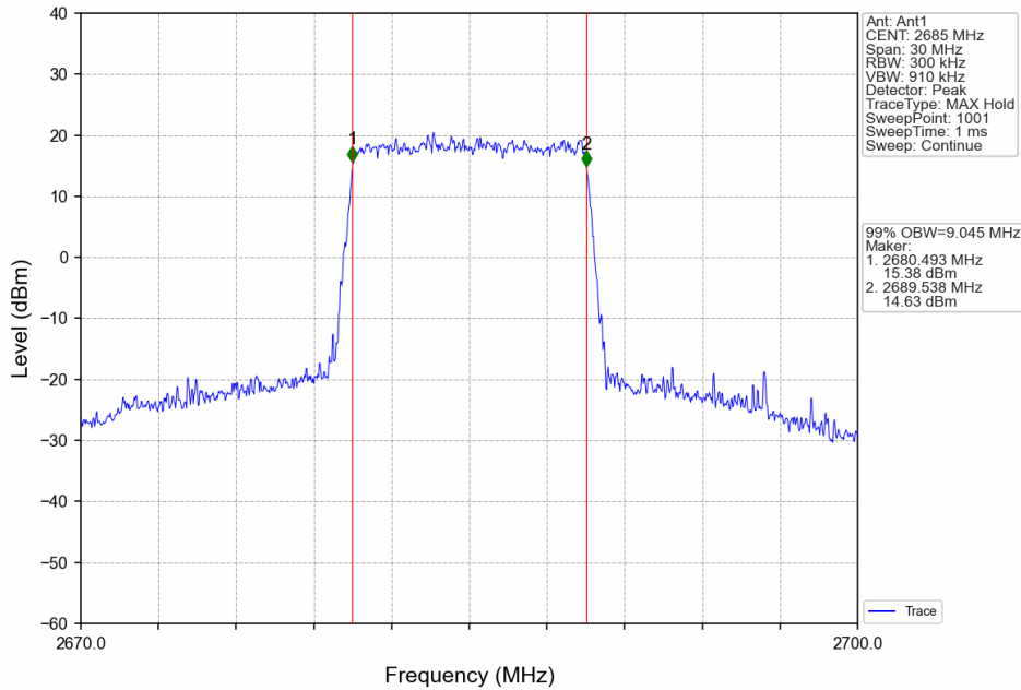
Band41_10MHz_64QAM_HCH_2685MHz_RB_50_0_NTNV
