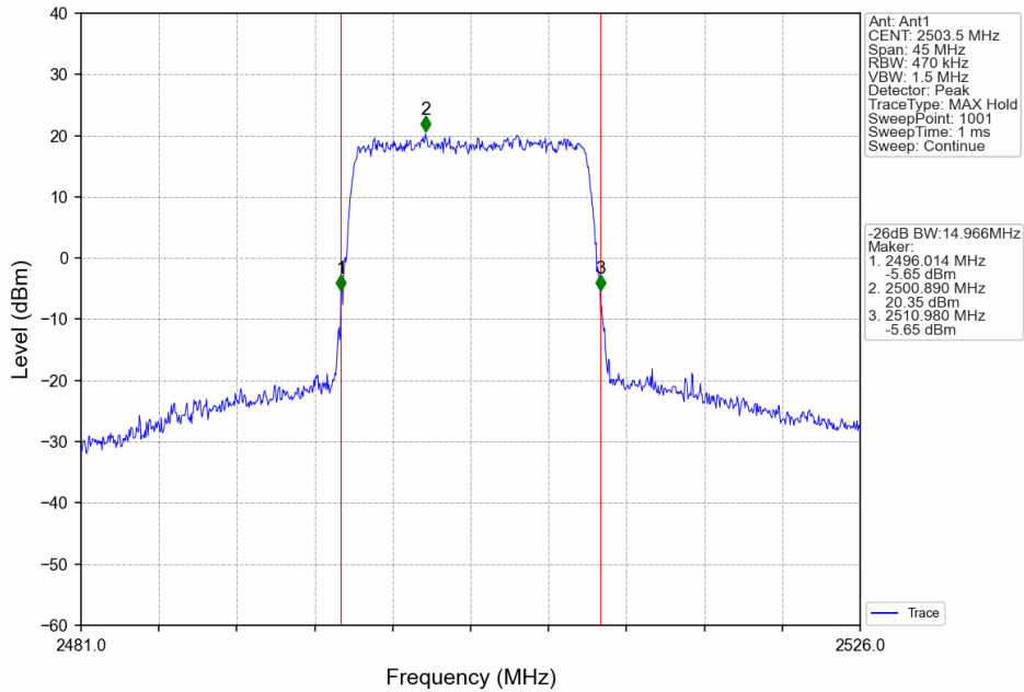
Band41_15MHz_64QAM_LCH_2503.5MHz_RB_75_0_NTNV
