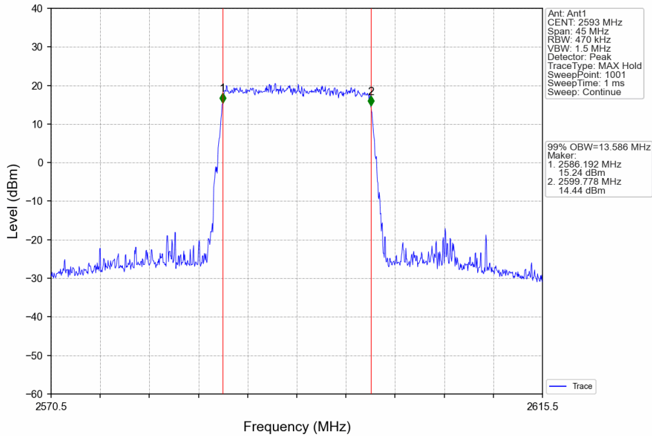
Band41_15MHz_64QAM_MCH_2593MHz_RB_75_0_NTNV
