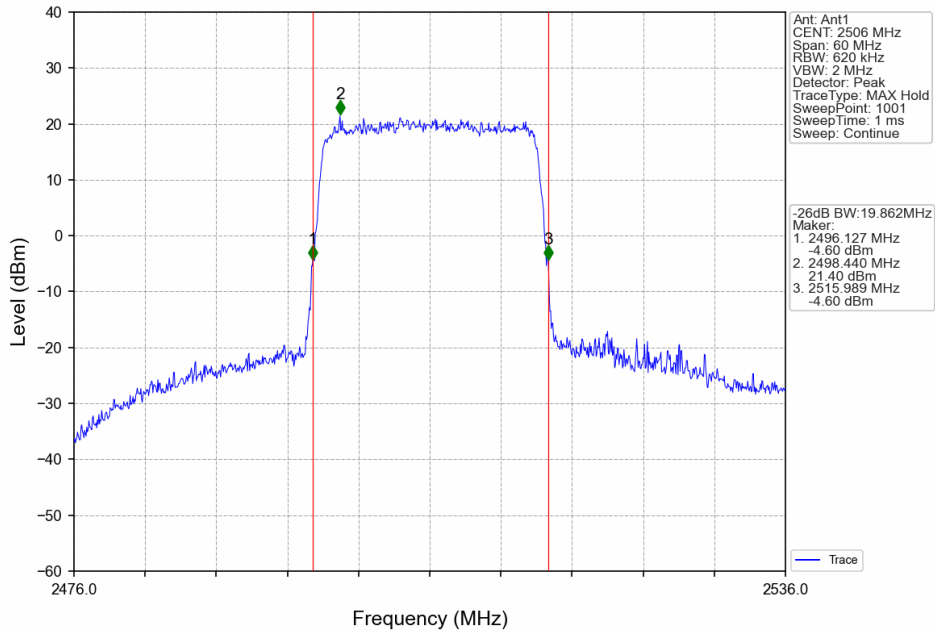
Band41_20MHz_16QAM_LCH_2506MHz_RB_100_0_NTNV
