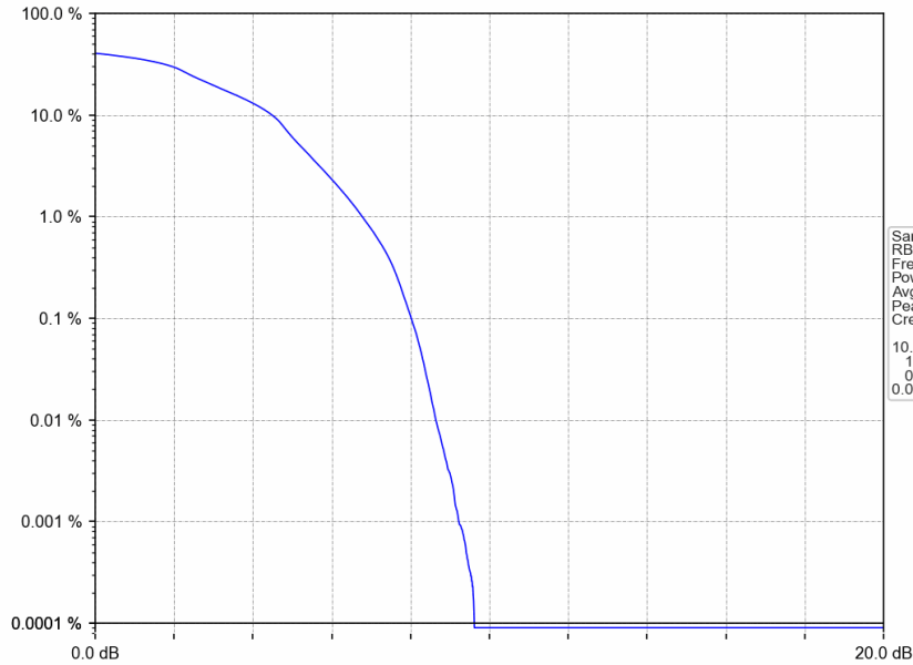
Band41_5MHz_16QAM_LCH_2498.5MHz_RB_25_0_NTNV
