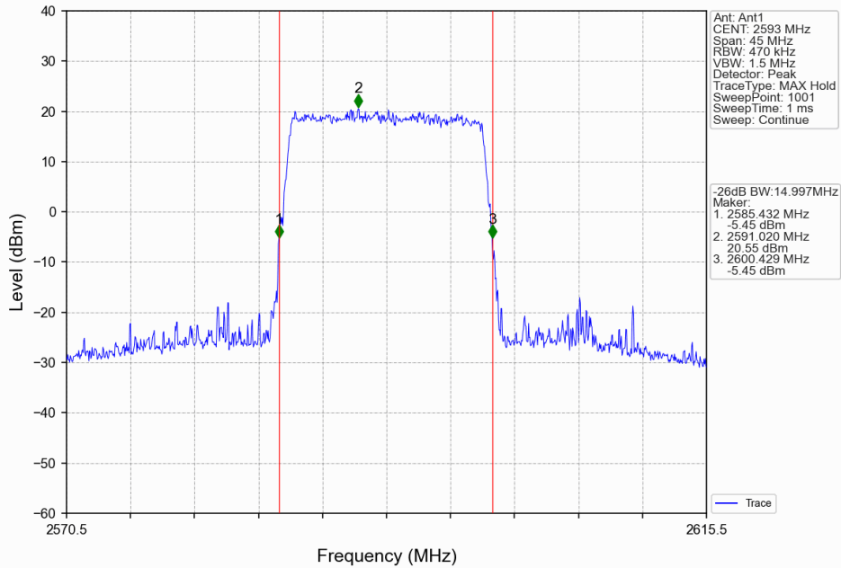
Band41_15MHz_64QAM_MCH_2593MHz_RB_75_0_NTNV
