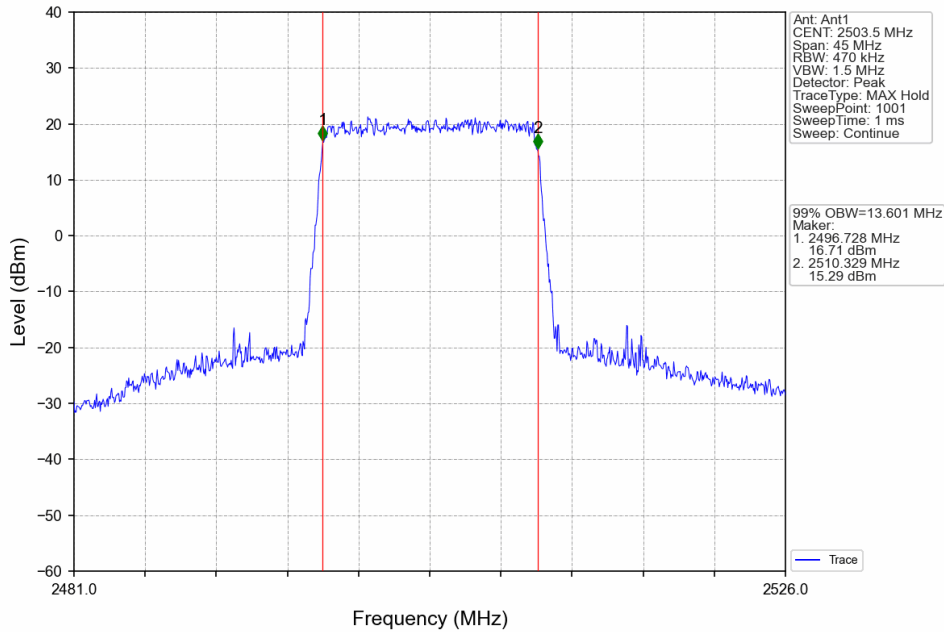
Band41_15MHz_16QAM_LCH_2503.5MHz_RB_75_0_NTNV
