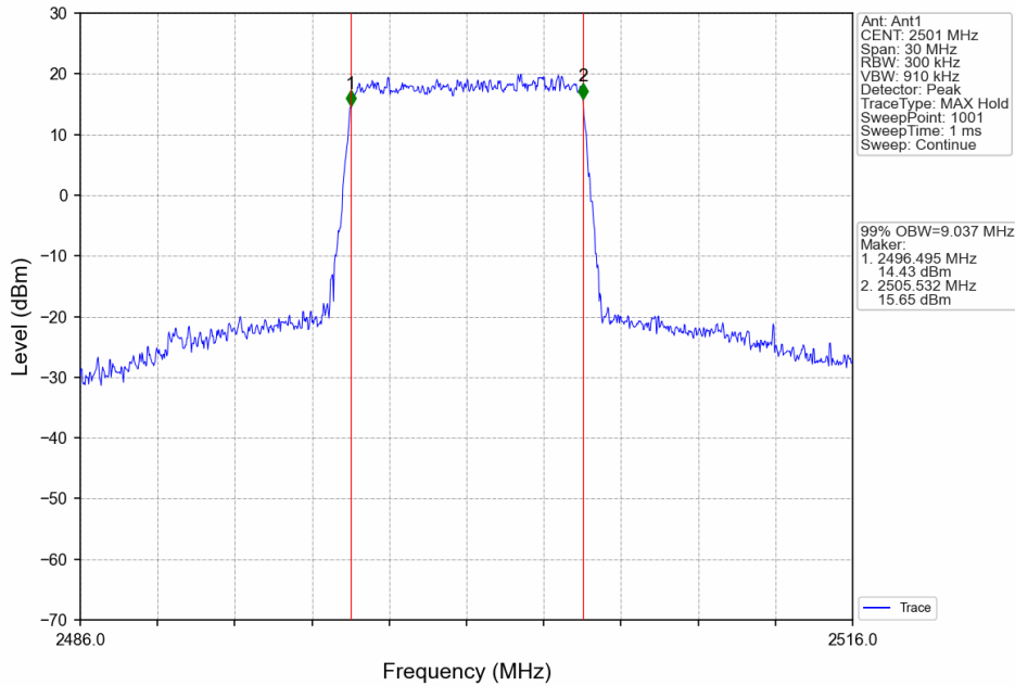
Band41_10MHz_64QAM_LCH_2501MHz_RB_50_0_NTNV
