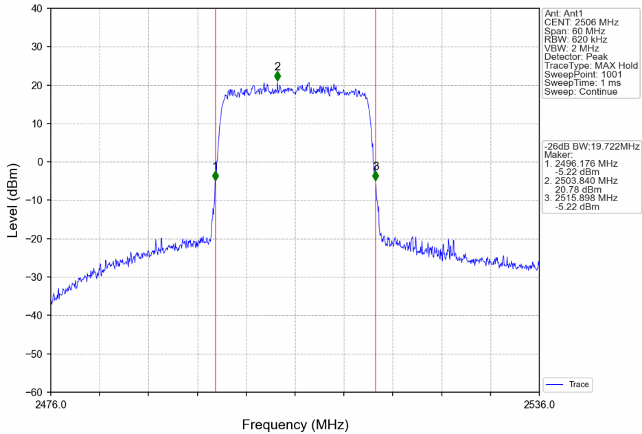
Band41_20MHz_64QAM_LCH_2506MHz_RB_100_0_NTNV
