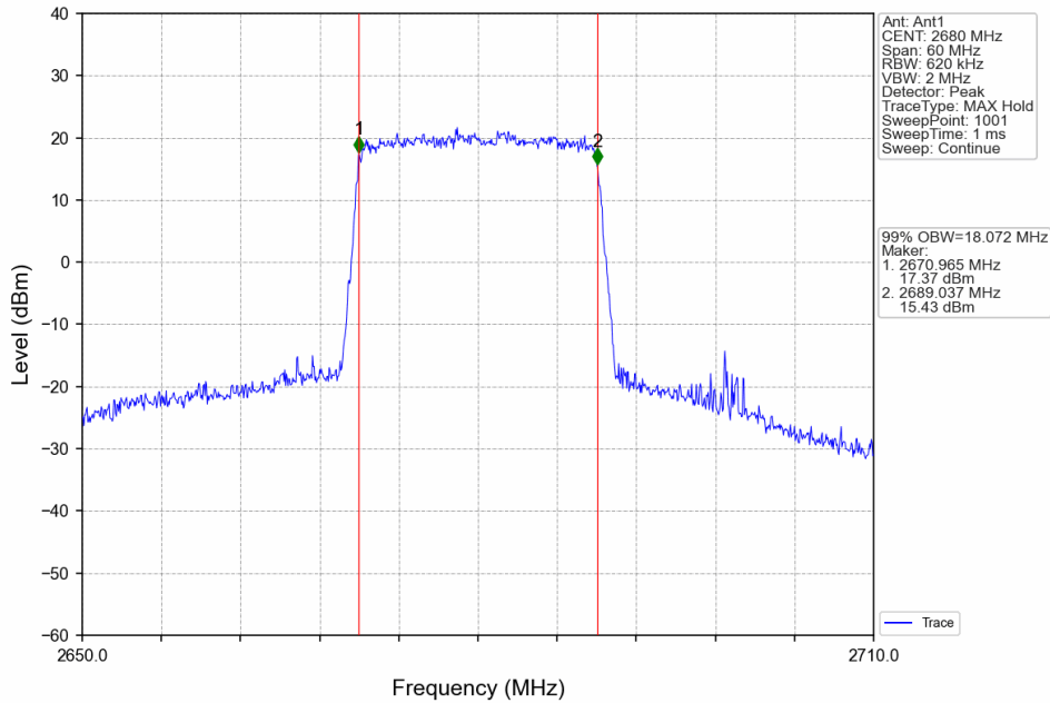
Band41_20MHz_16QAM_HCH_2680MHz_RB_100_0_NTNV
