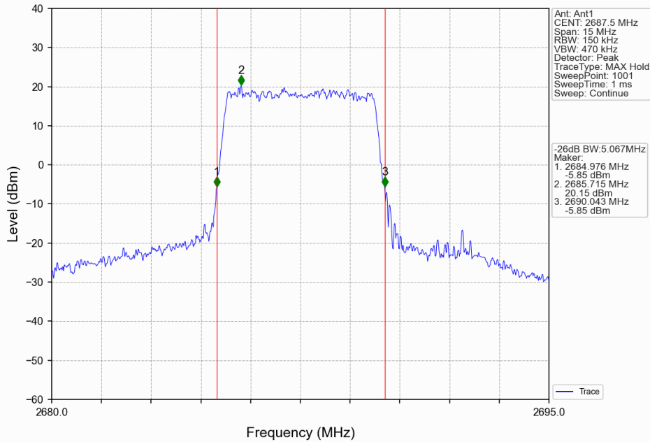
Band41_5MHz_64QAM_HCH_2687.5MHz_RB_25_0_NTNV
