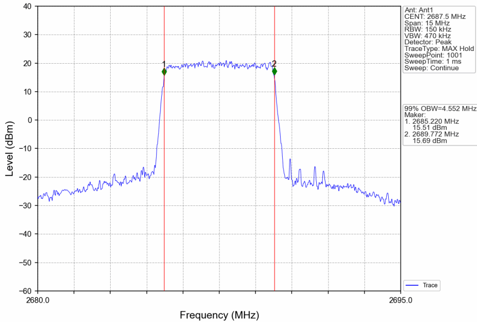
Band41_5MHz_16QAM_HCH_2687.5MHz_RB_25_0_NTNV
