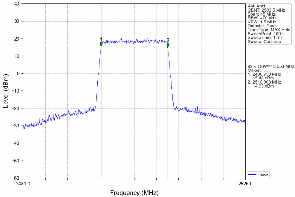
Band41_15MHz_64QAM_LCH_2503.5MHz_RB_75_0_NTNV
