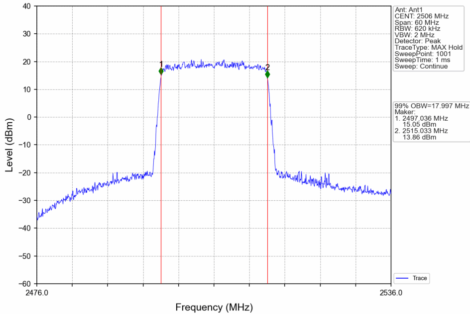
Band41_20MHz_64QAM_LCH_2506MHz_RB_100_0_NTNV
