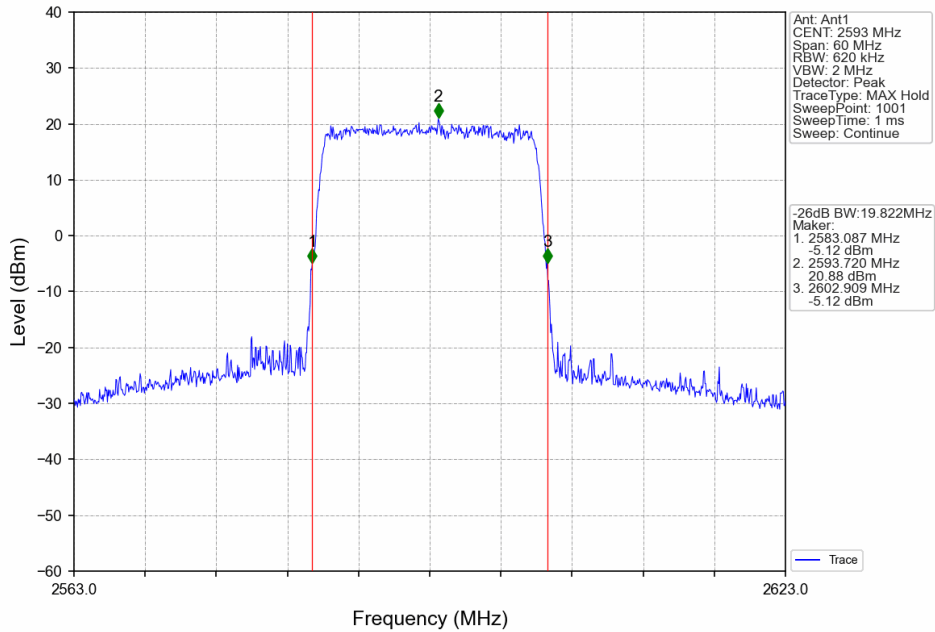
Band41_20MHz_64QAM_MCH_2593MHz_RB_100_0_NTNV
