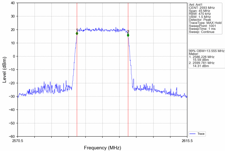
Band41_15MHz_16QAM_MCH_2593MHz_RB_75_0_NTNV
