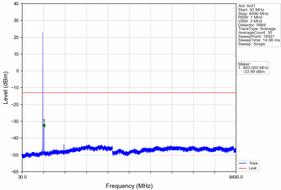
Band26b_10MHz_64QAM_HCH_844MHz_RB_1_0_NTNV
