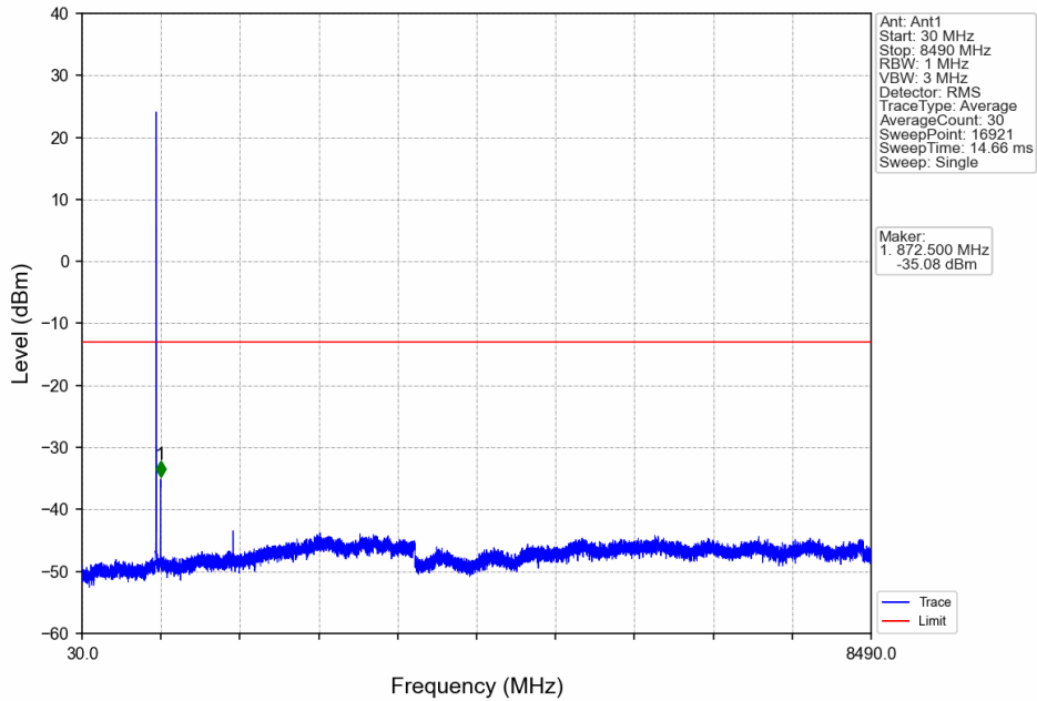
Band26b_5MHz_64QAM_LCH_826.5MHz_RB_1_0_NTNV
