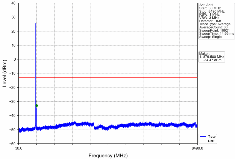
Band26b_10MHz_16QAM_MCH_836.5MHz_RB_1_0_NTNV
