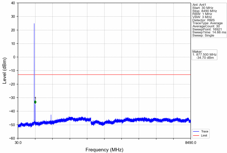
Band26b_10MHz_16QAM_LCH_829MHz_RB_1_0_NTNV
