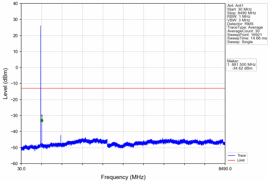
Band26b_5MHz_QPSK_MCH_836.5MHz_RB_1_0_NTNV
