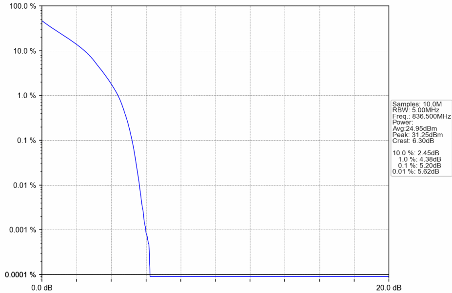
Band26b_3MHz_QPSK_MCH_836.5MHz_RB_15_0_NTNV
