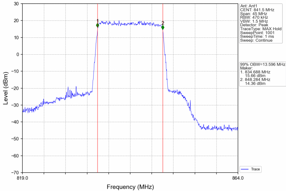
Band26c_15MHz_64QAM_HCH_841.5MHz_RB_75_0_NTNV
