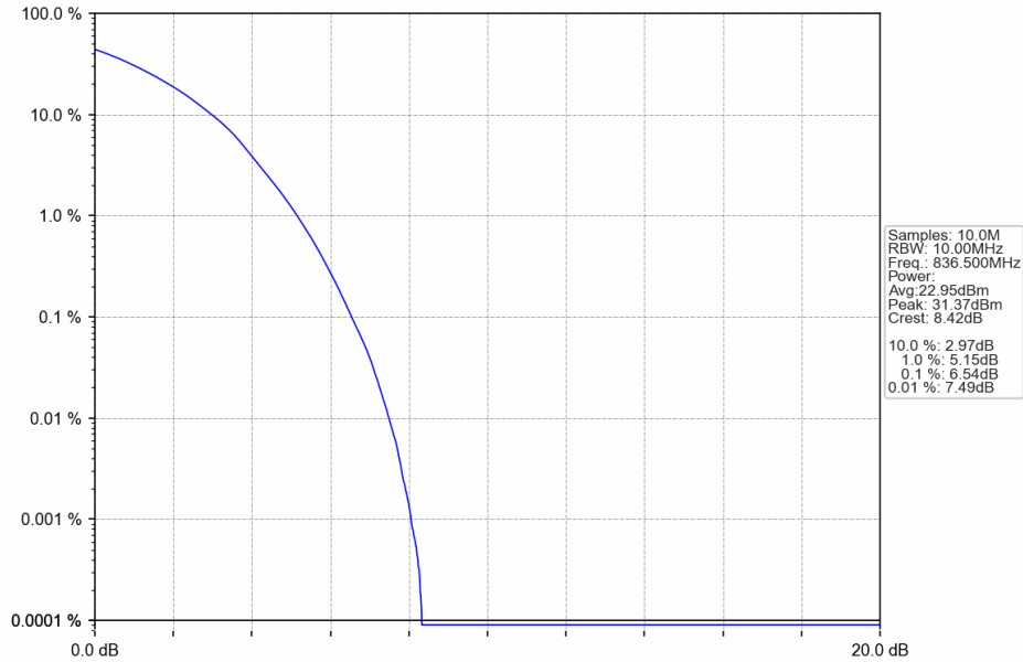
Band26b_10MHz_64QAM_MCH_836.5MHz_RB_50_0_NTNV
