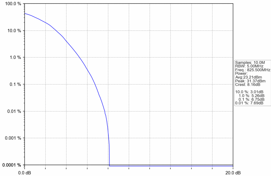
Band26b_3MHz_64QAM_LCH_825.5MHz_RB_15_0_NTNV
