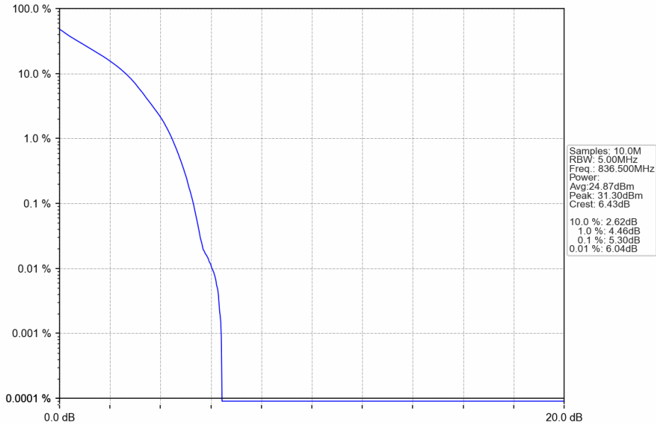
Band26b_1.4MHz_QPSK_MCH_836.5MHz_RB_6_0_NTNV
