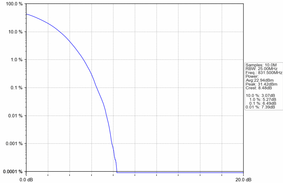
Band26c_15MHz_64QAM_MCH_831.5MHz_RB_75_0_NTNV
