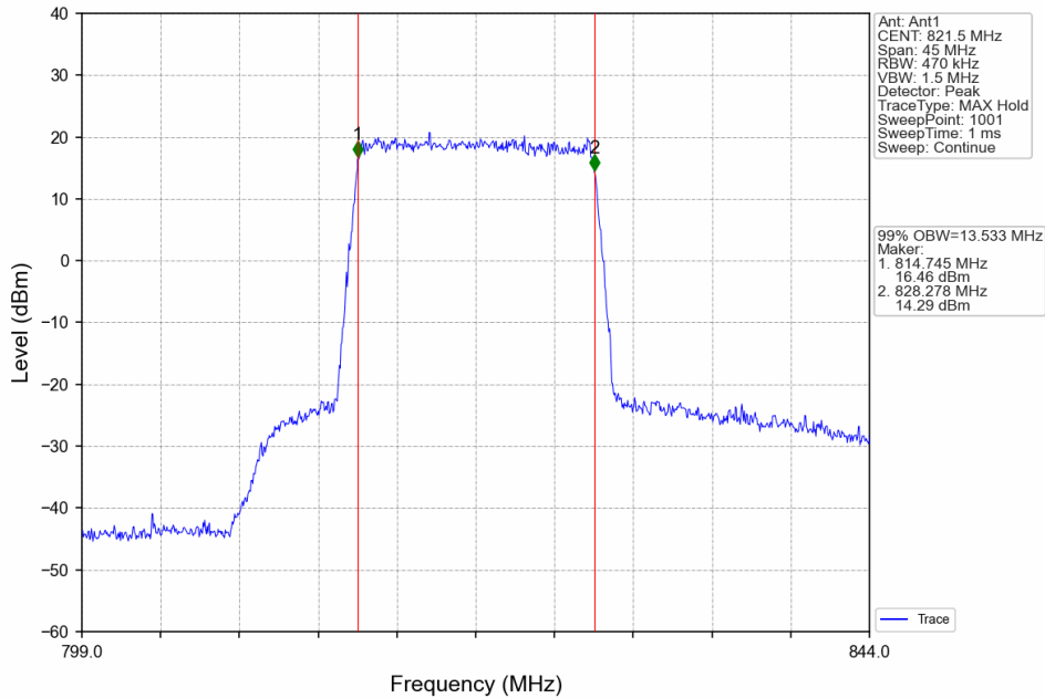
Band26c_15MHz_64QAM_LCH_821.5MHz_RB_75_0_NTNV
