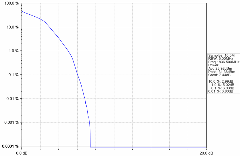
Band26b_1.4MHz_16QAM_MCH_836.5MHz_RB_6_0_NTNV
