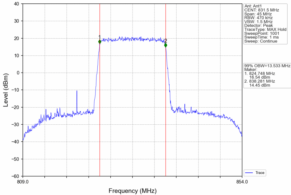
Band26c_15MHz_16QAM_MCH_831.5MHz_RB_75_0_NTNV
