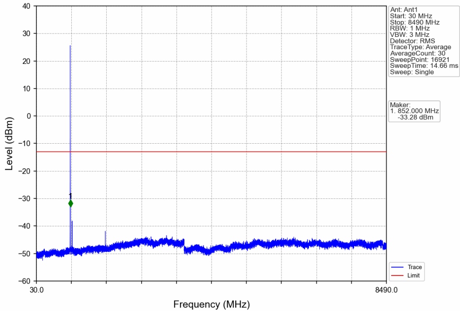
Band26b_1.4MHz_16QAM_HCH_848.3MHz_RB_1_0_NTNV
