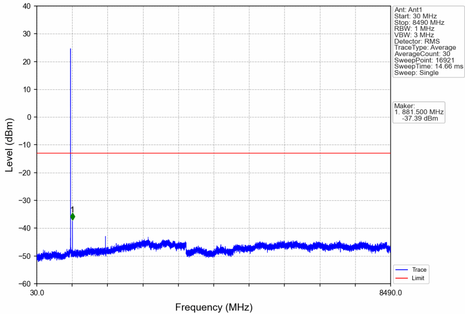
Band26b_1.4MHz_16QAM_MCH_836.5MHz_RB_1_0_NTNV
