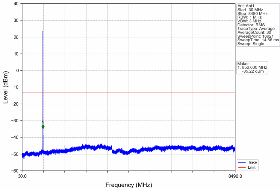
Band26b_1.4MHz_64QAM_HCH_848.3MHz_RB_1_0_NTNV
