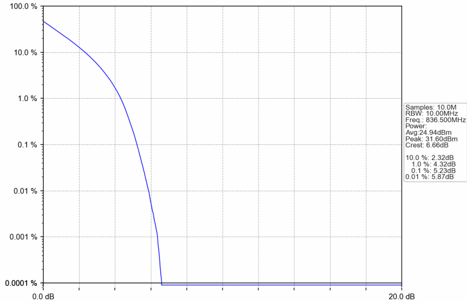
Band26b_10MHz_QPSK_MCH_836.5MHz_RB_50_0_NTNV
