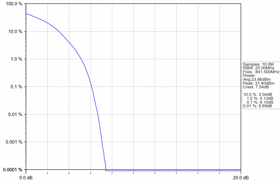
Band26c_15MHz_16QAM_HCH_841.5MHz_RB_75_0_NTNV
