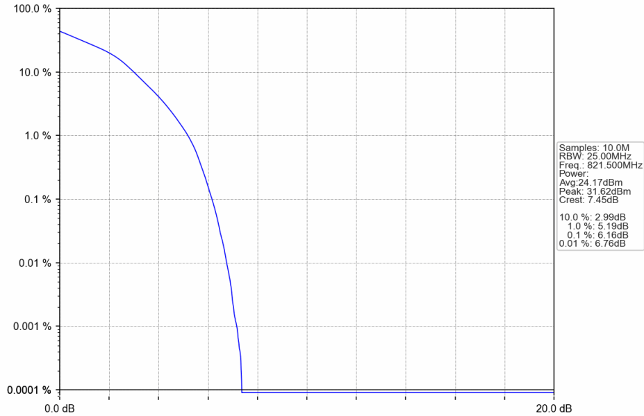
Band26c_15MHz_16QAM_LCH_821.5MHz_RB_75_0_NTNV
