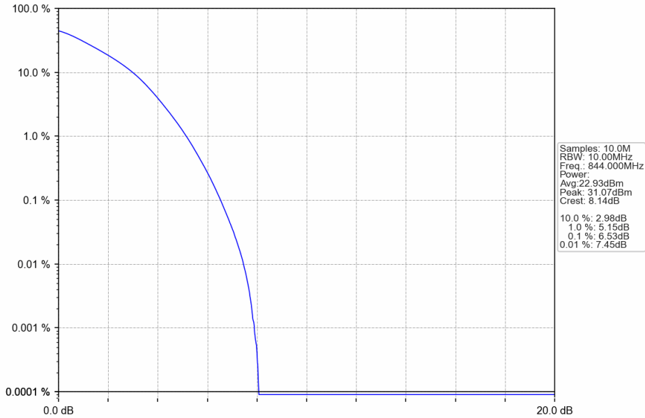
Band26b_10MHz_64QAM_HCH_844MHz_RB_50_0_NTNV
