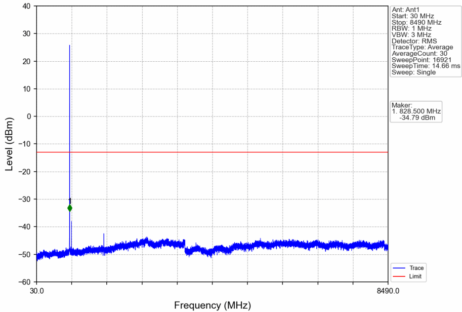
Band26b_1.4MHz_16QAM_LCH_824.7MHz_RB_1_0_NTNV
