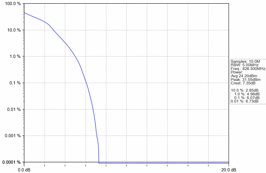
Band26b_5MHz_16QAM_LCH_826.5MHz_RB_25_0_NTNV
