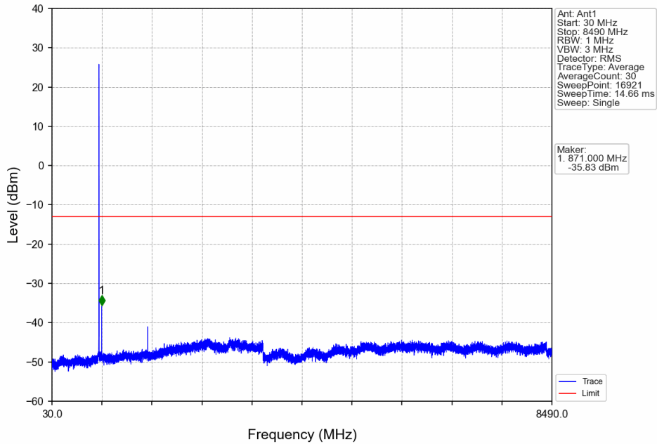
Band26b_3MHz_16QAM_LCH_825.5MHz_RB_1_0_NTNV
