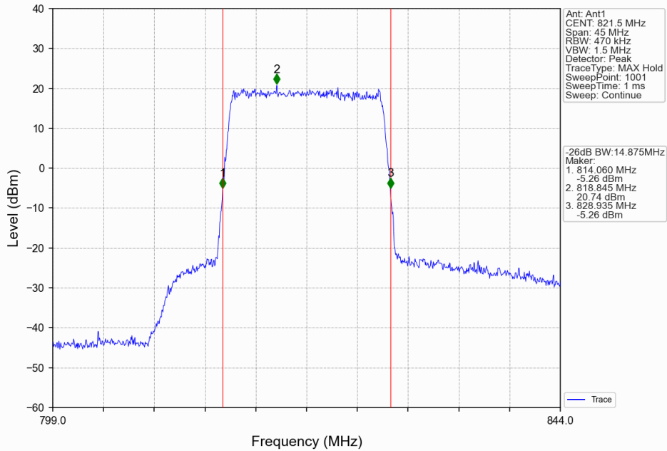
Band26c_15MHz_64QAM_LCH_821.5MHz_RB_75_0_NTNV
