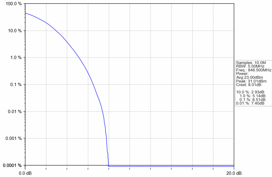
Band26b_5MHz_64QAM_HCH_846.5MHz_RB_25_0_NTNV
