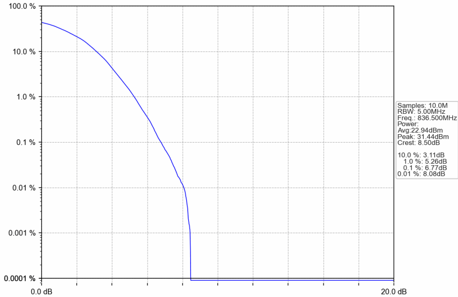
Band26b_1.4MHz_64QAM_MCH_836.5MHz_RB_6_0_NTNV
