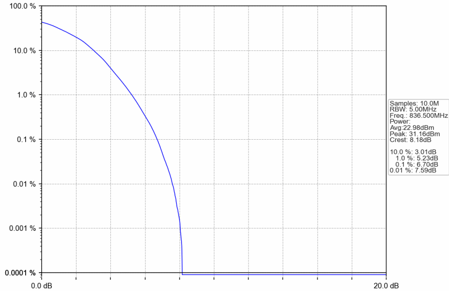
Band26b_3MHz_64QAM_MCH_836.5MHz_RB_15_0_NTNV
