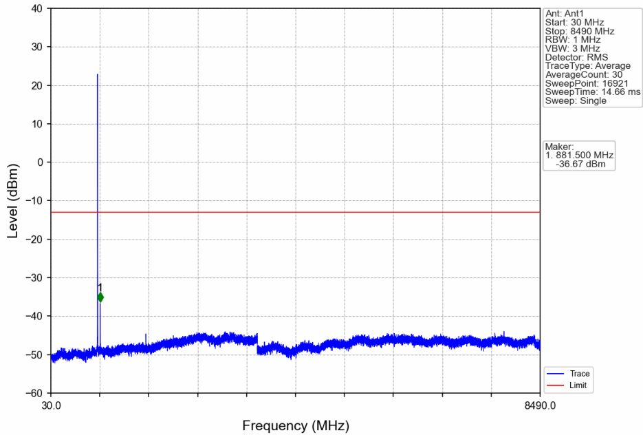
Band26b_1.4MHz_64QAM_MCH_836.5MHz_RB_1_0_NTNV
