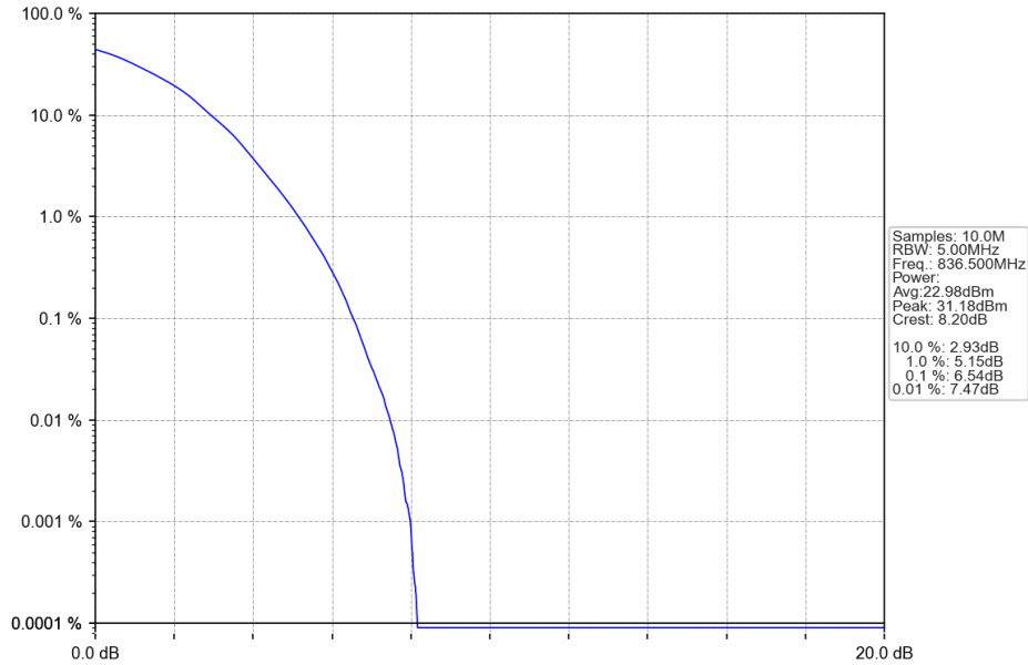
Band26b_5MHz_64QAM_MCH_836.5MHz_RB_25_0_NTNV
