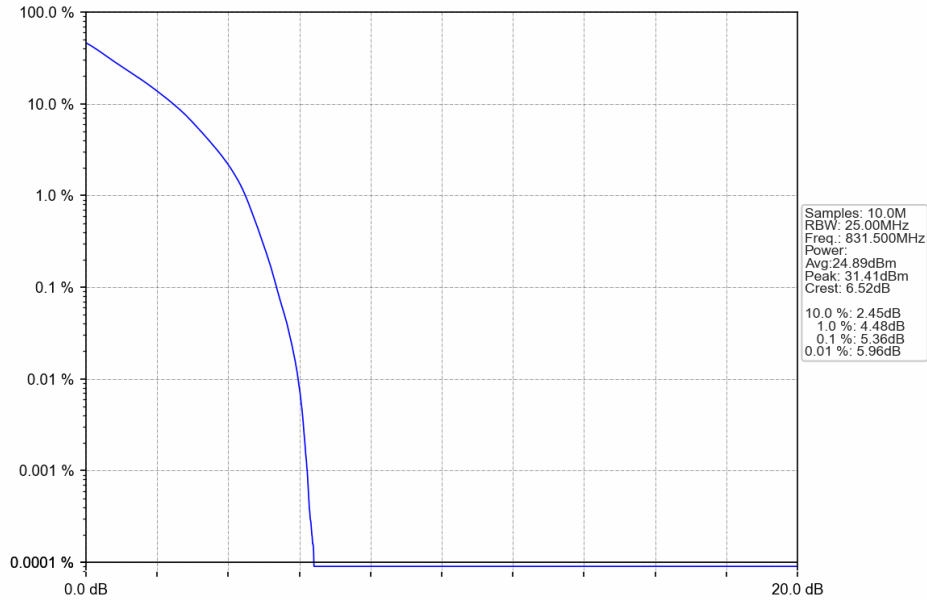
Band26c_15MHz_QPSK_MCH_831.5MHz_RB_75_0_NTNV
