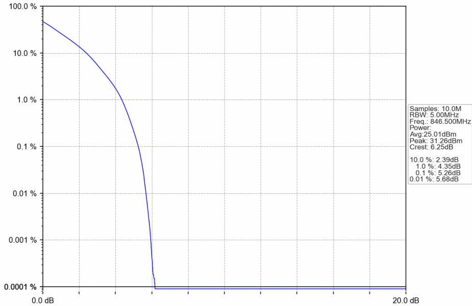
Band26b_5MHz_QPSK_HCH_846.5MHz_RB_25_0_NTNV
