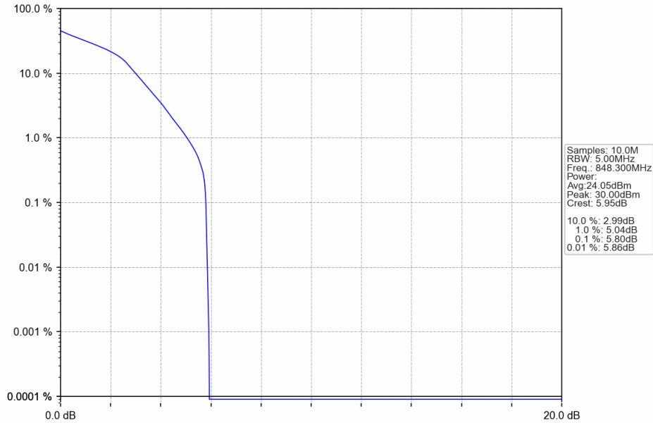
Band26b_1.4MHz_16QAM_HCH_848.3MHz_RB_6_0_NTNV
