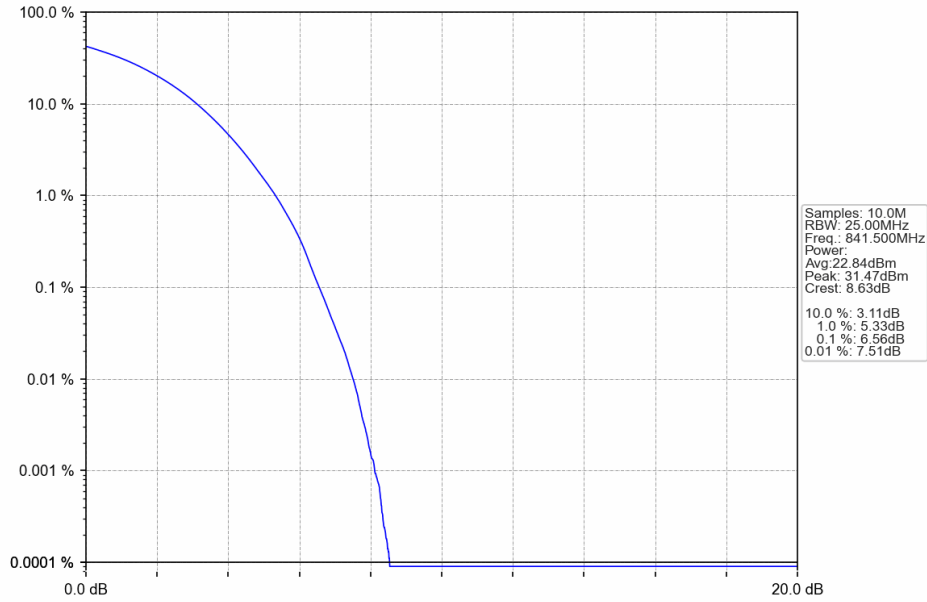
Band26c_15MHz_64QAM_HCH_841.5MHz_RB_75_0_NTNV
