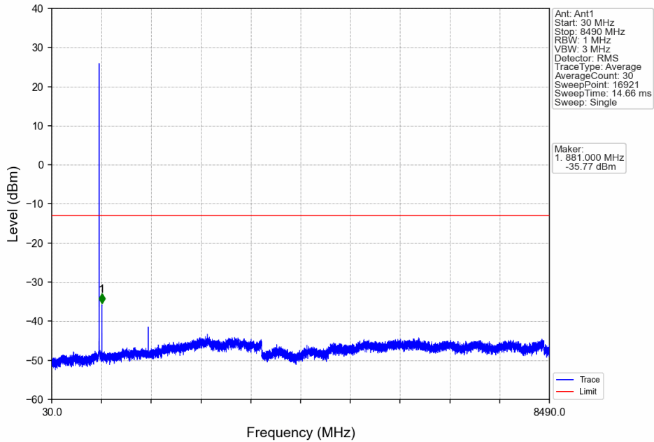
Band26b_3MHz_QPSK_MCH_836.5MHz_RB_1_0_NTNV
