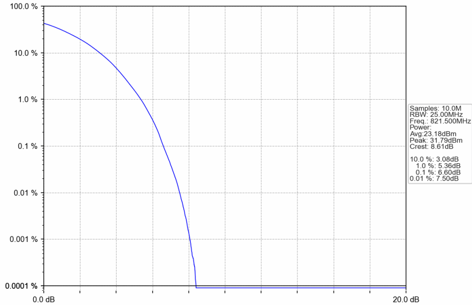
Band26c_15MHz_64QAM_LCH_821.5MHz_RB_75_0_NTNV
