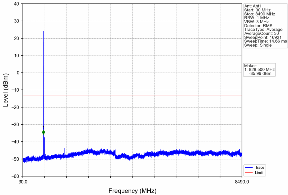
Band26b_1.4MHz_64QAM_LCH_824.7MHz_RB_1_0_NTNV
