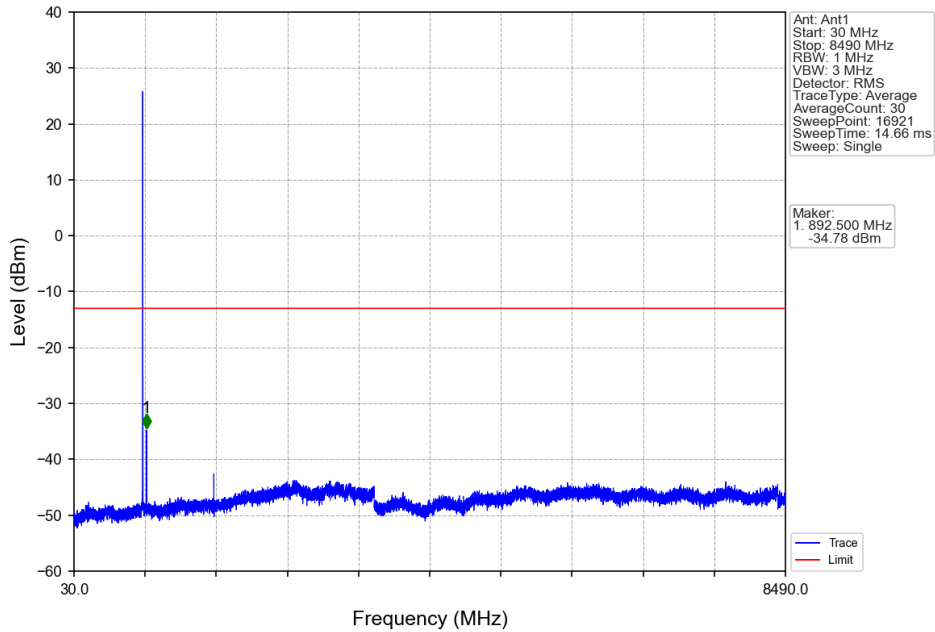
Band26b_3MHz_16QAM_HCH_847.5MHz_RB_1_0_NTNV
