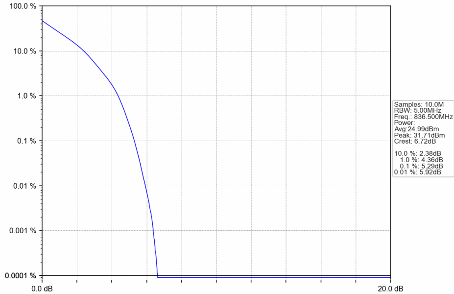
Band26b_5MHz_QPSK_MCH_836.5MHz_RB_25_0_NTNV
