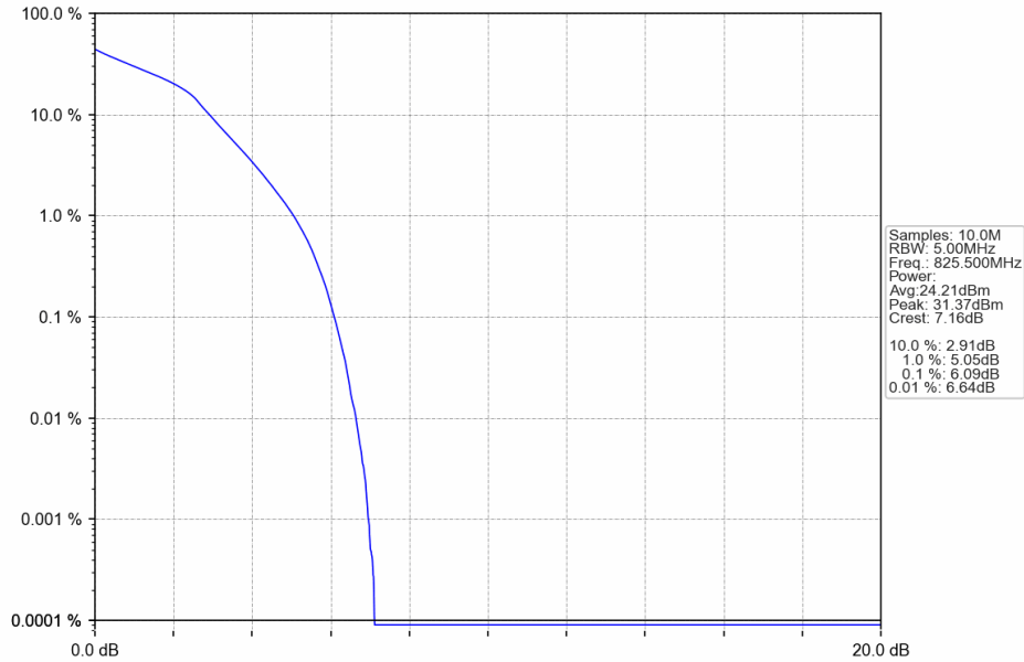
Band26b_3MHz_16QAM_LCH_825.5MHz_RB_15_0_NTNV
