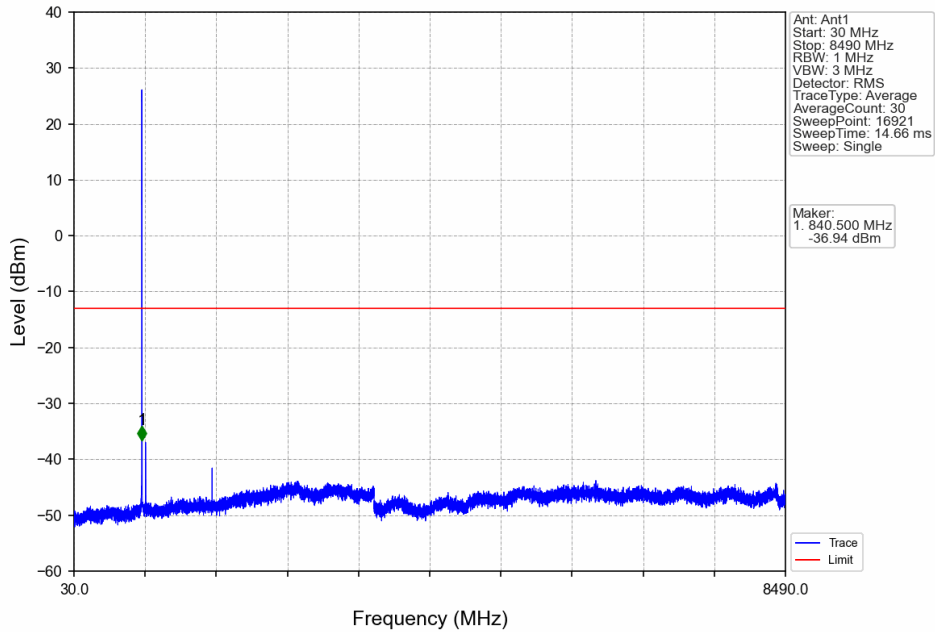
Band26b_1.4MHz_QPSK_MCH_836.5MHz_RB_1_0_NTNV
