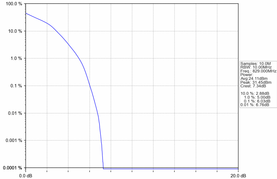
Band26b_10MHz_16QAM_LCH_829MHz_RB_50_0_NTNV
