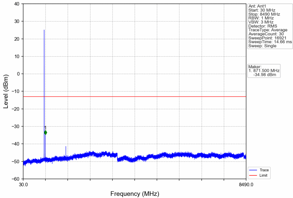
Band26b_3MHz_QPSK_LCH_825.5MHz_RB_1_0_NTNV
