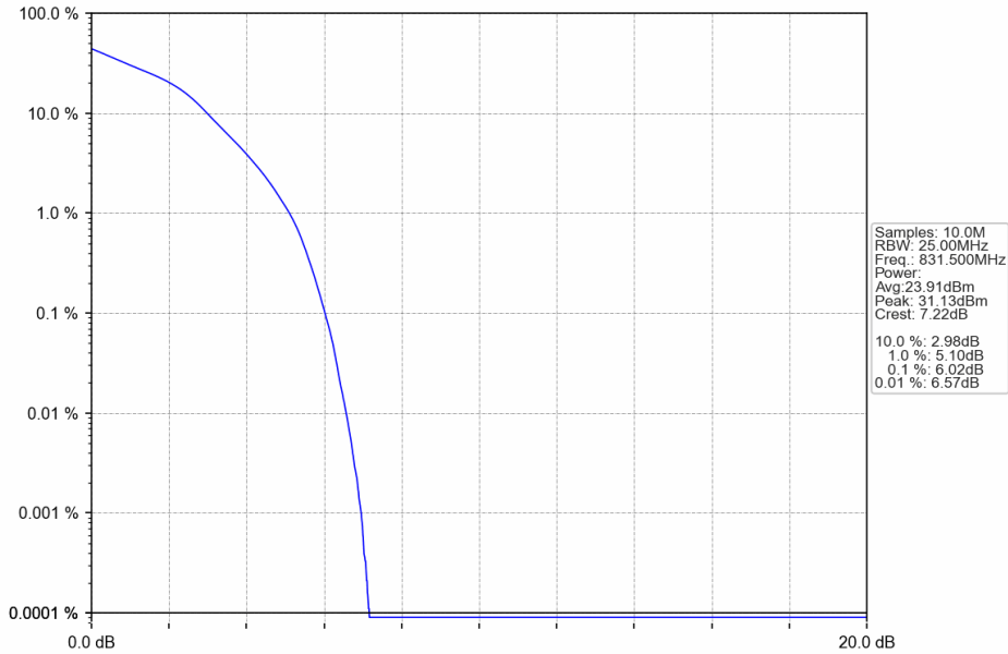
Band26c_15MHz_16QAM_MCH_831.5MHz_RB_75_0_NTNV
