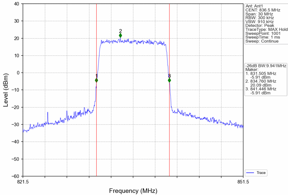
Band26b_10MHz_64QAM_MCH_836.5MHz_RB_50_0_NTNV
