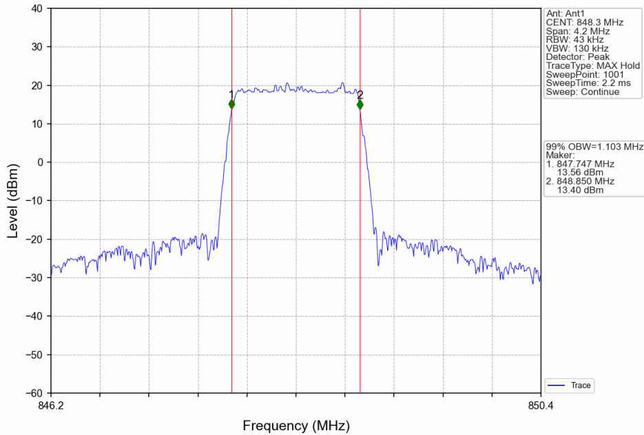
Band26b_1.4MHz_64QAM_HCH_848.3MHz_RB_6_0_NTNV
