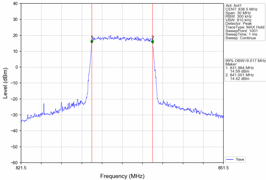
Band26b_10MHz_64QAM_MCH_836.5MHz_RB_50_0_NTNV
