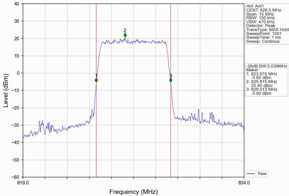
Band26b_5MHz_64QAM_LCH_826.5MHz_RB_25_0_NTNV
