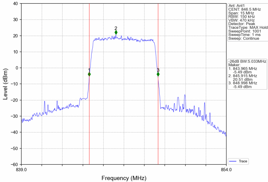
Band26b_5MHz_64QAM_HCH_846.5MHz_RB_25_0_NTNV
