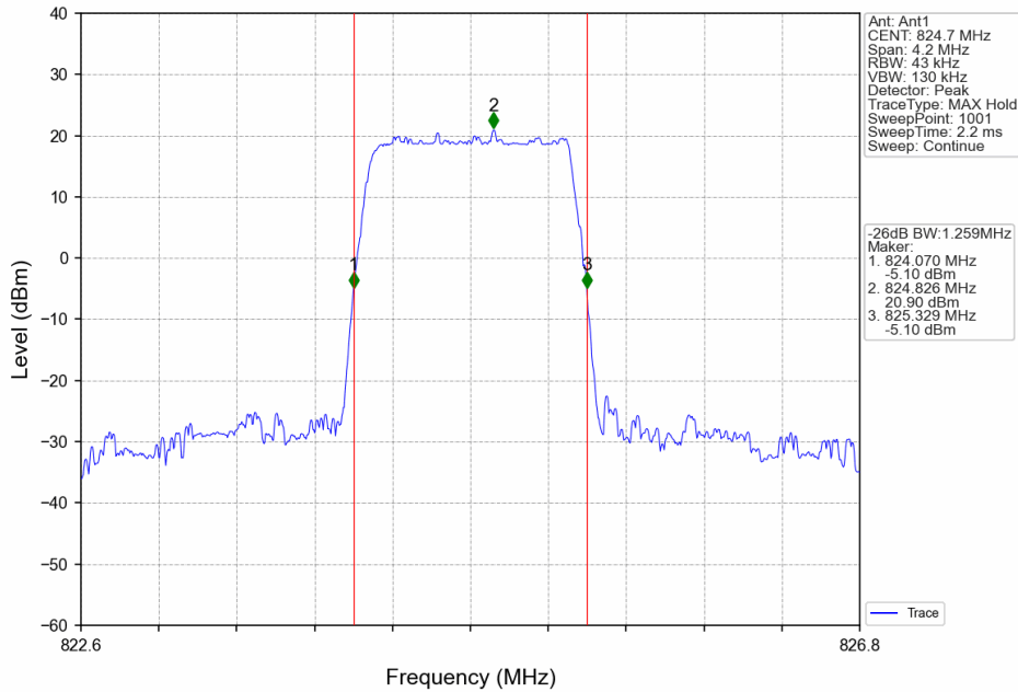
Band26b_1.4MHz_64QAM_LCH_824.7MHz_RB_6_0_NTNV
