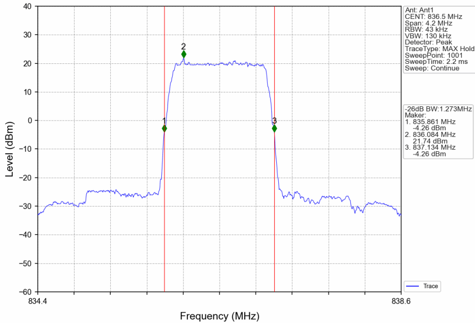
Band26b_1.4MHz_16QAM_MCH_836.5MHz_RB_6_0_NTNV
