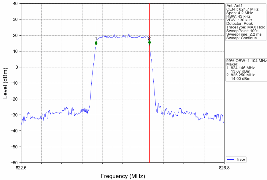
Band26b_1.4MHz_64QAM_LCH_824.7MHz_RB_6_0_NTNV
