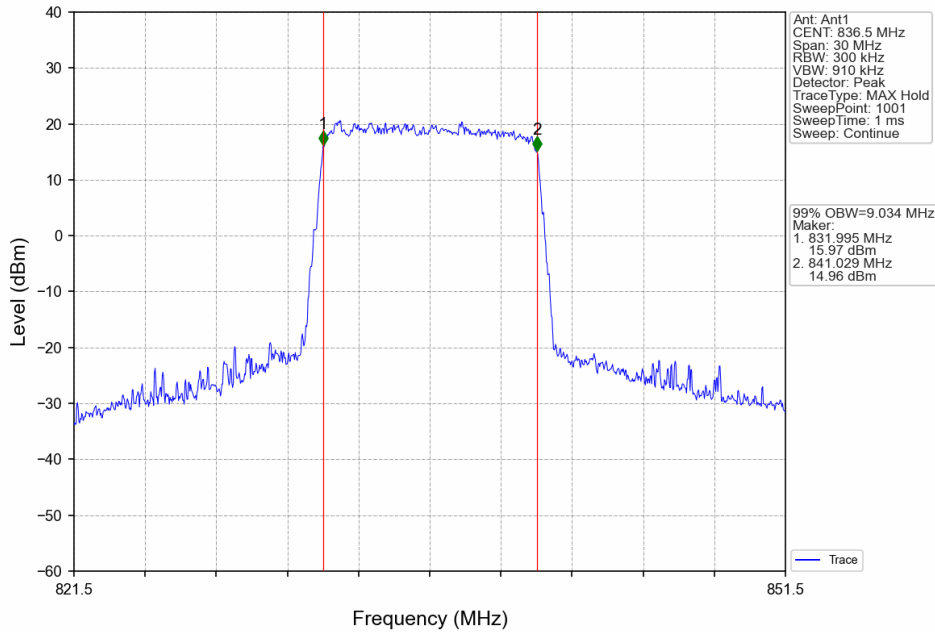
Band26b_10MHz_16QAM_MCH_836.5MHz_RB_50_0_NTNV
