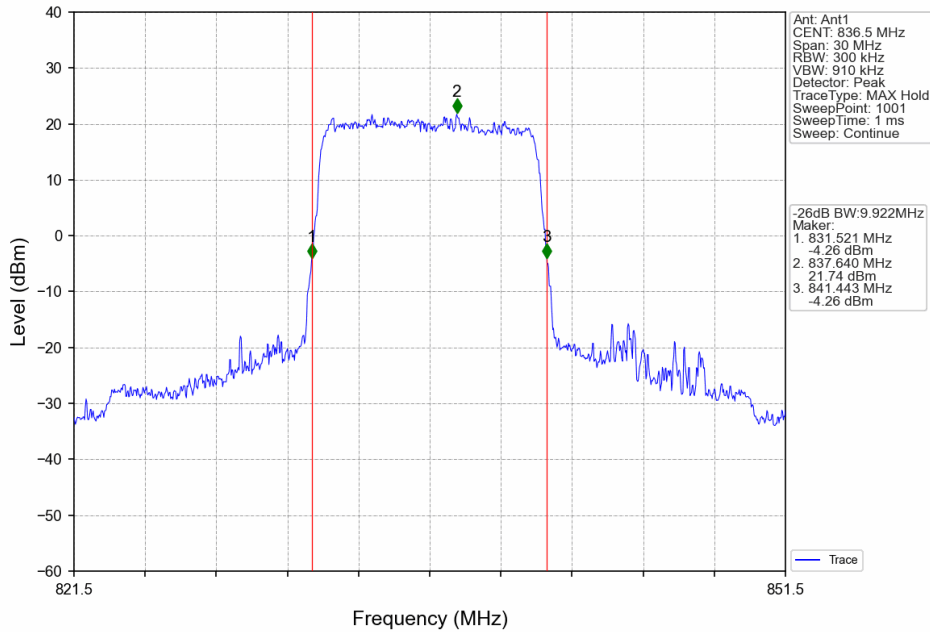
Band26b_10MHz_QPSK_MCH_836.5MHz_RB_50_0_NTNV
