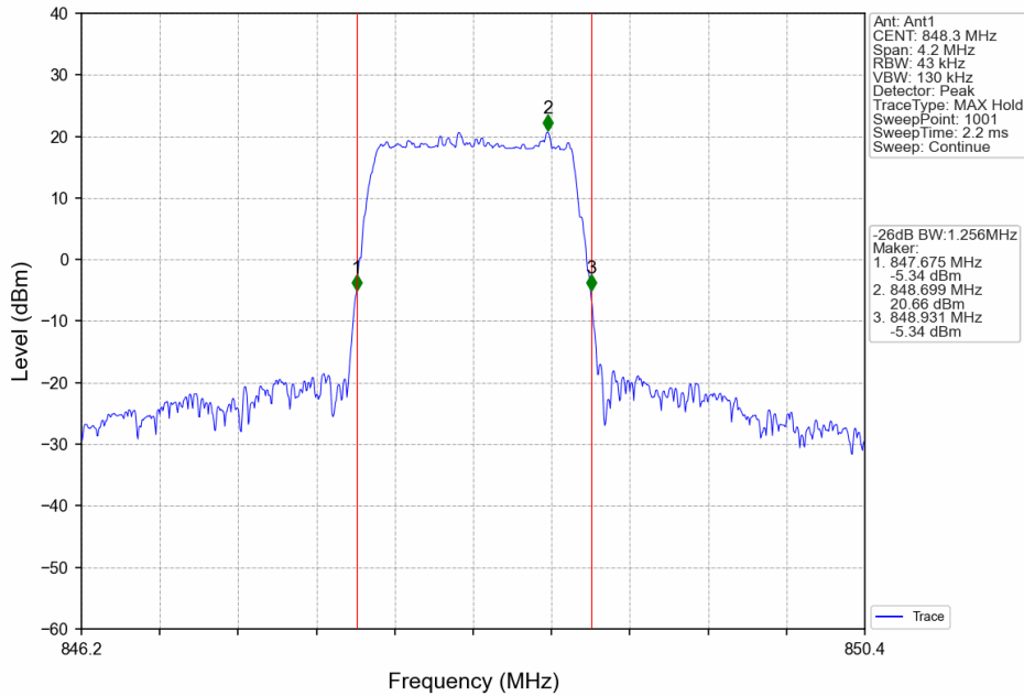
Band26b_1.4MHz_64QAM_HCH_848.3MHz_RB_6_0_NTNV
