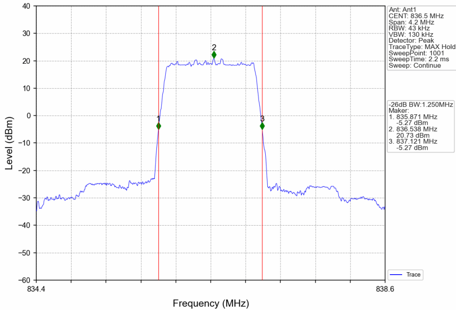
Band26b_1.4MHz_64QAM_MCH_836.5MHz_RB_6_0_NTNV
