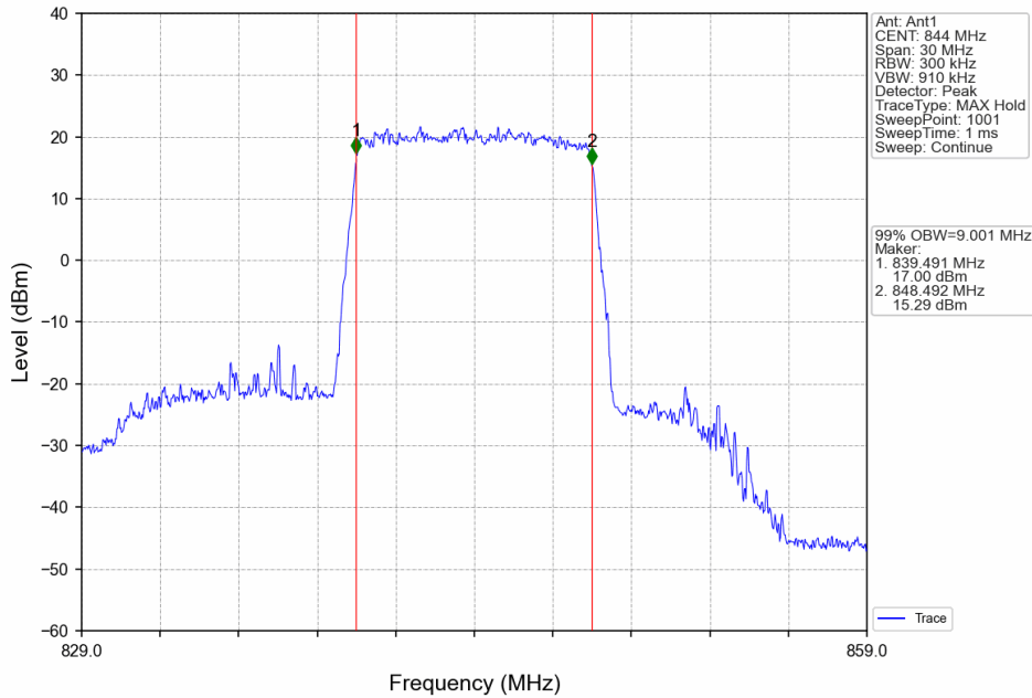
Band26b_10MHz_QPSK_HCH_844MHz_RB_50_0_NTNV
