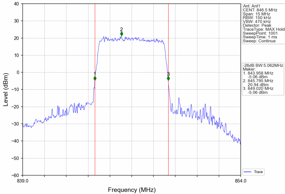
Band26b_5MHz_16QAM_HCH_846.5MHz_RB_25_0_NTNV
