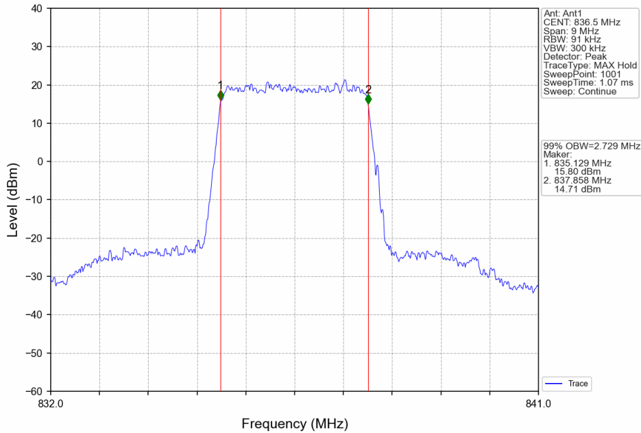
Band26b_3MHz_16QAM_MCH_836.5MHz_RB_15_0_NTNV
