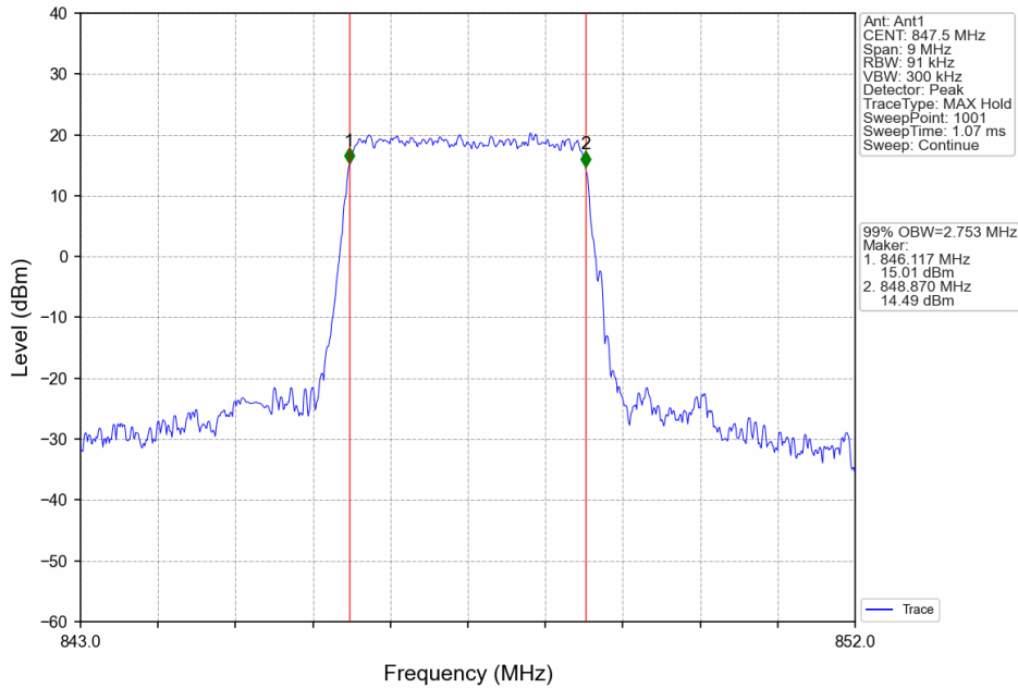
Band26b_3MHz_16QAM_HCH_847.5MHz_RB_15_0_NTNV
