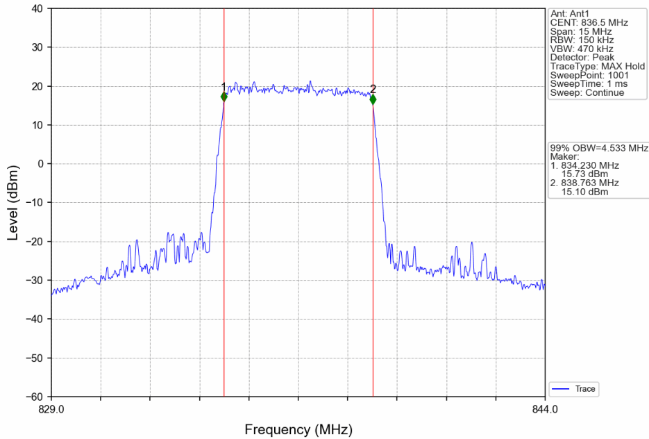
Band26b_5MHz_16QAM_MCH_836.5MHz_RB_25_0_NTNV
