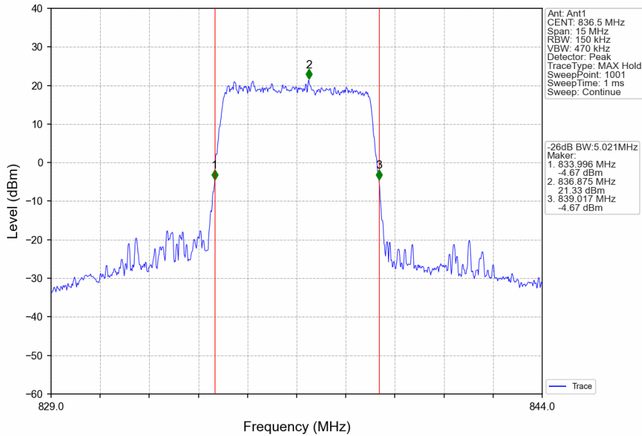
Band26b_5MHz_16QAM_MCH_836.5MHz_RB_25_0_NTNV
