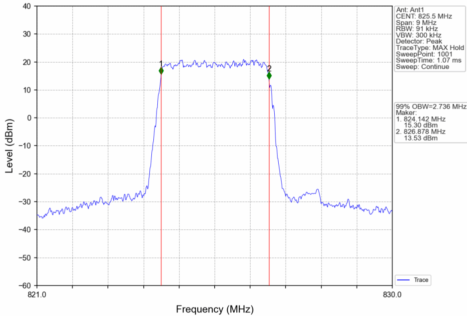
Band26b_3MHz_16QAM_LCH_825.5MHz_RB_15_0_NTNV
