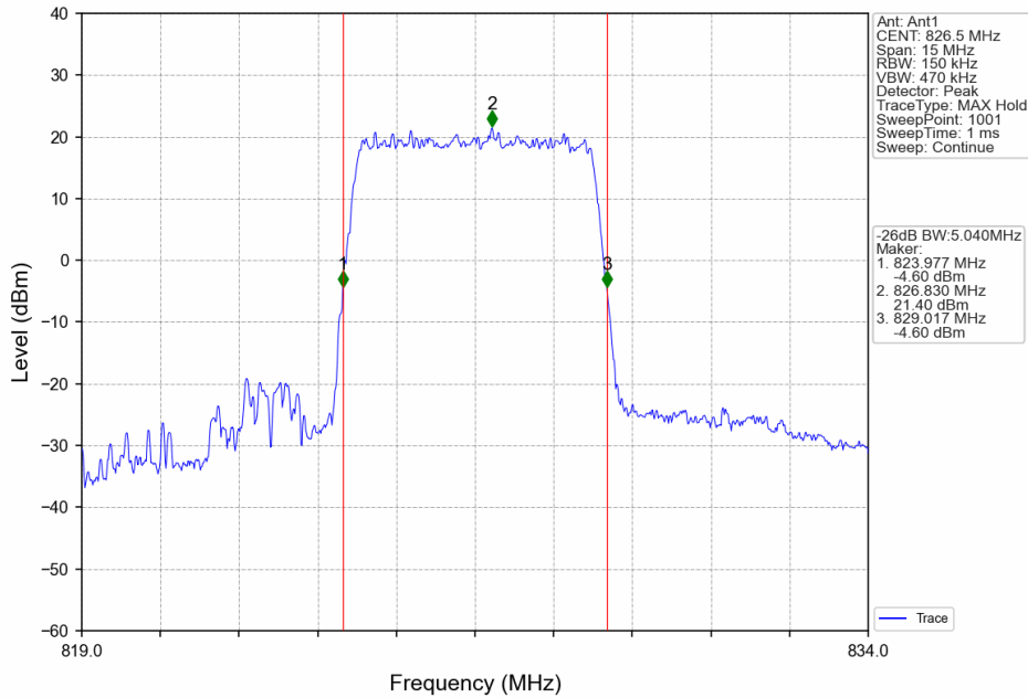
Band26b_5MHz_16QAM_LCH_826.5MHz_RB_25_0_NTNV
