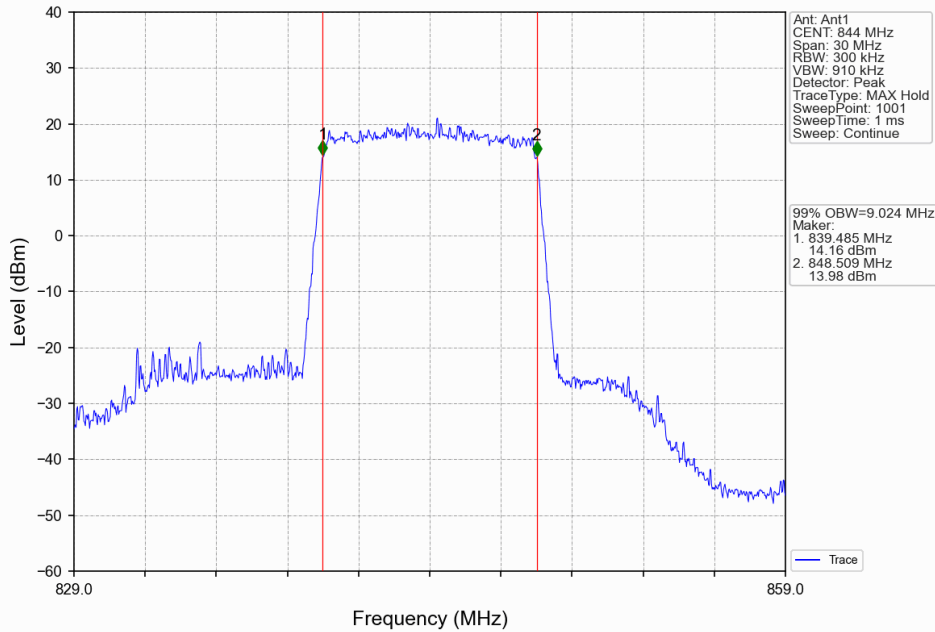
Band26b_10MHz_64QAM_HCH_844MHz_RB_50_0_NTNV
