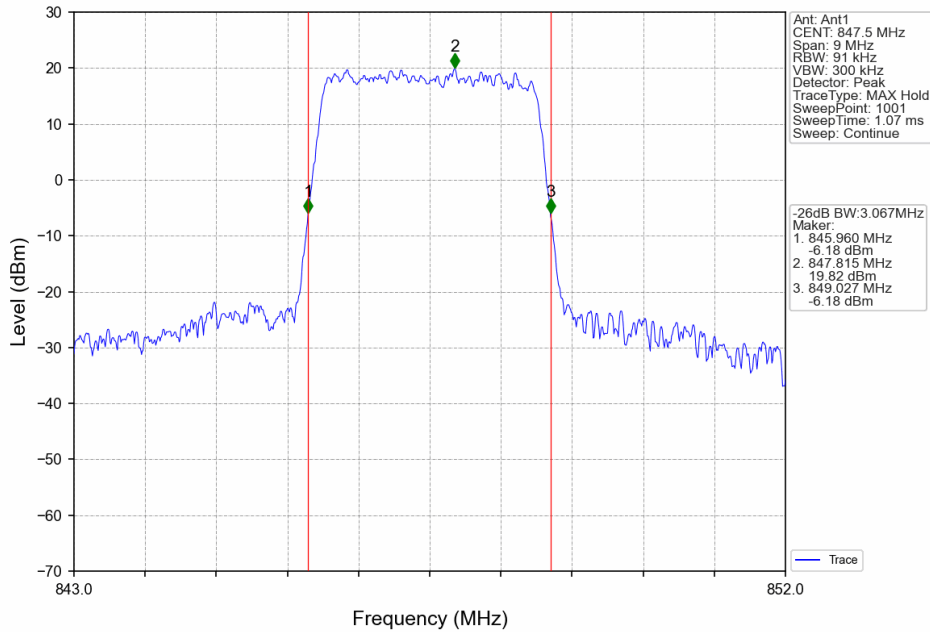
Band26b_3MHz_64QAM_HCH_847.5MHz_RB_15_0_NTNV
