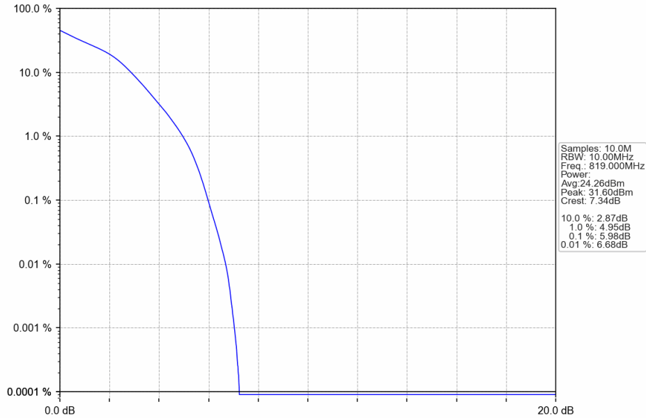
Band26a_10MHz_16QAM_MCH_819MHz_RB_50_0_NTNV
