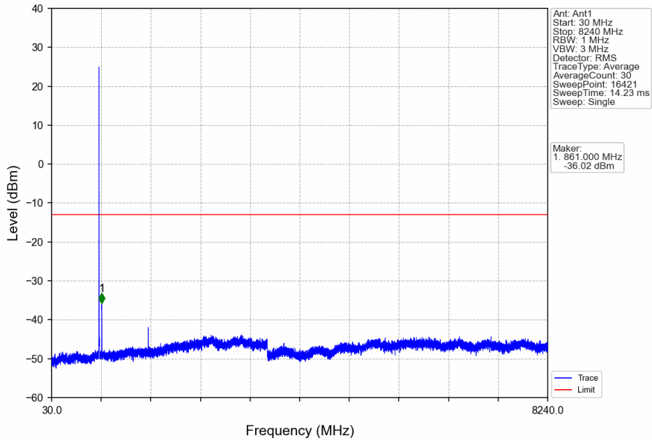
Band26a_5MHz_16QAM_LCH_816.5MHz_RB_1_0_NTNV
