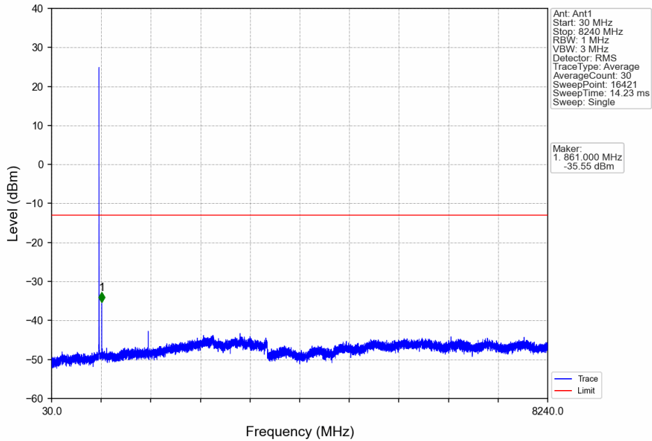
Band26a_3MHz_16QAM_LCH_815.5MHz_RB_1_0_NTNV
