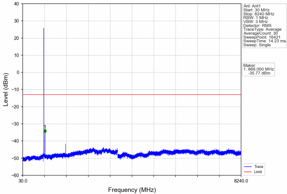
Band26a_3MHz_16QAM_HCH_822.5MHz_RB_1_0_NTNV
