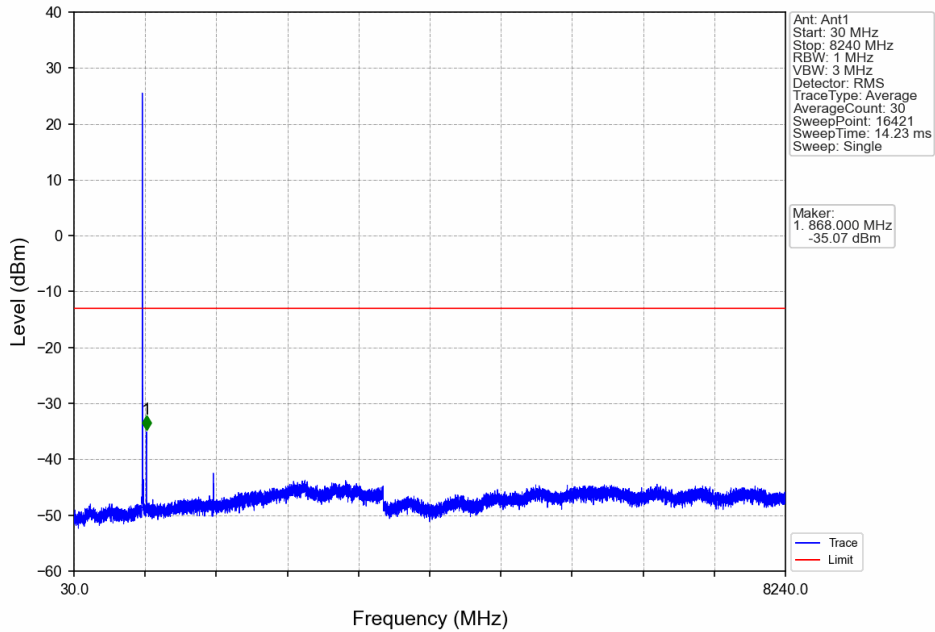
Band26a_5MHz_16QAM_HCH_821.5MHz_RB_1_0_NTNV
