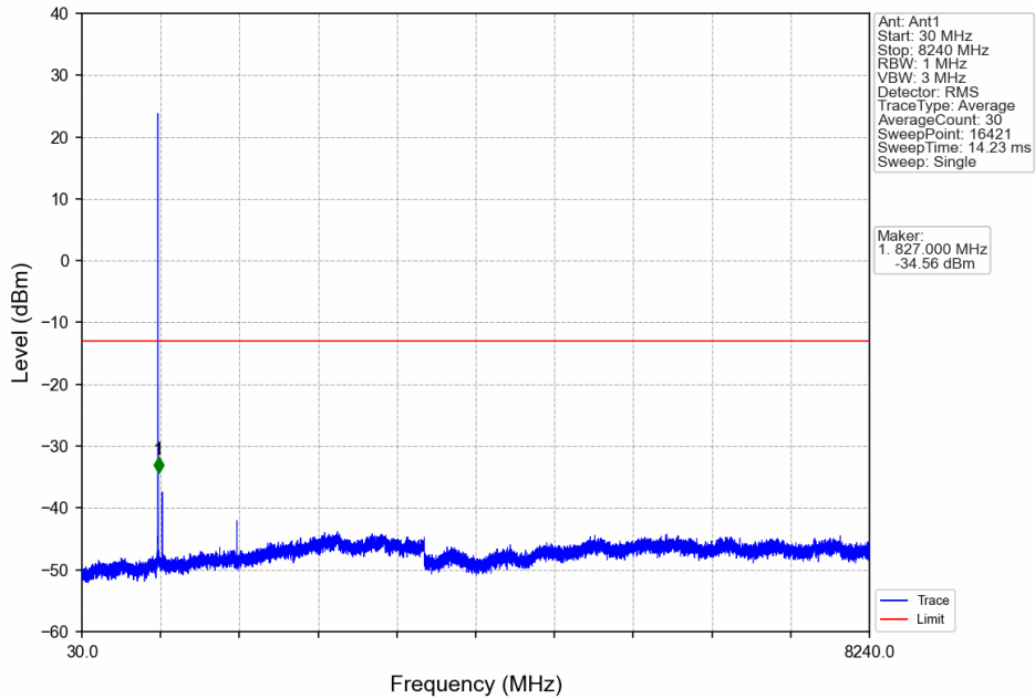
Band26a_1.4MHz_16QAM_HCH_823.3MHz_RB_1_0_NTNV
