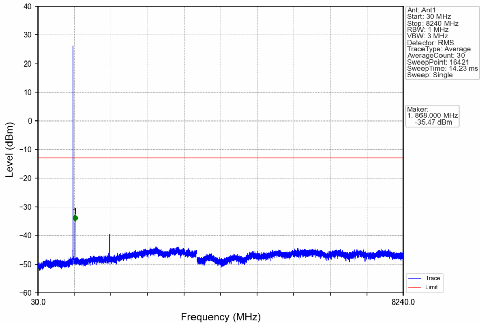
Band26a_5MHz_QPSK_HCH_821.5MHz_RB_1_0_NTNV
