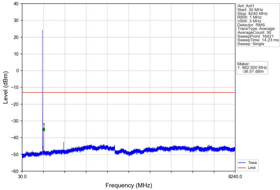
Band26a_5MHz_64QAM_LCH_816.5MHz_RB_1_0_NTNV
