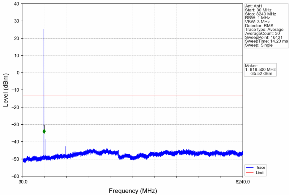
Band26a_1.4MHz_64QAM_LCH_814.7MHz_RB_1_0_NTNV
