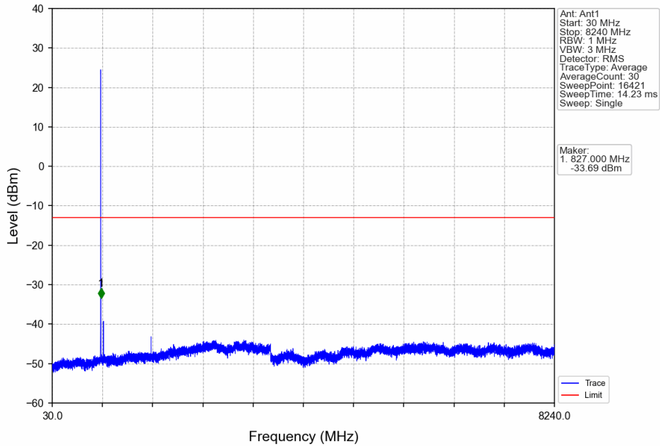
Band26a_1.4MHz_64QAM_HCH_823.3MHz_RB_1_0_NTNV
