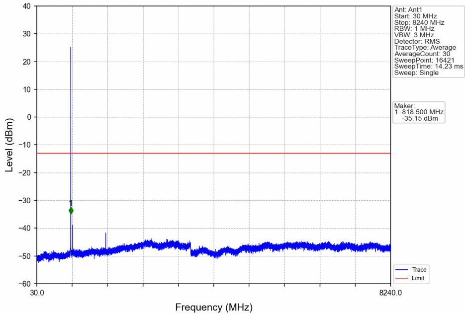
Band26a_1.4MHz_16QAM_LCH_814.7MHz_RB_1_0_NTNV
