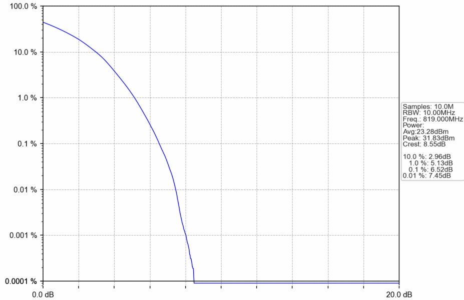
Band26a_10MHz_64QAM_MCH_819MHz_RB_50_0_NTNV
