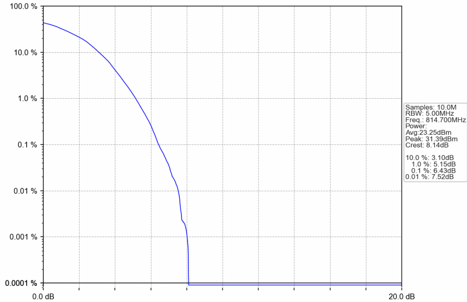
Band26a_1.4MHz_64QAM_LCH_814.7MHz_RB_6_0_NTNV
