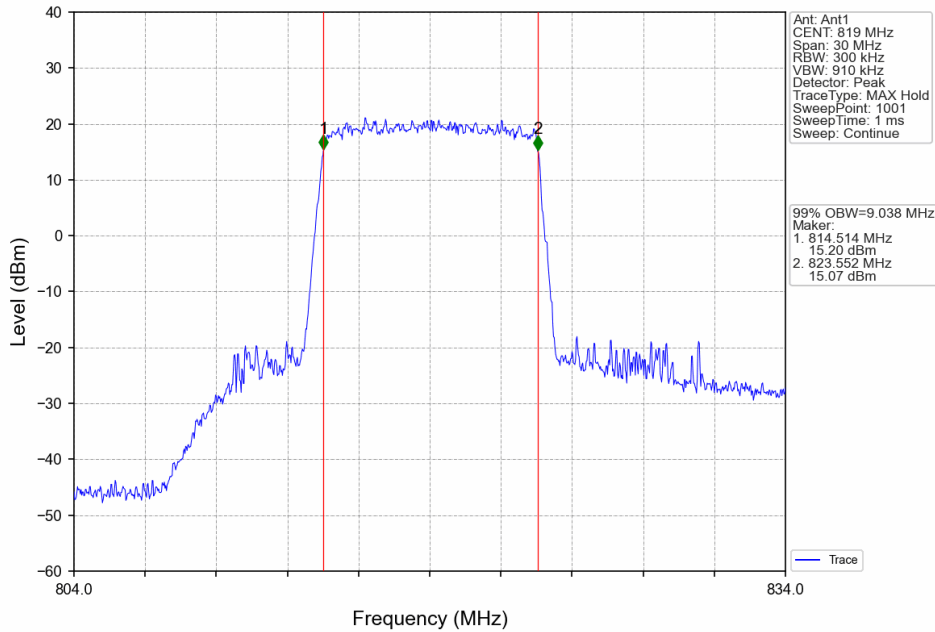
Band26a_10MHz_16QAM_MCH_819MHz_RB_50_0_NTNV
