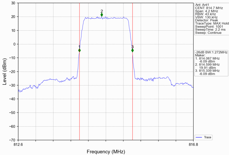
Band26a_1.4MHz_64QAM_LCH_814.7MHz_RB_6_0_NTNV
