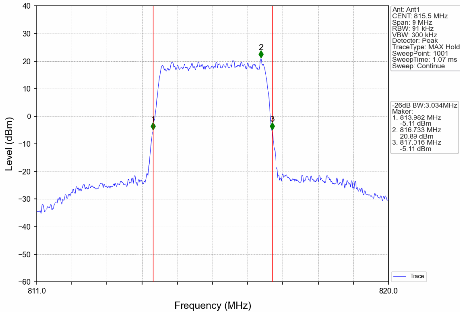
Band26a_3MHz_64QAM_LCH_815.5MHz_RB_15_0_NTNV
