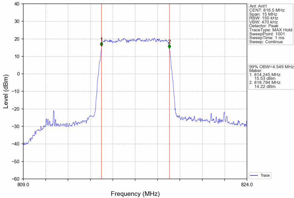
Band26a_5MHz_16QAM_LCH_816.5MHz_RB_25_0_NTNV
