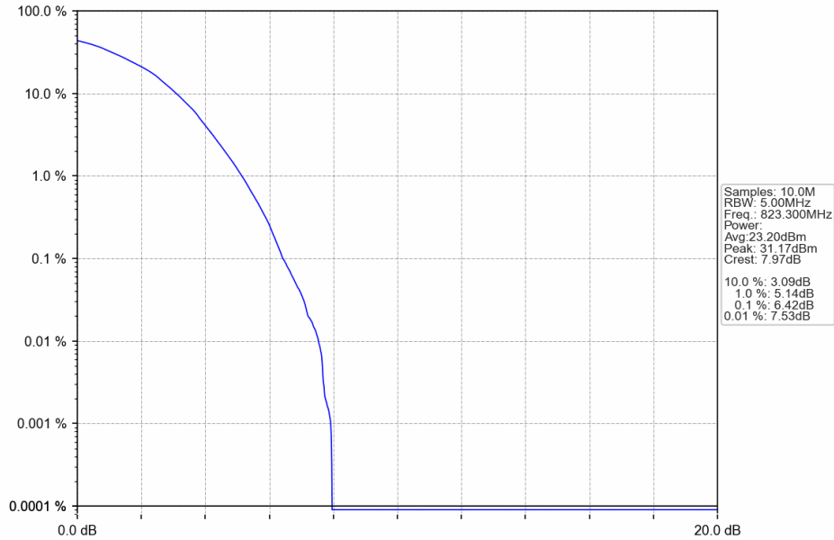
Band26a_1.4MHz_64QAM_HCH_823.3MHz_RB_6_0_NTNV
