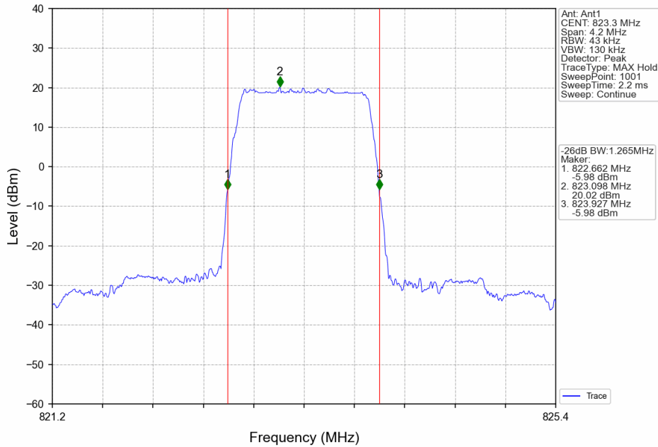
Band26a_1.4MHz_64QAM_HCH_823.3MHz_RB_6_0_NTNV
