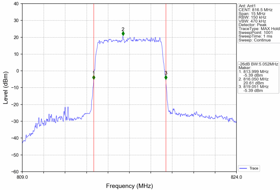
Band26a_5MHz_64QAM_LCH_816.5MHz_RB_25_0_NTNV
