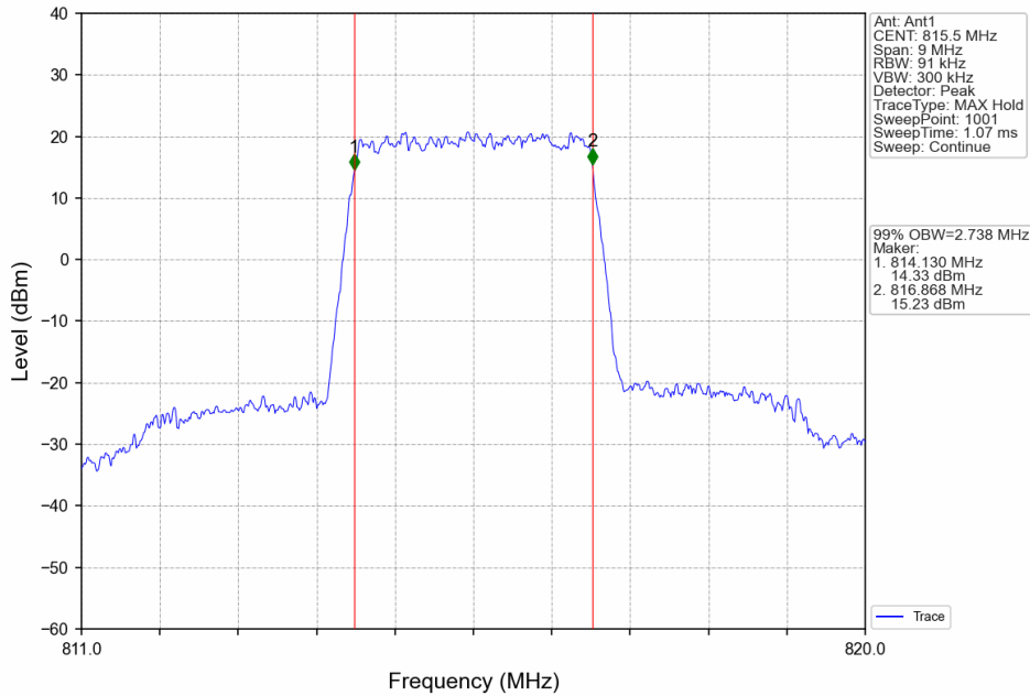
Band26a_3MHz_16QAM_LCH_815.5MHz_RB_15_0_NTNV
