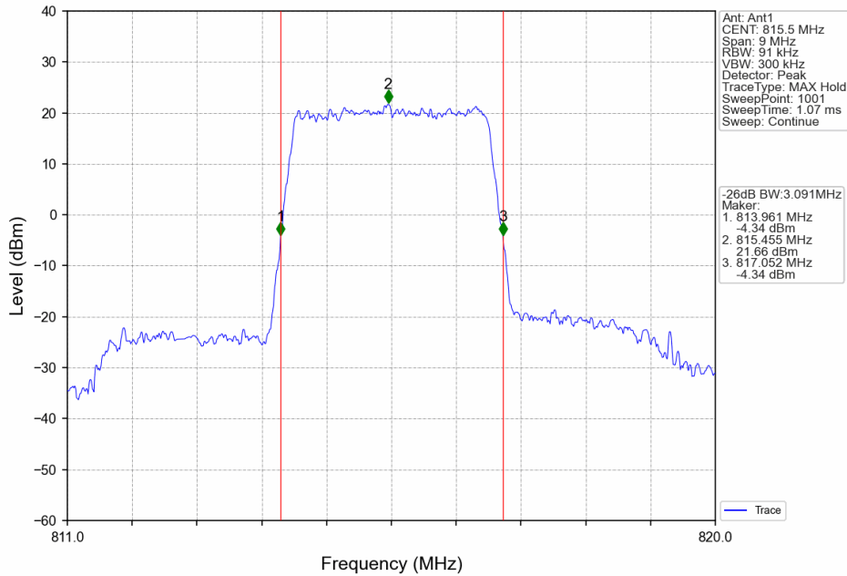
Band26a_3MHz_QPSK_LCH_815.5MHz_RB_15_0_NTNV
