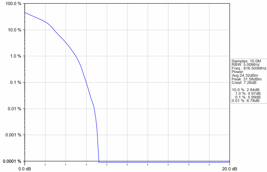
Band26a_5MHz_16QAM_LCH_816.5MHz_RB_25_0_NTNV
