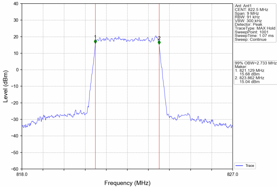
Band26a_3MHz_64QAM_HCH_822.5MHz_RB_15_0_NTNV
