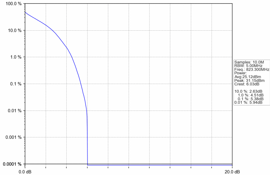
Band26a_1.4MHz_QPSK_HCH_823.3MHz_RB_6_0_NTNV
