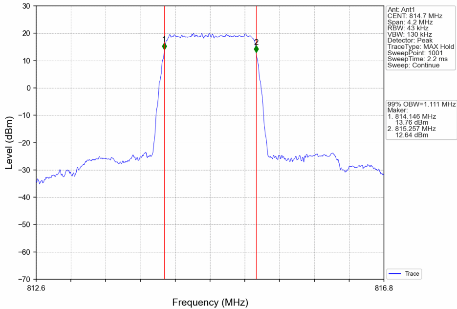
Band26a_1.4MHz_64QAM_LCH_814.7MHz_RB_6_0_NTNV
