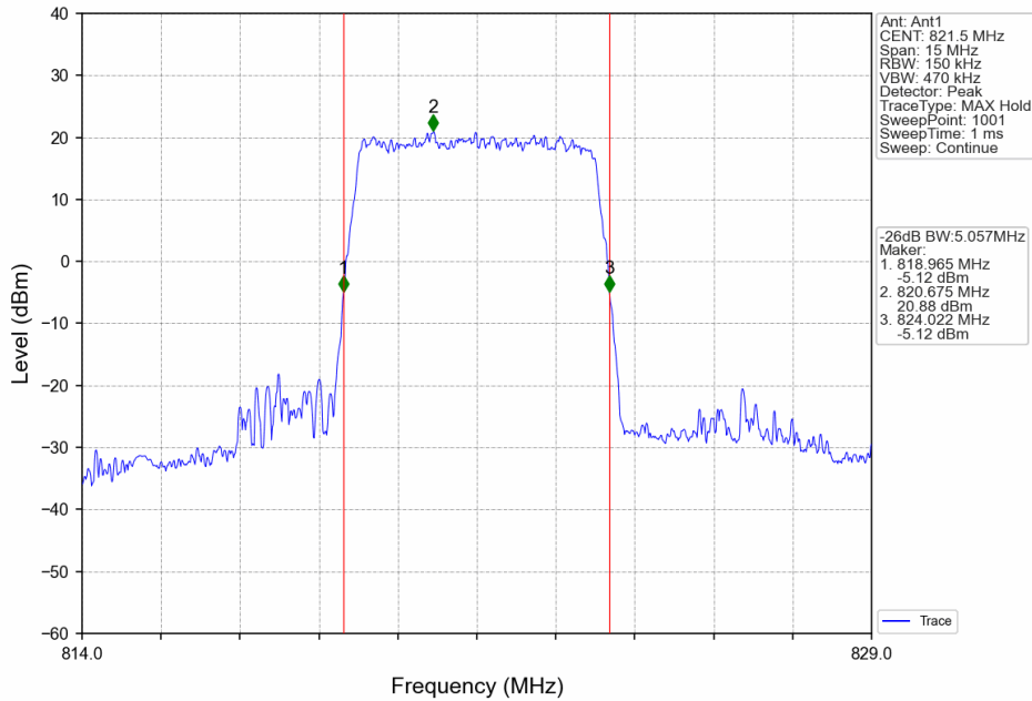
Band26a_5MHz_16QAM_HCH_821.5MHz_RB_25_0_NTNV
