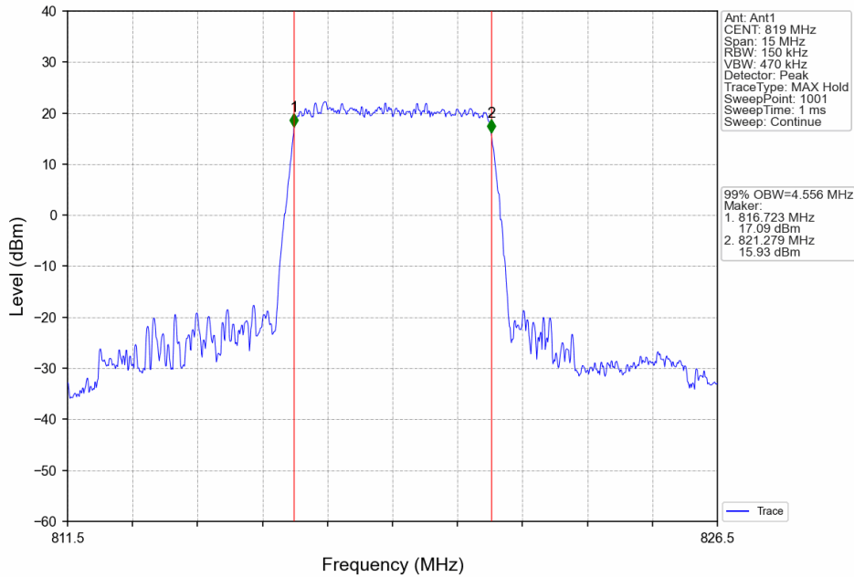
Band26a_5MHz_QPSK_MCH_819MHz_RB_25_0_NTNV
