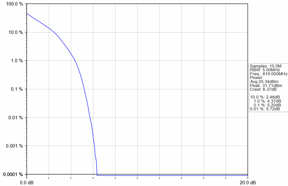
Band26a_3MHz_QPSK_MCH_819MHz_RB_15_0_NTNV
