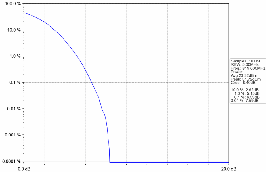
Band26a_5MHz_64QAM_MCH_819MHz_RB_25_0_NTNV
