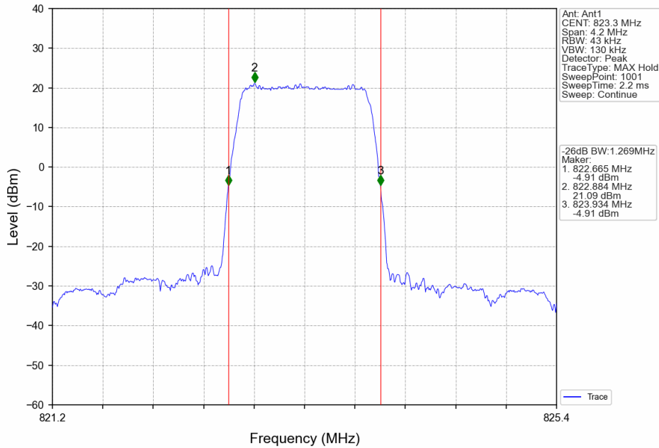
Band26a_1.4MHz_16QAM_HCH_823.3MHz_RB_6_0_NTNV
