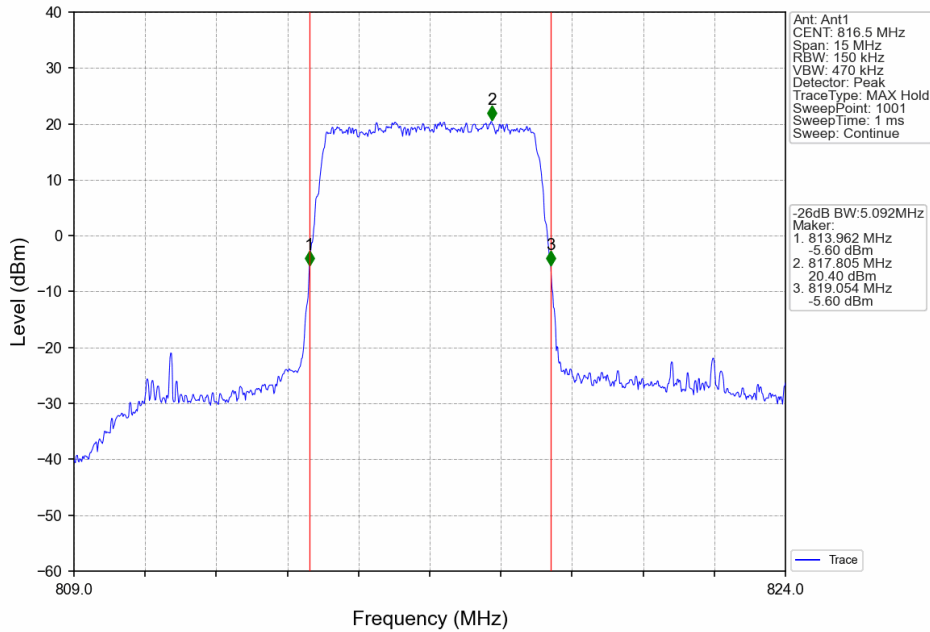
Band26a_5MHz_16QAM_LCH_816.5MHz_RB_25_0_NTNV
