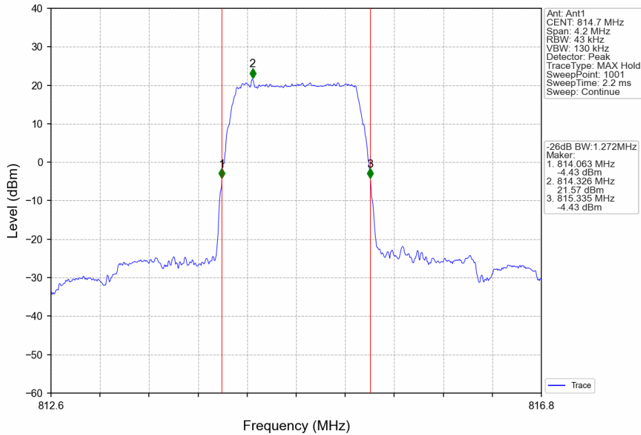
Band26a_1.4MHz_16QAM_LCH_814.7MHz_RB_6_0_NTNV
