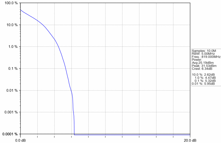
Band26a_1.4MHz_QPSK_MCH_819MHz_RB_6_0_NTNV
