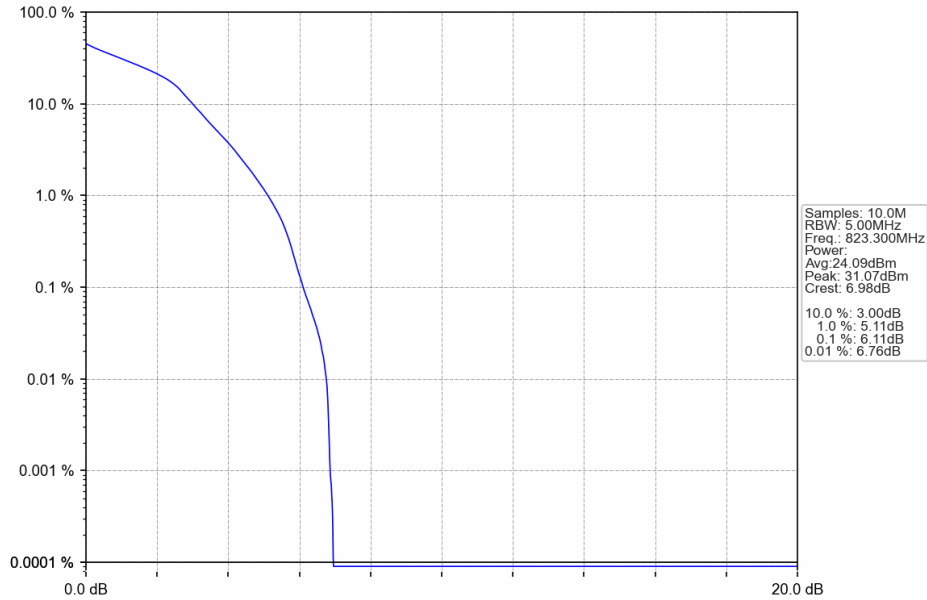
Band26a_1.4MHz_16QAM_HCH_823.3MHz_RB_6_0_NTNV
