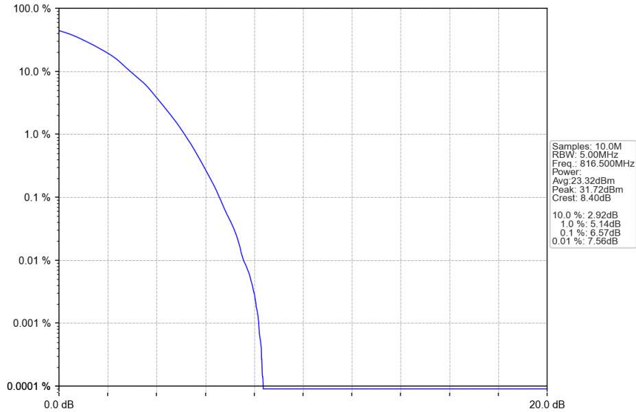
Band26a_5MHz_64QAM_LCH_816.5MHz_RB_25_0_NTNV
