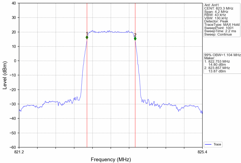
Band26a_1.4MHz_16QAM_HCH_823.3MHz_RB_6_0_NTNV
