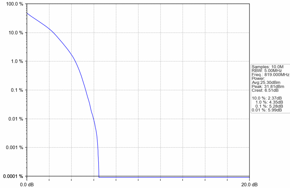
Band26a_5MHz_QPSK_MCH_819MHz_RB_25_0_NTNV
