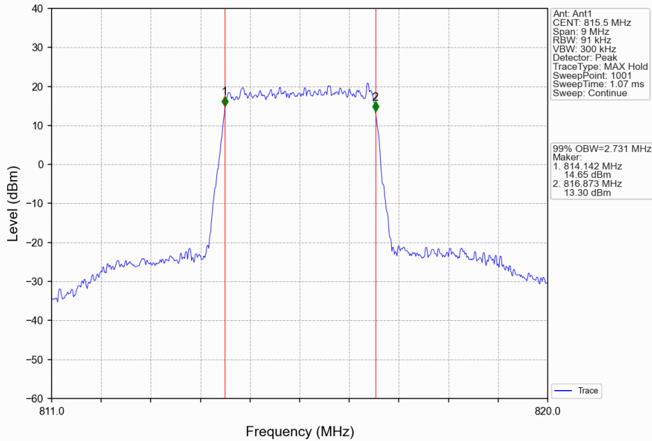
Band26a_3MHz_64QAM_LCH_815.5MHz_RB_15_0_NTNV
