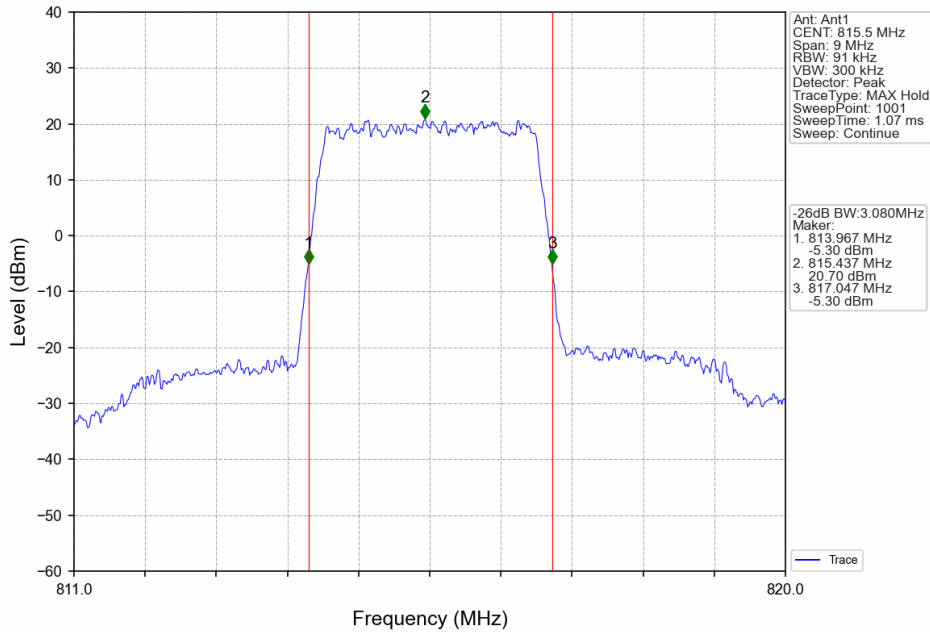
Band26a_3MHz_16QAM_LCH_815.5MHz_RB_15_0_NTNV
