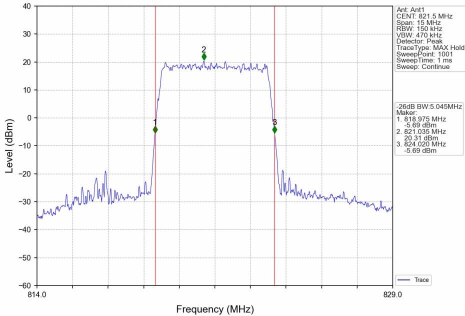
Band26a_5MHz_64QAM_HCH_821.5MHz_RB_25_0_NTNV
