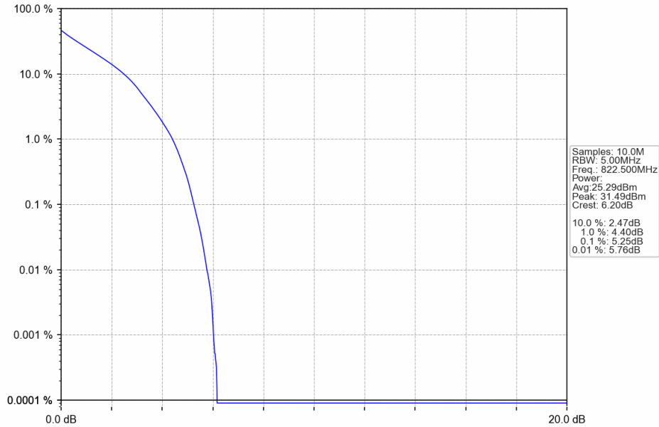
Band26a_3MHz_QPSK_HCH_822.5MHz_RB_15_0_NTNV
