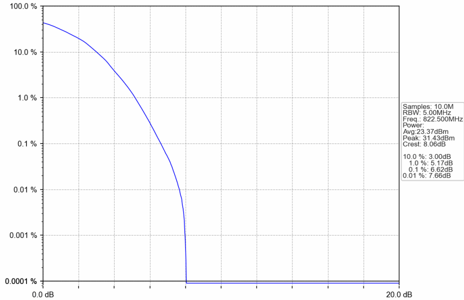
Band26a_3MHz_64QAM_HCH_822.5MHz_RB_15_0_NTNV
