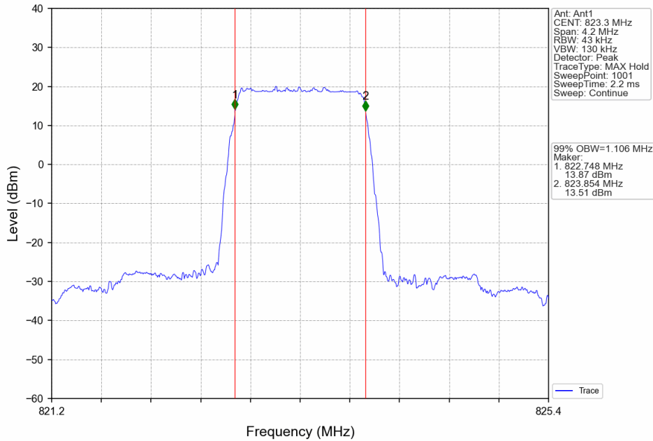
Band26a_1.4MHz_64QAM_HCH_823.3MHz_RB_6_0_NTNV
