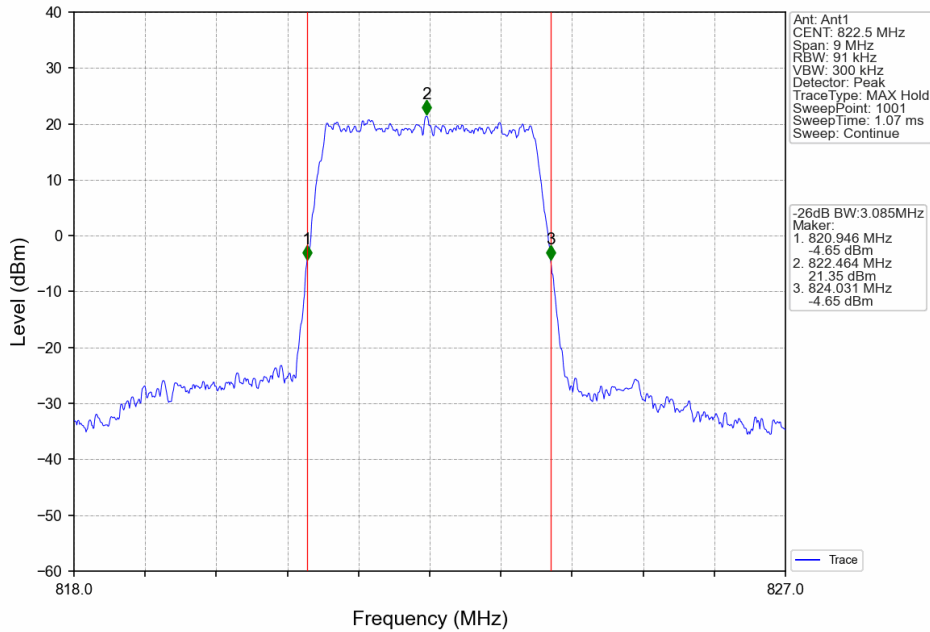
Band26a_3MHz_16QAM_HCH_822.5MHz_RB_15_0_NTNV
