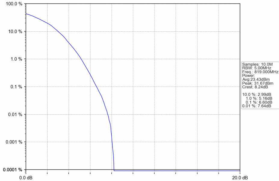
Band26a_3MHz_64QAM_MCH_819MHz_RB_15_0_NTNV
