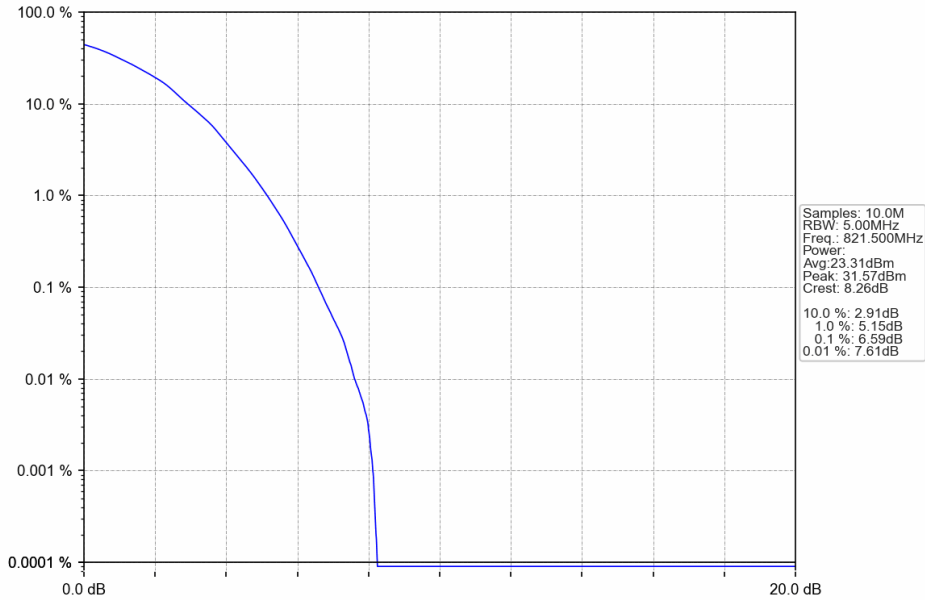
Band26a_5MHz_64QAM_HCH_821.5MHz_RB_25_0_NTNV
