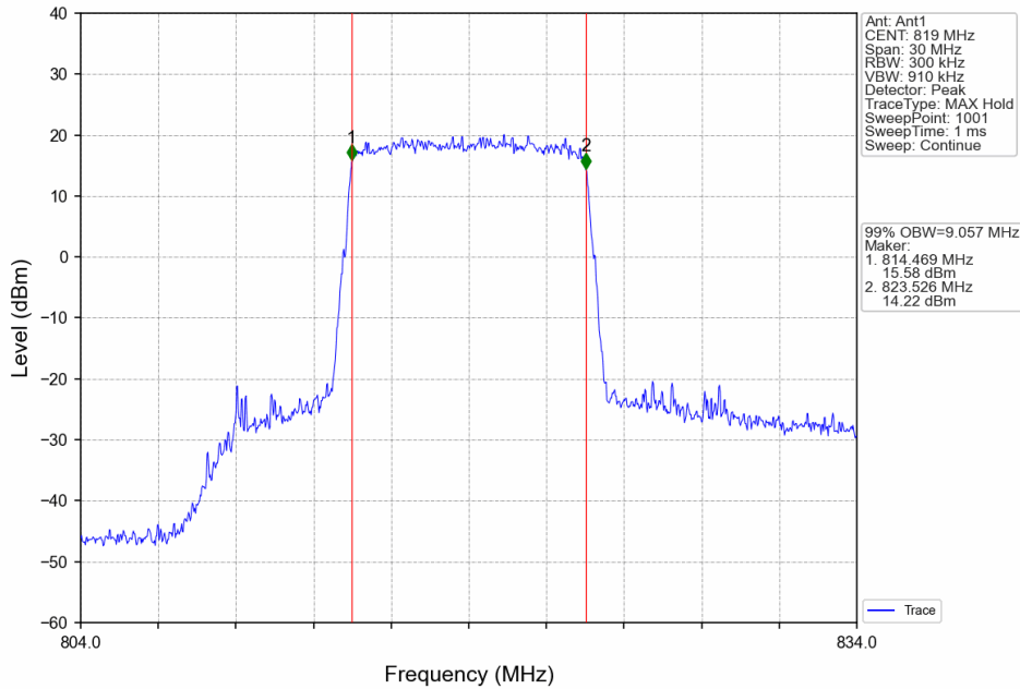
Band26a_10MHz_64QAM_MCH_819MHz_RB_50_0_NTNV
