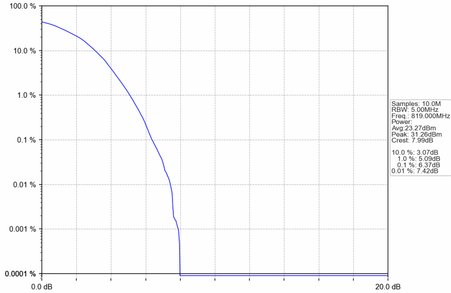
Band26a_1.4MHz_64QAM_MCH_819MHz_RB_6_0_NTNV
