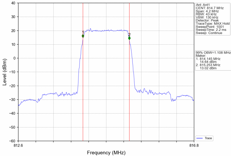
Band26a_1.4MHz_16QAM_LCH_814.7MHz_RB_6_0_NTNV
