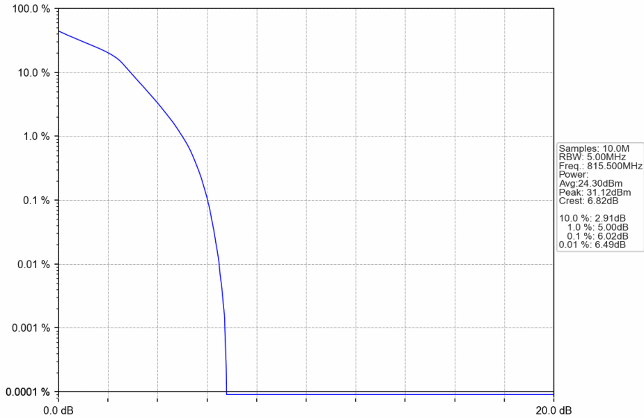
Band26a_3MHz_16QAM_LCH_815.5MHz_RB_15_0_NTNV
