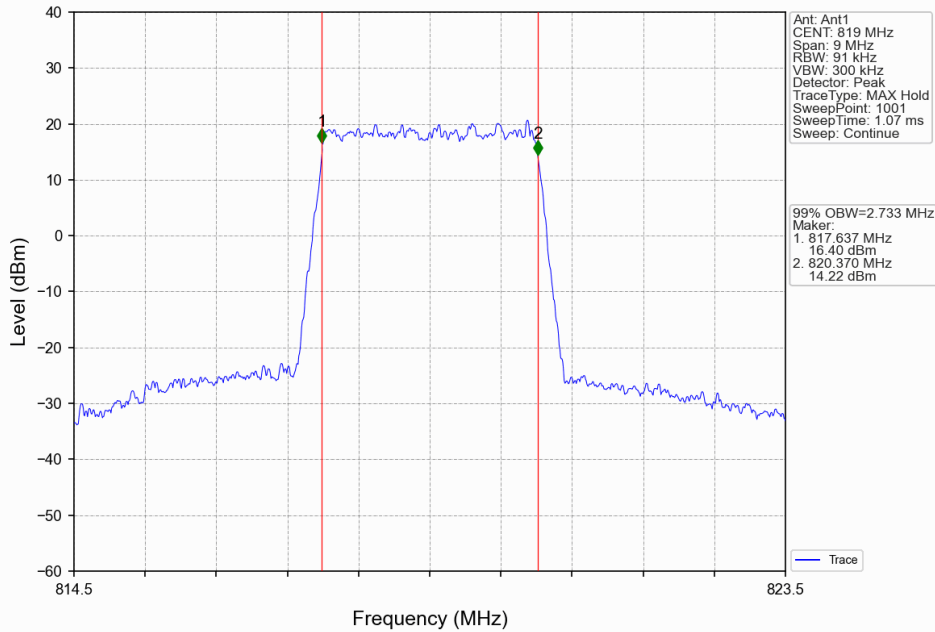
Band26a_3MHz_64QAM_MCH_819MHz_RB_15_0_NTNV
