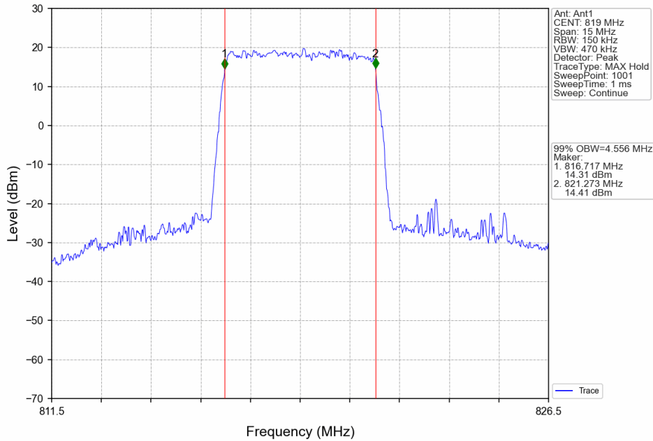
Band26a_5MHz_64QAM_MCH_819MHz_RB_25_0_NTNV
