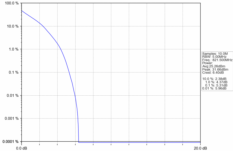
Band26a_5MHz_QPSK_HCH_821.5MHz_RB_25_0_NTNV
