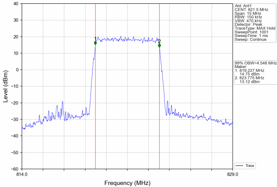
Band26a_5MHz_64QAM_HCH_821.5MHz_RB_25_0_NTNV
