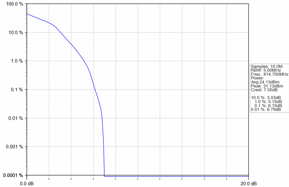
Band26a_1.4MHz_16QAM_LCH_814.7MHz_RB_6_0_NTNV
