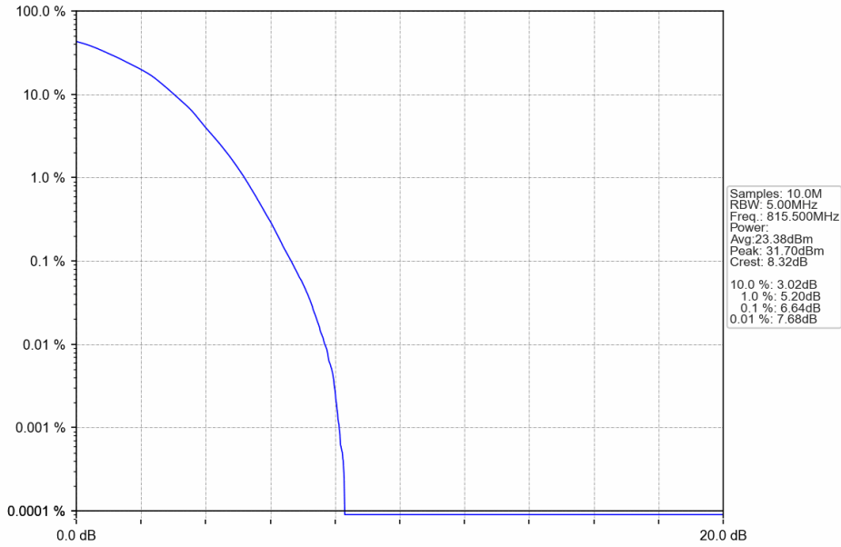
Band26a_3MHz_64QAM_LCH_815.5MHz_RB_15_0_NTNV
