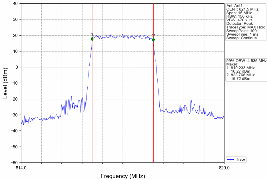
Band26a_5MHz_16QAM_HCH_821.5MHz_RB_25_0_NTNV
