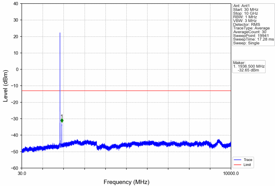
Band25_10MHz_64QAM_LCH_1855MHz_RB_1_0_NTNV
