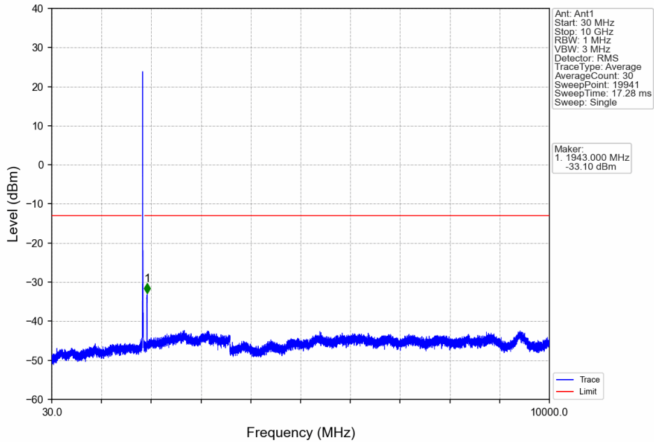
Band25_15MHz_64QAM_LCH_1857.5MHz_RB_1_0_NTNV
