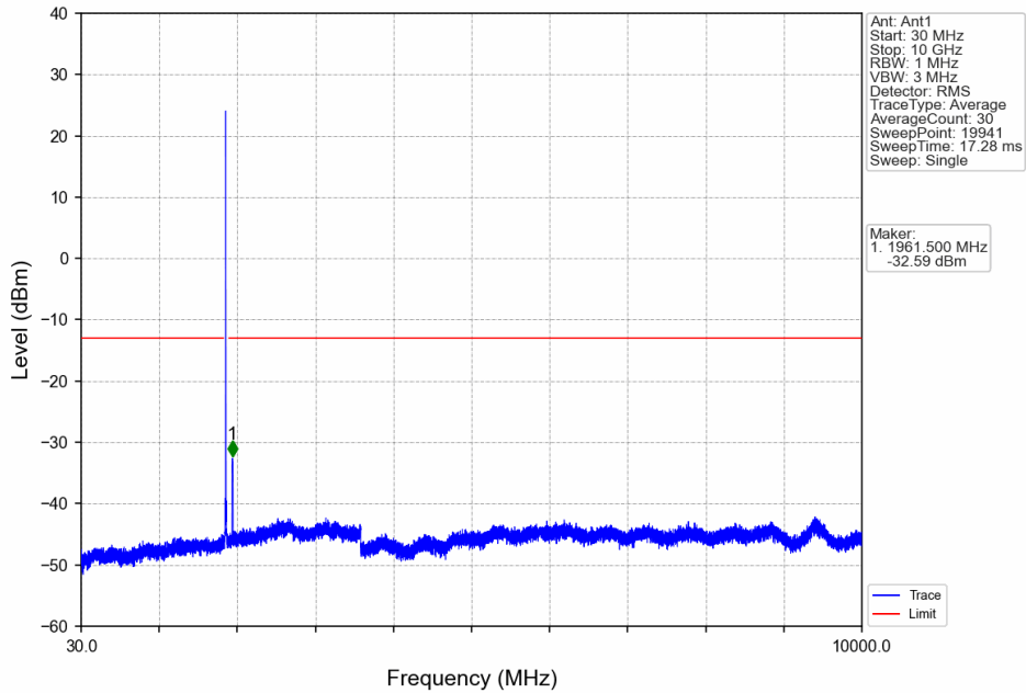
Band25_15MHz_64QAM_MCH_1882.5MHz_RB_1_0_NTNV
