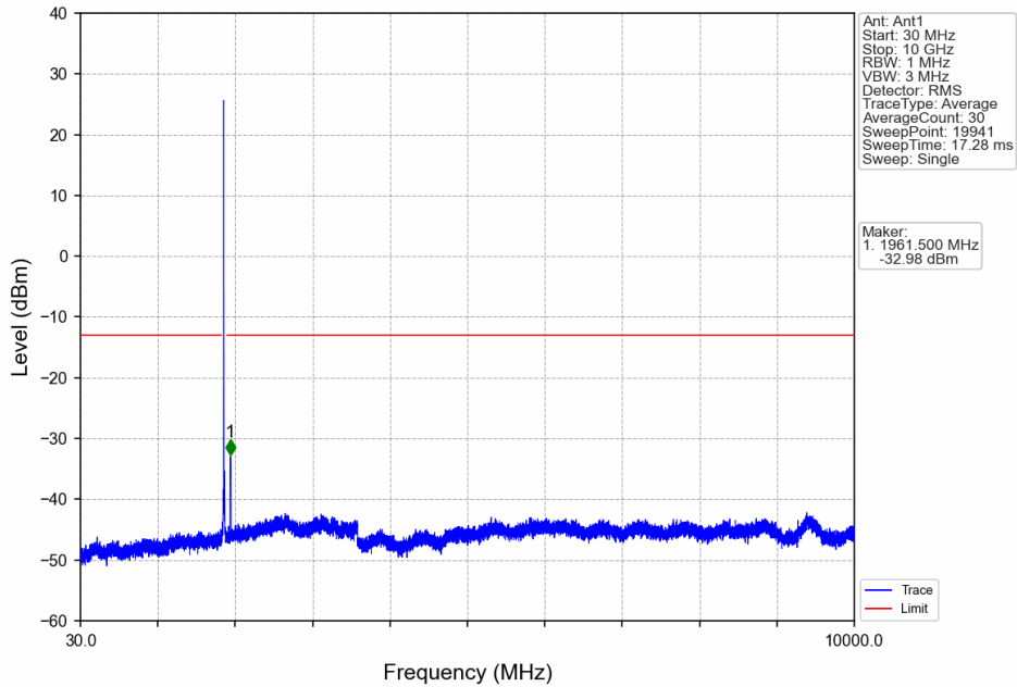
Band25_15MHz_QPSK_MCH_1882.5MHz_RB_1_0_NTNV
