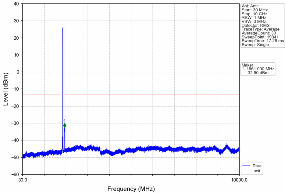
Band25_20MHz_QPSK_MCH_1882.5MHz_RB_1_0_NTNV
