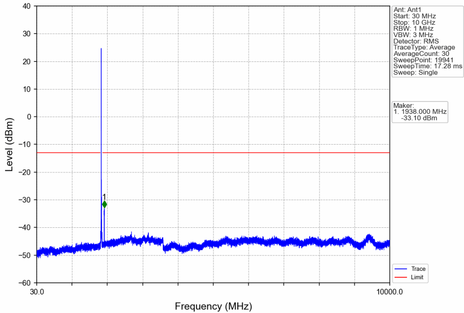
Band25_15MHz_16QAM_LCH_1857.5MHz_RB_1_0_NTNV
