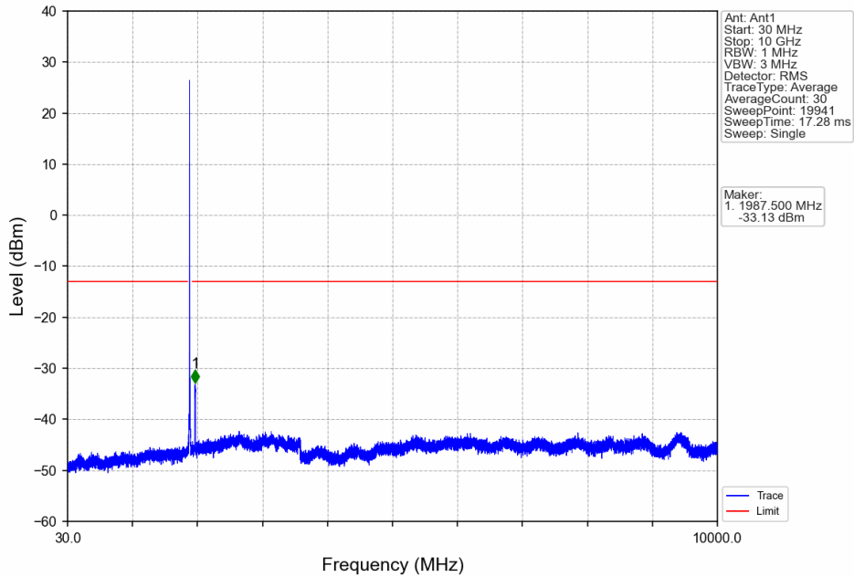
Band25_15MHz_QPSK_HCH_1907.5MHz_RB_1_0_NTNV
