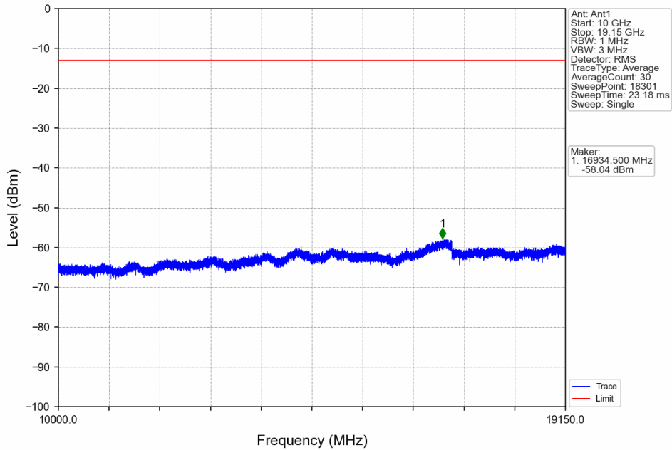
Band25_20MHz_16QAM_LCH_1860MHz_RB_100_0_NTNV
