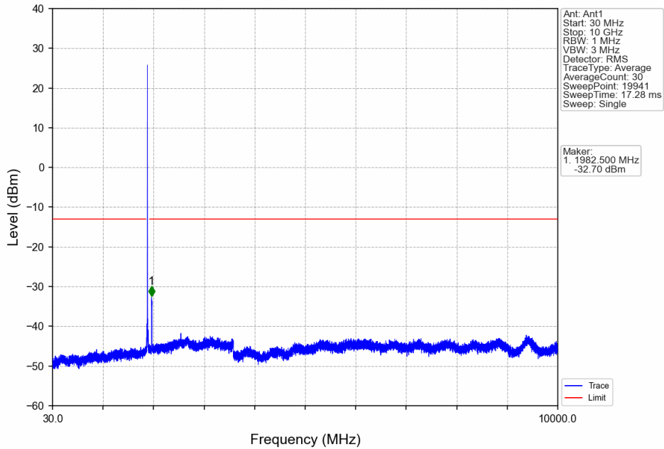
Band25_15MHz_16QAM_HCH_1907.5MHz_RB_1_0_NTNV
