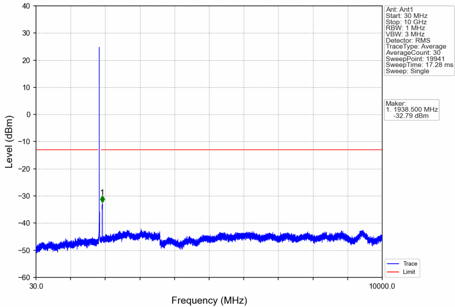
Band25_20MHz_16QAM_LCH_1860MHz_RB_1_0_NTNV
