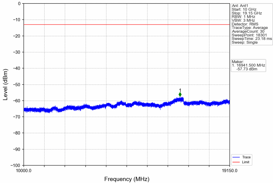
Band25_20MHz_64QAM_HCH_1905MHz_RB_1_0_NTNV
