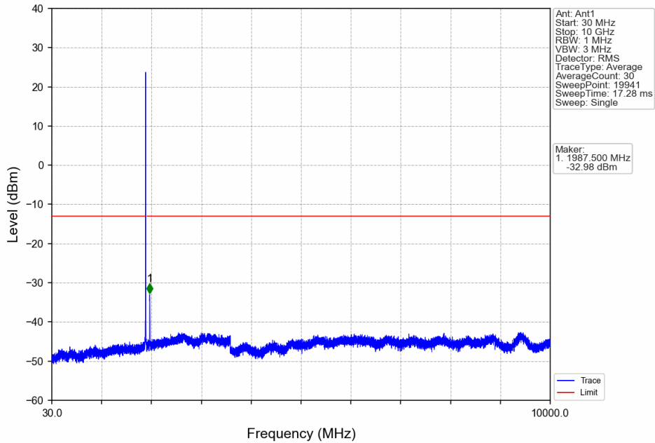
Band25_10MHz_16QAM_HCH_1910MHz_RB_1_0_NTNV
