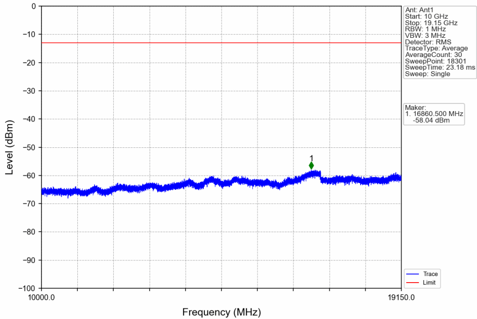
Band25_3MHz_64QAM_LCH_1851.5MHz_RB_1_0_NTNV
