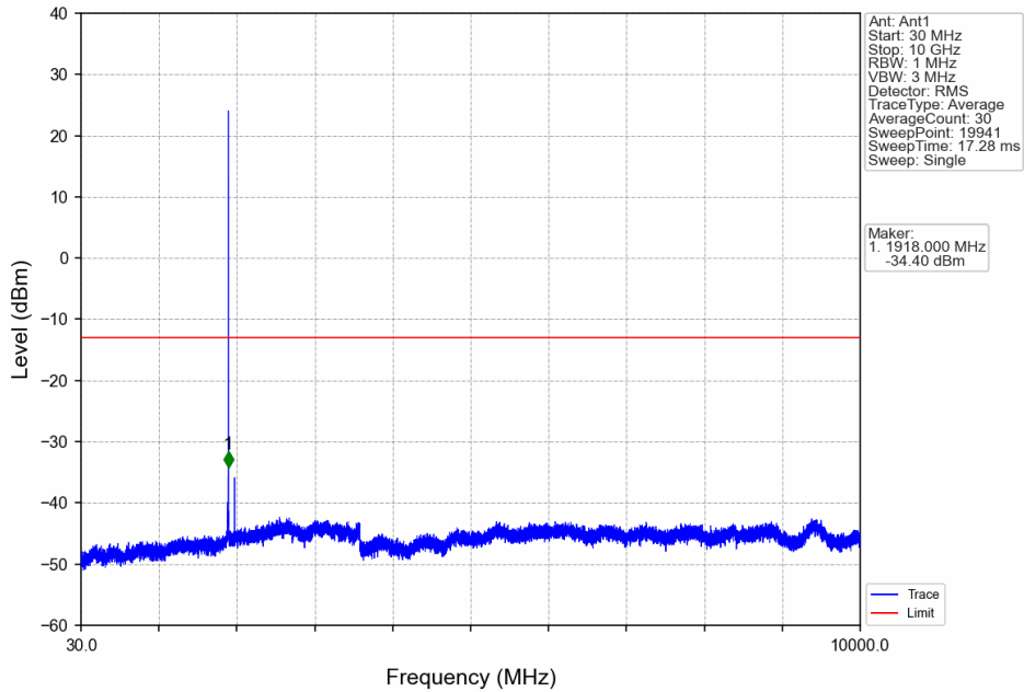
Band25_1.4MHz_64QAM_HCH_1914.3MHz_RB_1_0_NTNV
