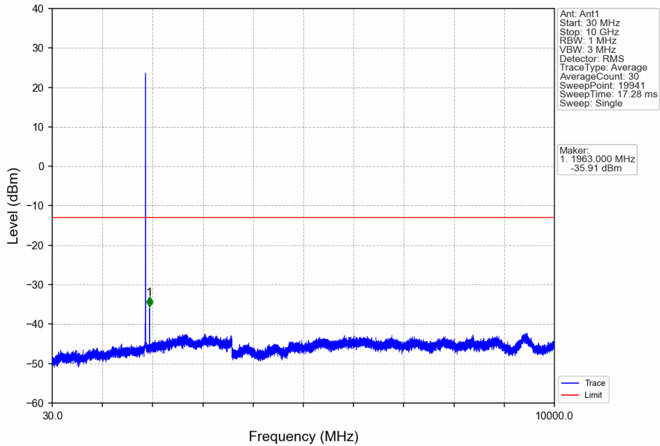
Band25_1.4MHz_16QAM_MCH_1882.5MHz_RB_1_0_NTNV
