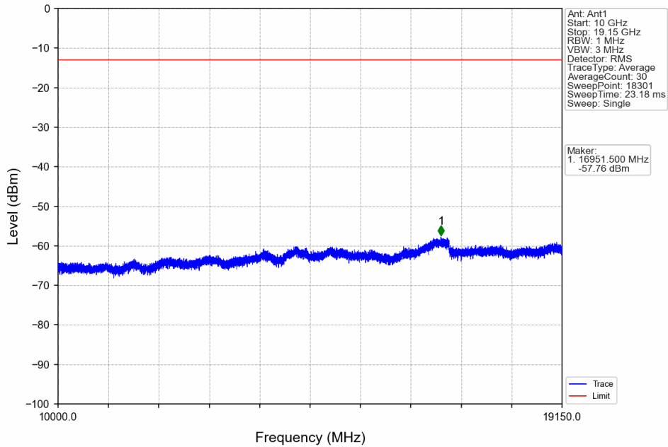
Band25_3MHz_64QAM_MCH_1882.5MHz_RB_1_0_NTNV
