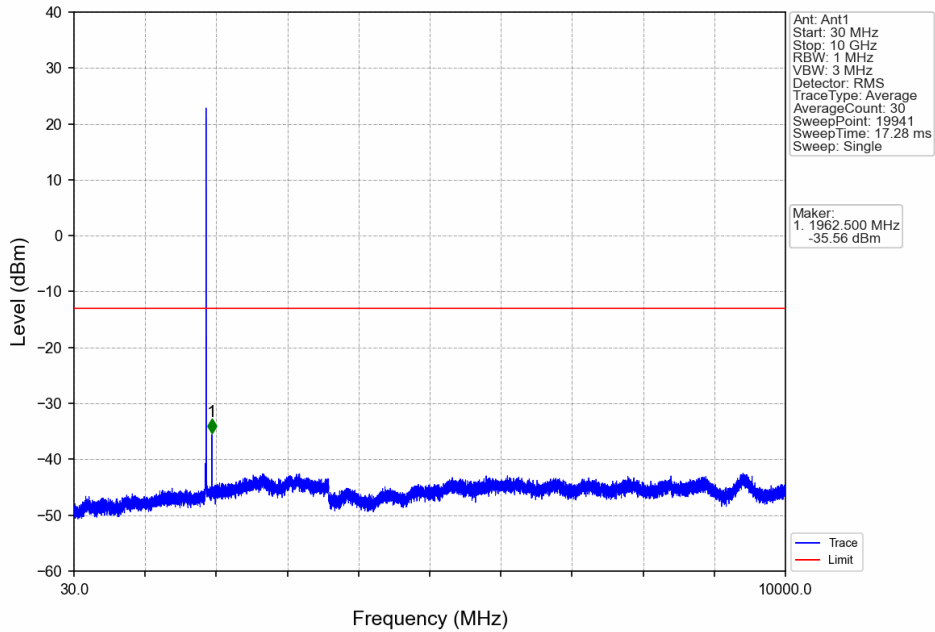
Band25_1.4MHz_64QAM_MCH_1882.5MHz_RB_1_0_NTNV
