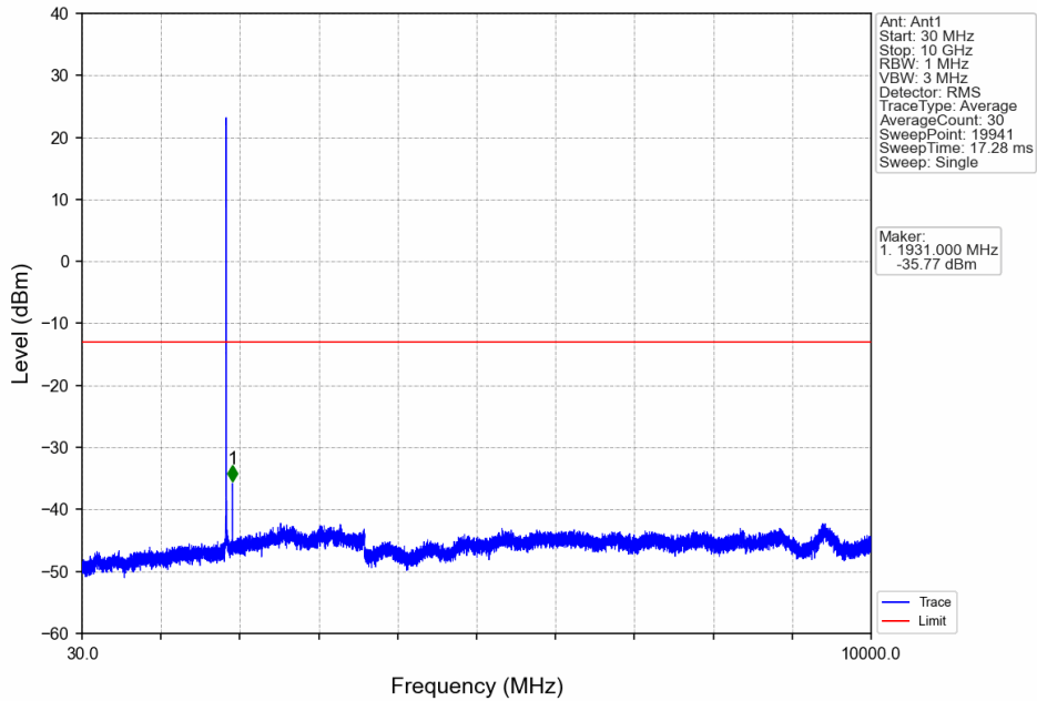
Band25_1.4MHz_64QAM_LCH_1850.7MHz_RB_1_0_NTNV
