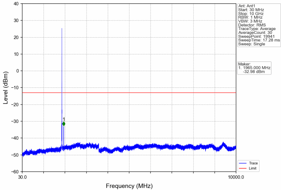
Band25_10MHz_QPSK_MCH_1882.5MHz_RB_1_0_NTNV
