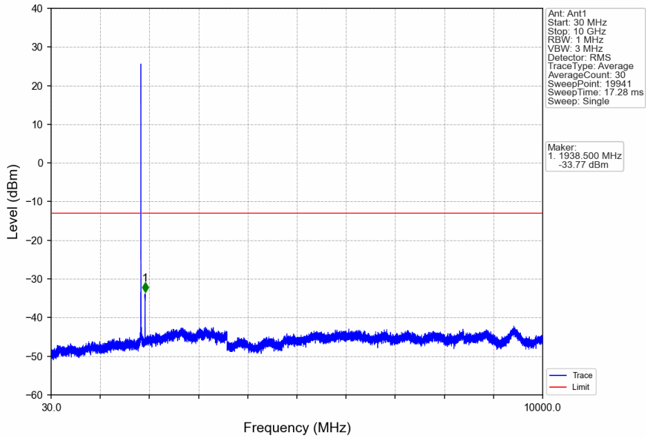
Band25_10MHz_16QAM_LCH_1855MHz_RB_1_0_NTNV
