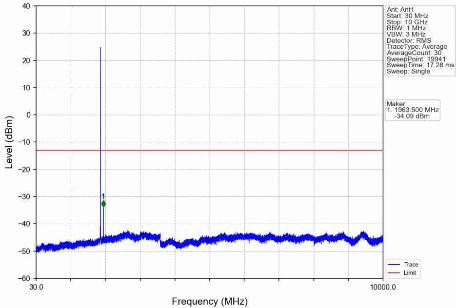
Band25_3MHz_64QAM_MCH_1882.5MHz_RB_1_0_NTNV
