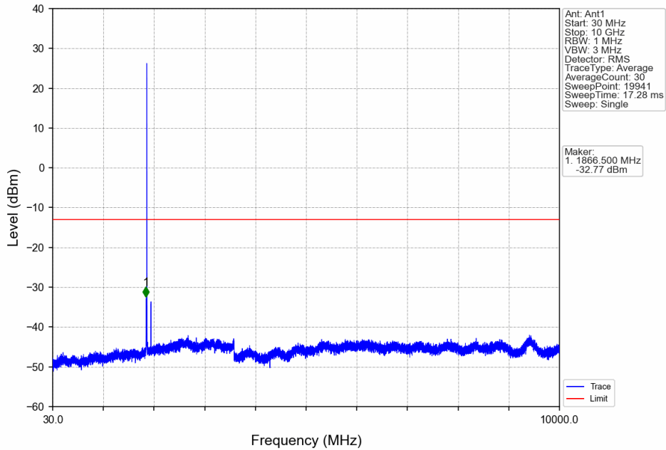
Band25_5MHz_QPSK_MCH_1882.5MHz_RB_1_0_NTNV
