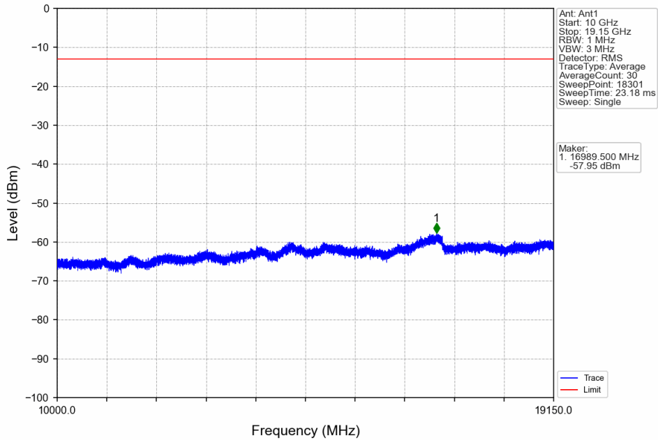
Band25_3MHz_16QAM_MCH_1882.5MHz_RB_1_0_NTNV
