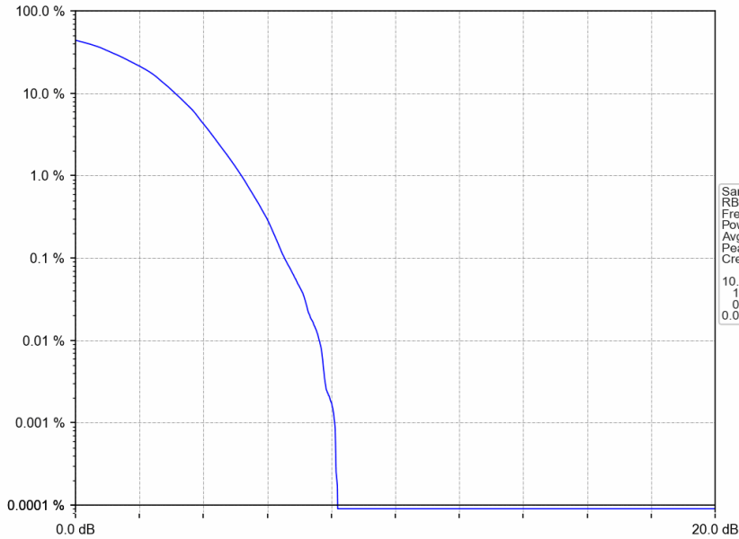
Band25_1.4MHz_64QAM_LCH_1850.7MHz_RB_6_0_NTNV
