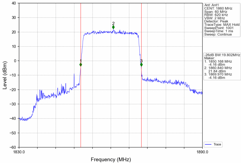
Band25_20MHz_16QAM_LCH_1860MHz_RB_100_0_NTNV
