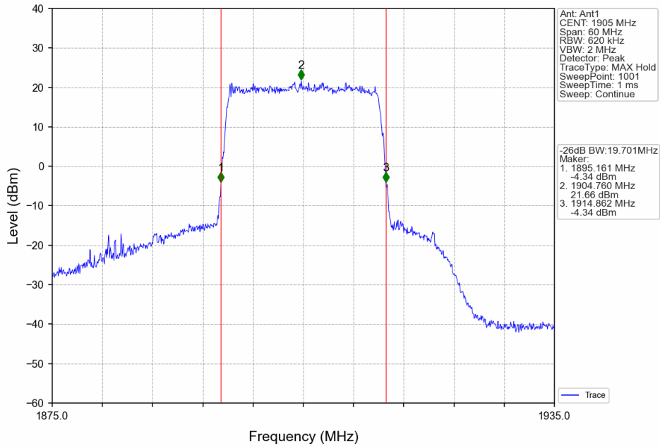
Band25_20MHz_16QAM_HCH_1905MHz_RB_100_0_NTNV
