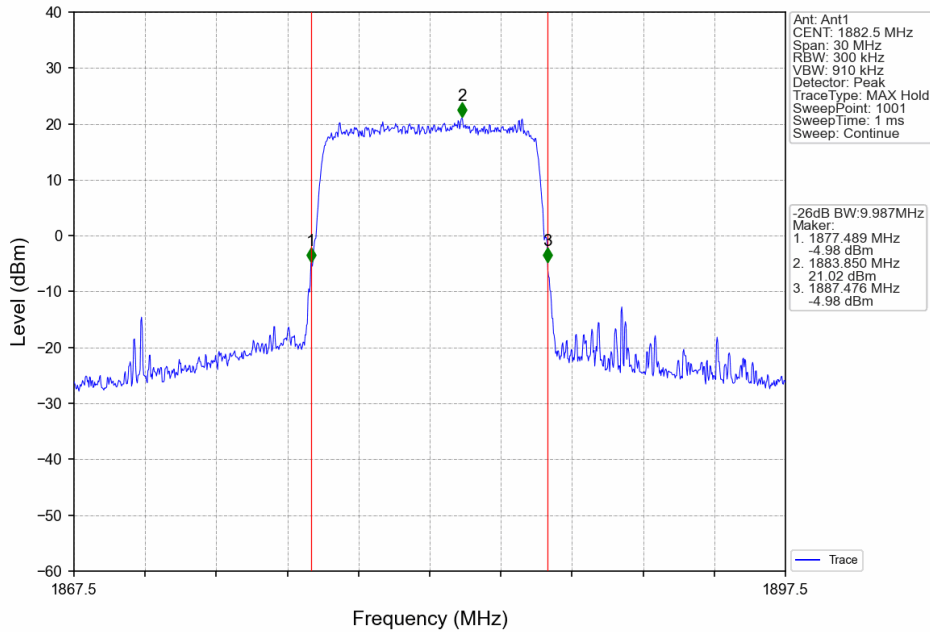
Band25_10MHz_16QAM_MCH_1882.5MHz_RB_50_0_NTNV
