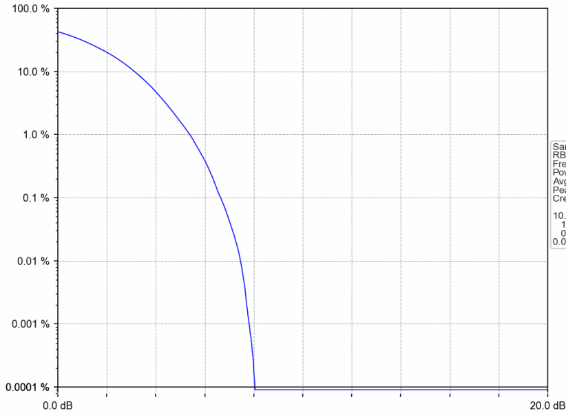
Band25_15MHz_64QAM_HCH_1907.5MHz_RB_75_0_NTNV
