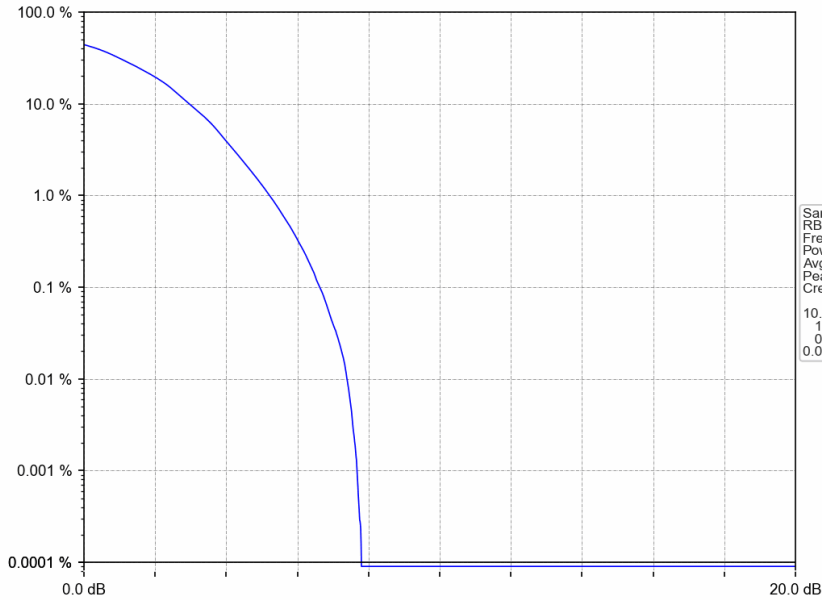
Band25_5MHz_64QAM_HCH_1912.5MHz_RB_25_0_NTNV
