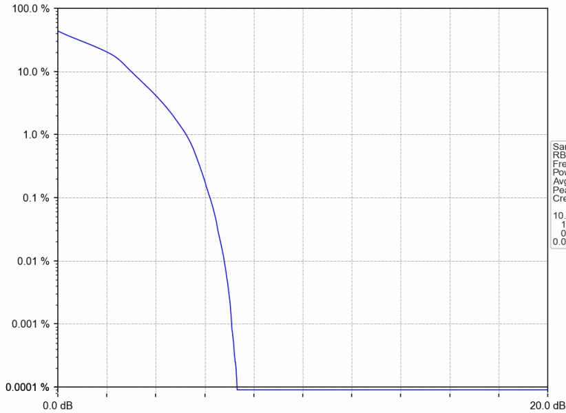
Band25_15MHz_16QAM_LCH_1857.5MHz_RB_75_0_NTNV
