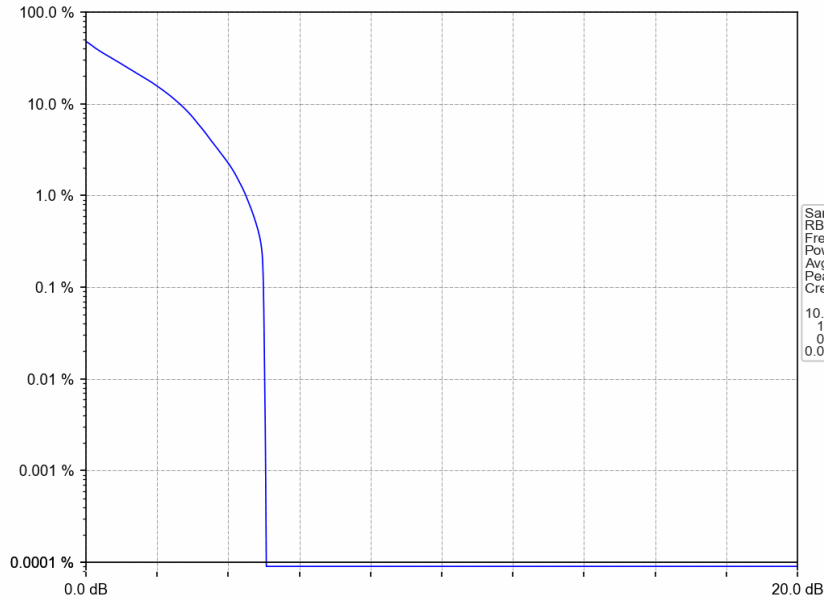
Band25_1.4MHz_QPSK_HCH_1914.3MHz_RB_6_0_NTNV
