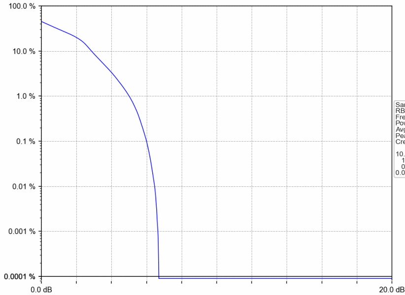
Band25_5MHz_16QAM_HCH_1912.5MHz_RB_25_0_NTNV
