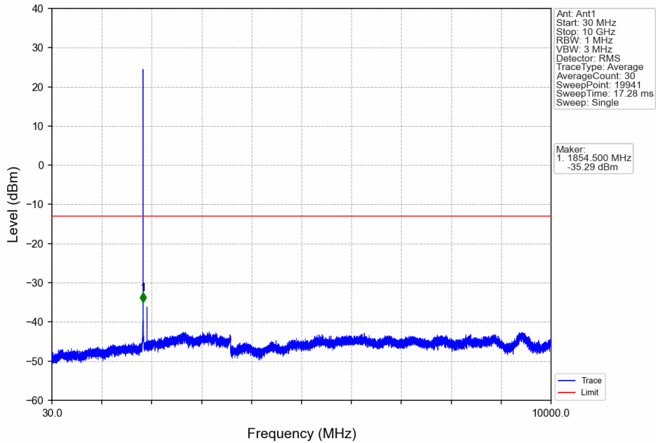
Band25_1.4MHz_16QAM_LCH_1850.7MHz_RB_1_0_NTNV
