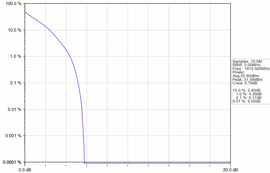
Band25_5MHz_QPSK_HCH_1912.5MHz_RB_25_0_NTNV
