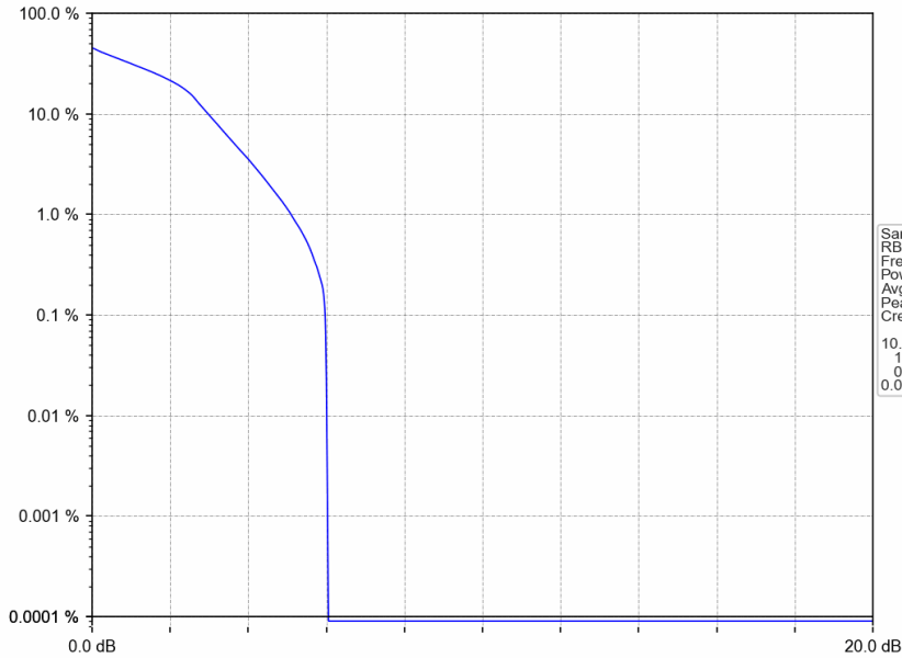
Band25_1.4MHz_16QAM_HCH_1914.3MHz_RB_6_0_NTNV
