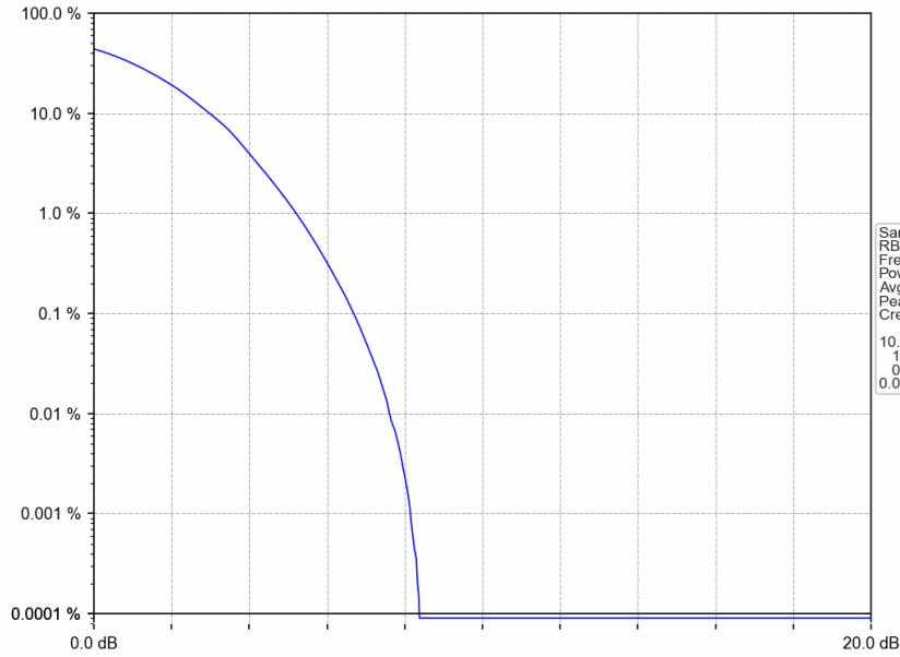
Band25_20MHz_64QAM_LCH_1860MHz_RB_100_0_NTNV
