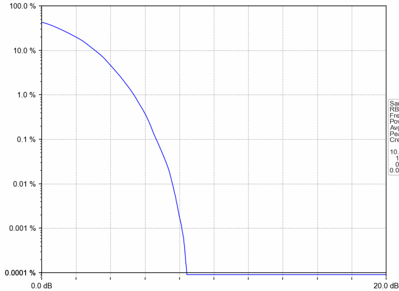
Band25_15MHz_64QAM_MCH_1882.5MHz_RB_75_0_NTNV
