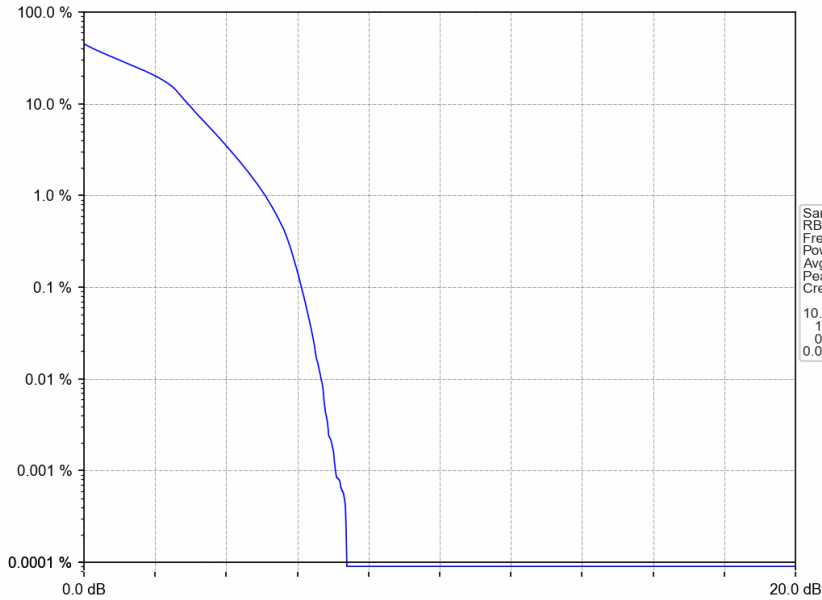
Band25_3MHz_16QAM_MCH_1882.5MHz_RB_15_0_NTNV
