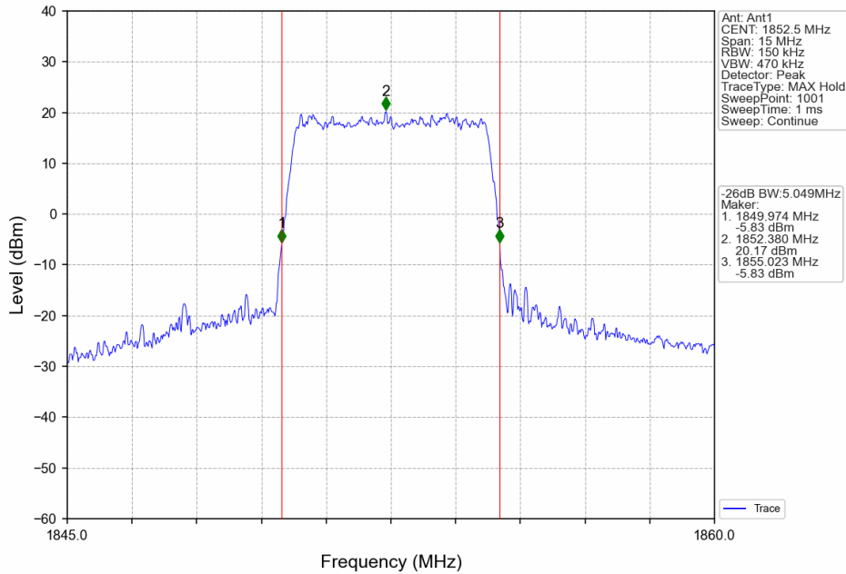
Band25_5MHz_64QAM_LCH_1852.5MHz_RB_25_0_NTNV
