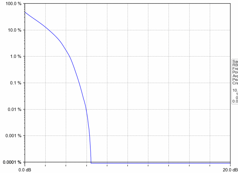
Band25_10MHz_QPSK_MCH_1882.5MHz_RB_50_0_NTNV
