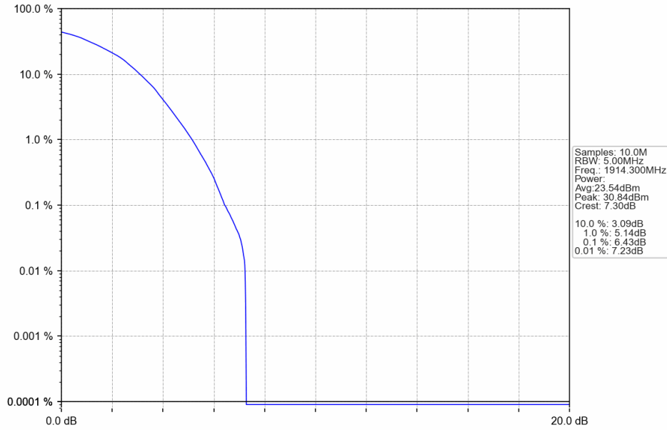
Band25_1.4MHz_64QAM_HCH_1914.3MHz_RB_6_0_NTNV
