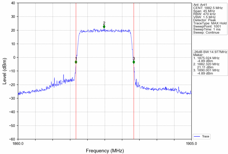
Band25_15MHz_16QAM_MCH_1882.5MHz_RB_75_0_NTNV
