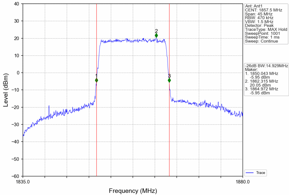
Band25_15MHz_64QAM_LCH_1857.5MHz_RB_75_0_NTNV
