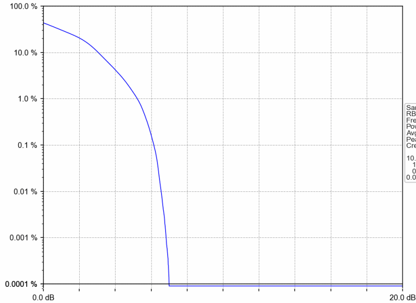
Band25_15MHz_16QAM_HCH_1907.5MHz_RB_75_0_NTNV
