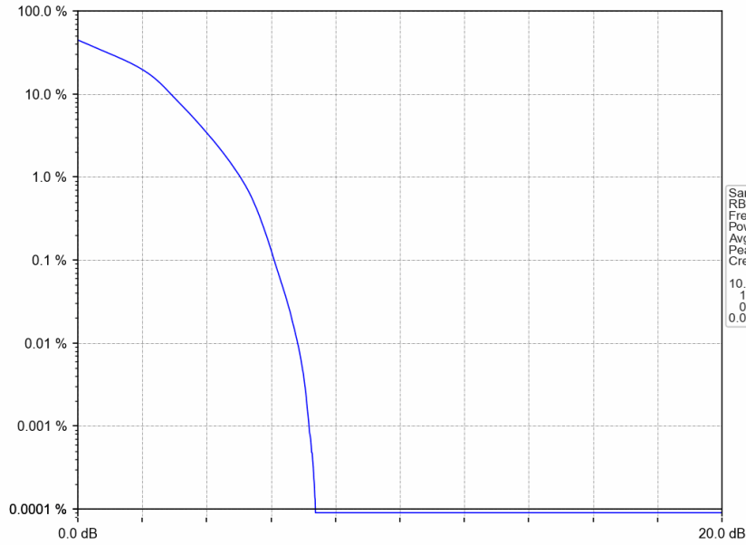
Band25_20MHz_16QAM_LCH_1860MHz_RB_100_0_NTNV
