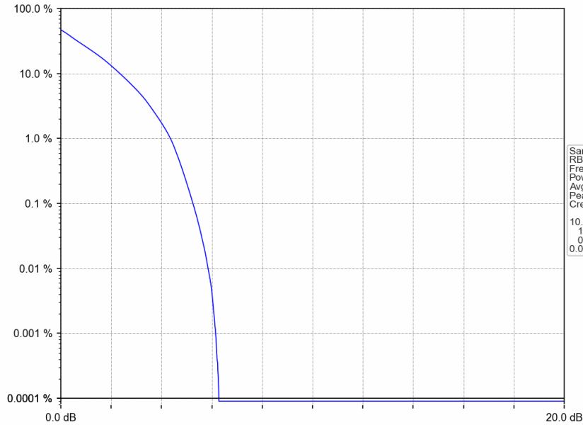
Band25_20MHz_QPSK_MCH_1882.5MHz_RB_100_0_NTNV
