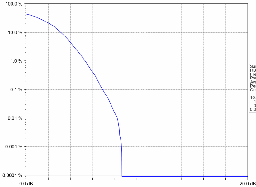
Band25_1.4MHz_64QAM_MCH_1882.5MHz_RB_6_0_NTNV
