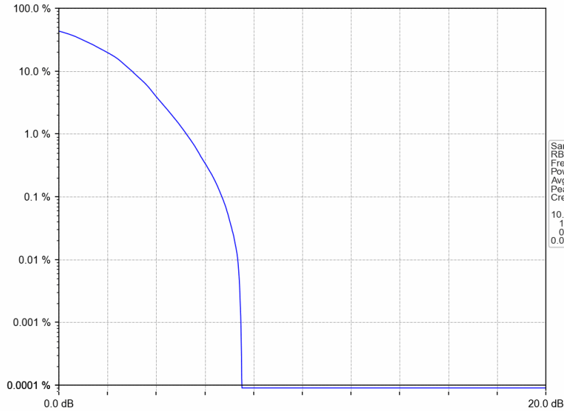
Band25_3MHz_64QAM_HCH_1913.5MHz_RB_15_0_NTNV
