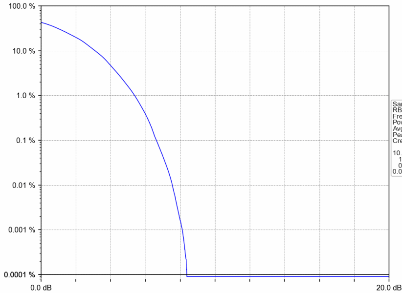
Band25_15MHz_64QAM_LCH_1857.5MHz_RB_75_0_NTNV
