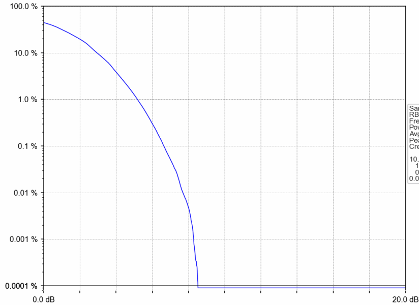
Band25_5MHz_64QAM_MCH_1882.5MHz_RB_25_0_NTNV
