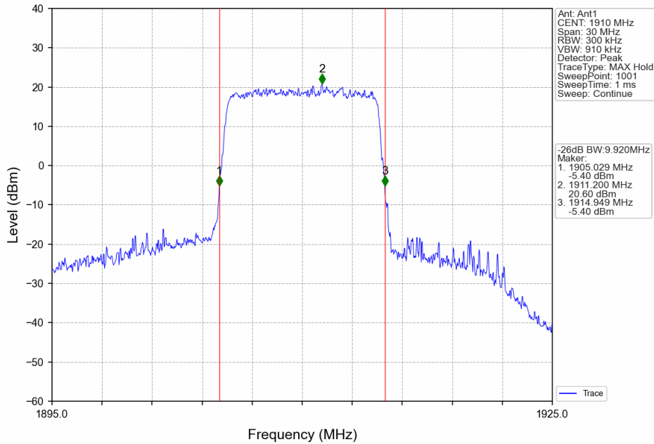
Band25_10MHz_64QAM_HCH_1910MHz_RB_50_0_NTNV
