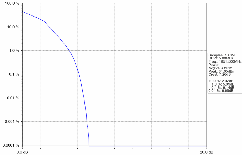
Band25_3MHz_16QAM_LCH_1851.5MHz_RB_15_0_NTNV
