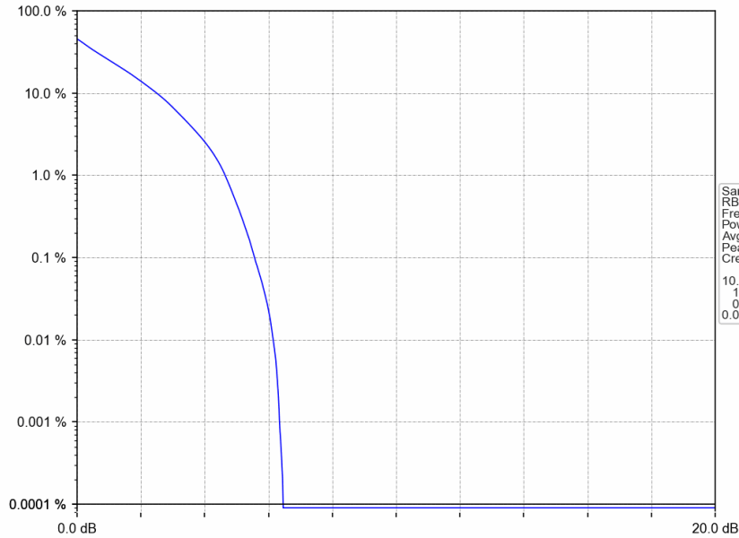
Band25_15MHz_QPSK_MCH_1882.5MHz_RB_75_0_NTNV
