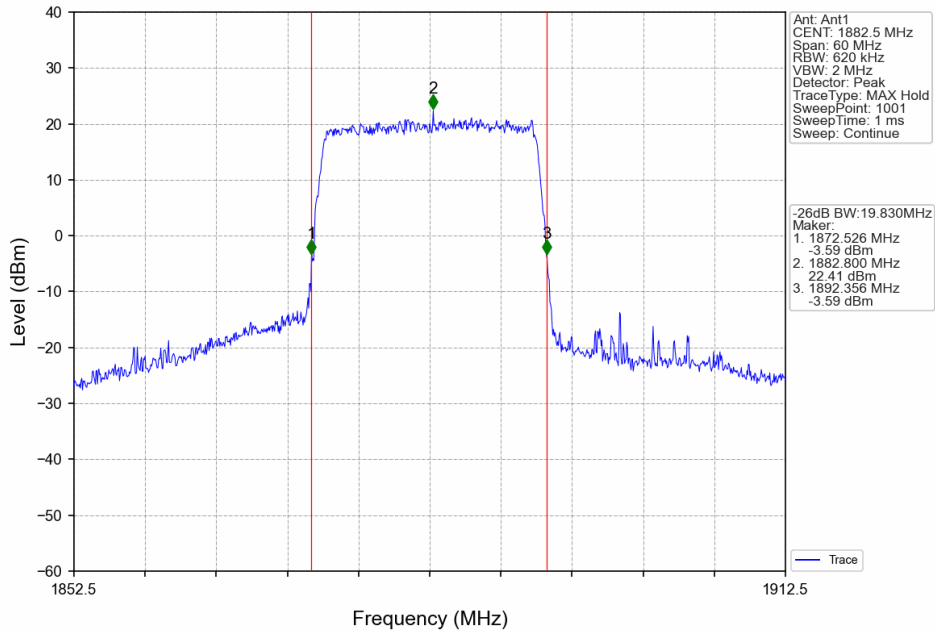
Band25_20MHz_16QAM_MCH_1882.5MHz_RB_100_0_NTNV
