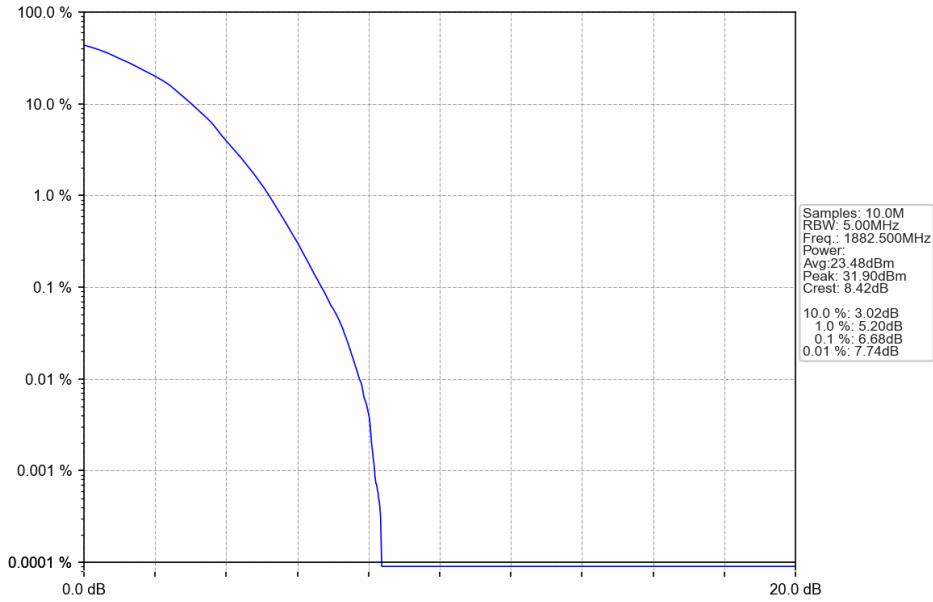
Band25_3MHz_64QAM_MCH_1882.5MHz_RB_15_0_NTNV
