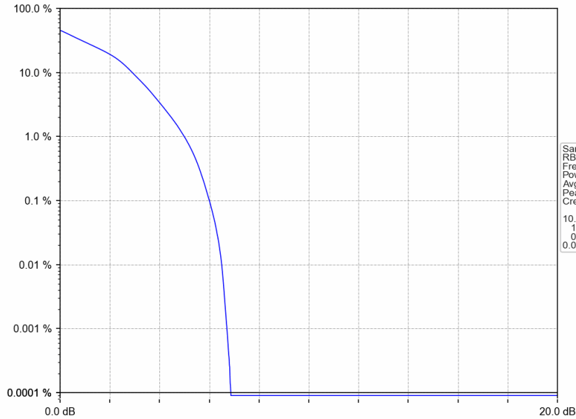
Band25_10MHz_16QAM_HCH_1910MHz_RB_50_0_NTNV
