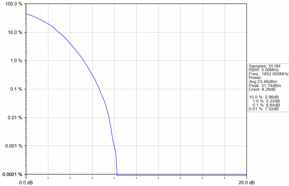
Band25_5MHz_64QAM_LCH_1852.5MHz_RB_25_0_NTNV
