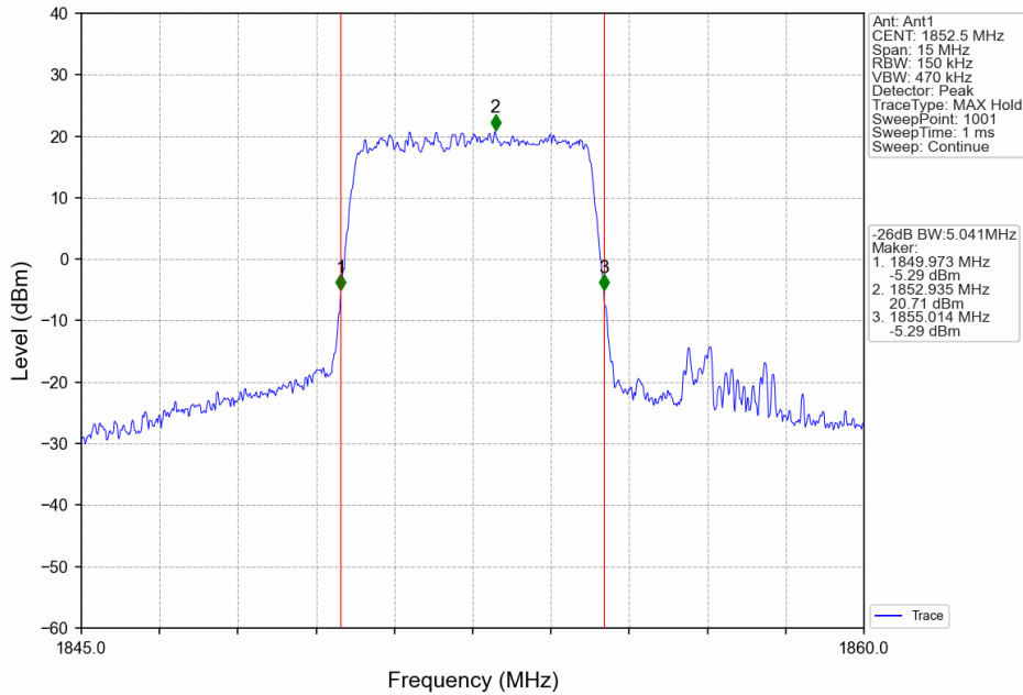
Band25_5MHz_16QAM_LCH_1852.5MHz_RB_25_0_NTNV
