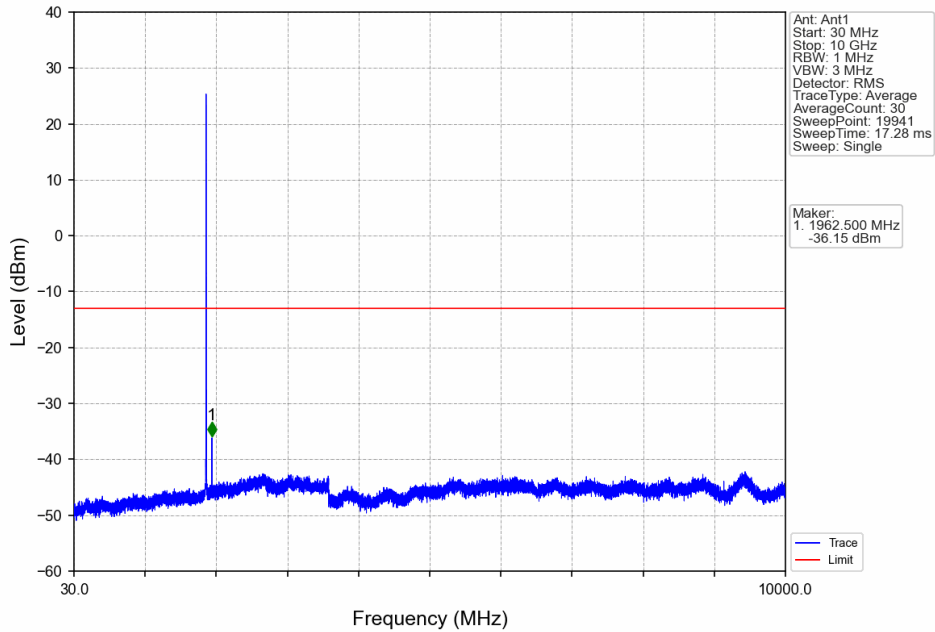
Band25_1.4MHz_QPSK_MCH_1882.5MHz_RB_1_0_NTNV
