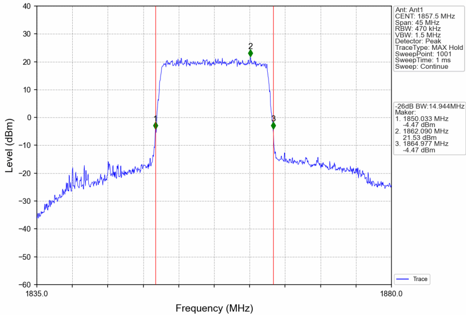
Band25_15MHz_16QAM_LCH_1857.5MHz_RB_75_0_NTNV
