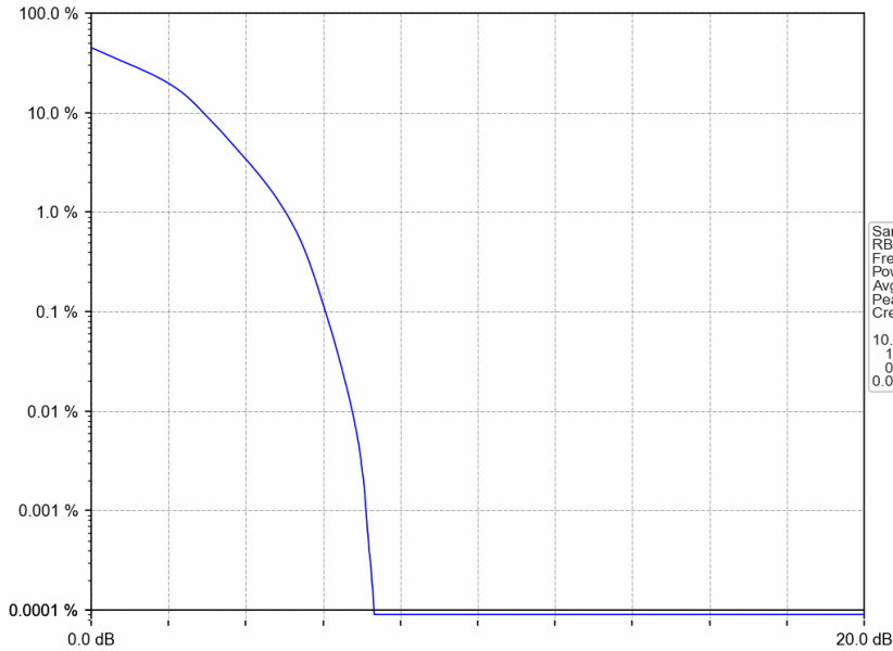
Band25_20MHz_16QAM_MCH_1882.5MHz_RB_100_0_NTNV
