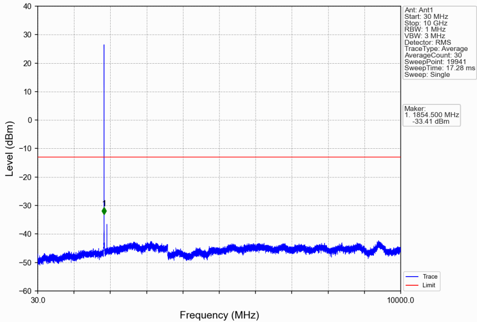
Band25_1.4MHz_QPSK_LCH_1850.7MHz_RB_1_0_NTNV
