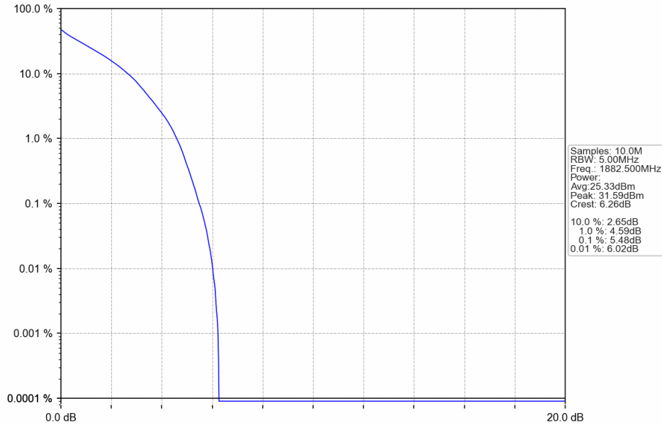
Band25_1.4MHz_QPSK_MCH_1882.5MHz_RB_6_0_NTNV
