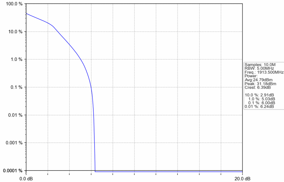
Band25_3MHz_16QAM_HCH_1913.5MHz_RB_15_0_NTNV
