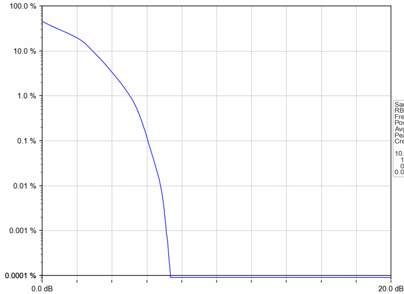
Band25_10MHz_16QAM_LCH_1855MHz_RB_50_0_NTNV
