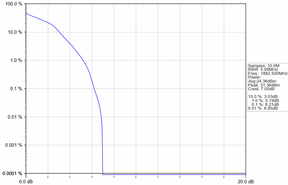
Band25_1.4MHz_16QAM_MCH_1882.5MHz_RB_6_0_NTNV
