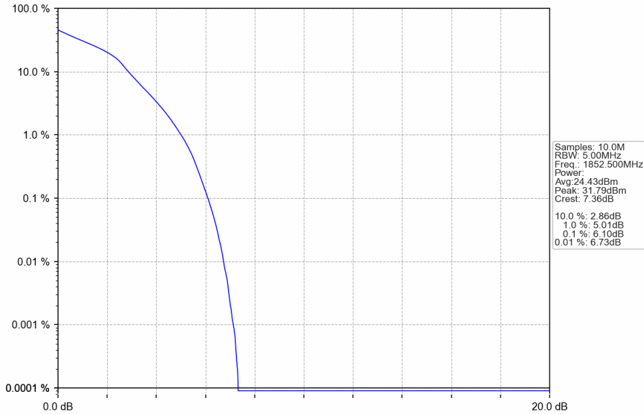
Band25_5MHz_16QAM_LCH_1852.5MHz_RB_25_0_NTNV
