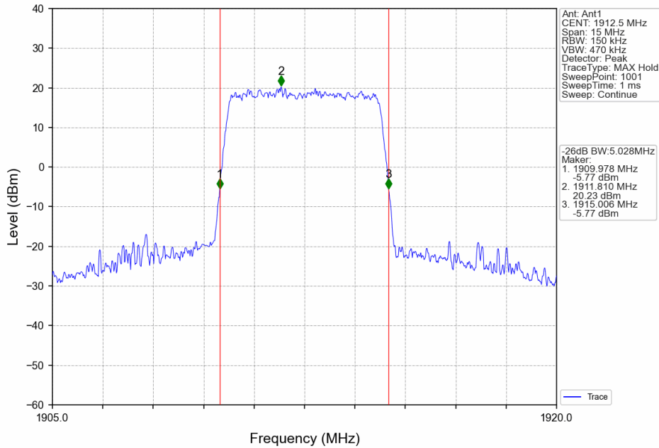
Band25_5MHz_64QAM_HCH_1912.5MHz_RB_25_0_NTNV
