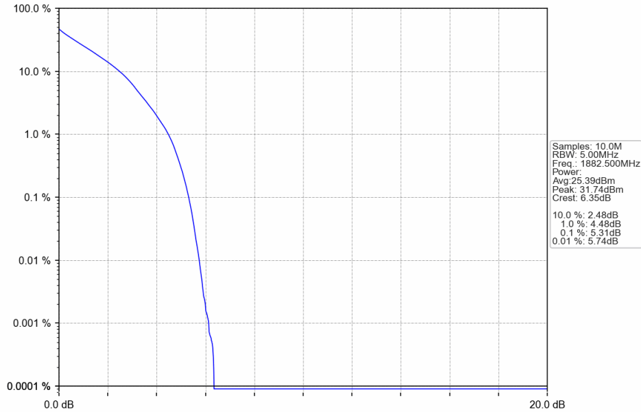
Band25_3MHz_QPSK_MCH_1882.5MHz_RB_15_0_NTNV
