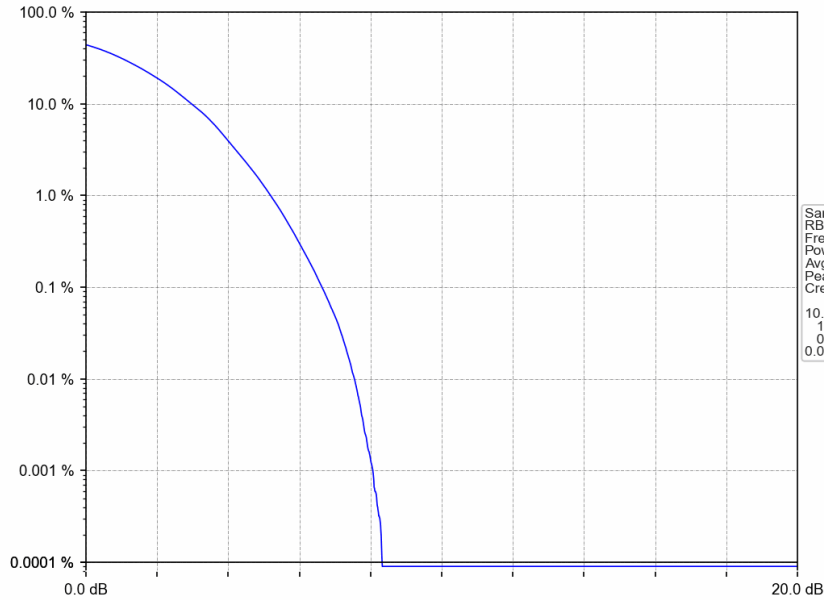
Band25_20MHz_64QAM_MCH_1882.5MHz_RB_100_0_NTNV
