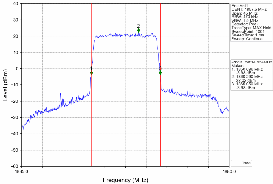
Band25_15MHz_QPSK_LCH_1857.5MHz_RB_75_0_NTNV
