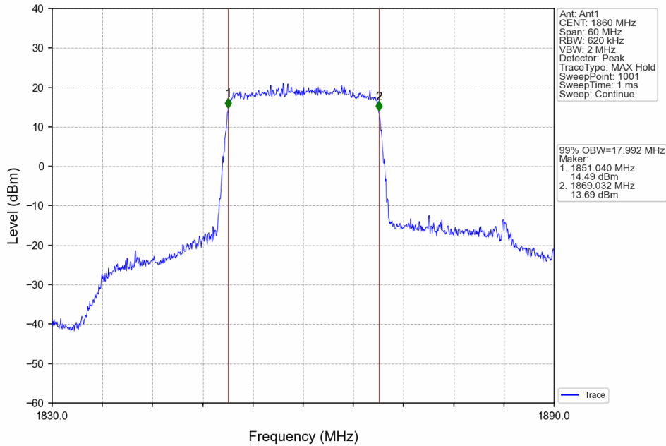
Band25_20MHz_64QAM_LCH_1860MHz_RB_100_0_NTNV
