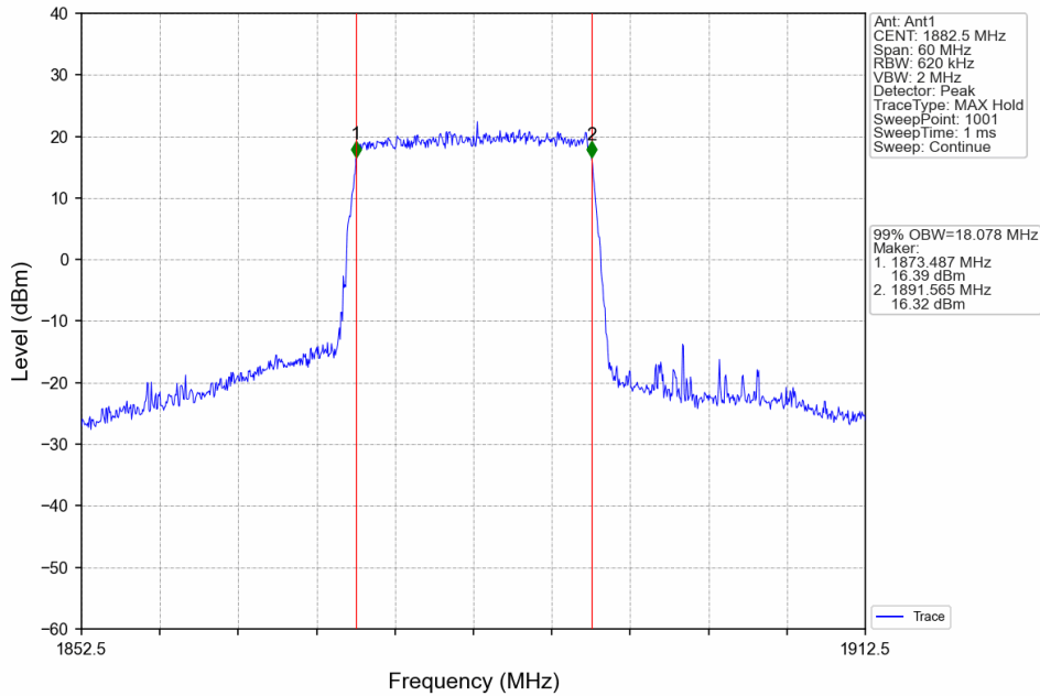
Band25_20MHz_16QAM_MCH_1882.5MHz_RB_100_0_NTNV
