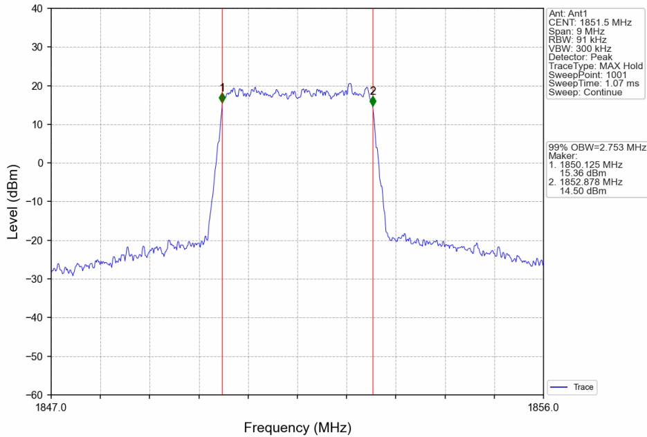
Band25_3MHz_64QAM_LCH_1851.5MHz_RB_15_0_NTNV
