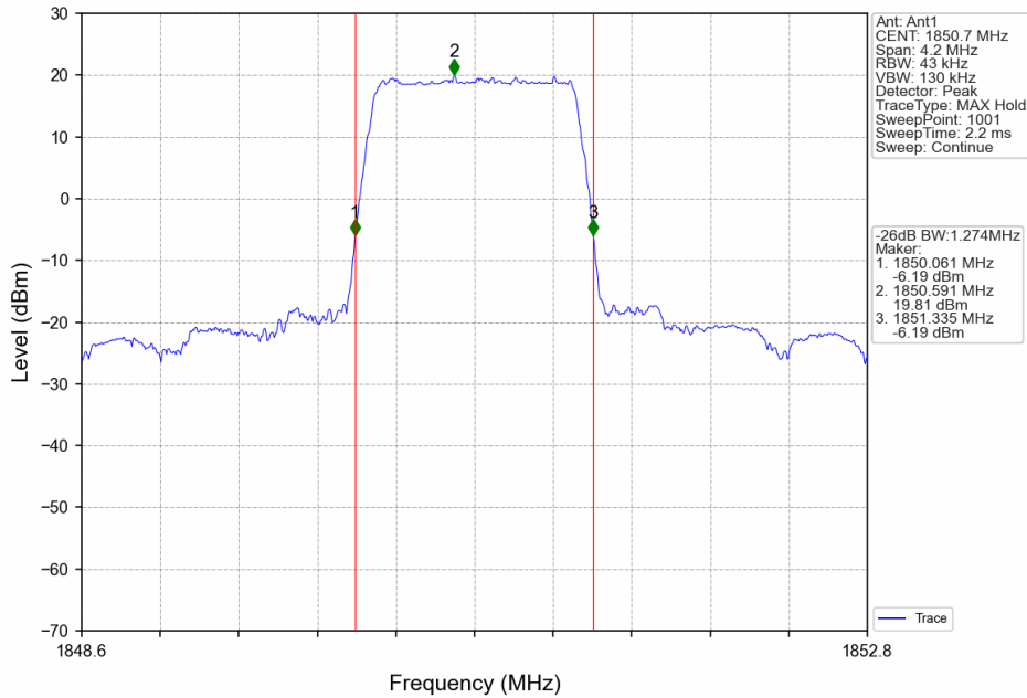
Band25_1.4MHz_64QAM_LCH_1850.7MHz_RB_6_0_NTNV
