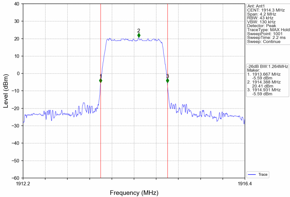
Band25_1.4MHz_64QAM_HCH_1914.3MHz_RB_6_0_NTNV
