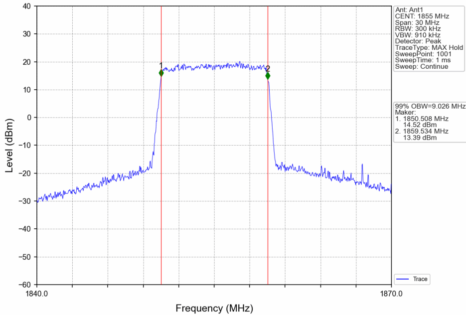
Band25_10MHz_64QAM_LCH_1855MHz_RB_50_0_NTNV
