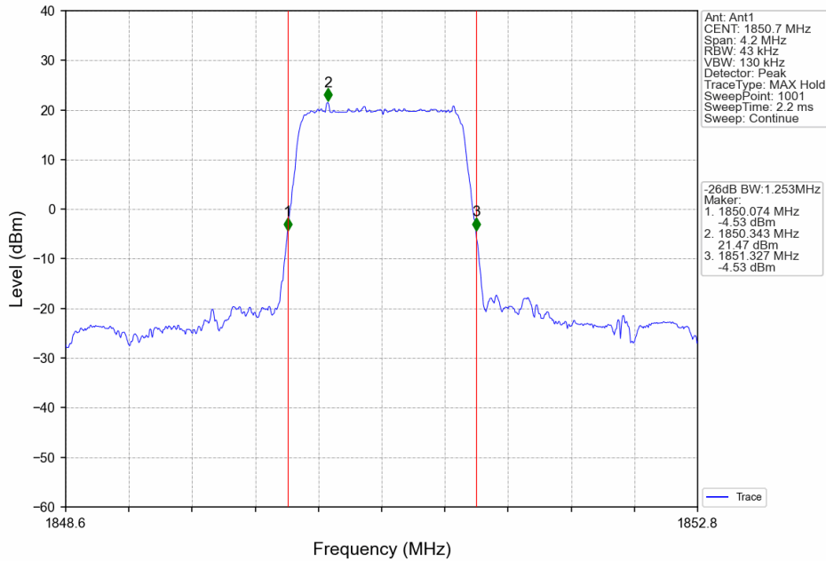
Band25_1.4MHz_16QAM_LCH_1850.7MHz_RB_6_0_NTNV
