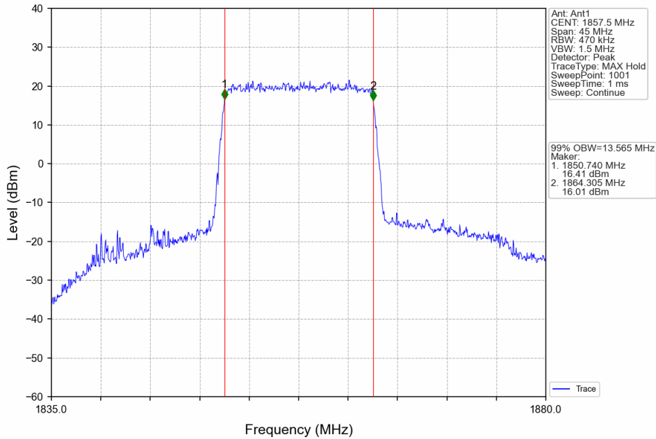
Band25_15MHz_16QAM_LCH_1857.5MHz_RB_75_0_NTNV
