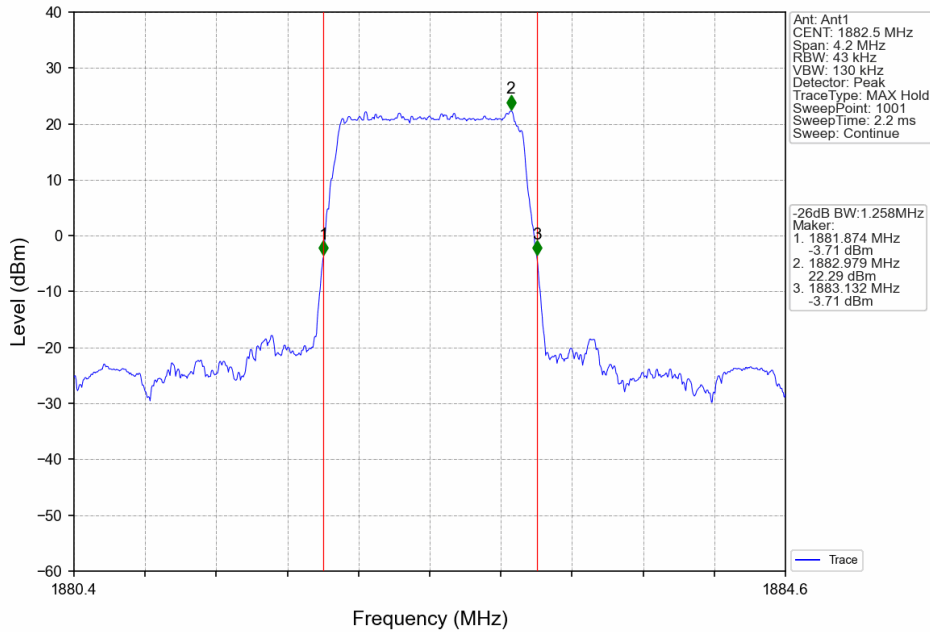
Band25_1.4MHz_QPSK_MCH_1882.5MHz_RB_6_0_NTNV
