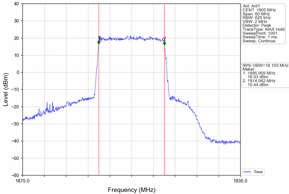
Band25_20MHz_16QAM_HCH_1905MHz_RB_100_0_NTNV
