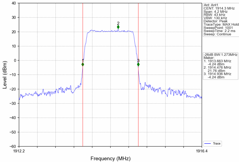
Band25_1.4MHz_16QAM_HCH_1914.3MHz_RB_6_0_NTNV
