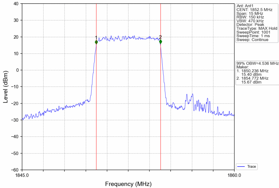
Band25_5MHz_16QAM_LCH_1852.5MHz_RB_25_0_NTNV
