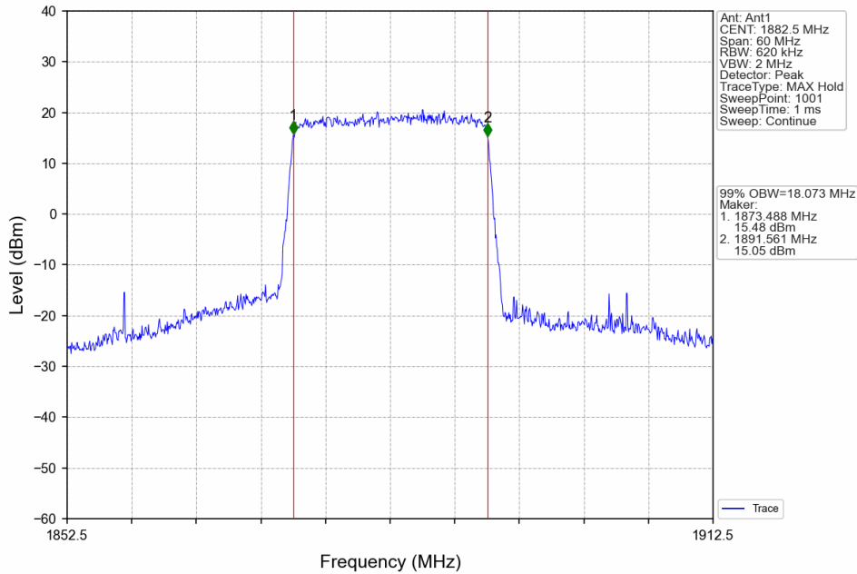
Band25_20MHz_64QAM_MCH_1882.5MHz_RB_100_0_NTNV
