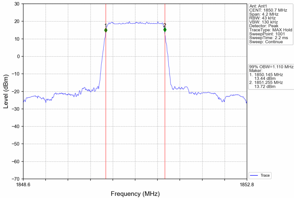
Band25_1.4MHz_64QAM_LCH_1850.7MHz_RB_6_0_NTNV
