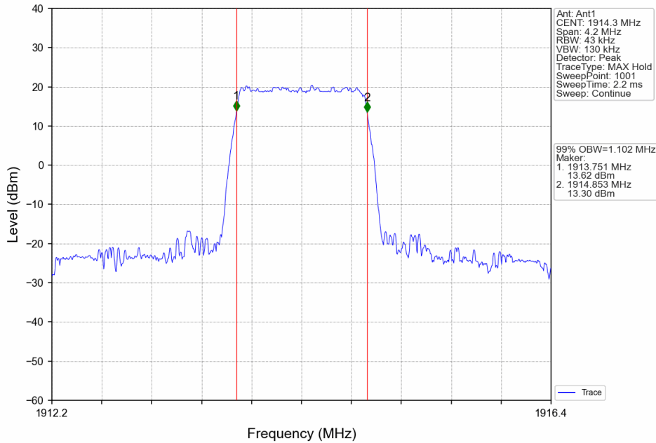
Band25_1.4MHz_64QAM_HCH_1914.3MHz_RB_6_0_NTNV
