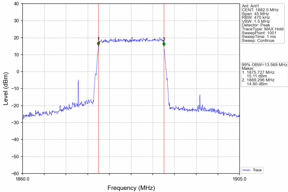
Band25_15MHz_64QAM_MCH_1882.5MHz_RB_75_0_NTNV
