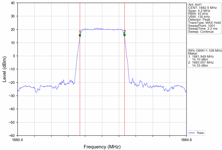
Band25_1.4MHz_16QAM_MCH_1882.5MHz_RB_6_0_NTNV
