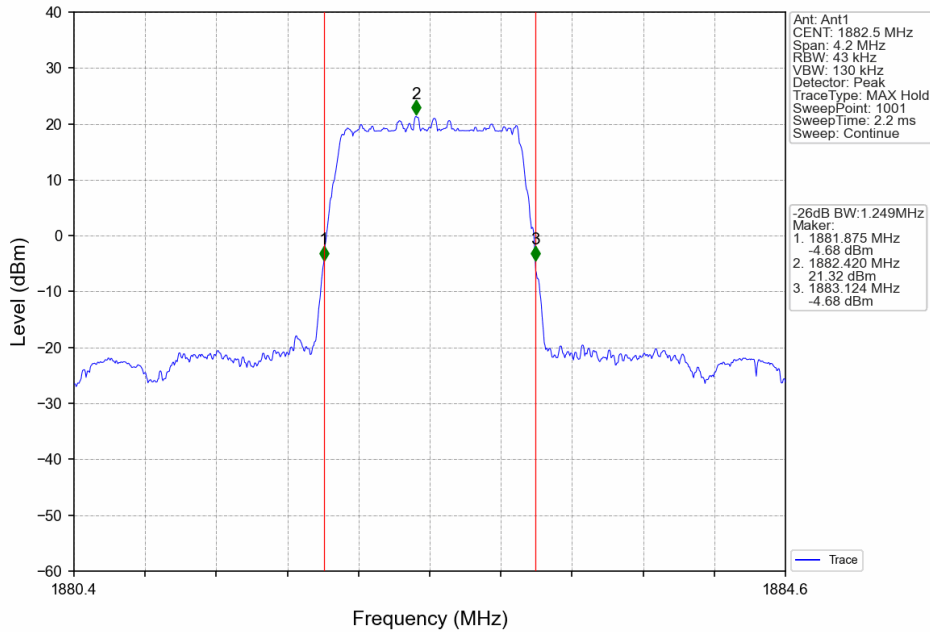
Band25_1.4MHz_64QAM_MCH_1882.5MHz_RB_6_0_NTNV
