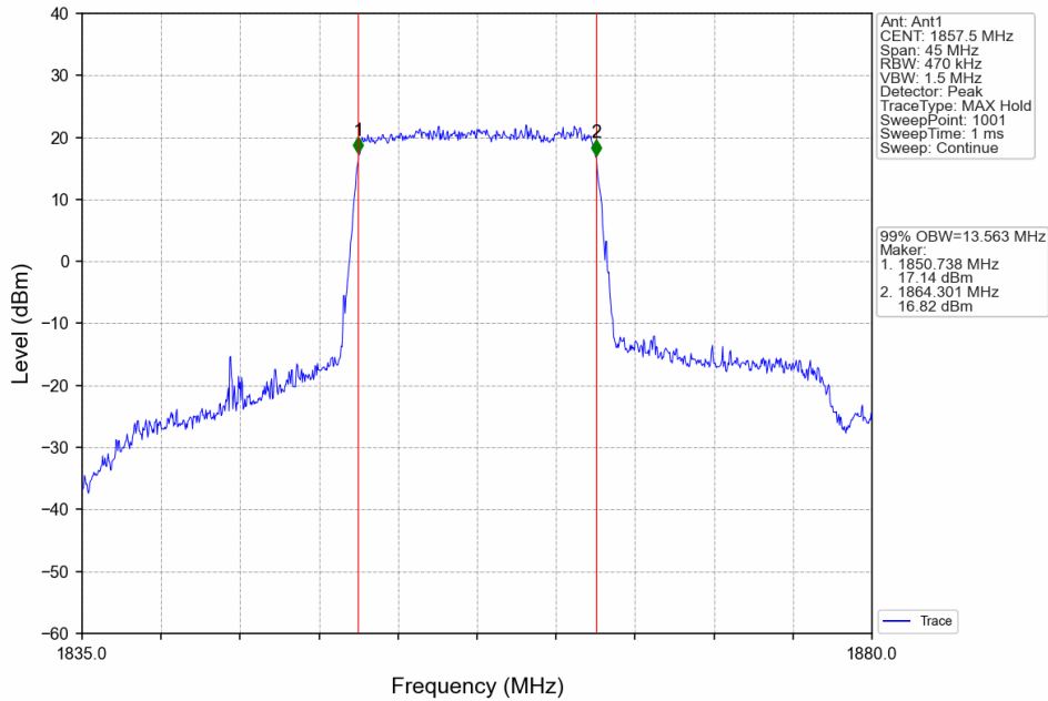
Band25_15MHz_QPSK_LCH_1857.5MHz_RB_75_0_NTNV
