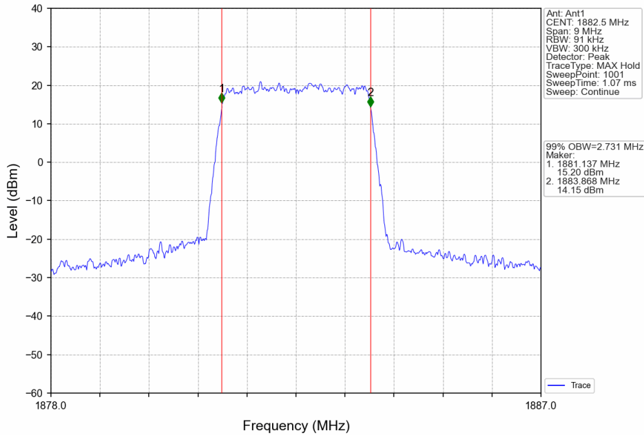
Band25_3MHz_16QAM_MCH_1882.5MHz_RB_15_0_NTNV
