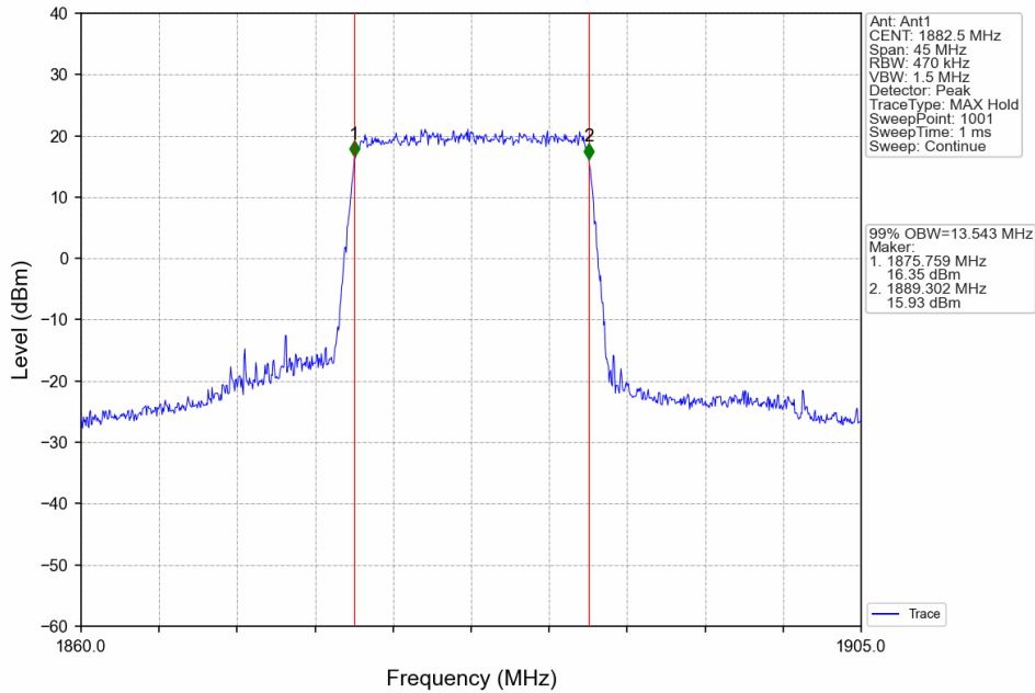
Band25_15MHz_16QAM_MCH_1882.5MHz_RB_75_0_NTNV
