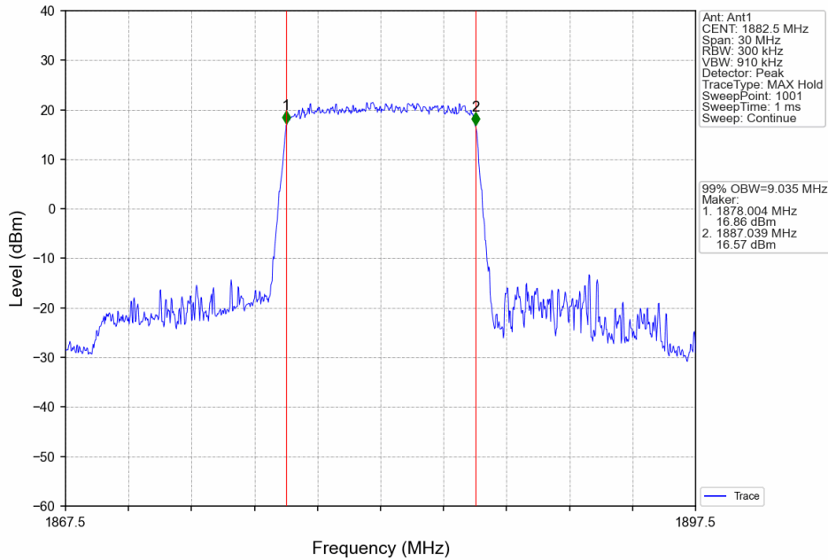
Band25_10MHz_QPSK_MCH_1882.5MHz_RB_50_0_NTNV
