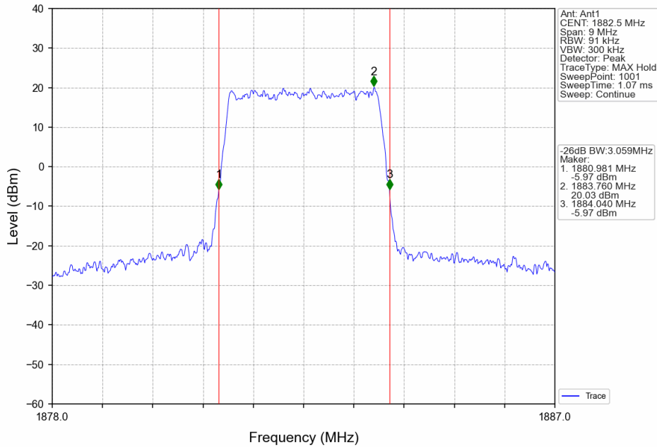
Band25_3MHz_64QAM_MCH_1882.5MHz_RB_15_0_NTNV
