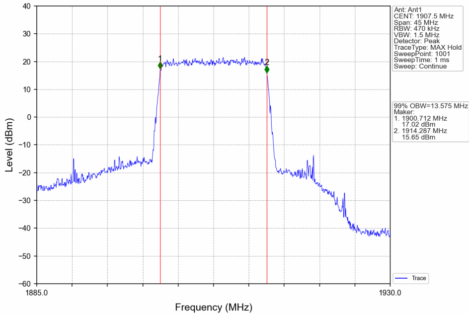
Band25_15MHz_16QAM_HCH_1907.5MHz_RB_75_0_NTNV
