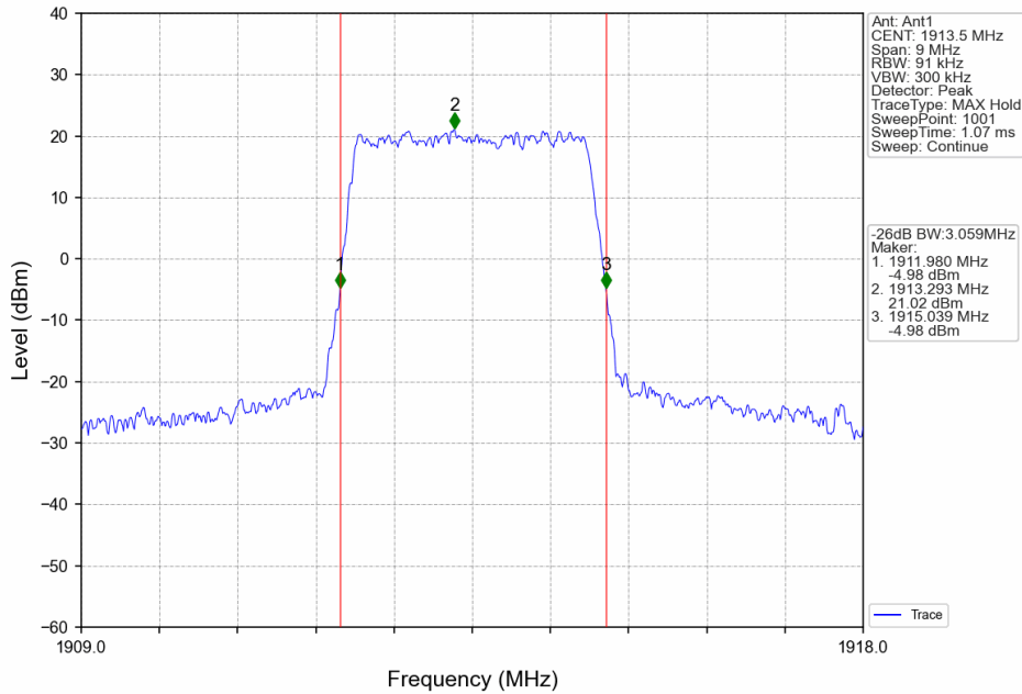
Band25_3MHz_16QAM_HCH_1913.5MHz_RB_15_0_NTNV
