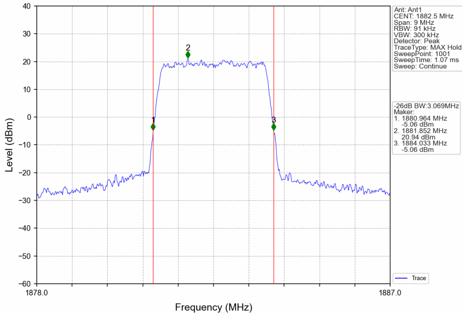
Band25_3MHz_16QAM_MCH_1882.5MHz_RB_15_0_NTNV
