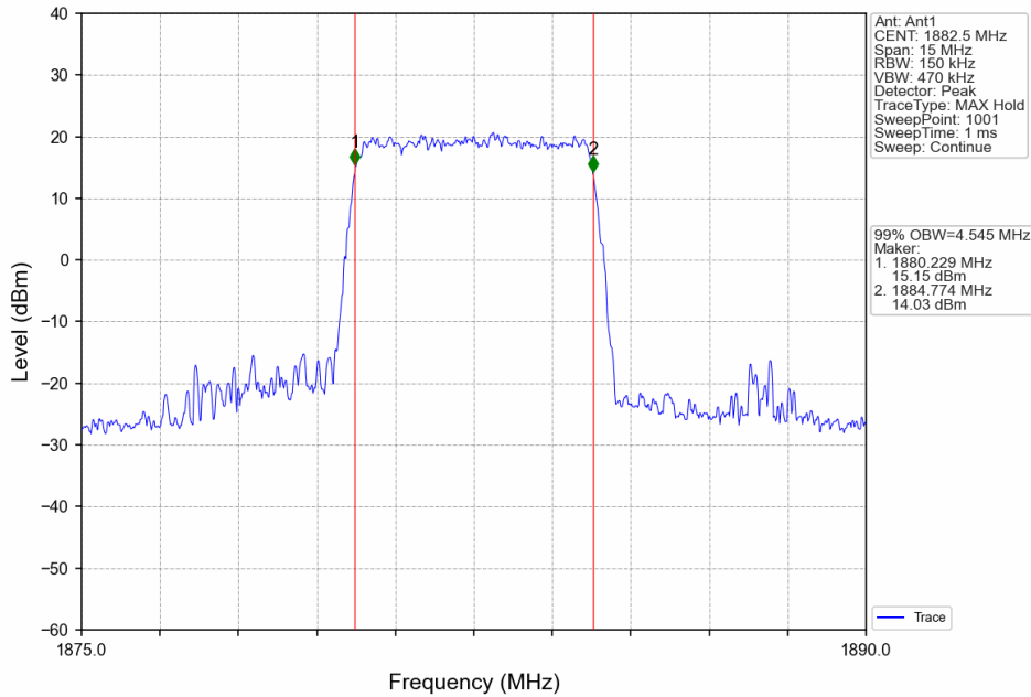
Band25_5MHz_16QAM_MCH_1882.5MHz_RB_25_0_NTNV
