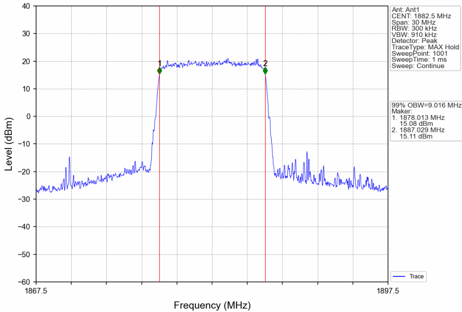
Band25_10MHz_16QAM_MCH_1882.5MHz_RB_50_0_NTNV
