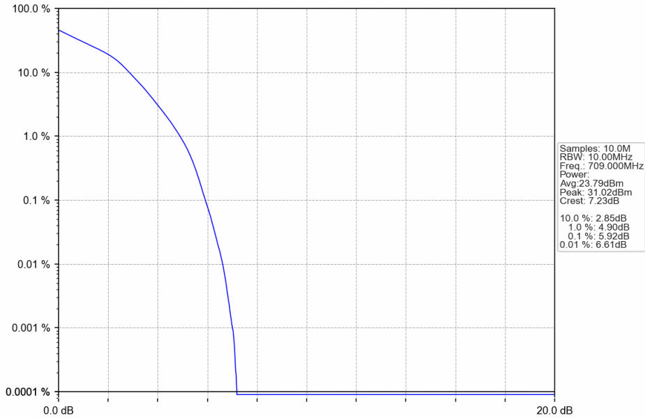
Band17_10MHz_16QAM_LCH_709MHz_RB_50_0_NTNV
