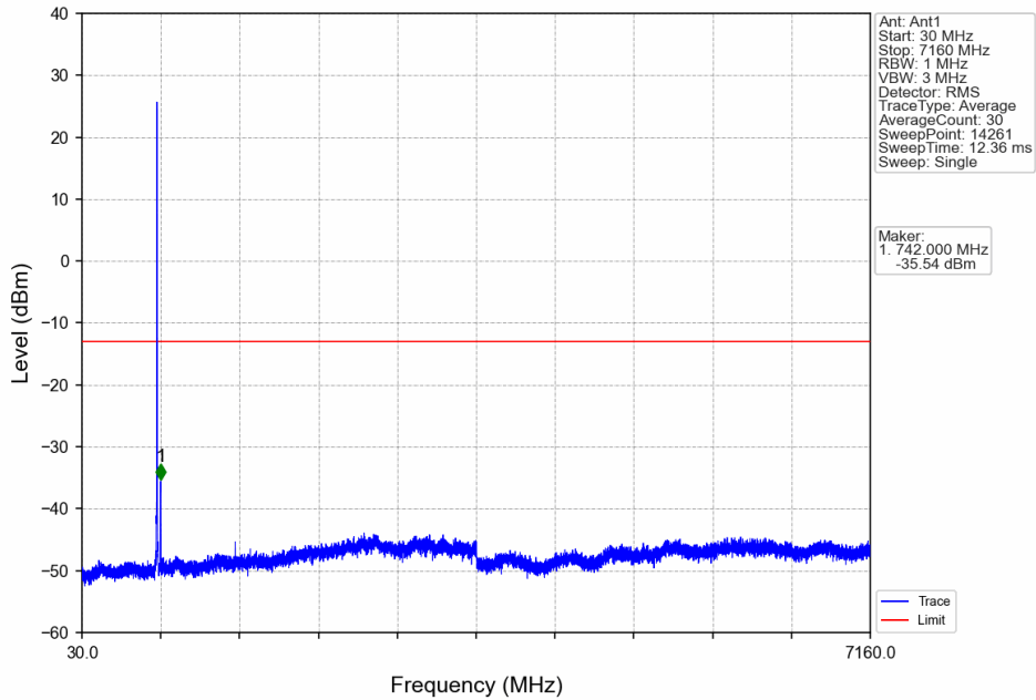
Band17_5MHz_16QAM_MCH_710MHz_RB_1_0_NTNV
