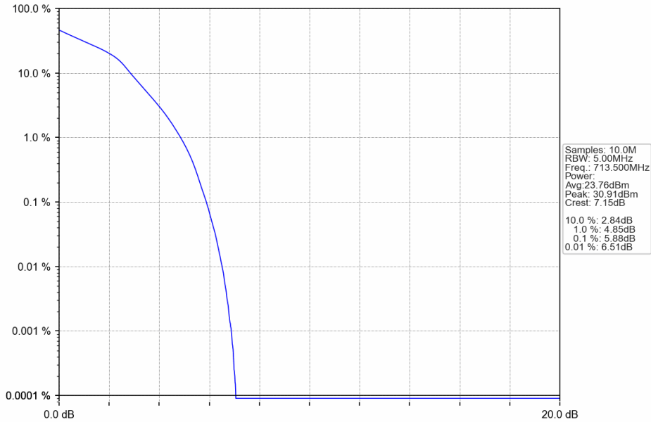
Band17_5MHz_16QAM_HCH_713.5MHz_RB_25_0_NTNV
