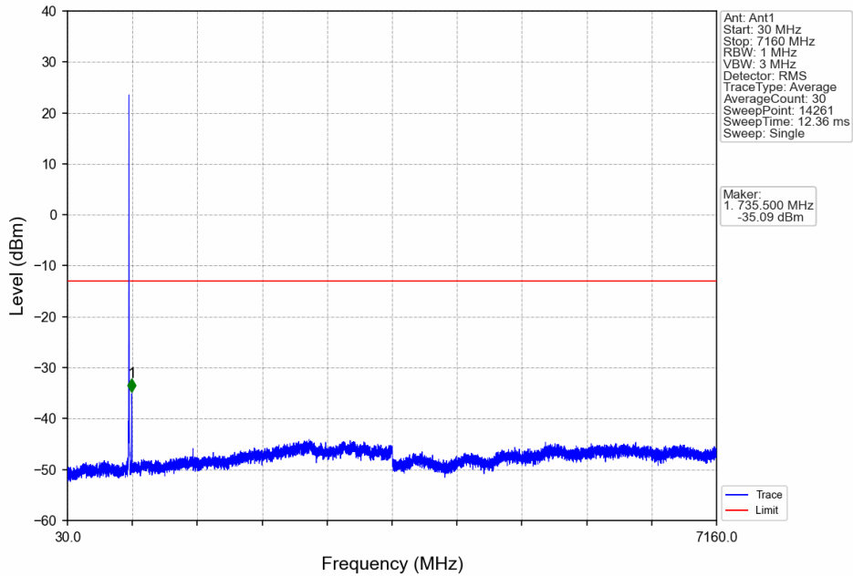
Band17_5MHz_64QAM_LCH_706.5MHz_RB_1_0_NTNV
