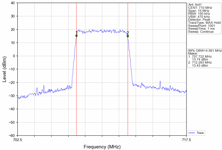
Band17_5MHz_16QAM_MCH_710MHz_RB_25_0_NTNV
