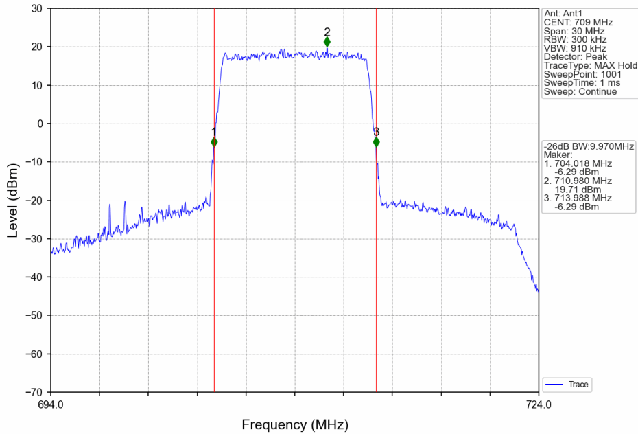
Band17_10MHz_64QAM_LCH_709MHz_RB_50_0_NTNV
