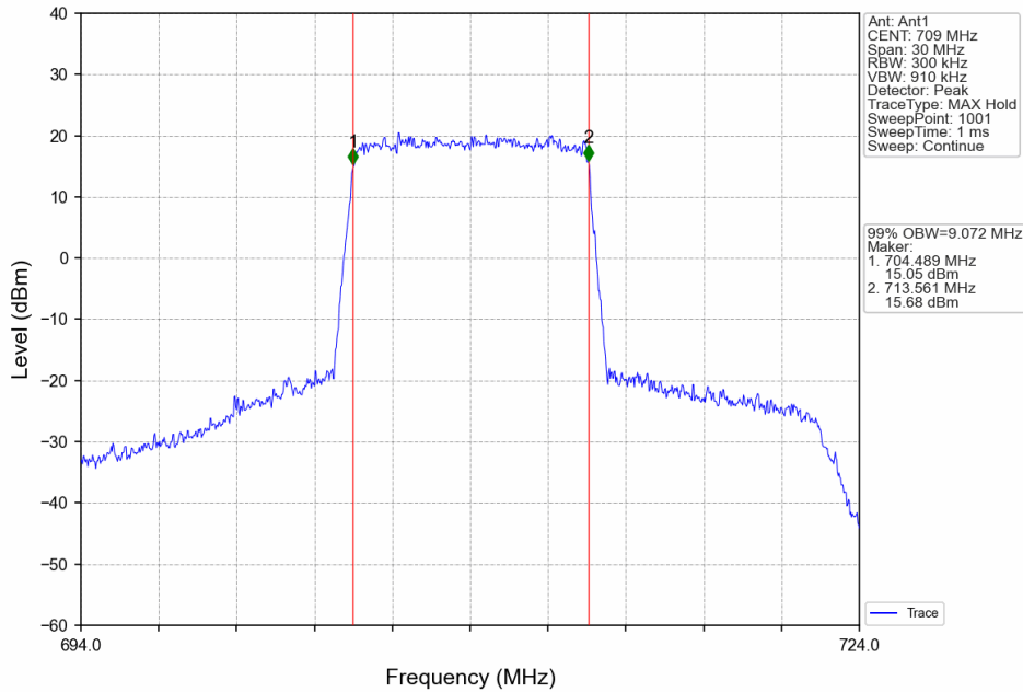
Band17_10MHz_16QAM_LCH_709MHz_RB_50_0_NTNV
