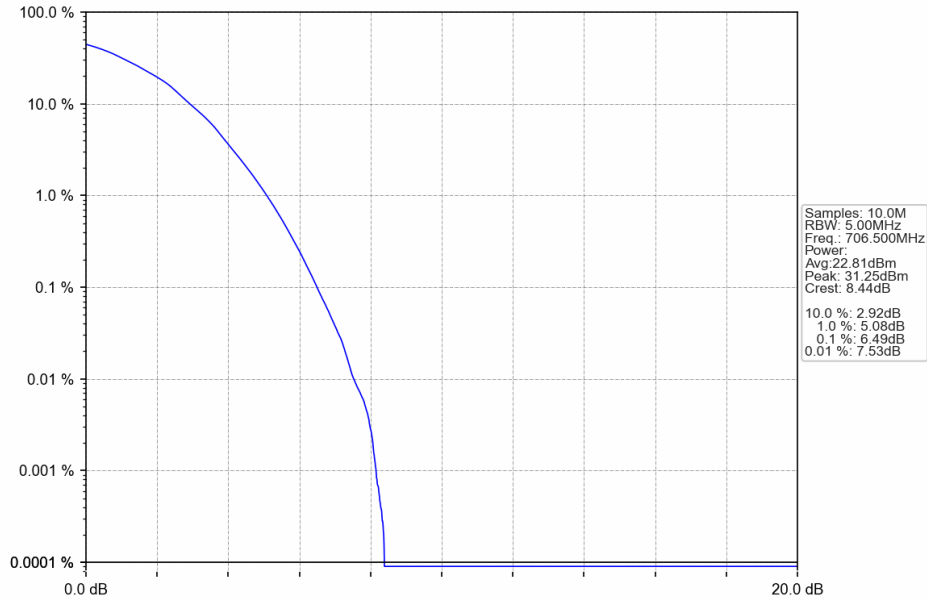
Band17_5MHz_64QAM_LCH_706.5MHz_RB_25_0_NTNV
