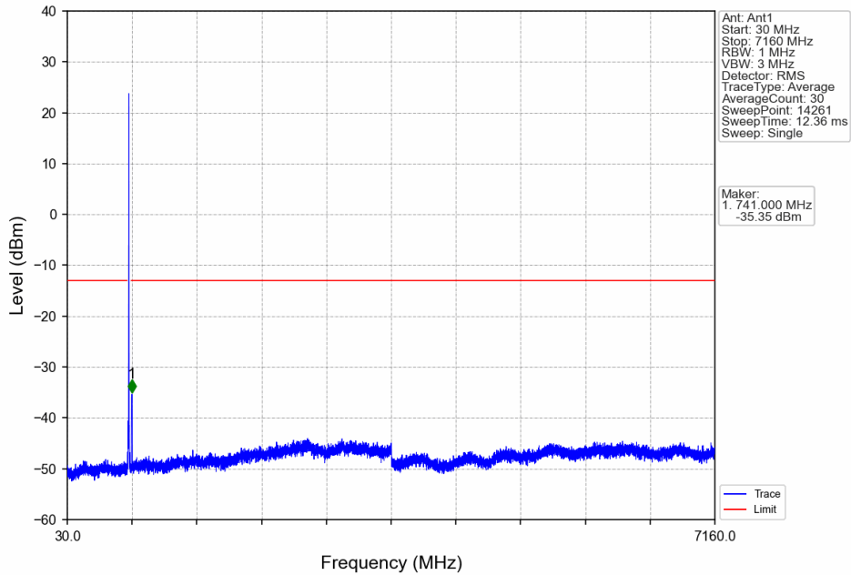
Band17_10MHz_64QAM_MCH_710MHz_RB_1_0_NTNV
