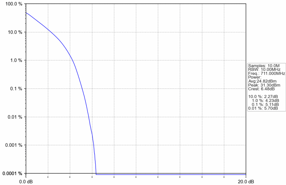
Band17_10MHz_QPSK_HCH_711MHz_RB_50_0_NTNV
