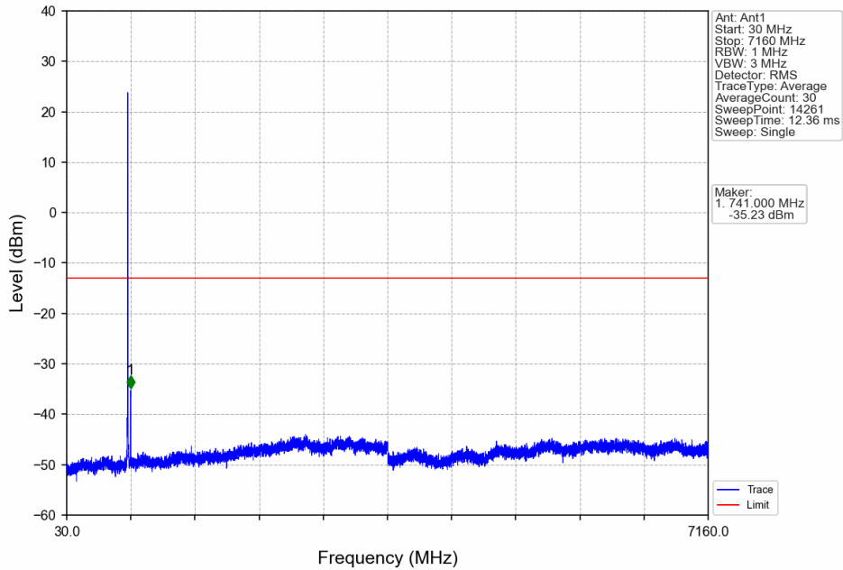
Band17_5MHz_64QAM_MCH_710MHz_RB_1_0_NTNV
