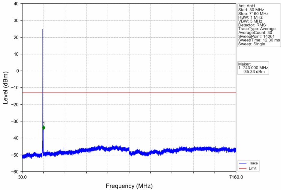
Band17_5MHz_64QAM_HCH_713.5MHz_RB_1_0_NTNV
