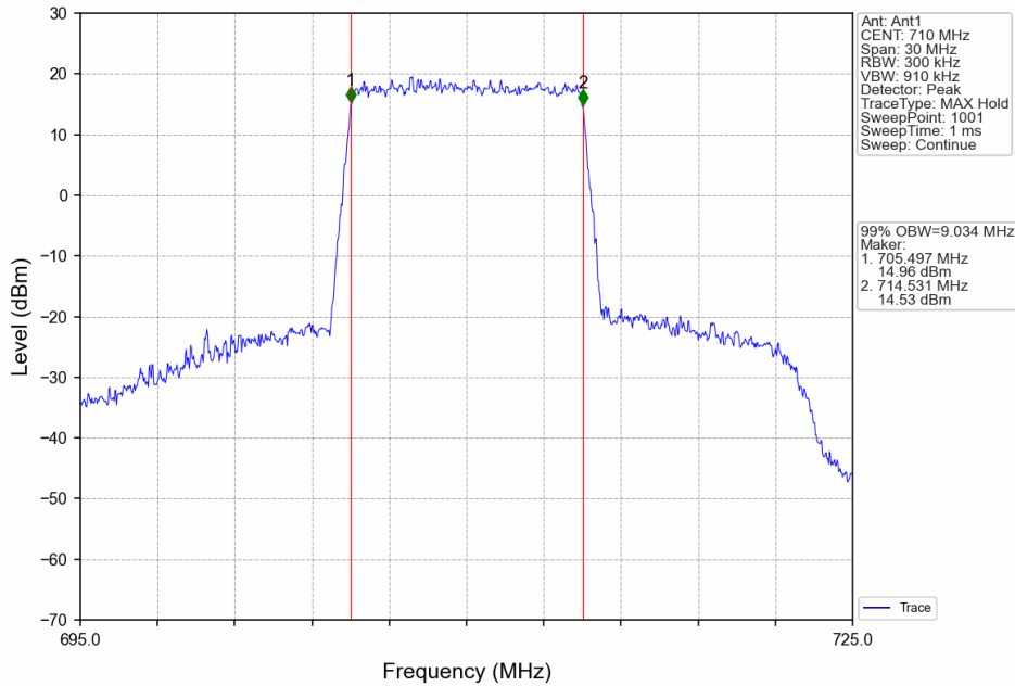
Band17_10MHz_64QAM_MCH_710MHz_RB_50_0_NTNV
