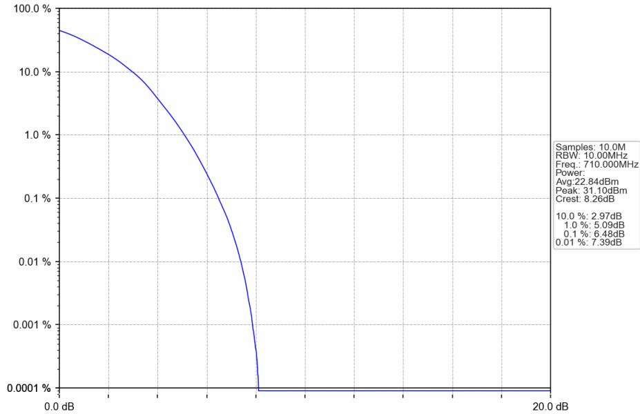
Band17_10MHz_64QAM_MCH_710MHz_RB_50_0_NTNV
