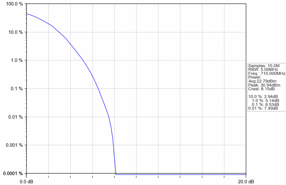
Band17_5MHz_64QAM_MCH_710MHz_RB_25_0_NTNV
