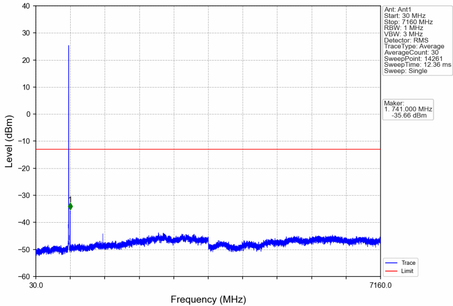
Band17_5MHz_QPSK_MCH_710MHz_RB_1_0_NTNV
