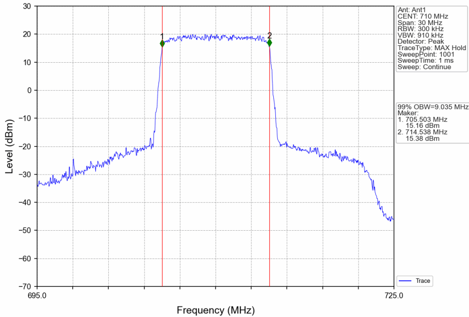
Band17_10MHz_16QAM_MCH_710MHz_RB_50_0_NTNV
