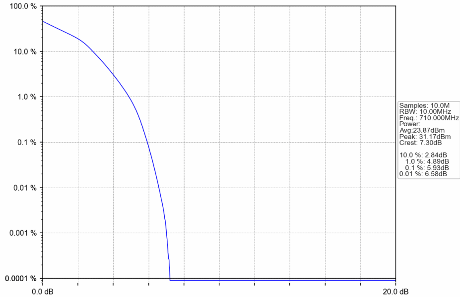
Band17_10MHz_16QAM_MCH_710MHz_RB_50_0_NTNV
