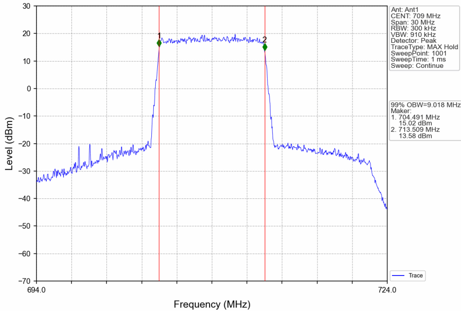
Band17_10MHz_64QAM_LCH_709MHz_RB_50_0_NTNV
