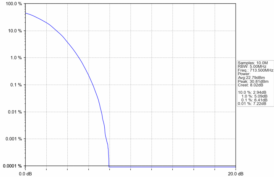
Band17_5MHz_64QAM_HCH_713.5MHz_RB_25_0_NTNV
