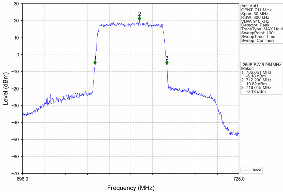
Band17_10MHz_64QAM_HCH_711MHz_RB_50_0_NTNV
