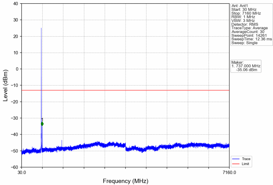
Band17_5MHz_QPSK_LCH_706.5MHz_RB_1_0_NTNV
