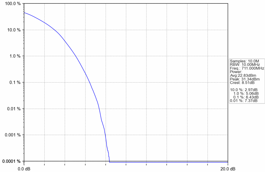
Band17_10MHz_64QAM_HCH_711MHz_RB_50_0_NTNV
