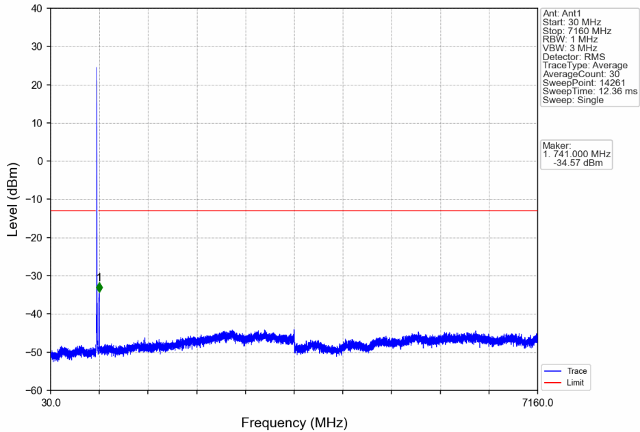
Band17_10MHz_16QAM_LCH_709MHz_RB_1_0_NTNV
