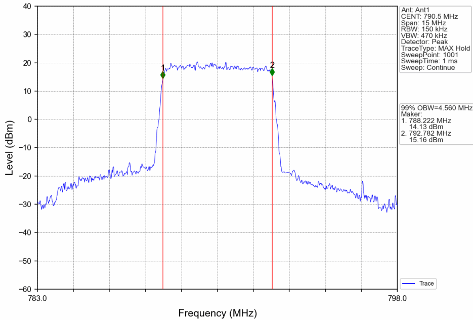
Band14_5MHz_16QAM_LCH_790.5MHz_RB_25_0_NTNV
