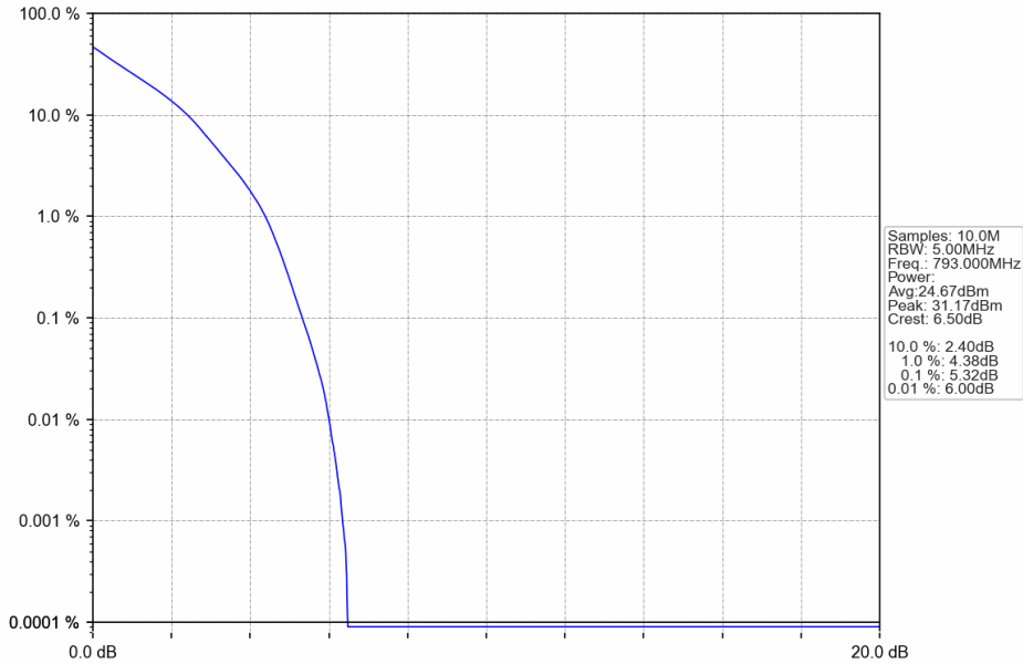
Band14_5MHz_QPSK_MCH_793MHz_RB_25_0_NTNV
