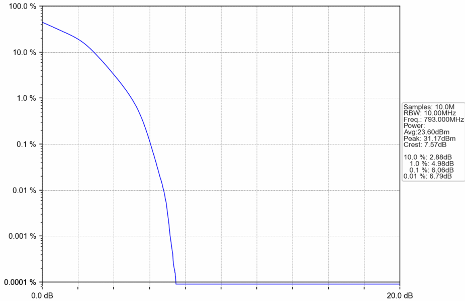
Band14_10MHz_16QAM_MCH_793MHz_RB_50_0_NTNV
