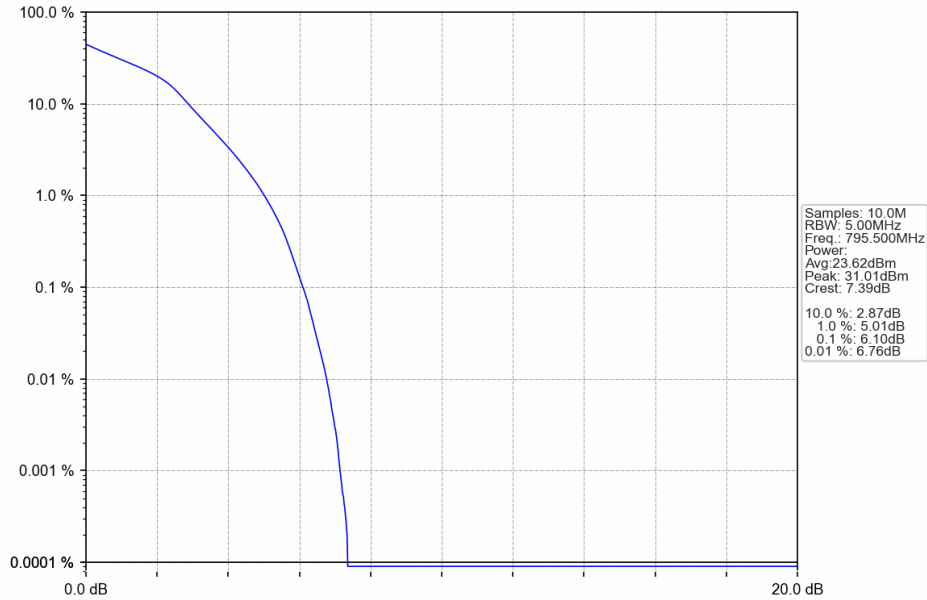
Band14_5MHz_16QAM_HCH_795.5MHz_RB_25_0_NTNV
