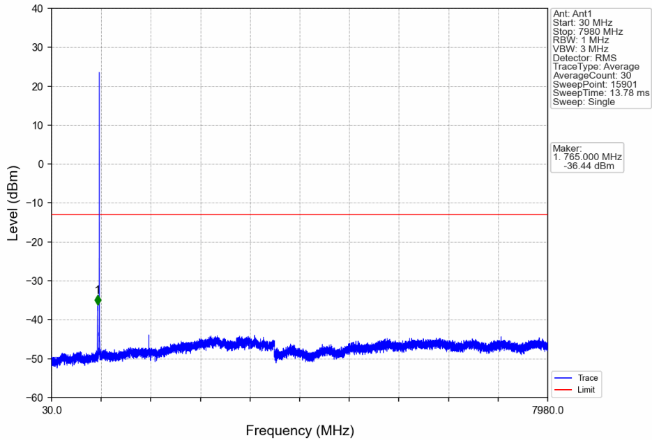
Band14_5MHz_64QAM_HCH_795.5MHz_RB_1_0_NTNV
