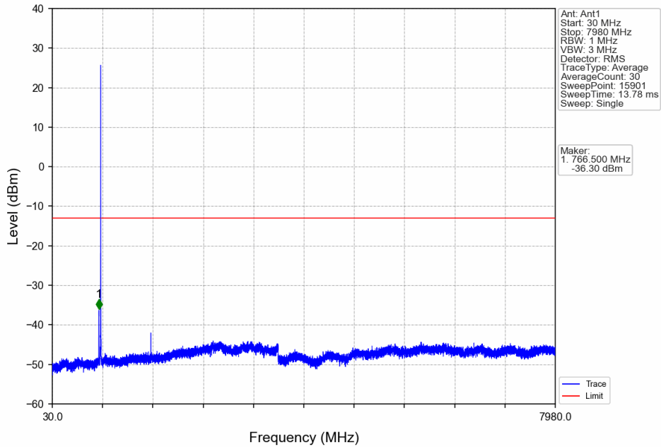
Band14_5MHz_QPSK_HCH_795.5MHz_RB_1_0_NTNV
