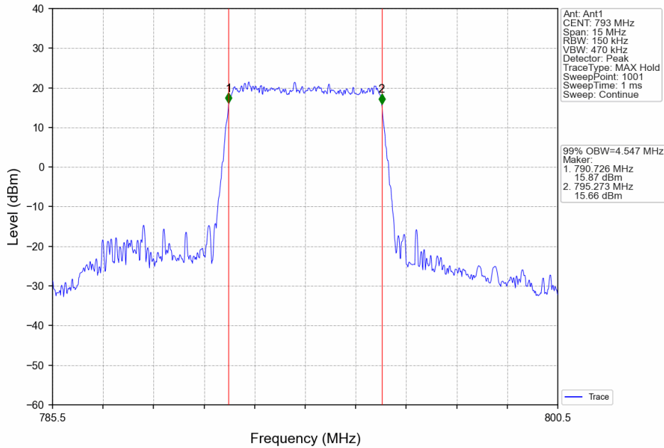
Band14_5MHz_QPSK_MCH_793MHz_RB_25_0_NTNV
