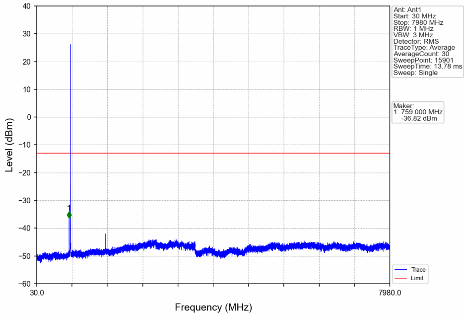
Band14_5MHz_QPSK_LCH_790.5MHz_RB_1_0_NTNV
