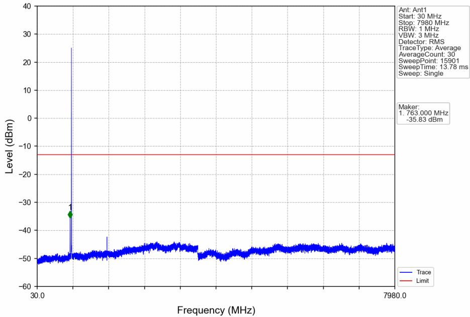
Band14_5MHz_16QAM_MCH_793MHz_RB_1_0_NTNV
