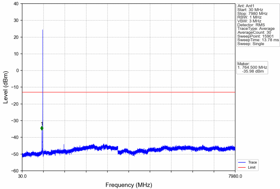
Band14_5MHz_16QAM_HCH_795.5MHz_RB_1_0_NTNV
