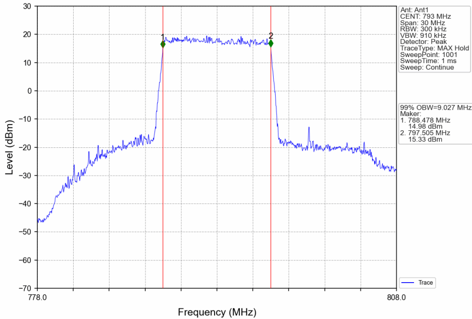
Band14_10MHz_64QAM_MCH_793MHz_RB_50_0_NTNV
