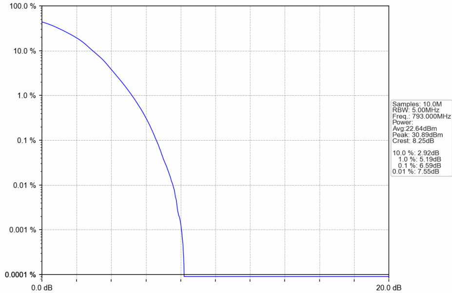
Band14_5MHz_64QAM_MCH_793MHz_RB_25_0_NTNV
