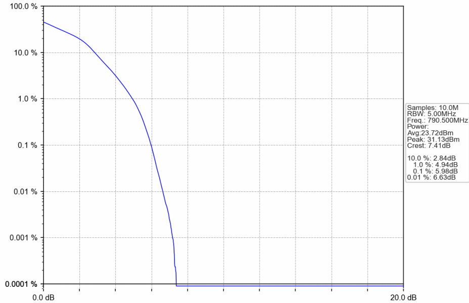
Band14_5MHz_16QAM_LCH_790.5MHz_RB_25_0_NTNV
