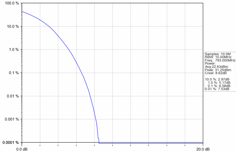
Band14_10MHz_64QAM_MCH_793MHz_RB_50_0_NTNV
