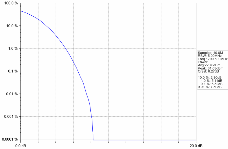
Band14_5MHz_64QAM_LCH_790.5MHz_RB_25_0_NTNV
