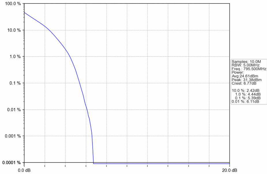
Band14_5MHz_QPSK_HCH_795.5MHz_RB_25_0_NTNV
