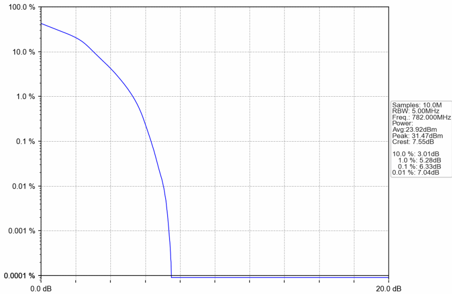
Band13_5MHz_16QAM_MCH_782MHz_RB_25_0_NTNV
