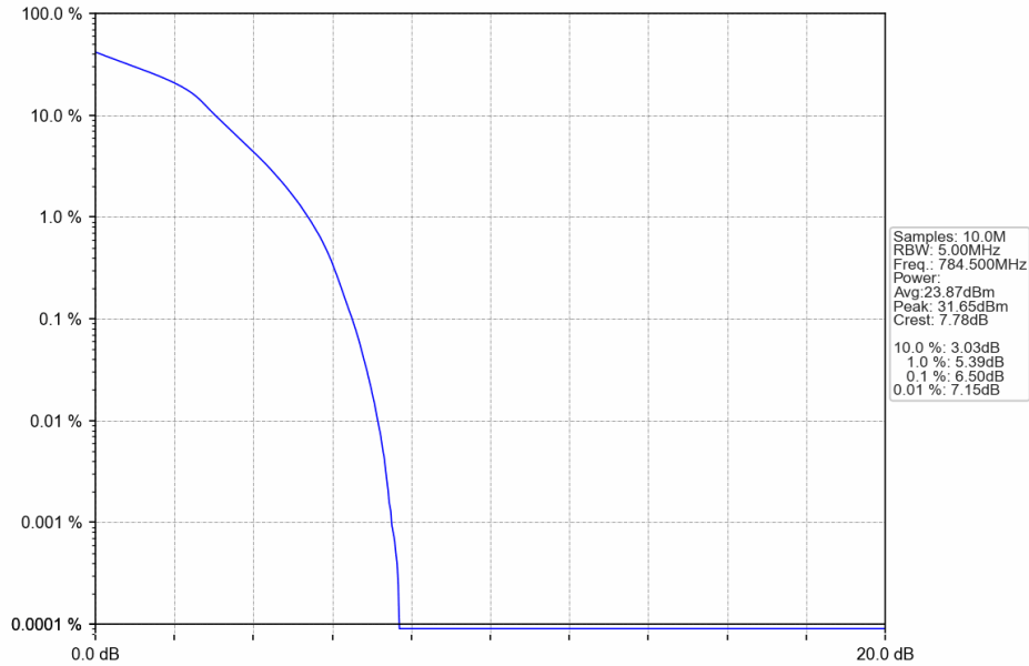
Band13_5MHz_16QAM_HCH_784.5MHz_RB_25_0_NTNV
