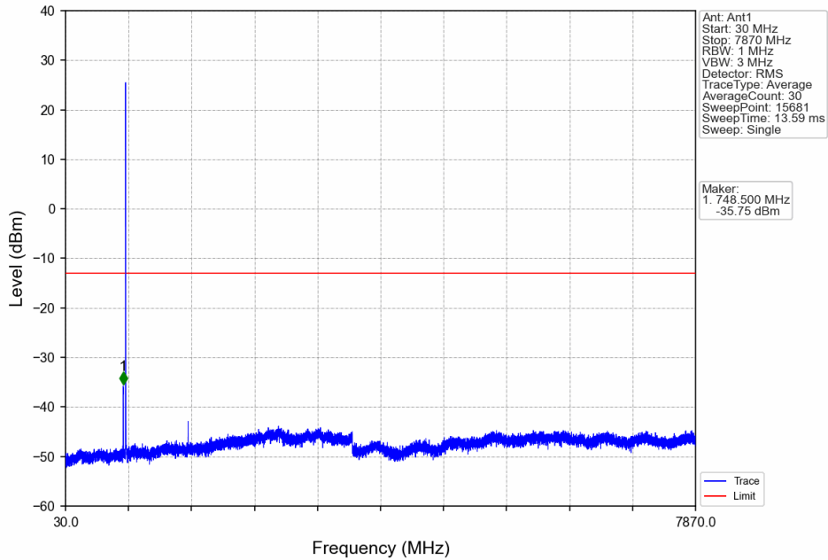
Band13_5MHz_QPSK_LCH_779.5MHz_RB_1_0_NTNV
