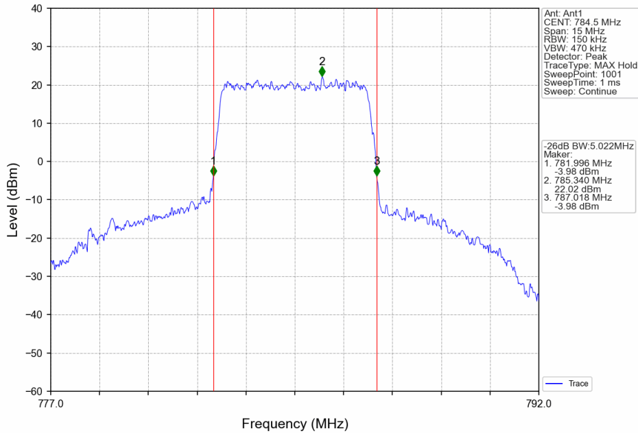
Band13_5MHz_QPSK_HCH_784.5MHz_RB_25_0_NTNV
