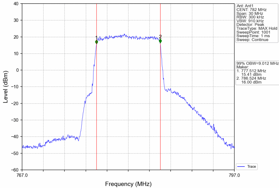
Band13_10MHz_QPSK_MCH_782MHz_RB_50_0_NTNV
