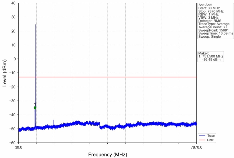
Band13_5MHz_16QAM_MCH_782MHz_RB_1_0_NTNV
