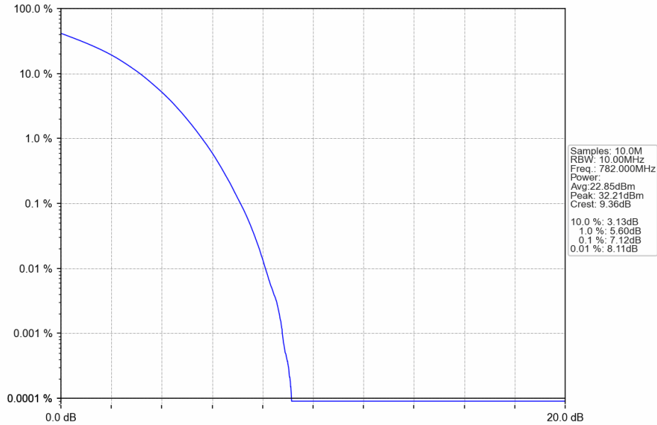
Band13_10MHz_64QAM_MCH_782MHz_RB_50_0_NTNV
