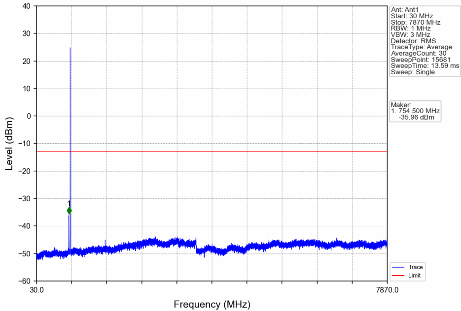
Band13_5MHz_64QAM_HCH_784.5MHz_RB_1_0_NTNV
