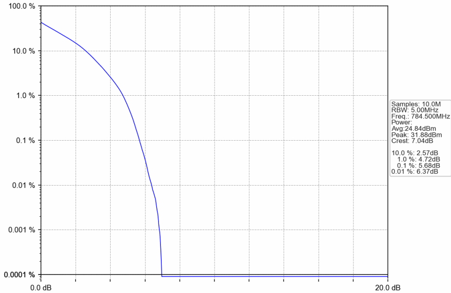
Band13_5MHz_QPSK_HCH_784.5MHz_RB_25_0_NTNV
