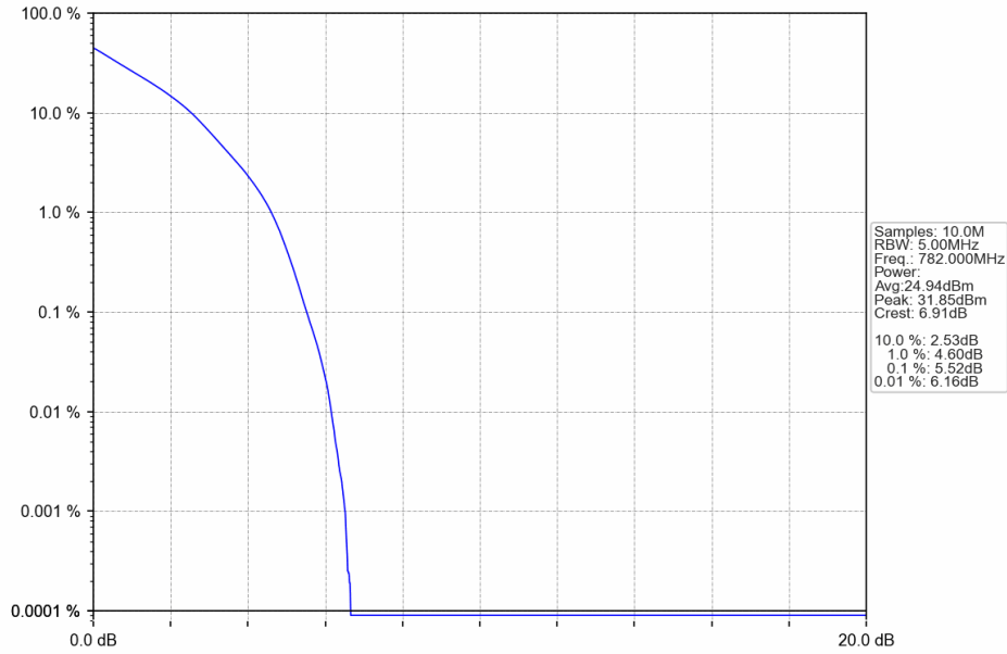
Band13_5MHz_QPSK_MCH_782MHz_RB_25_0_NTNV
