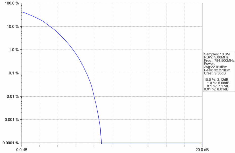
Band13_5MHz_64QAM_HCH_784.5MHz_RB_25_0_NTNV
