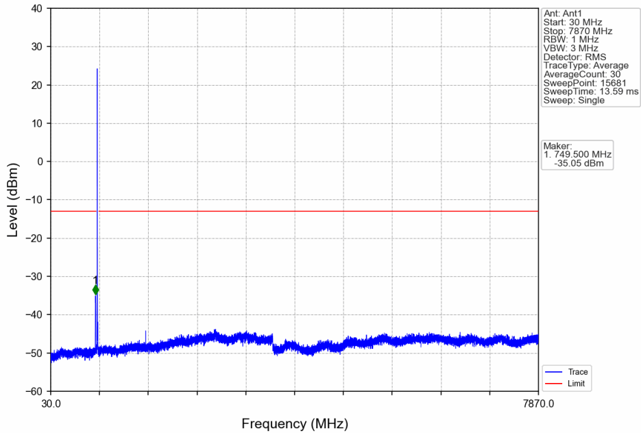
Band13_10MHz_16QAM_MCH_782MHz_RB_1_0_NTNV
