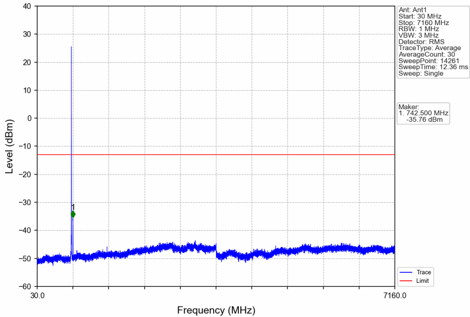
Band12_5MHz_16QAM_HCH_713.5MHz_RB_1_0_NTNV
