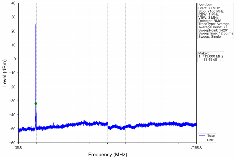
Band12_1.4MHz_16QAM_HCH_715.3MHz_RB_1_0_NTNV
