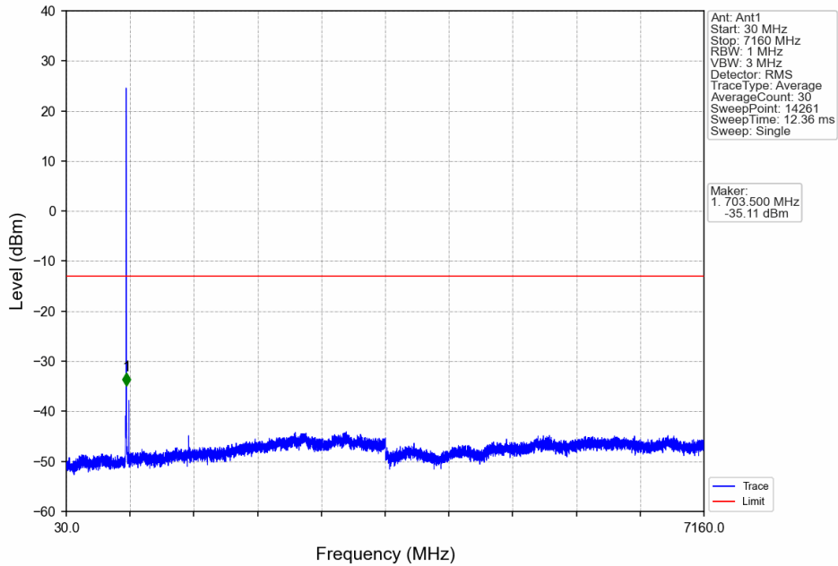
Band12_1.4MHz_64QAM_LCH_699.7MHz_RB_1_0_NTNV
