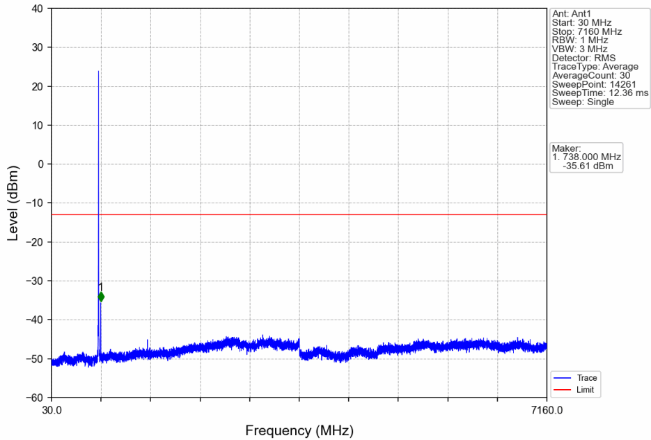
Band12_5MHz_64QAM_MCH_707.5MHz_RB_1_0_NTNV
