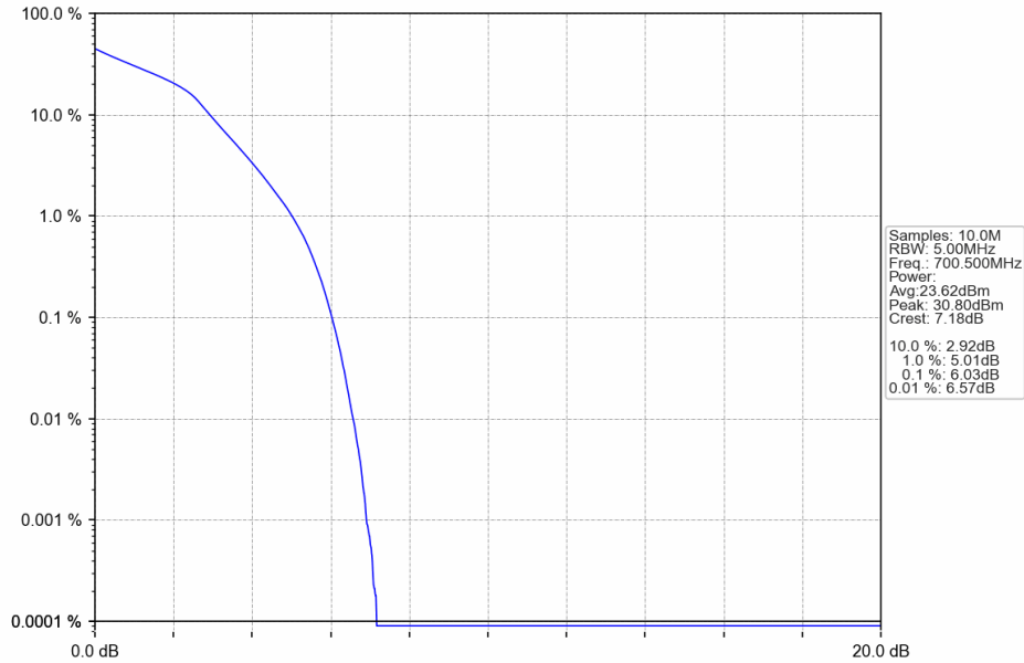
Band12_3MHz_16QAM_LCH_700.5MHz_RB_15_0_NTNV
