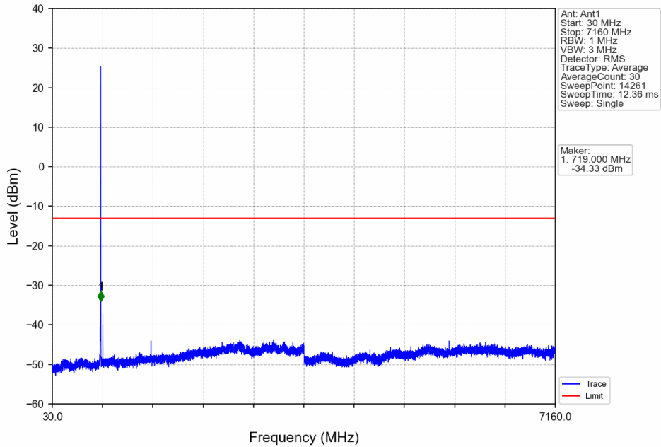
Band12_1.4MHz_QPSK_HCH_715.3MHz_RB_1_0_NTNV
