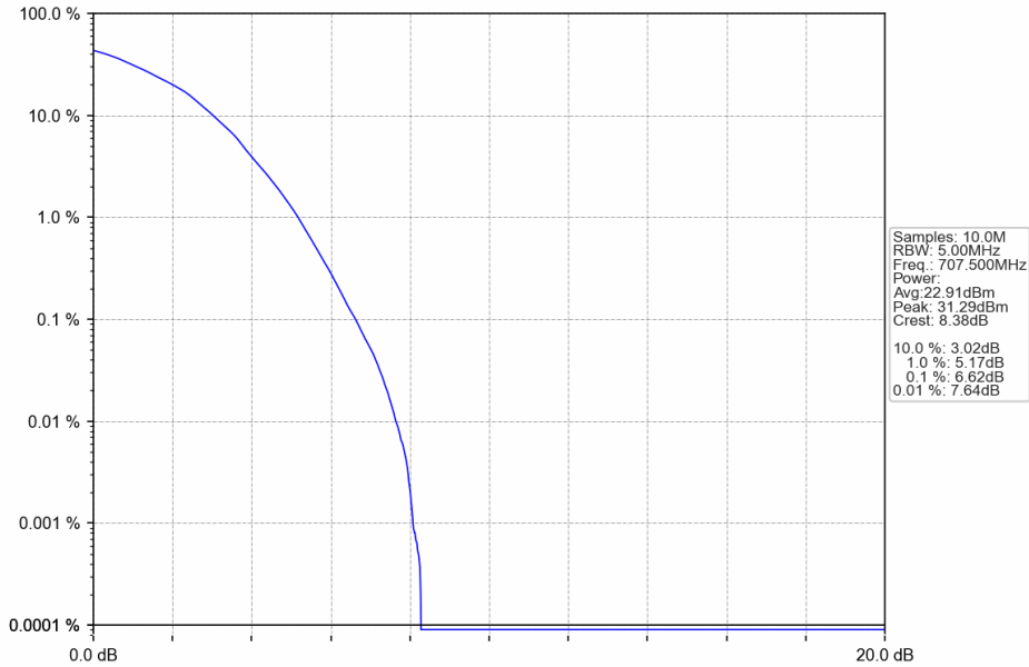
Band12_3MHz_64QAM_MCH_707.5MHz_RB_15_0_NTNV
