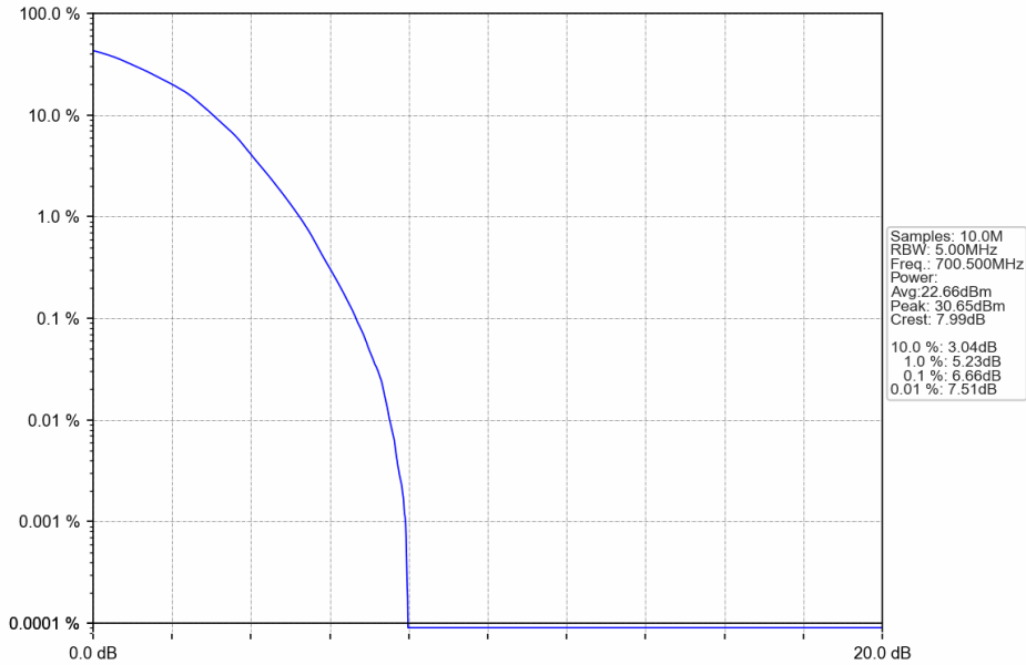
Band12_3MHz_64QAM_LCH_700.5MHz_RB_15_0_NTNV
