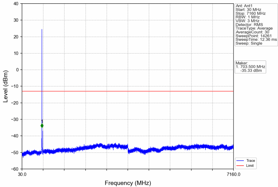
Band12_1.4MHz_16QAM_LCH_699.7MHz_RB_1_0_NTNV
