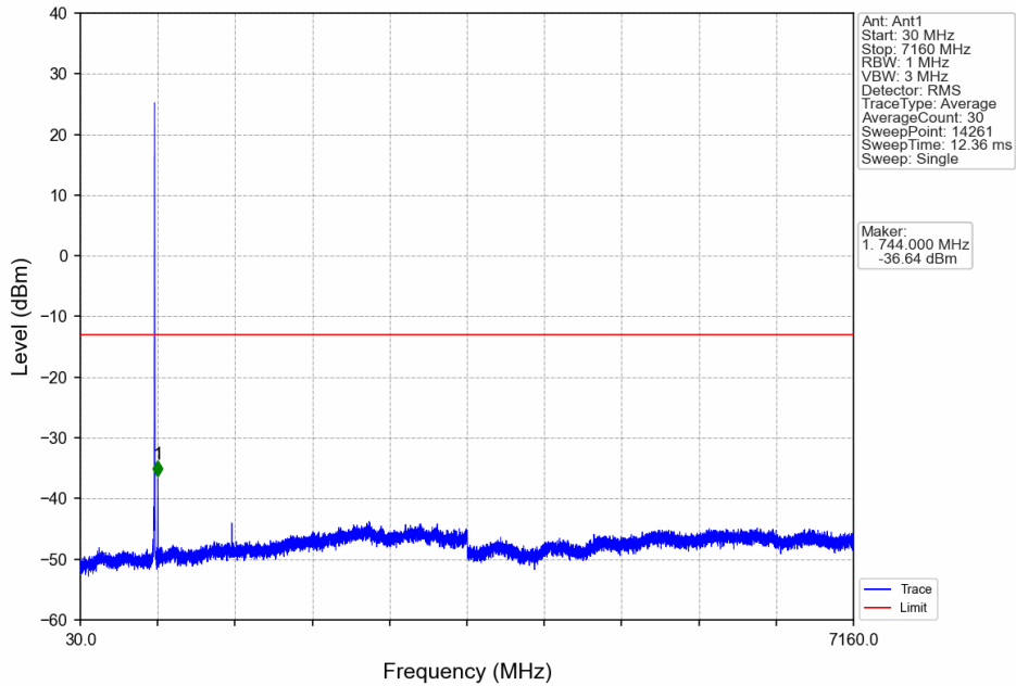
Band12_3MHz_16QAM_HCH_714.5MHz_RB_1_0_NTNV
