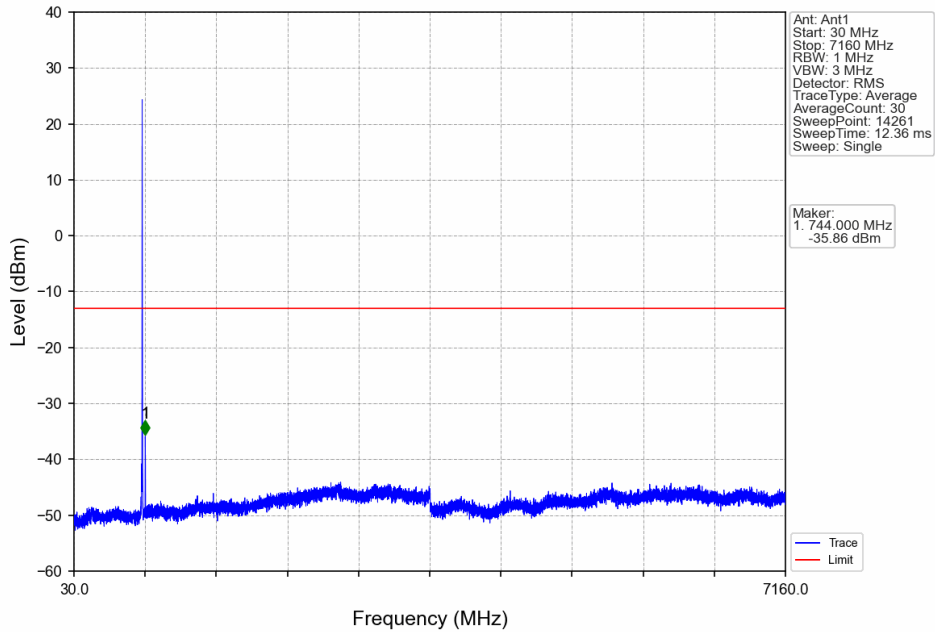
Band12_3MHz_64QAM_HCH_714.5MHz_RB_1_0_NTNV
