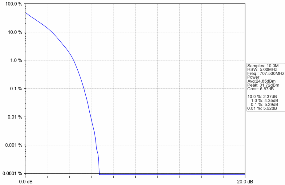
Band12_5MHz_QPSK_MCH_707.5MHz_RB_25_0_NTNV
