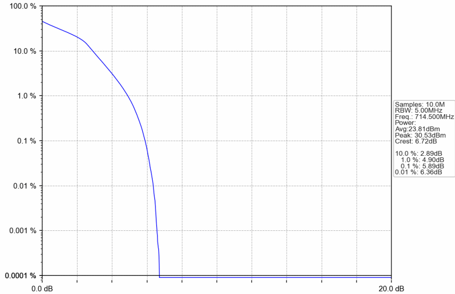
Band12_3MHz_16QAM_HCH_714.5MHz_RB_15_0_NTNV
