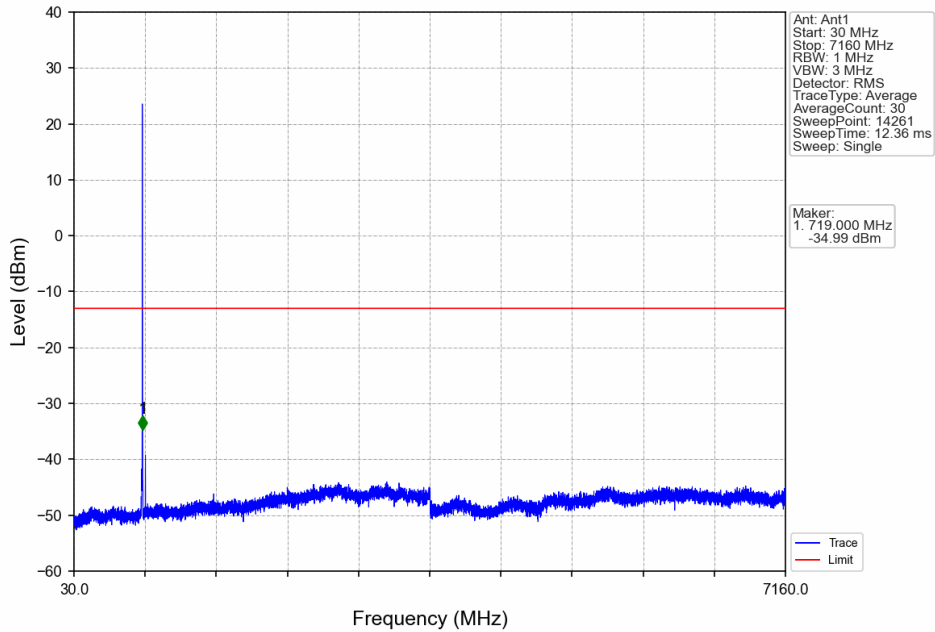
Band12_1.4MHz_64QAM_HCH_715.3MHz_RB_1_0_NTNV
