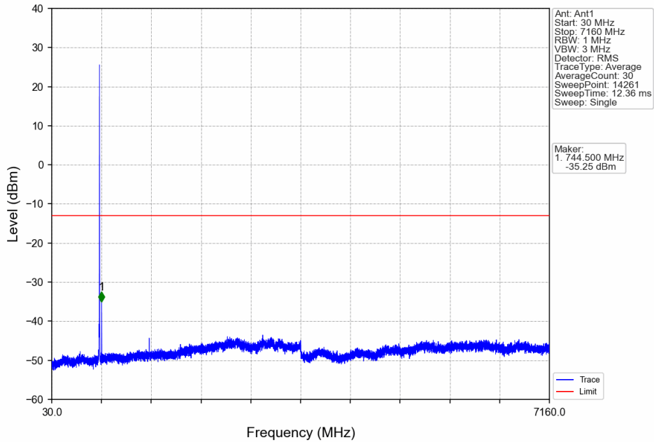
Band12_3MHz_QPSK_HCH_714.5MHz_RB_1_0_NTNV
