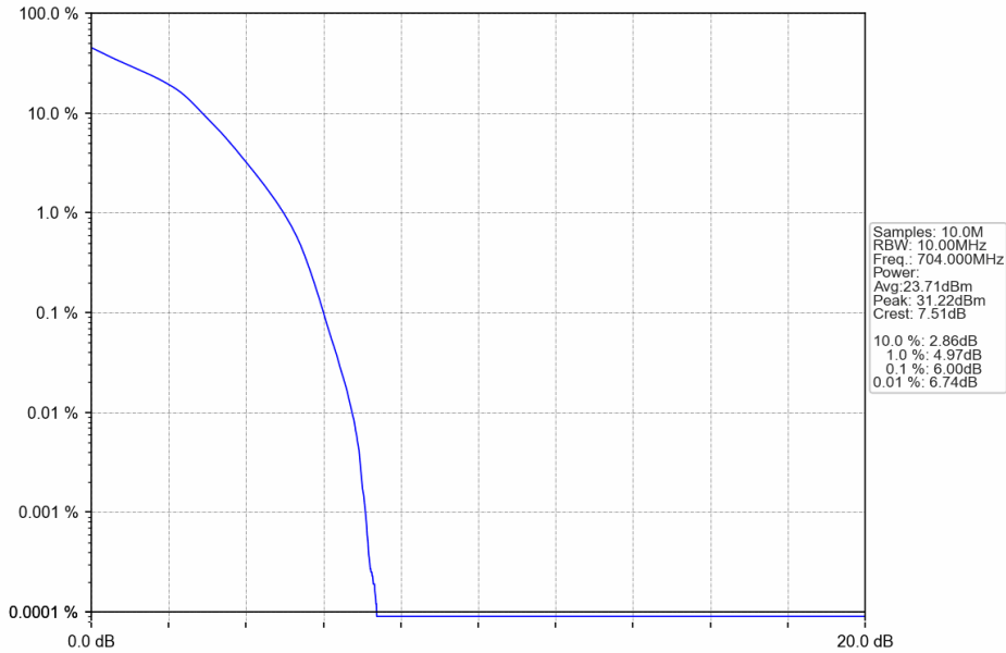
Band12_10MHz_16QAM_LCH_704MHz_RB_50_0_NTNV
