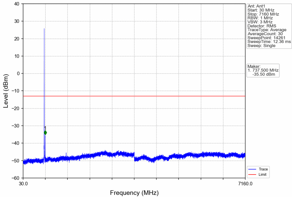
Band12_5MHz_16QAM_MCH_707.5MHz_RB_1_0_NTNV
