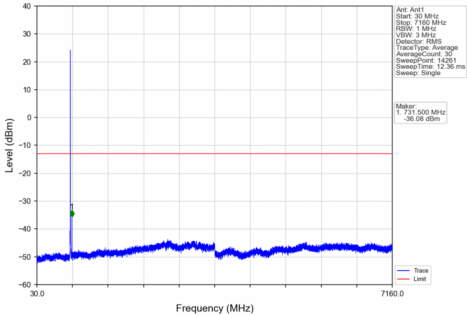
Band12_3MHz_16QAM_LCH_700.5MHz_RB_1_0_NTNV
