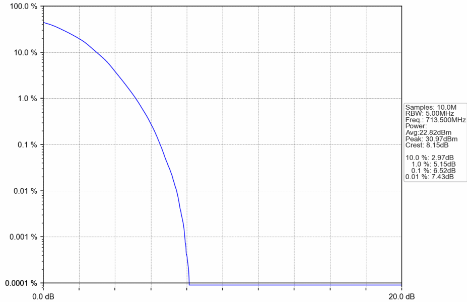
Band12_5MHz_64QAM_HCH_713.5MHz_RB_25_0_NTNV
