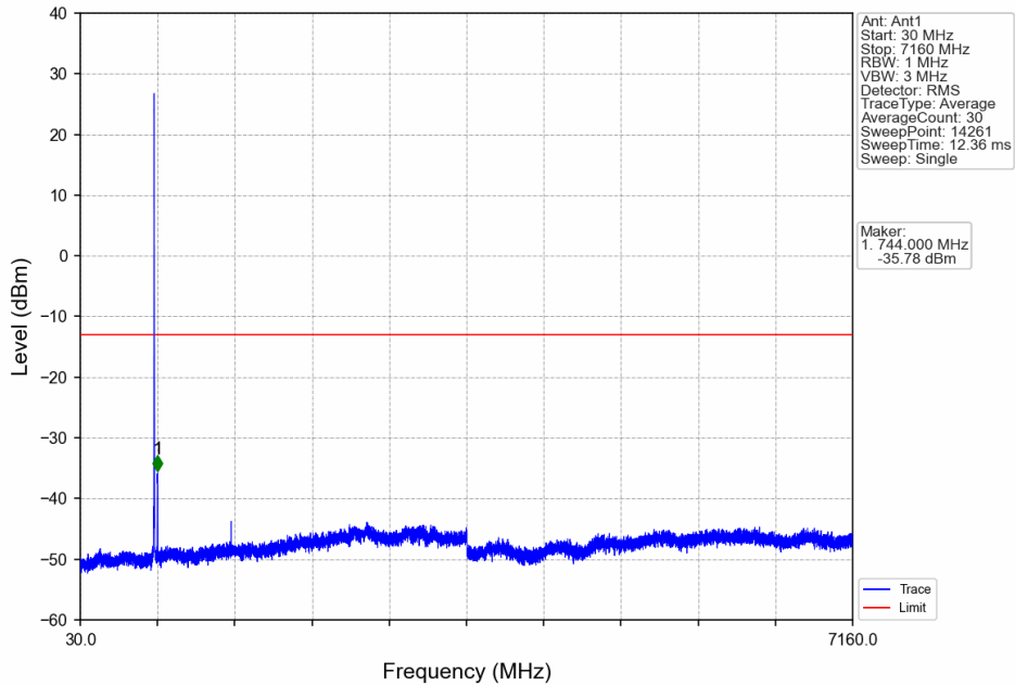
Band12_5MHz_QPSK_HCH_713.5MHz_RB_1_0_NTNV
