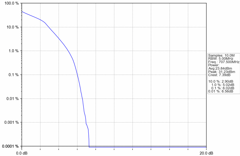
Band12_3MHz_16QAM_MCH_707.5MHz_RB_15_0_NTNV
