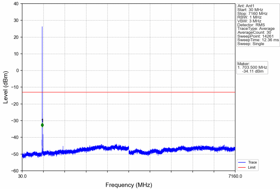
Band12_1.4MHz_QPSK_LCH_699.7MHz_RB_1_0_NTNV
