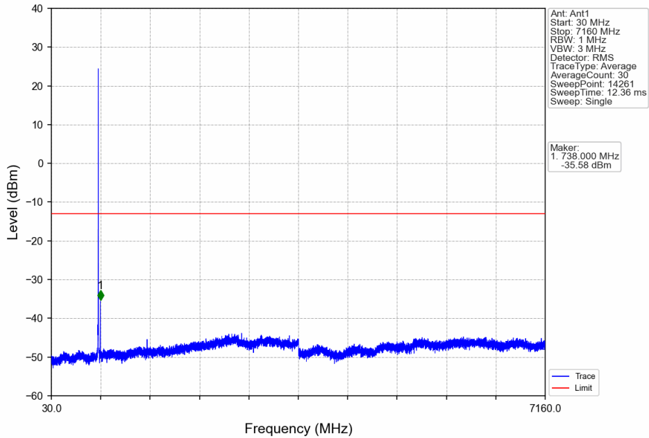
Band12_3MHz_16QAM_MCH_707.5MHz_RB_1_0_NTNV
