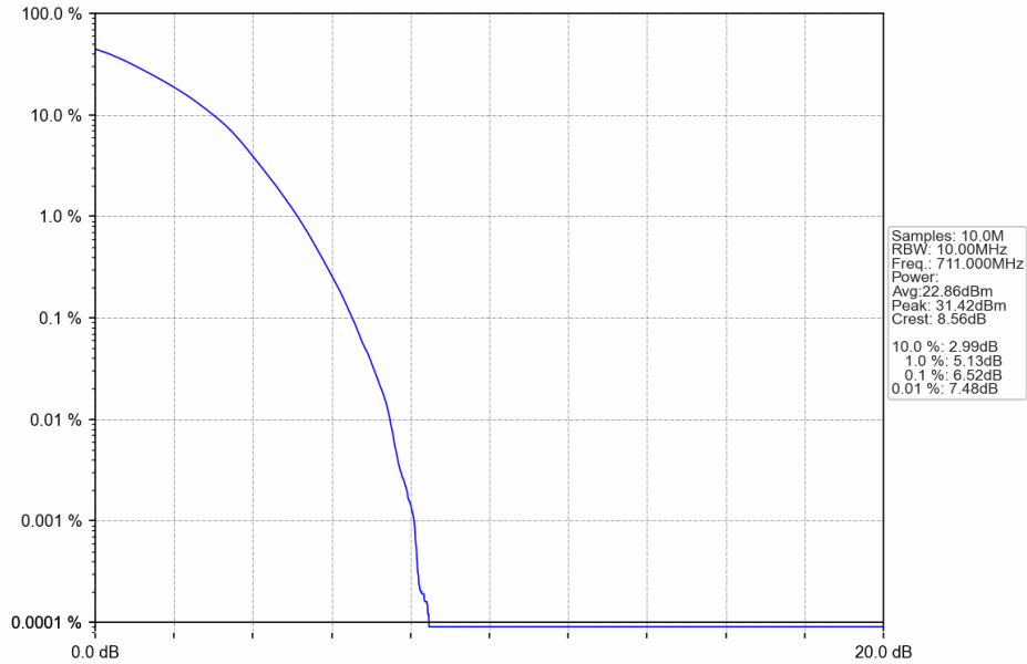
Band12_10MHz_64QAM_HCH_711MHz_RB_50_0_NTNV
