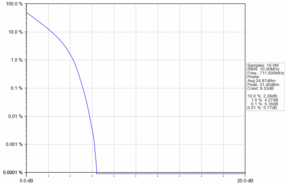
Band12_10MHz_QPSK_HCH_711MHz_RB_50_0_NTNV
