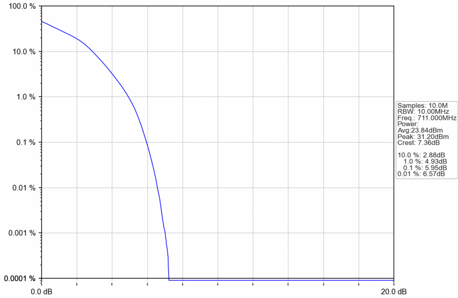
Band12_10MHz_16QAM_HCH_711MHz_RB_50_0_NTNV
