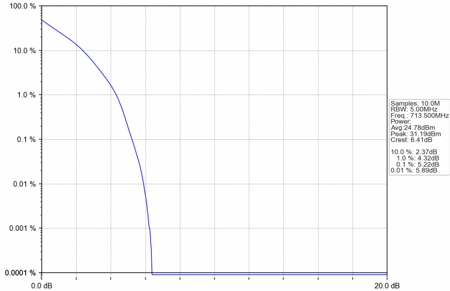
Band12_5MHz_QPSK_HCH_713.5MHz_RB_25_0_NTNV
