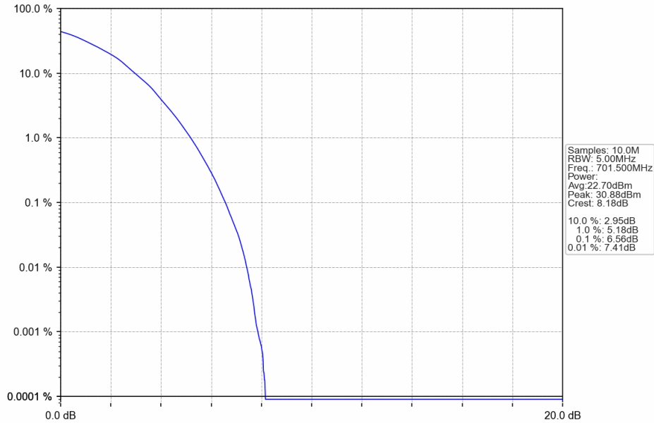
Band12_5MHz_64QAM_LCH_701.5MHz_RB_25_0_NTNV
