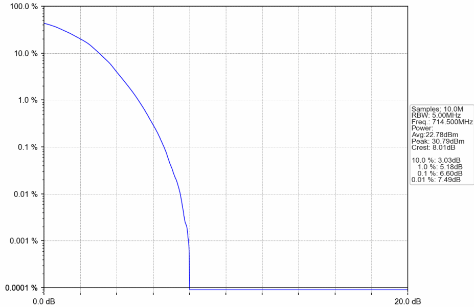
Band12_3MHz_64QAM_HCH_714.5MHz_RB_15_0_NTNV
