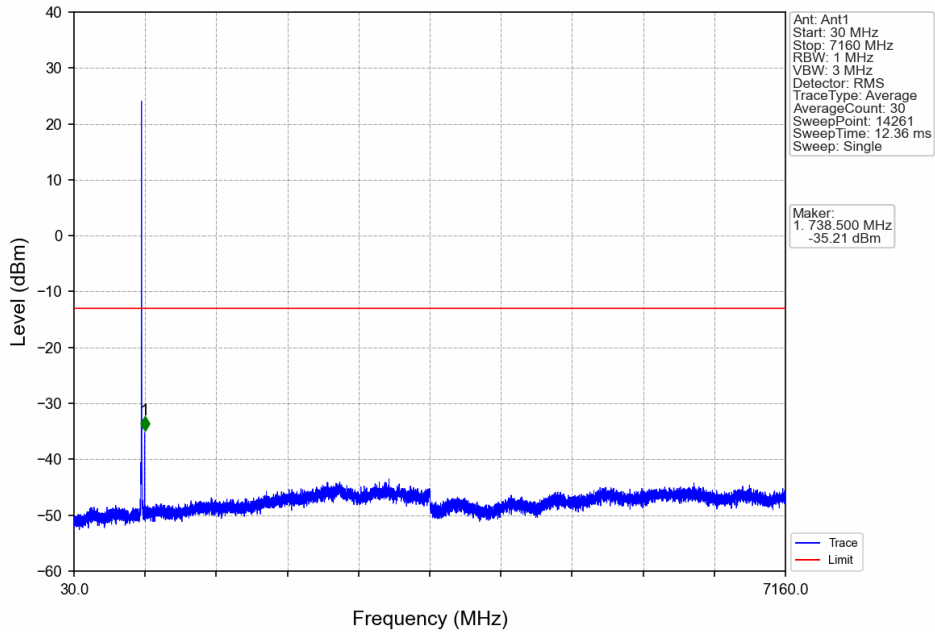
Band12_3MHz_64QAM_MCH_707.5MHz_RB_1_0_NTNV
