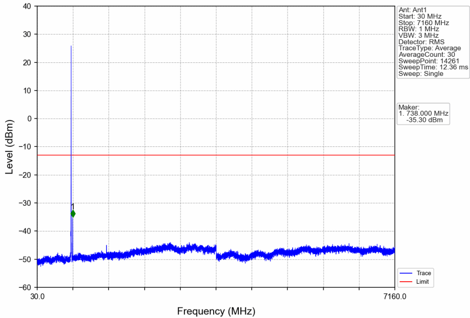
Band12_5MHz_QPSK_MCH_707.5MHz_RB_1_0_NTNV
