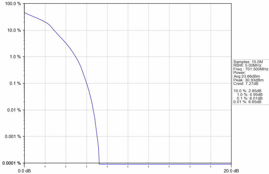
Band12_5MHz_16QAM_LCH_701.5MHz_RB_25_0_NTNV
