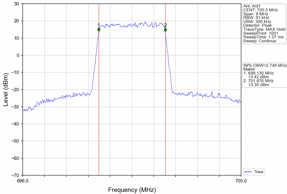
Band12_3MHz_64QAM_LCH_700.5MHz_RB_15_0_NTNV
