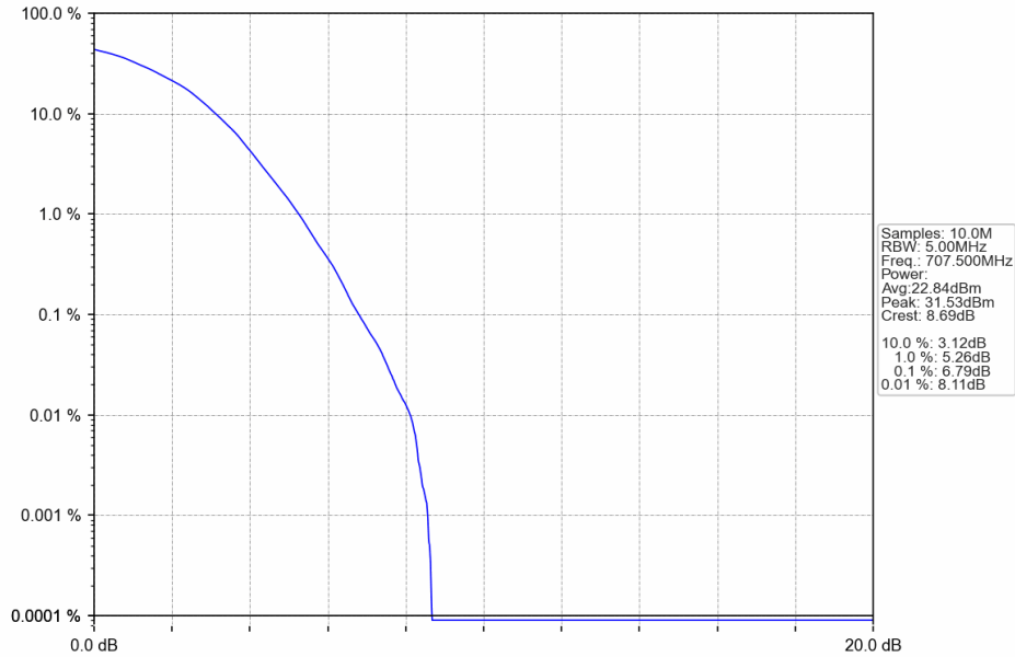
Band12_1.4MHz_64QAM_MCH_707.5MHz_RB_6_0_NTNV
