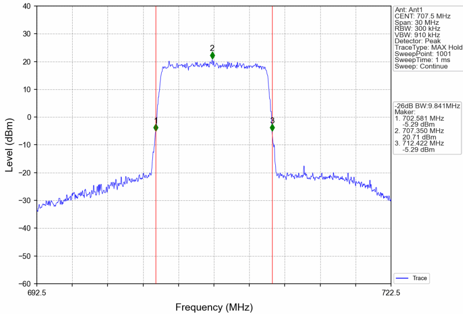
Band12_10MHz_16QAM_MCH_707.5MHz_RB_50_0_NTNV
