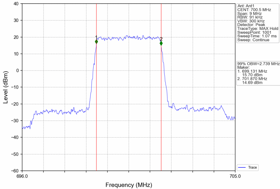
Band12_3MHz_QPSK_LCH_700.5MHz_RB_15_0_NTNV
