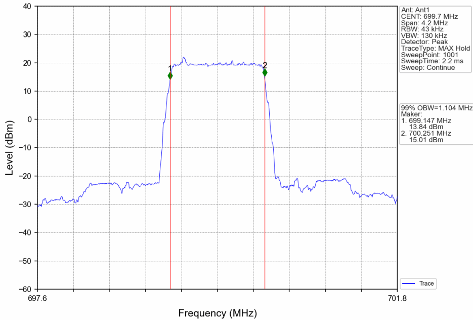
Band12_1.4MHz_16QAM_LCH_699.7MHz_RB_6_0_NTNV
