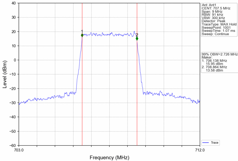
Band12_3MHz_64QAM_MCH_707.5MHz_RB_15_0_NTNV
