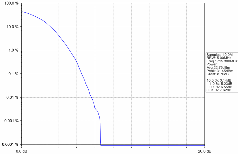
Band12_1.4MHz_64QAM_HCH_715.3MHz_RB_6_0_NTNV
