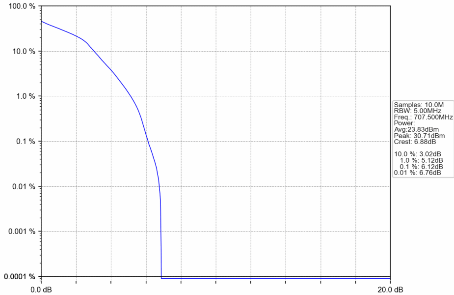
Band12_1.4MHz_16QAM_MCH_707.5MHz_RB_6_0_NTNV
