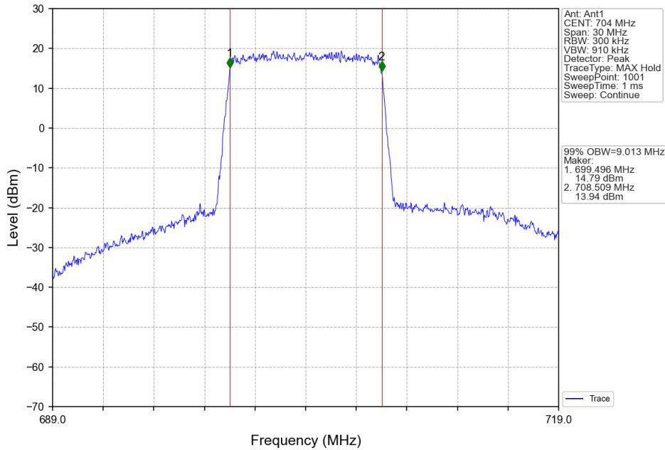
Band12_10MHz_64QAM_LCH_704MHz_RB_50_0_NTNV
