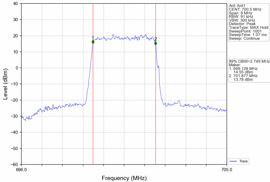
Band12_3MHz_16QAM_LCH_700.5MHz_RB_15_0_NTNV
