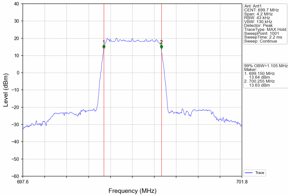
Band12_1.4MHz_64QAM_LCH_699.7MHz_RB_6_0_NTNV
