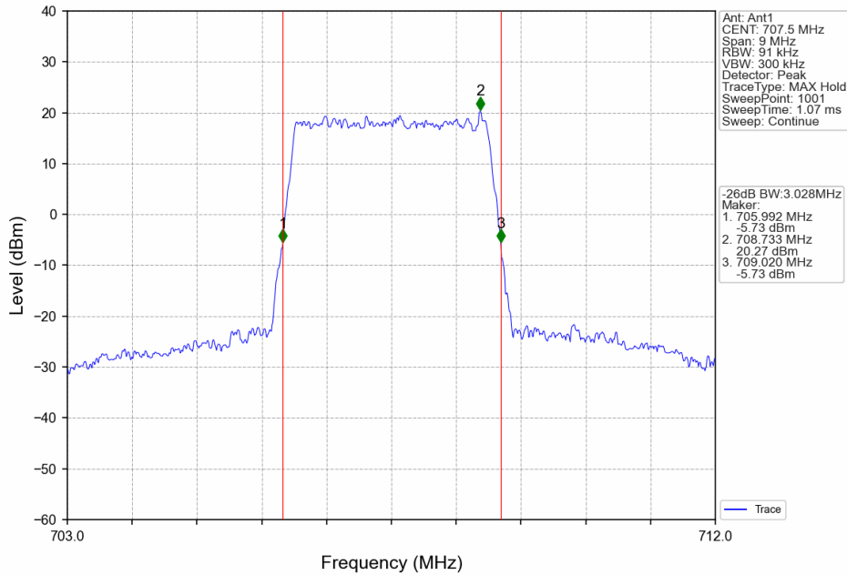
Band12_3MHz_64QAM_MCH_707.5MHz_RB_15_0_NTNV
