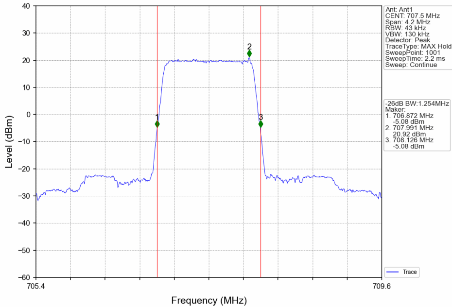
Band12_1.4MHz_16QAM_MCH_707.5MHz_RB_6_0_NTNV
