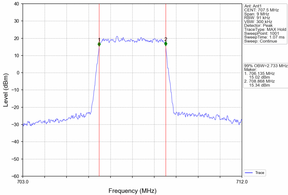
Band12_3MHz_16QAM_MCH_707.5MHz_RB_15_0_NTNV
