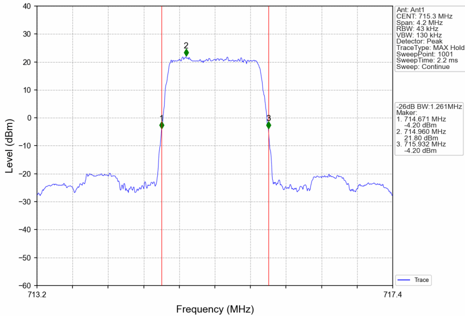
Band12_1.4MHz_QPSK_HCH_715.3MHz_RB_6_0_NTNV
