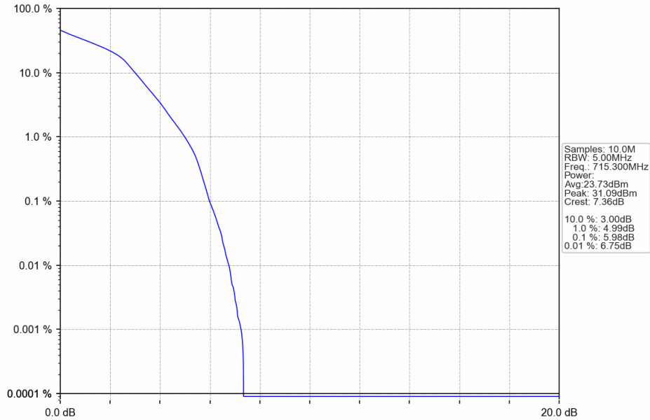
Band12_1.4MHz_16QAM_HCH_715.3MHz_RB_6_0_NTNV
