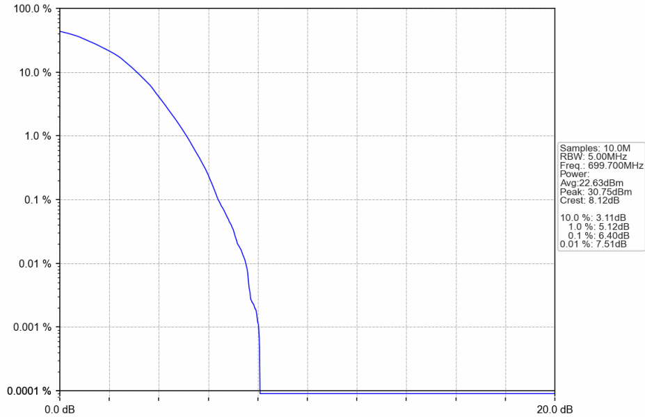
Band12_1.4MHz_64QAM_LCH_699.7MHz_RB_6_0_NTNV
