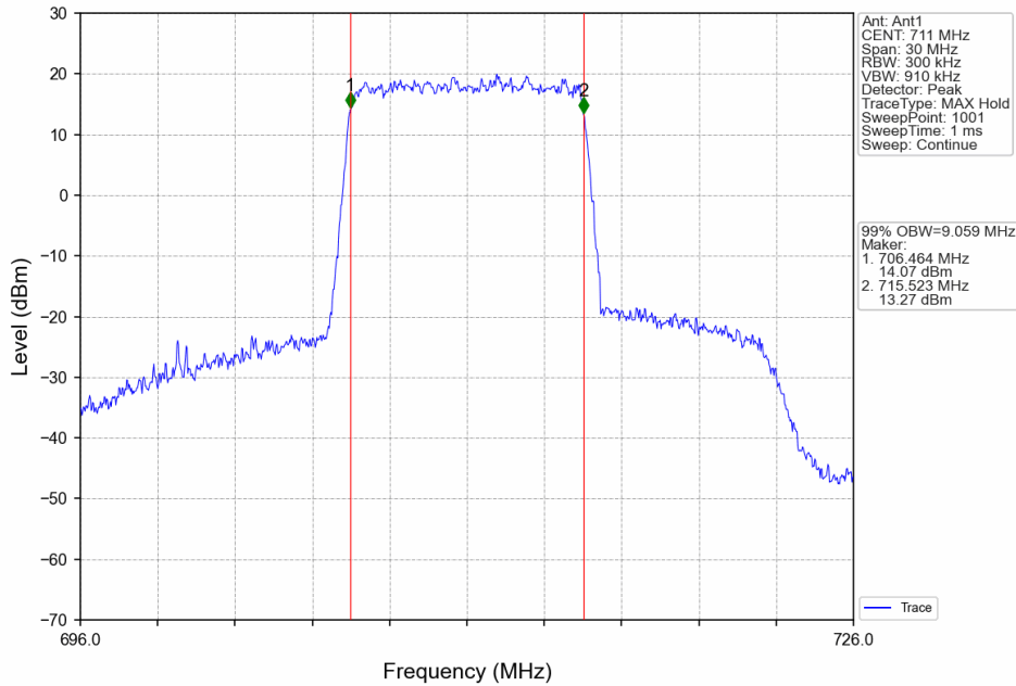
Band12_10MHz_64QAM_HCH_711MHz_RB_50_0_NTNV
