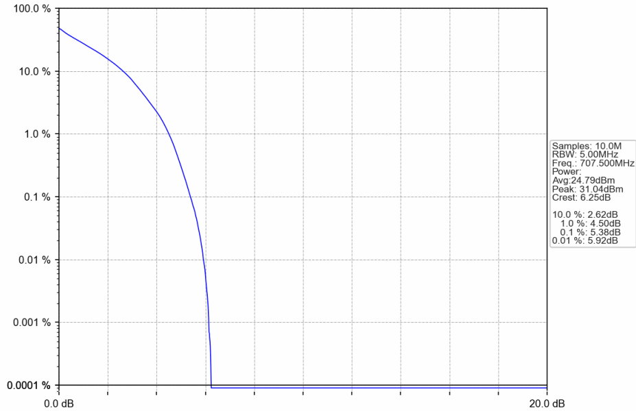
Band12_1.4MHz_QPSK_MCH_707.5MHz_RB_6_0_NTNV
