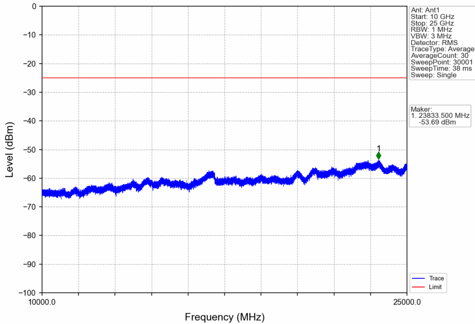
Band7_15MHz_QPSK_MCH_2535MHz_RB_1_0_NTNV
