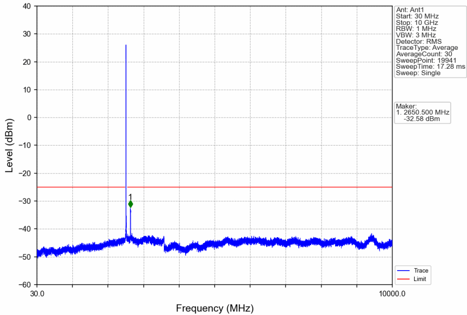
Band7_15MHz_QPSK_MCH_2535MHz_RB_1_0_NTNV
