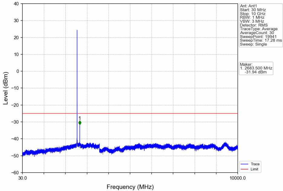
Band7_10MHz_64QAM_HCH_2565MHz_RB_1_0_NTNV
