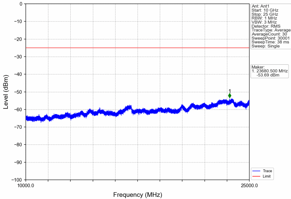
Band7_10MHz_64QAM_MCH_2535MHz_RB_1_0_NTNV
