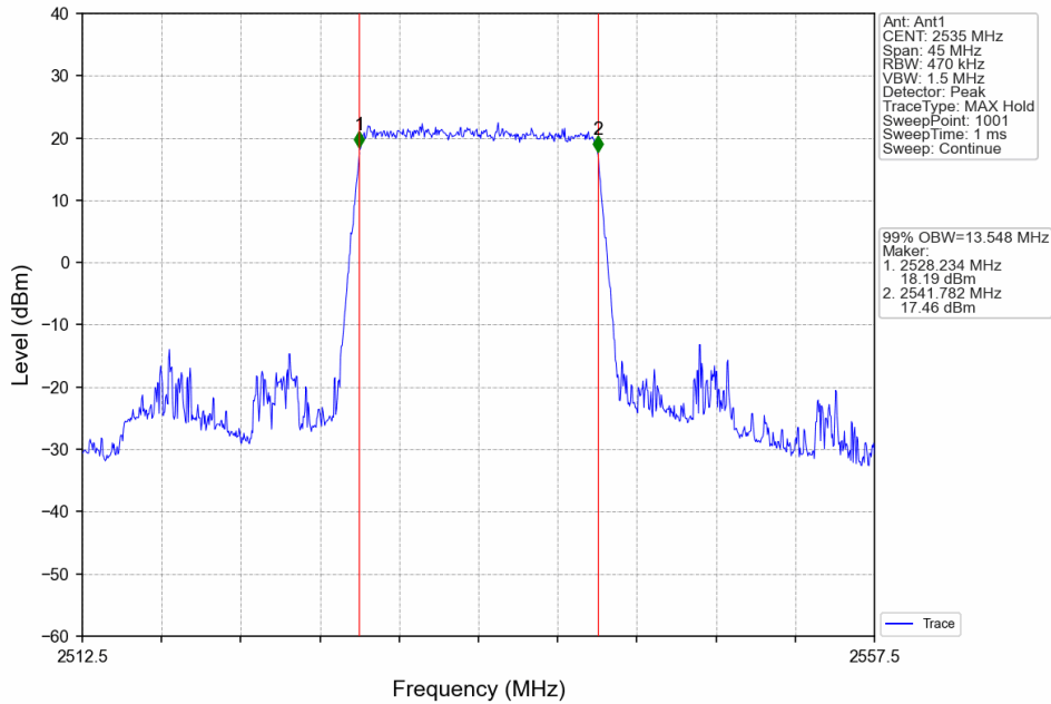
Band7_15MHz_QPSK_MCH_2535MHz_RB_75_0_NTNV
