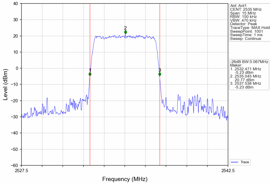
Band7_5MHz_16QAM_MCH_2535MHz_RB_25_0_NTNV
