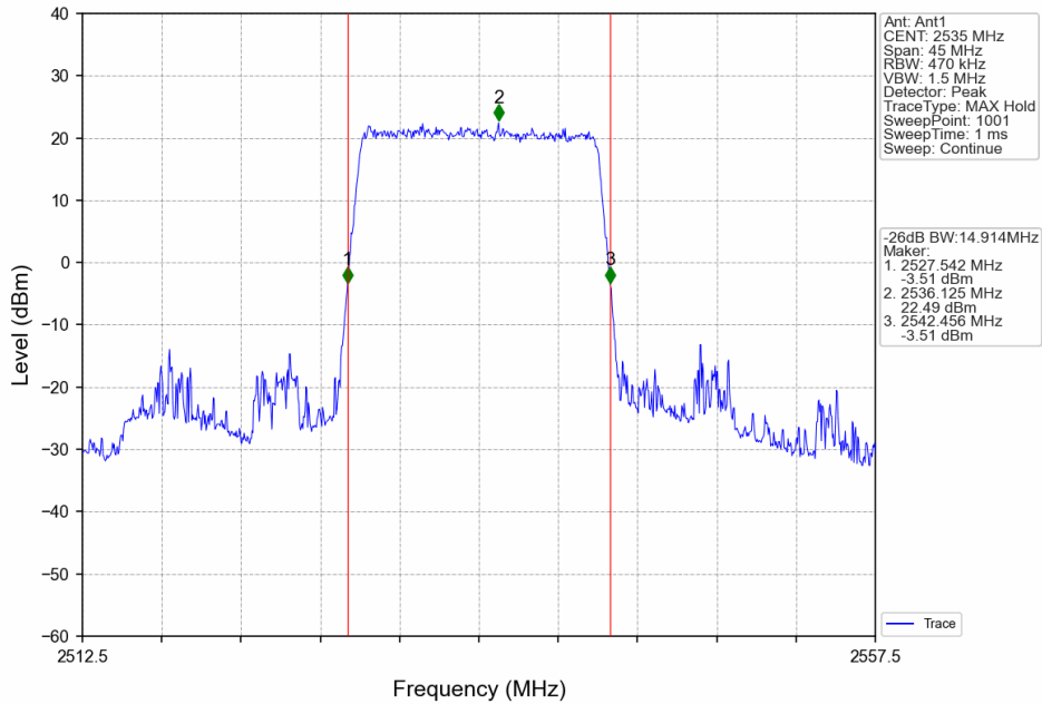
Band7_15MHz_QPSK_MCH_2535MHz_RB_75_0_NTNV
