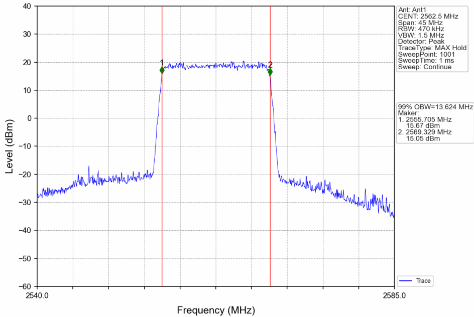
Band7_15MHz_64QAM_HCH_2562.5MHz_RB_75_0_NTNV
