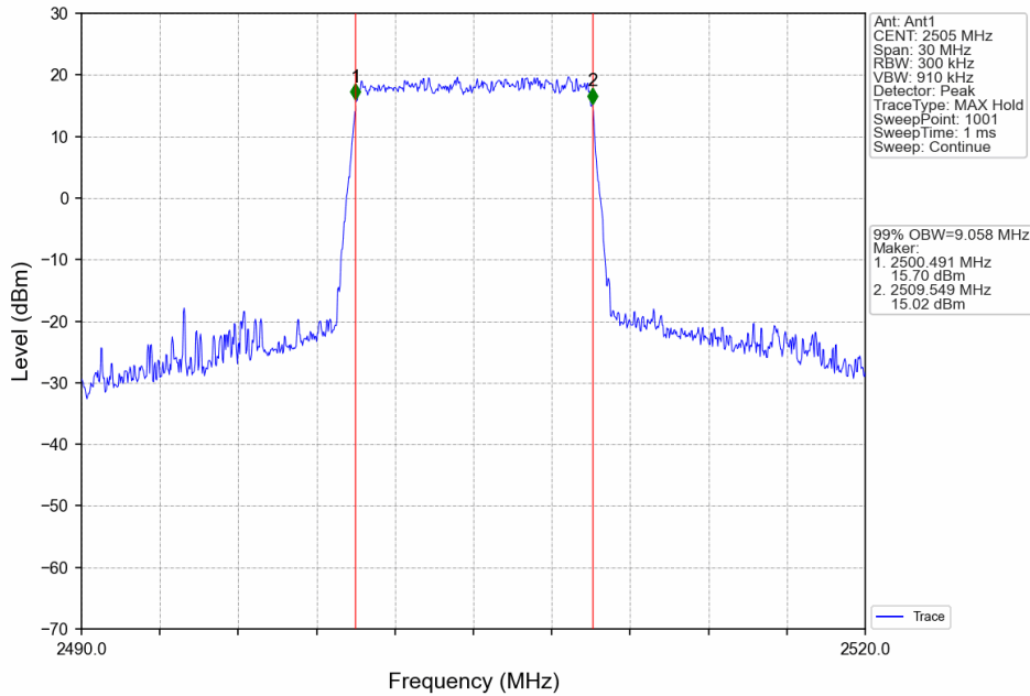
Band7_10MHz_64QAM_LCH_2505MHz_RB_50_0_NTNV
