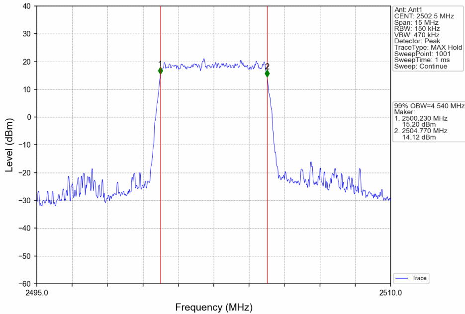
Band7_5MHz_64QAM_LCH_2502.5MHz_RB_25_0_NTNV
