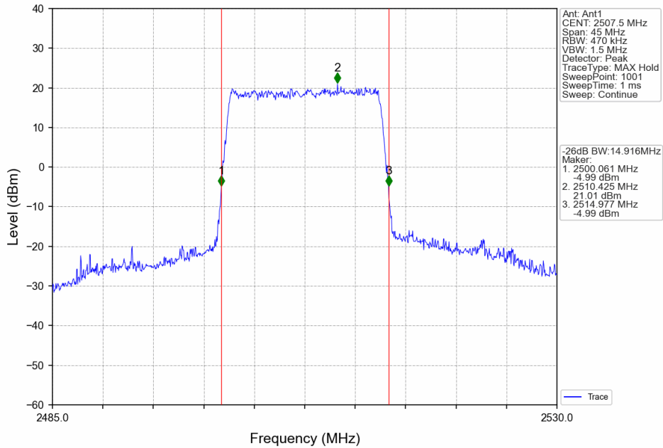
Band7_15MHz_64QAM_LCH_2507.5MHz_RB_75_0_NTNV
