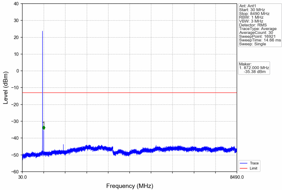
Band5_10MHz_64QAM_LCH_829MHz_RB_1_0_NTNV
