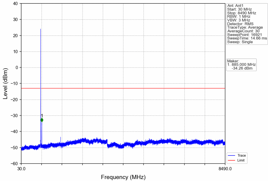
Band5_10MHz_64QAM_MCH_836.5MHz_RB_1_0_NTNV
