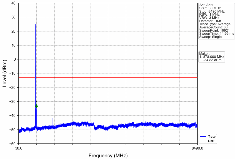
Band5_10MHz_16QAM_LCH_829MHz_RB_1_0_NTNV
