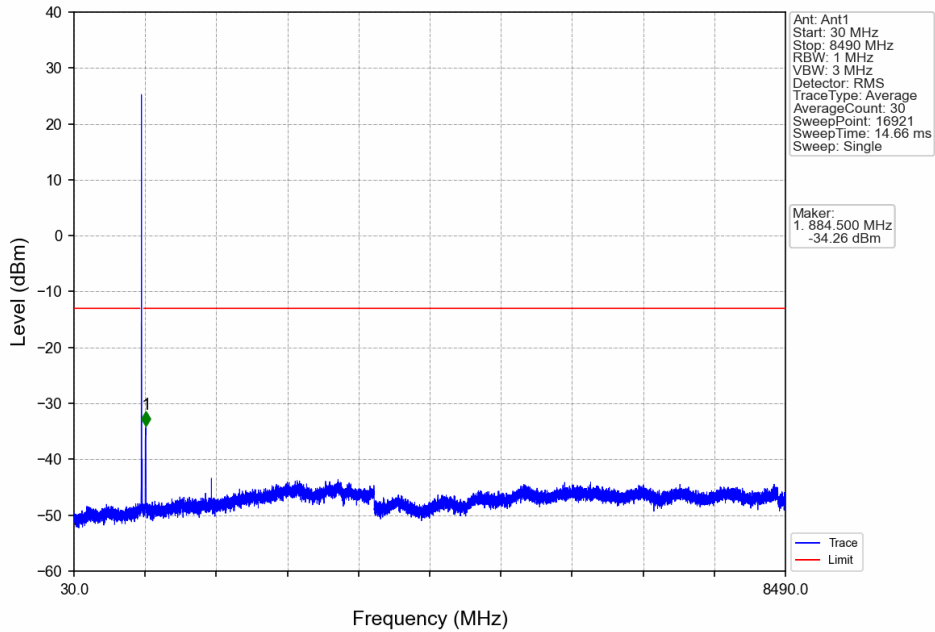
Band5_10MHz_16QAM_MCH_836.5MHz_RB_1_0_NTNV
