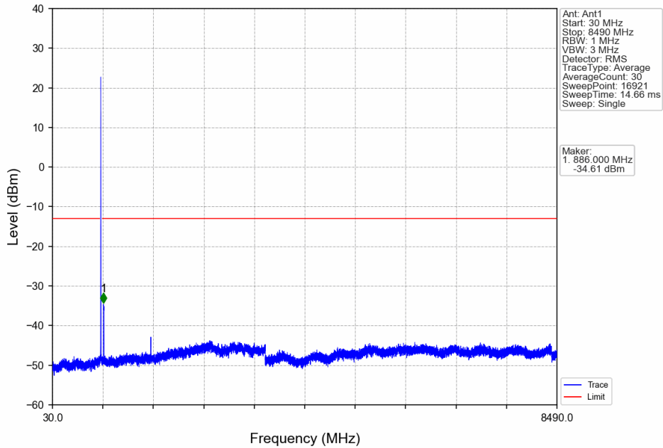
Band5_10MHz_64QAM_HCH_844MHz_RB_1_0_NTNV
