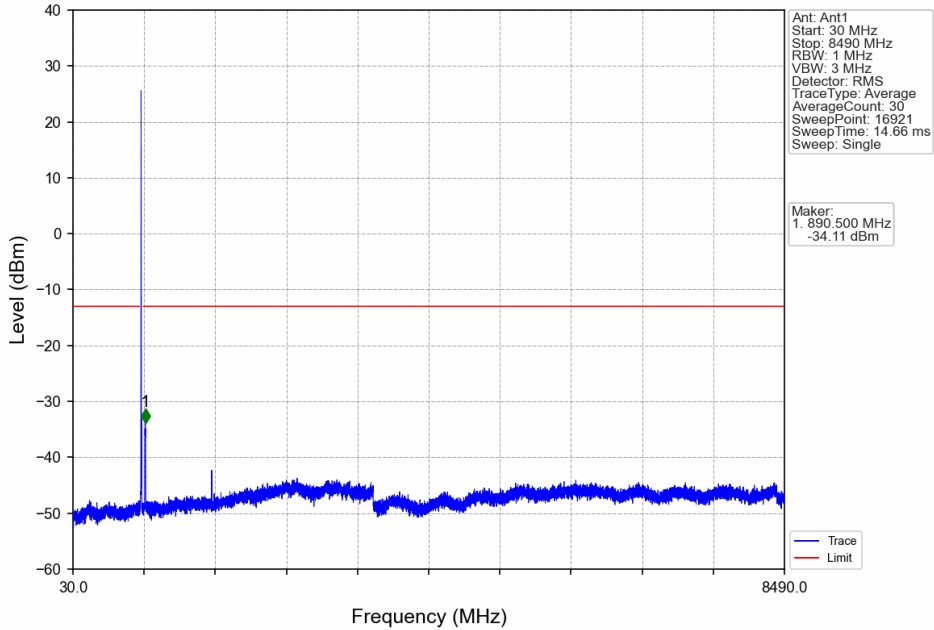
Band5_10MHz_16QAM_HCH_844MHz_RB_1_0_NTNV
