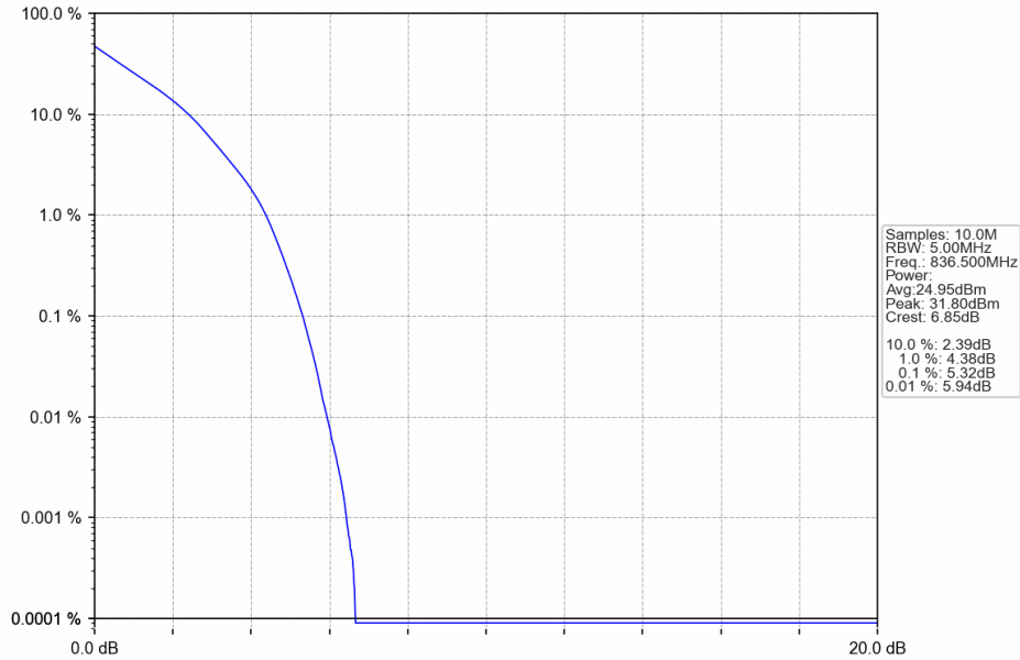
Band5_5MHz_QPSK_MCH_836.5MHz_RB_25_0_NTNV
