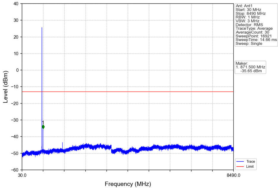
Band5_3MHz_64QAM_LCH_825.5MHz_RB_1_0_NTNV
