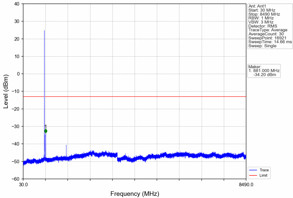
Band5_10MHz_QPSK_MCH_836.5MHz_RB_1_0_NTNV
