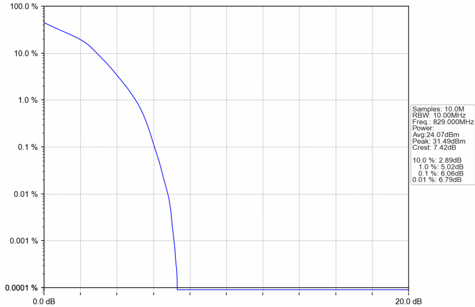
Band5_10MHz_16QAM_LCH_829MHz_RB_50_0_NTNV
