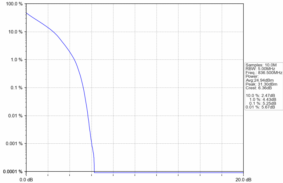
Band5_3MHz_QPSK_MCH_836.5MHz_RB_15_0_NTNV
