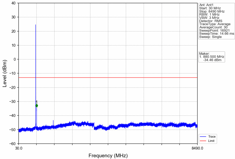
Band5_5MHz_64QAM_MCH_836.5MHz_RB_1_0_NTNV
