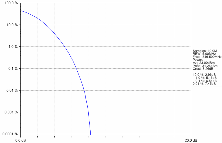
Band5_5MHz_64QAM_HCH_846.5MHz_RB_25_0_NTNV
