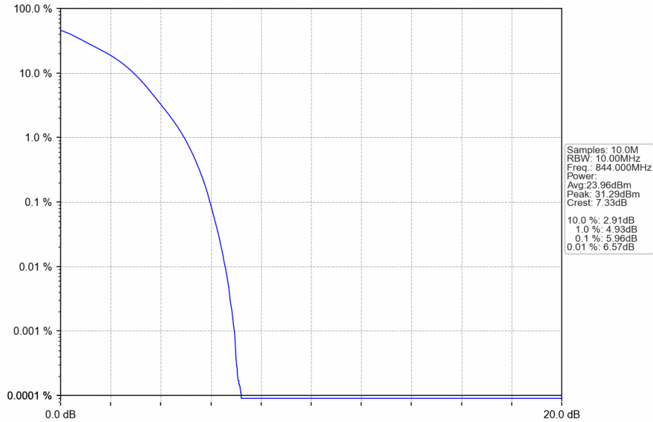
Band5_10MHz_16QAM_HCH_844MHz_RB_50_0_NTNV
