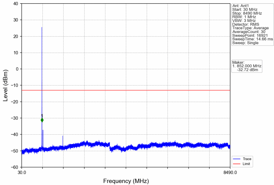
Band5_1.4MHz_QPSK_HCH_848.3MHz_RB_1_0_NTNV
