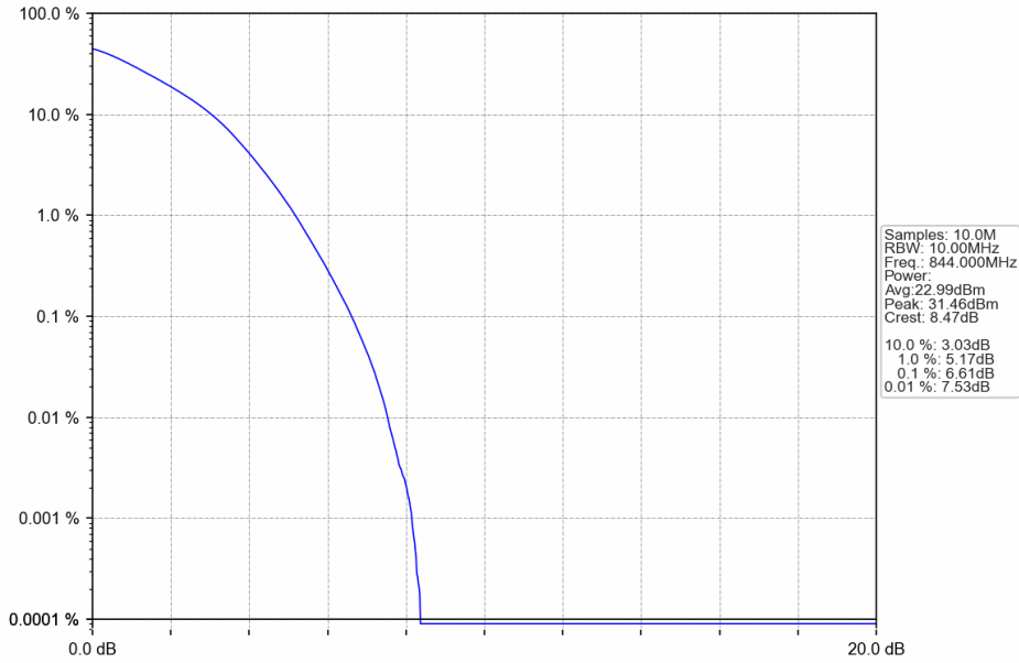
Band5_10MHz_64QAM_HCH_844MHz_RB_50_0_NTNV
