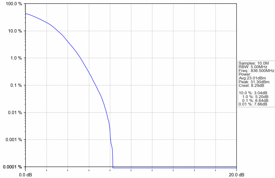
Band5_3MHz_64QAM_MCH_836.5MHz_RB_15_0_NTNV
