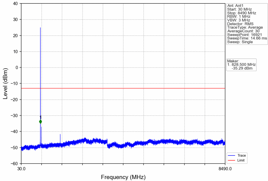
Band5_1.4MHz_QPSK_LCH_824.7MHz_RB_1_0_NTNV
