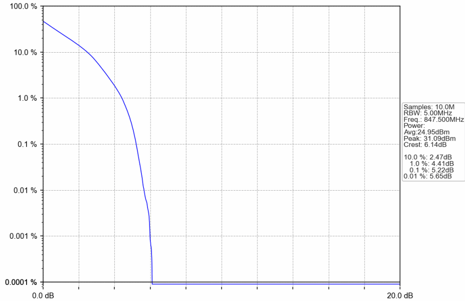
Band5_3MHz_QPSK_HCH_847.5MHz_RB_15_0_NTNV
