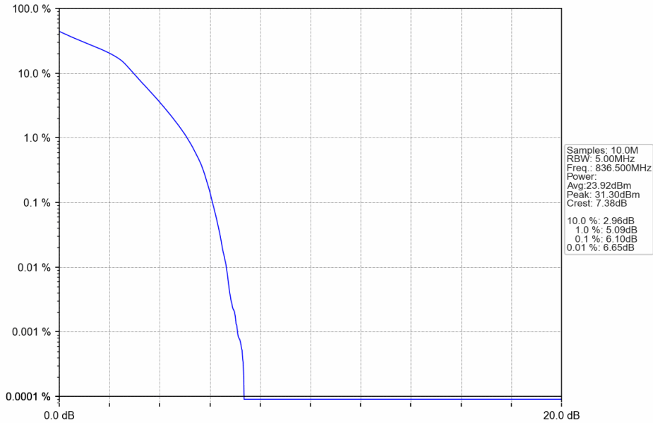
Band5_3MHz_16QAM_MCH_836.5MHz_RB_15_0_NTNV
