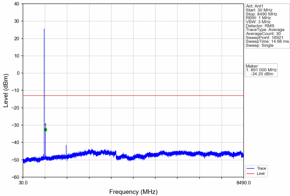
Band5_5MHz_16QAM_HCH_846.5MHz_RB_1_0_NTNV
