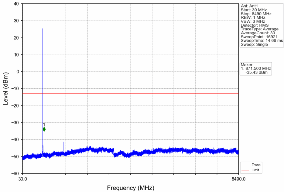
Band5_5MHz_16QAM_LCH_826.5MHz_RB_1_0_NTNV
