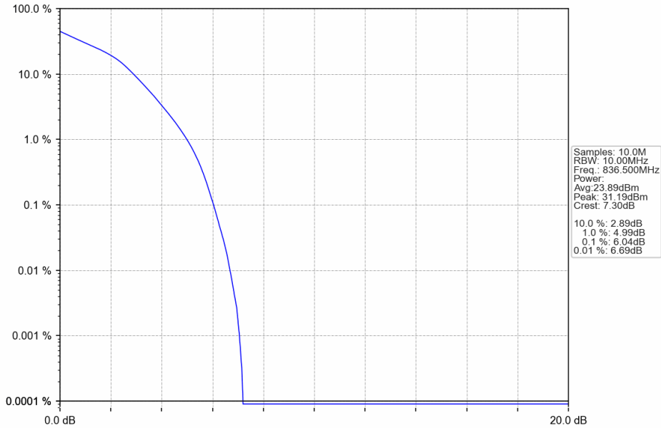
Band5_10MHz_16QAM_MCH_836.5MHz_RB_50_0_NTNV
