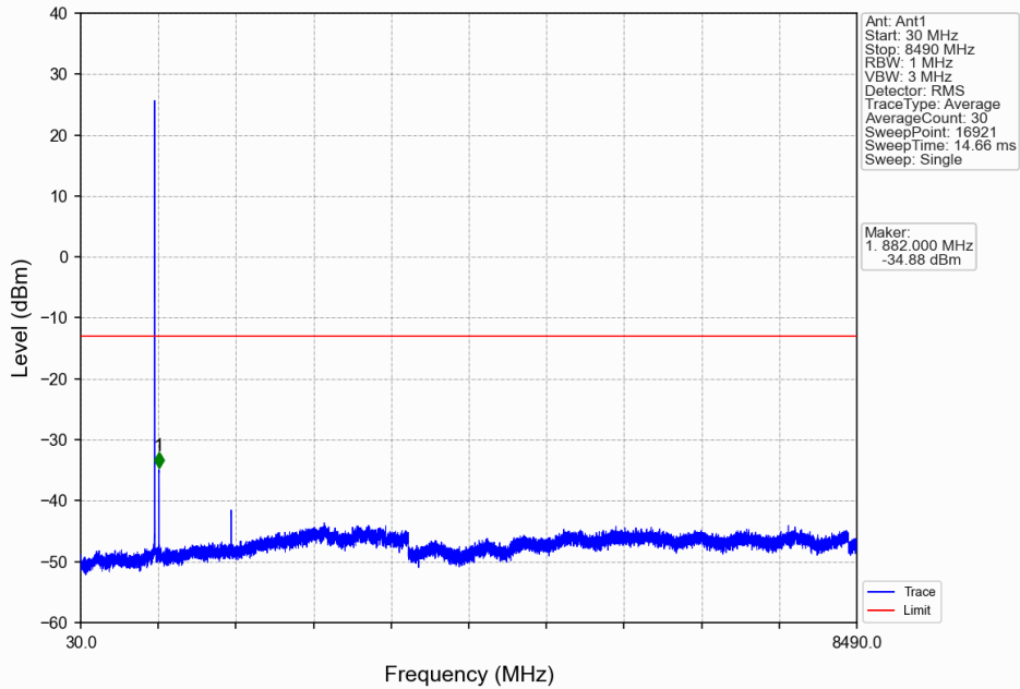
Band5_3MHz_16QAM_MCH_836.5MHz_RB_1_0_NTNV
