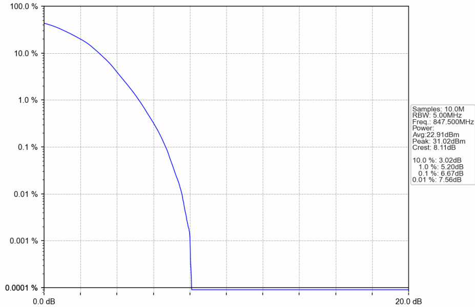
Band5_3MHz_64QAM_HCH_847.5MHz_RB_15_0_NTNV
