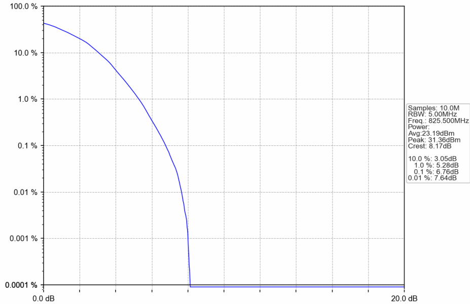
Band5_3MHz_64QAM_LCH_825.5MHz_RB_15_0_NTNV
