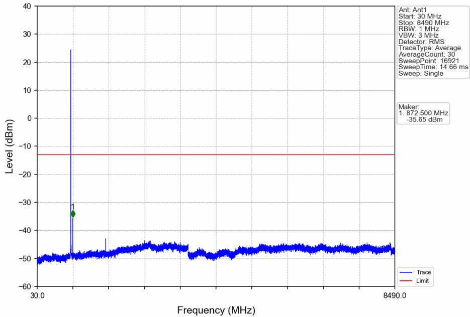
Band5_5MHz_64QAM_LCH_826.5MHz_RB_1_0_NTNV
