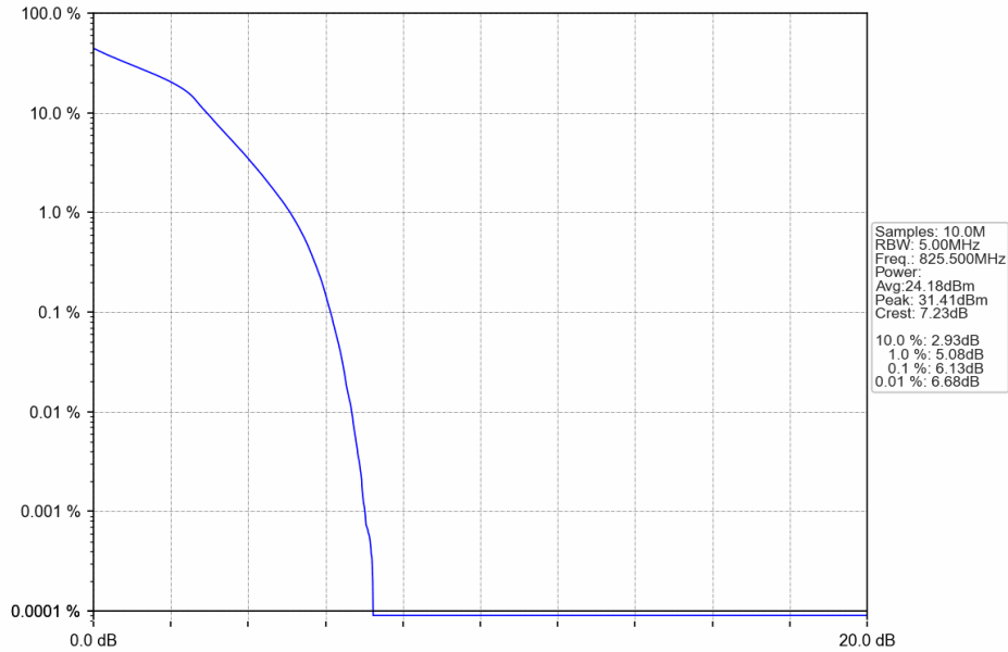
Band5_3MHz_16QAM_LCH_825.5MHz_RB_15_0_NTNV
