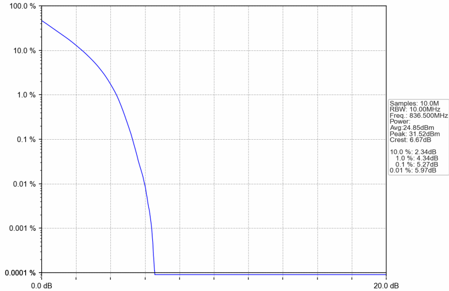
Band5_10MHz_QPSK_MCH_836.5MHz_RB_50_0_NTNV
