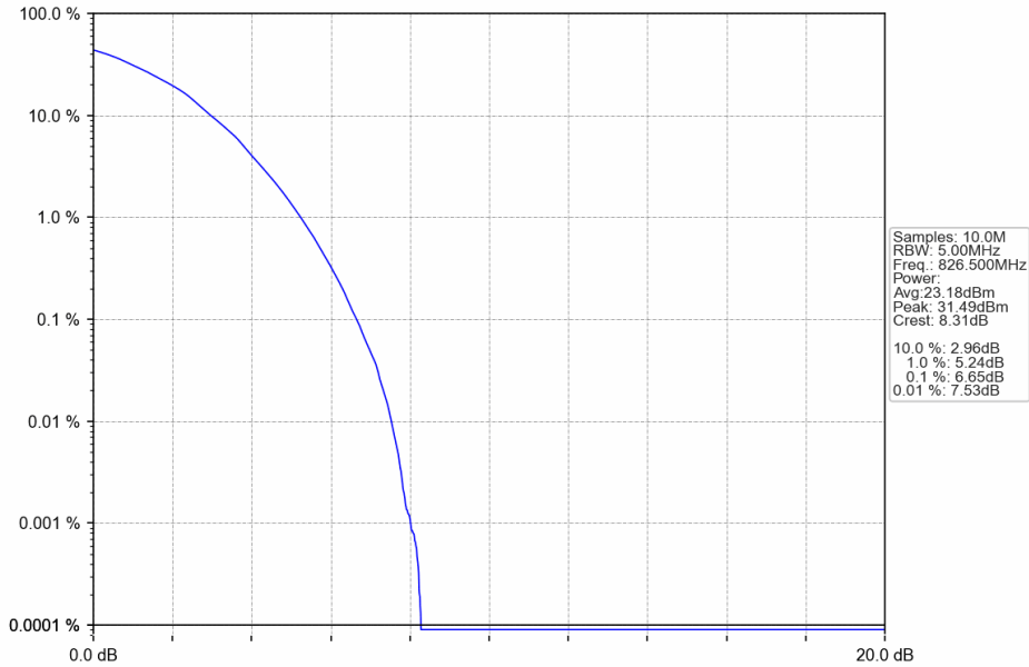
Band5_5MHz_64QAM_LCH_826.5MHz_RB_25_0_NTNV
