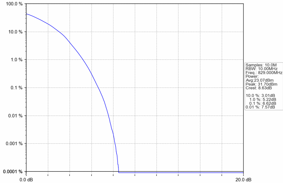
Band5_10MHz_64QAM_LCH_829MHz_RB_50_0_NTNV
