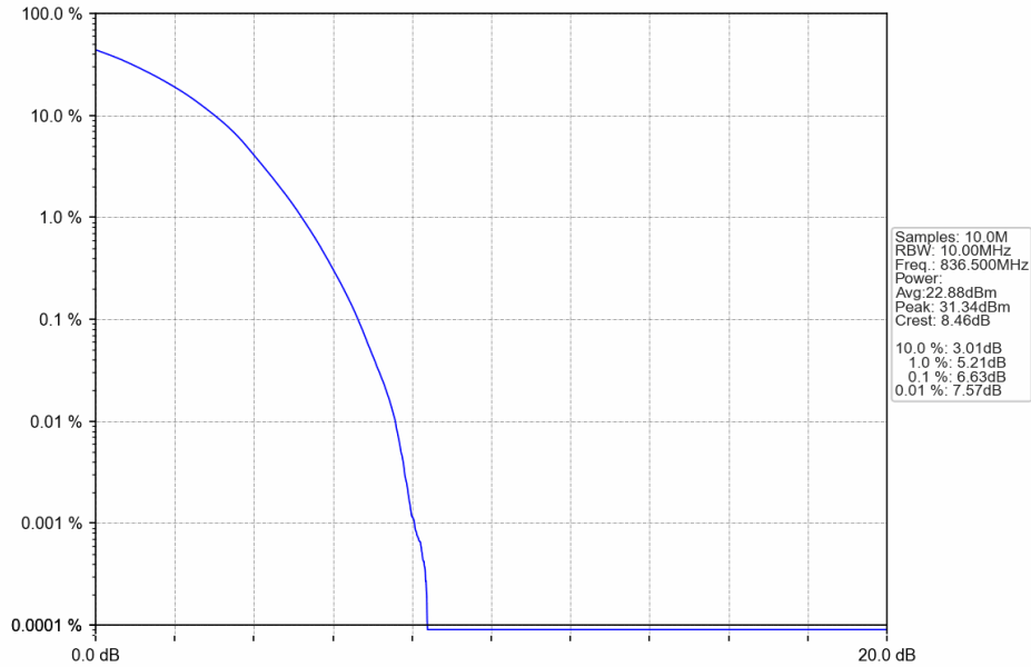
Band5_10MHz_64QAM_MCH_836.5MHz_RB_50_0_NTNV
