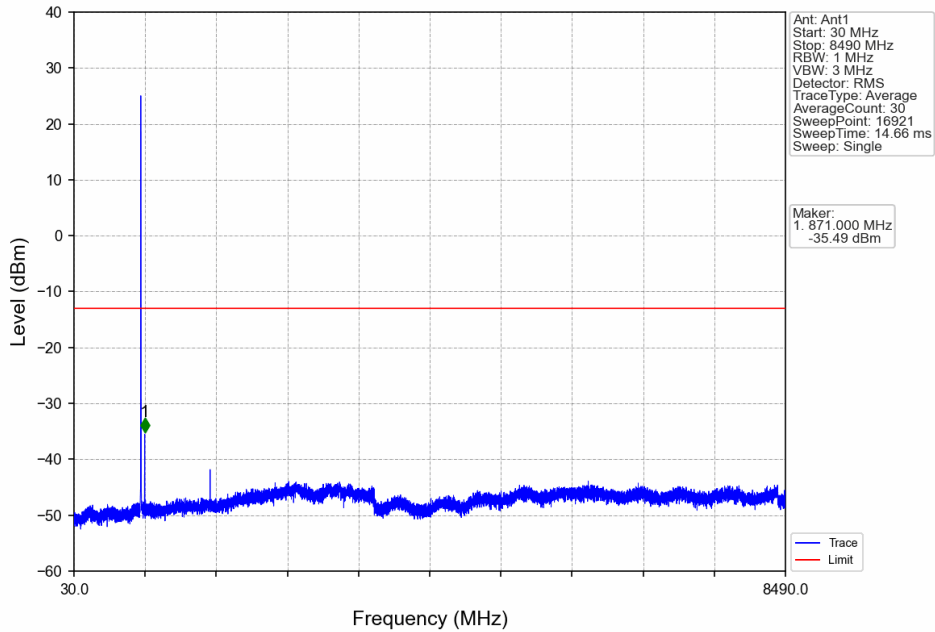
Band5_3MHz_16QAM_LCH_825.5MHz_RB_1_0_NTNV
