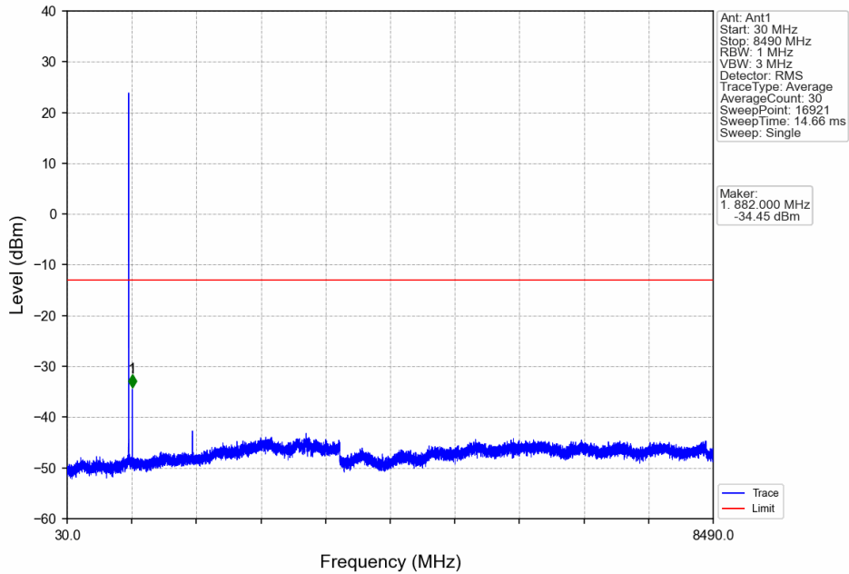
Band5_3MHz_64QAM_MCH_836.5MHz_RB_1_0_NTNV
