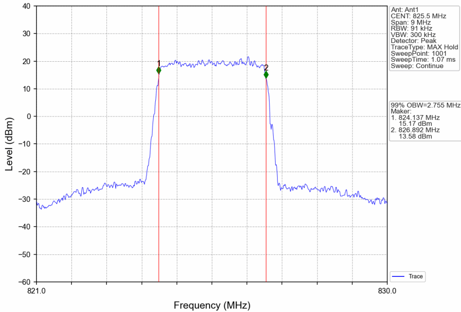
Band5_3MHz_16QAM_LCH_825.5MHz_RB_15_0_NTNV
