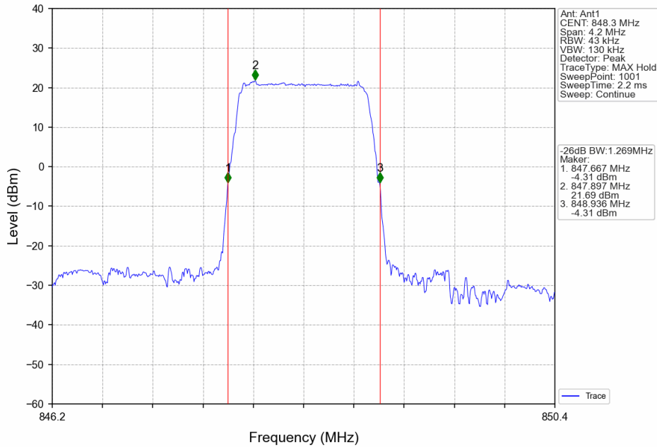
Band5_1.4MHz_QPSK_HCH_848.3MHz_RB_6_0_NTNV
