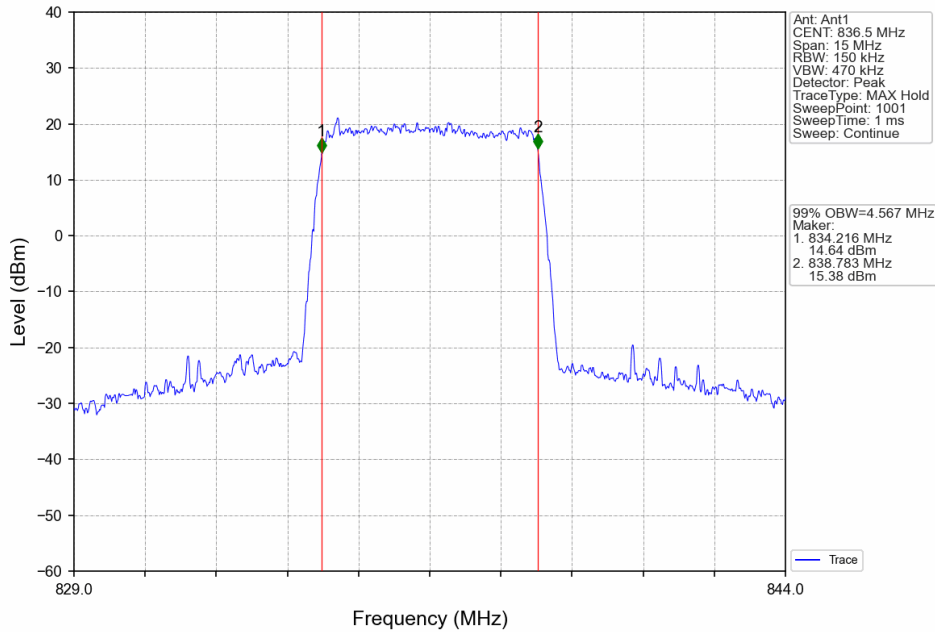
Band5_5MHz_16QAM_MCH_836.5MHz_RB_25_0_NTNV
