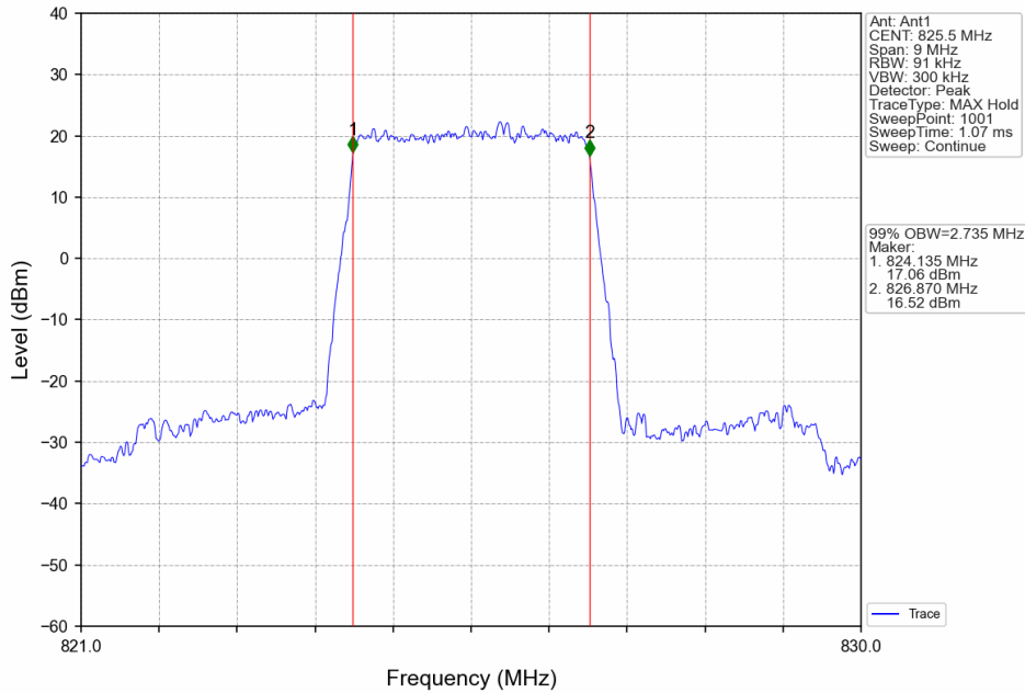
Band5_3MHz_QPSK_LCH_825.5MHz_RB_15_0_NTNV
