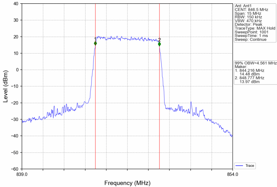
Band5_5MHz_16QAM_HCH_846.5MHz_RB_25_0_NTNV
