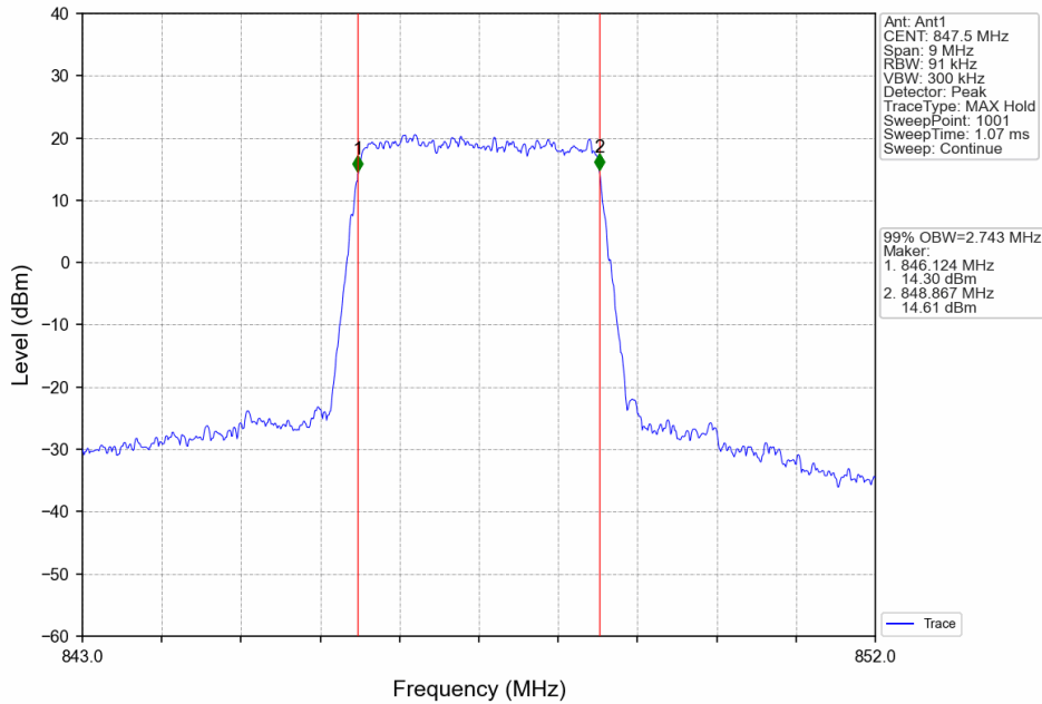
Band5_3MHz_16QAM_HCH_847.5MHz_RB_15_0_NTNV
