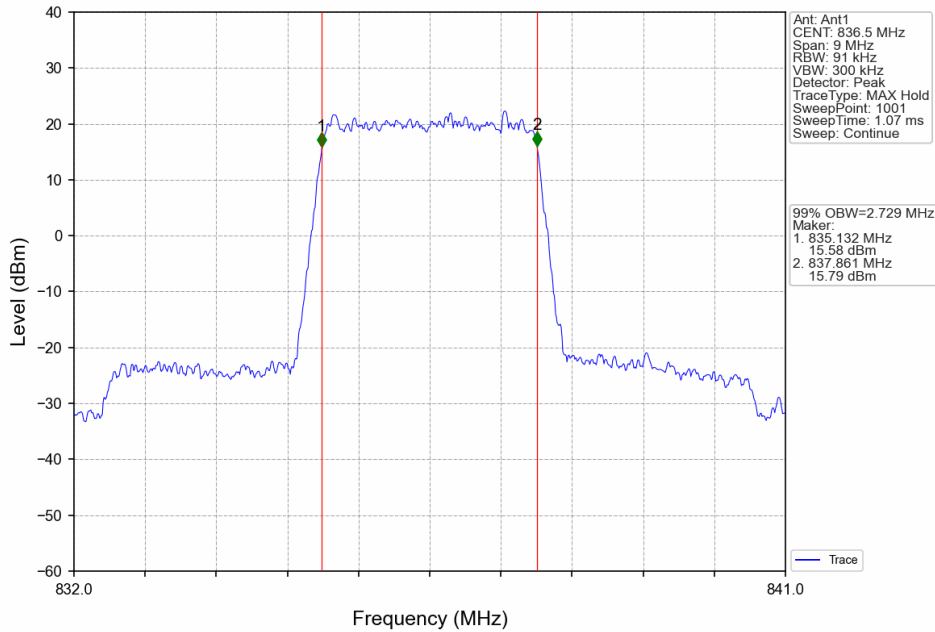
Band5_3MHz_QPSK_MCH_836.5MHz_RB_15_0_NTNV
