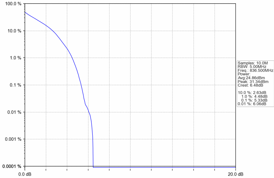
Band5_1.4MHz_QPSK_MCH_836.5MHz_RB_6_0_NTNV
