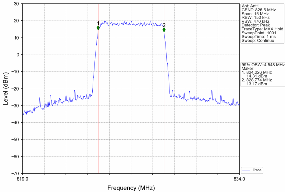
Band5_5MHz_64QAM_LCH_826.5MHz_RB_25_0_NTNV
