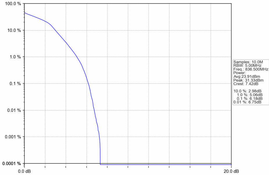
Band5_1.4MHz_16QAM_MCH_836.5MHz_RB_6_0_NTNV
