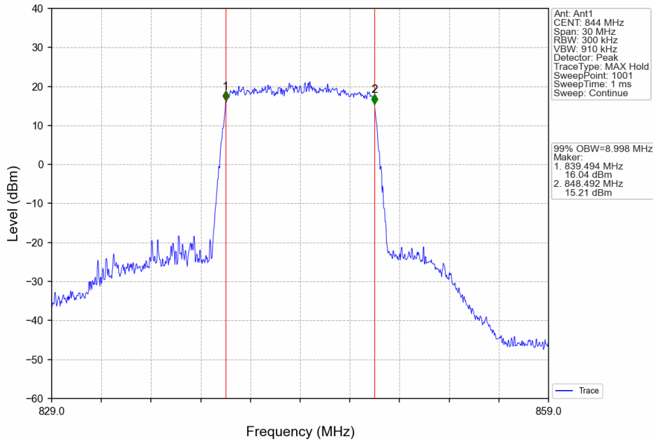
Band5_10MHz_16QAM_HCH_844MHz_RB_50_0_NTNV
