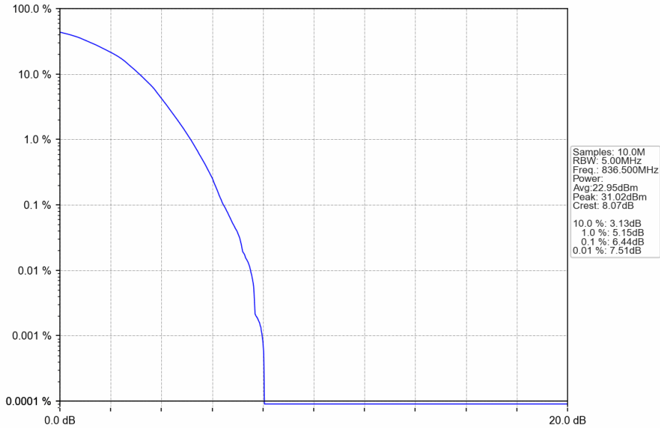
Band5_1.4MHz_64QAM_MCH_836.5MHz_RB_6_0_NTNV
