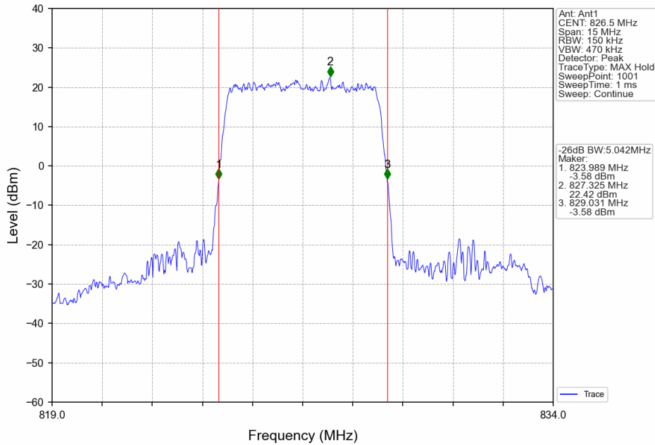
Band5_5MHz_QPSK_LCH_826.5MHz_RB_25_0_NTNV
