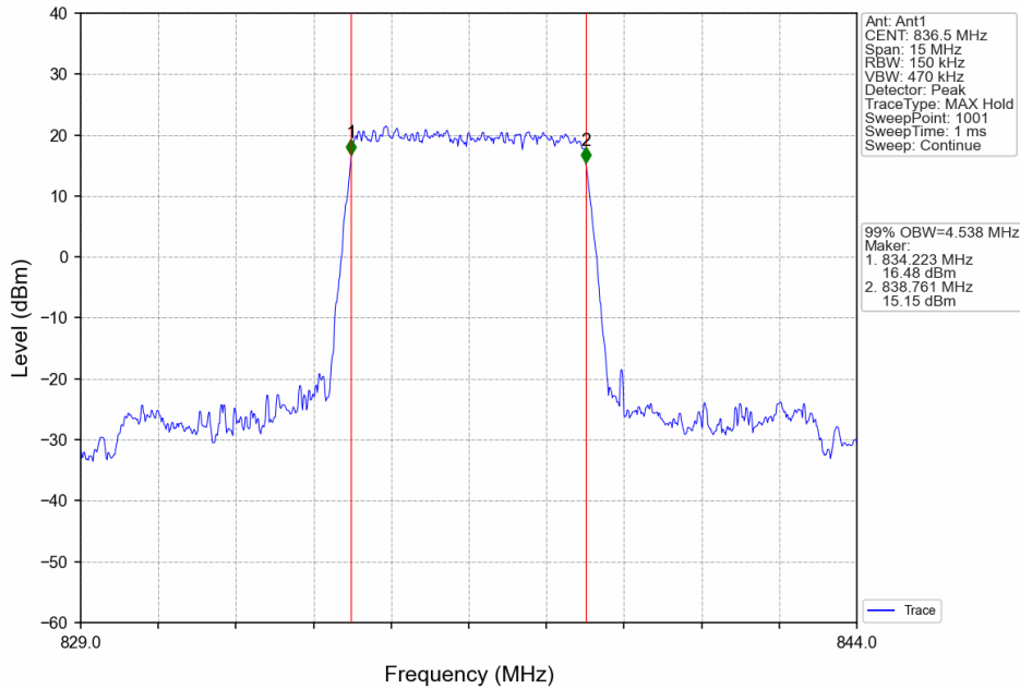
Band5_5MHz_QPSK_MCH_836.5MHz_RB_25_0_NTNV
