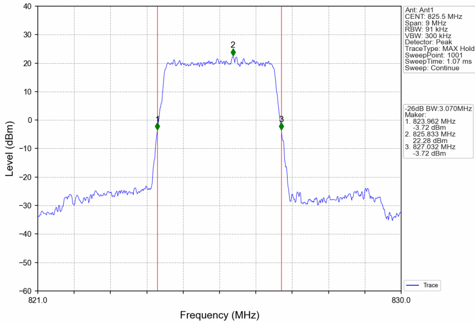
Band5_3MHz_QPSK_LCH_825.5MHz_RB_15_0_NTNV
