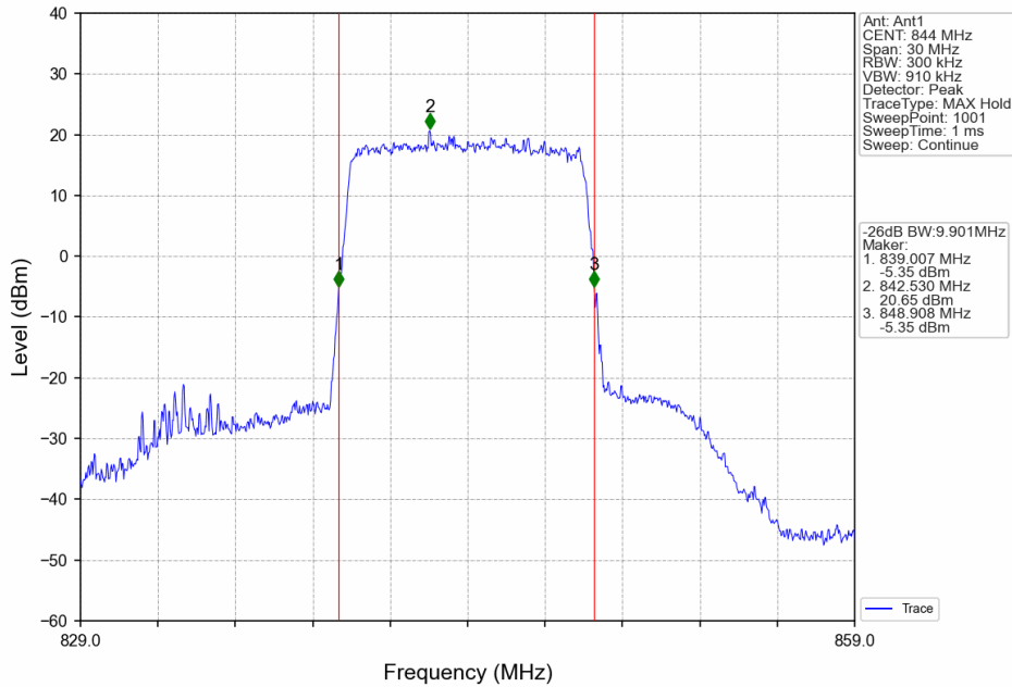
Band5_10MHz_64QAM_HCH_844MHz_RB_50_0_NTNV
