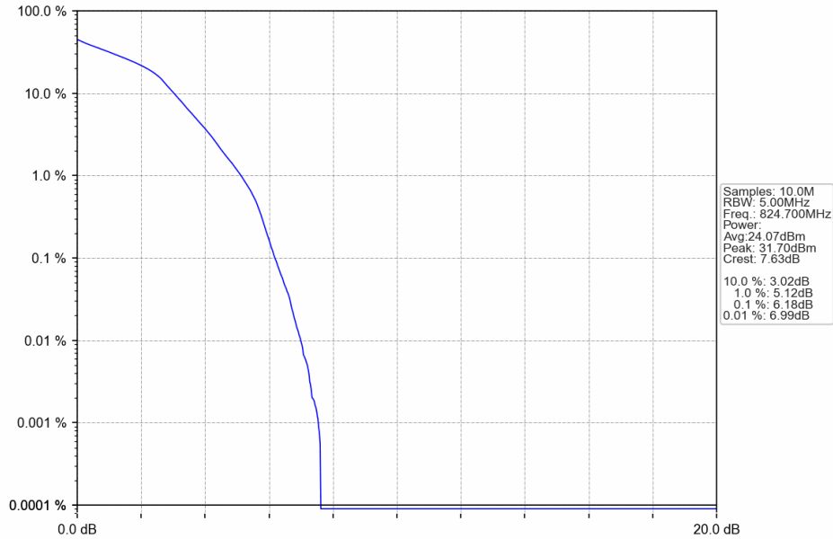
Band5_1.4MHz_16QAM_LCH_824.7MHz_RB_6_0_NTNV
