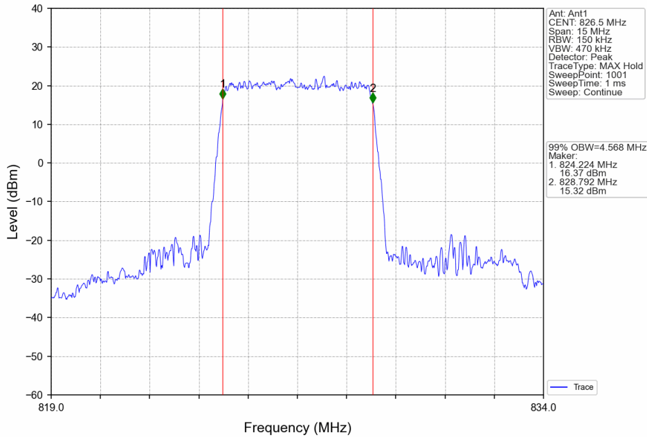
Band5_5MHz_QPSK_LCH_826.5MHz_RB_25_0_NTNV
