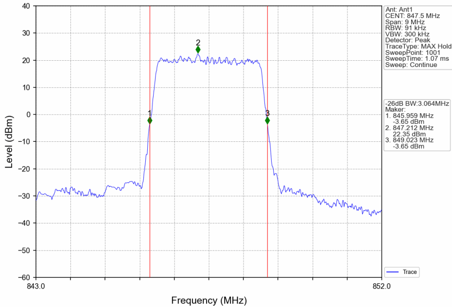
Band5_3MHz_QPSK_HCH_847.5MHz_RB_15_0_NTNV
