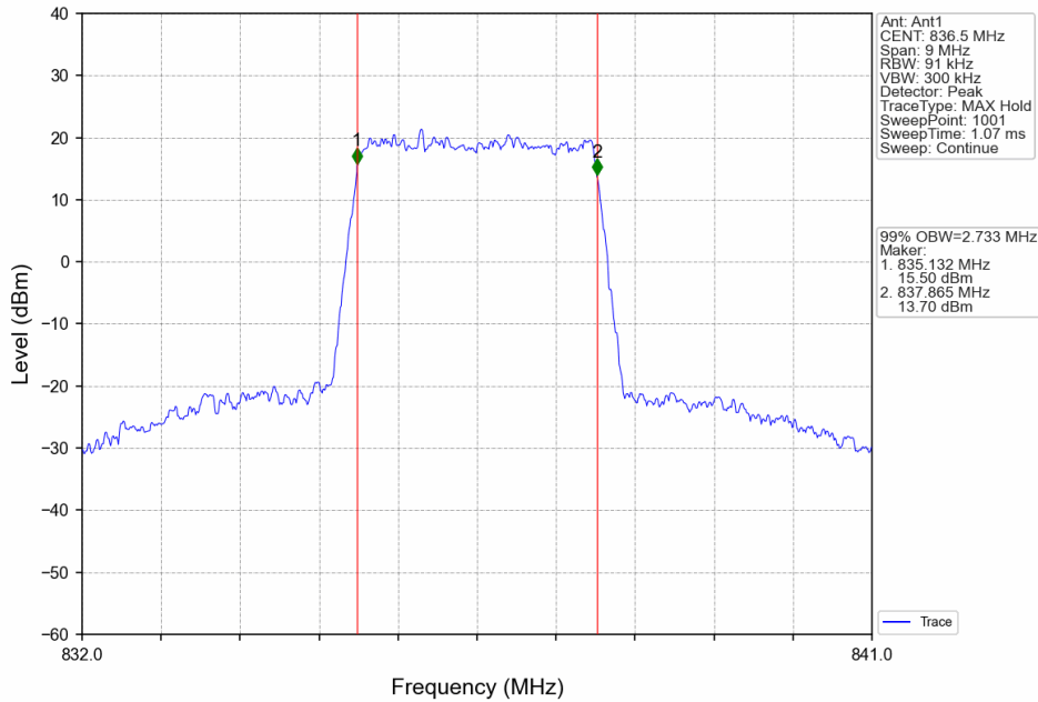
Band5_3MHz_16QAM_MCH_836.5MHz_RB_15_0_NTNV
