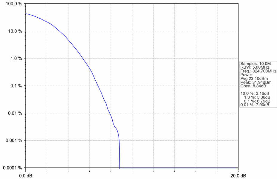
Band5_1.4MHz_64QAM_LCH_824.7MHz_RB_6_0_NTNV
