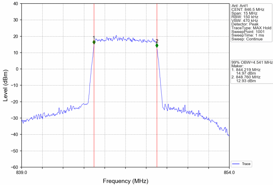
Band5_5MHz_64QAM_HCH_846.5MHz_RB_25_0_NTNV
