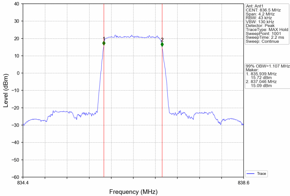
Band5_1.4MHz_QPSK_MCH_836.5MHz_RB_6_0_NTNV
