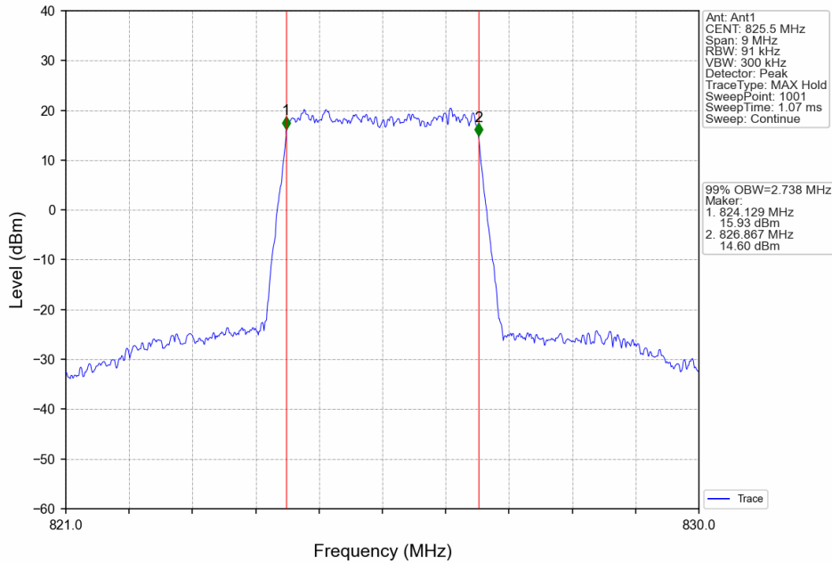
Band5_3MHz_64QAM_LCH_825.5MHz_RB_15_0_NTNV
