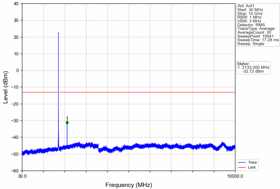
Band4_15MHz_64QAM_MCH_1732.5MHz_RB_1_0_NTNV
