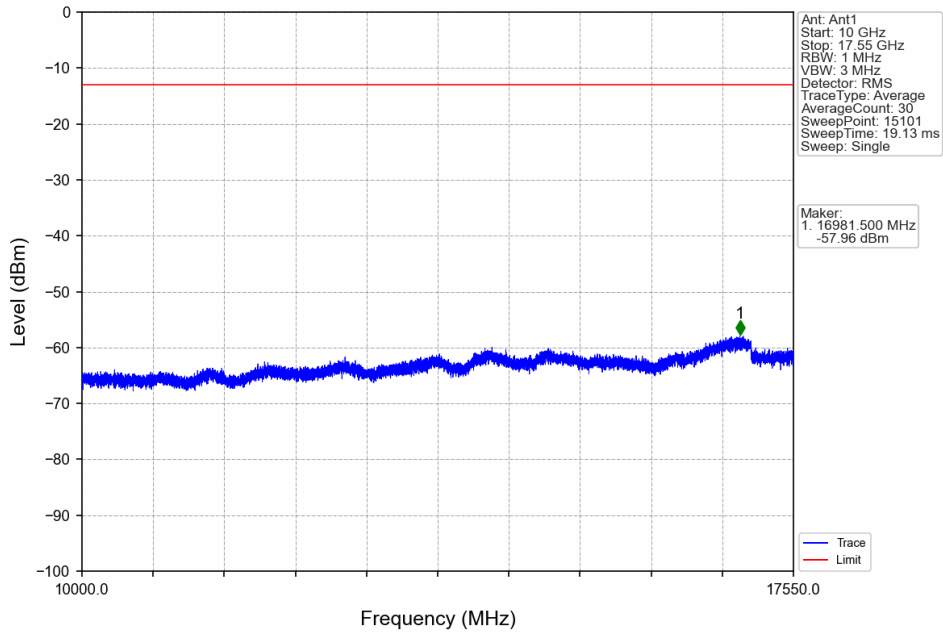
Band4_20MHz_64QAM_LCH_1720MHz_RB_1_0_NTNV
