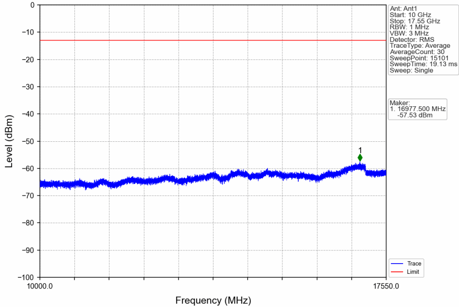
Band4_15MHz_64QAM_HCH_1747.5MHz_RB_1_0_NTNV
