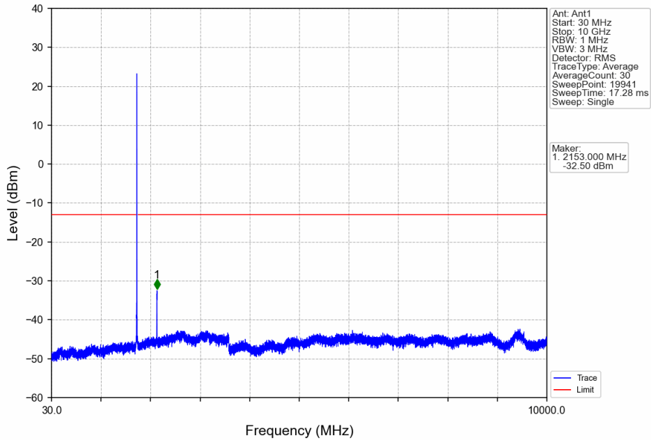
Band4_10MHz_64QAM_HCH_1750MHz_RB_1_0_NTNV
