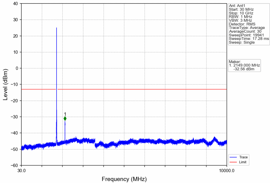
Band4_20MHz_16QAM_HCH_1745MHz_RB_1_0_NTNV
