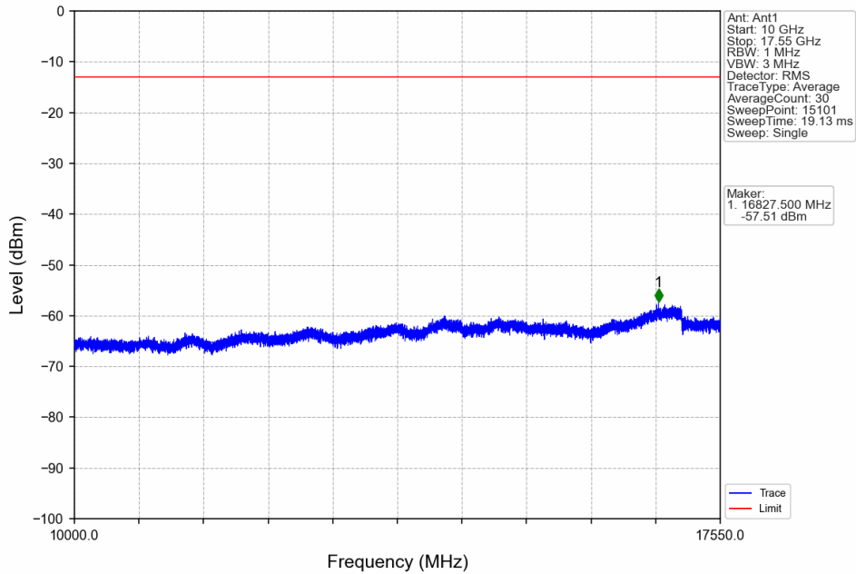
Band4_3MHz_QPSK_LCH_1711.5MHz_RB_1_0_NTNV
