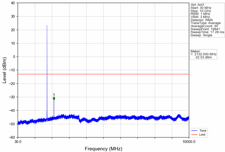
Band4_5MHz_16QAM_MCH_1732.5MHz_RB_1_0_NTNV
