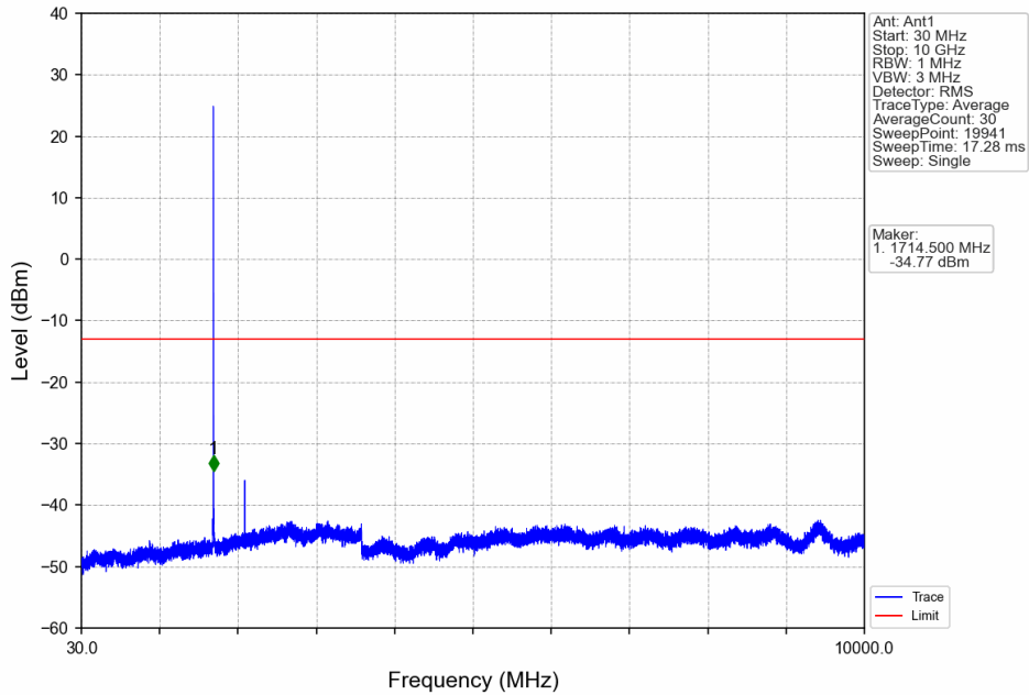
Band4_1.4MHz_64QAM_LCH_1710.7MHz_RB_1_0_NTNV
