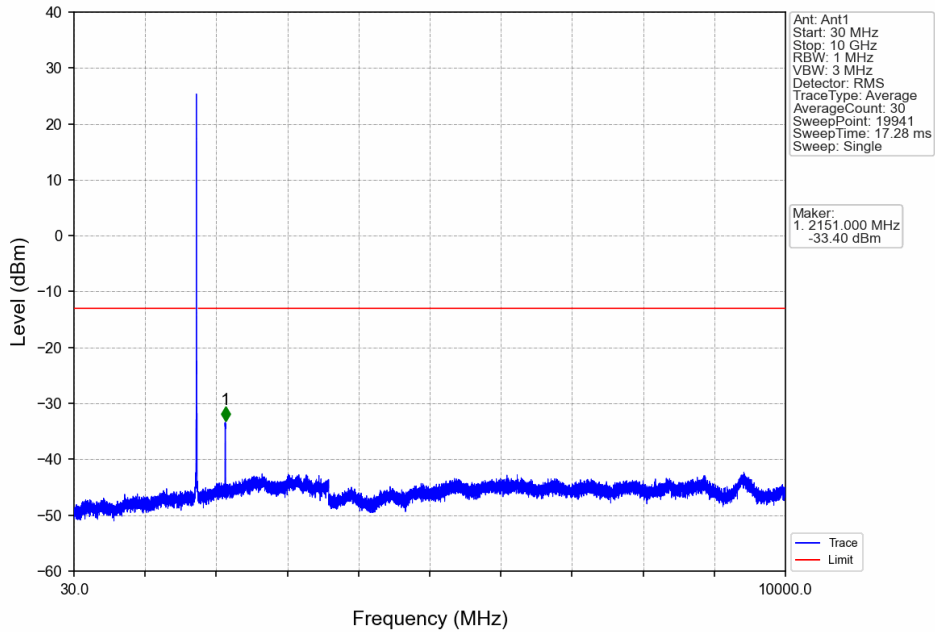
Band4_10MHz_16QAM_HCH_1750MHz_RB_1_0_NTNV
