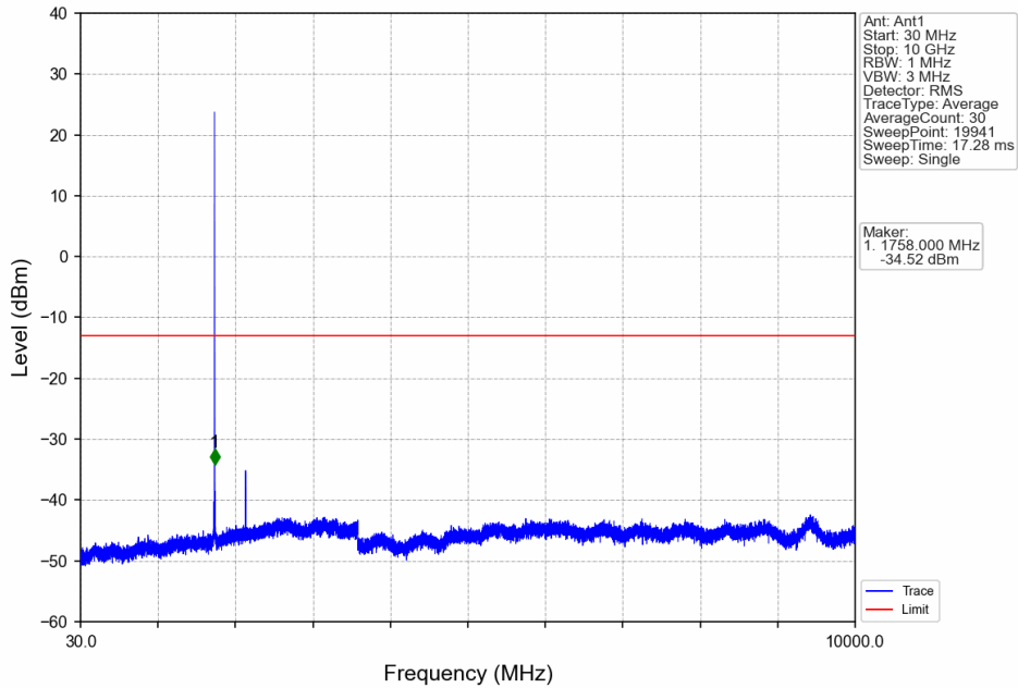
Band4_1.4MHz_64QAM_HCH_1754.3MHz_RB_1_0_NTNV
