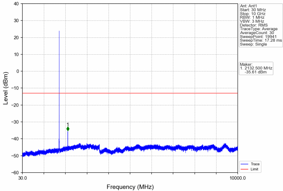
Band4_1.4MHz_64QAM_MCH_1732.5MHz_RB_1_0_NTNV
