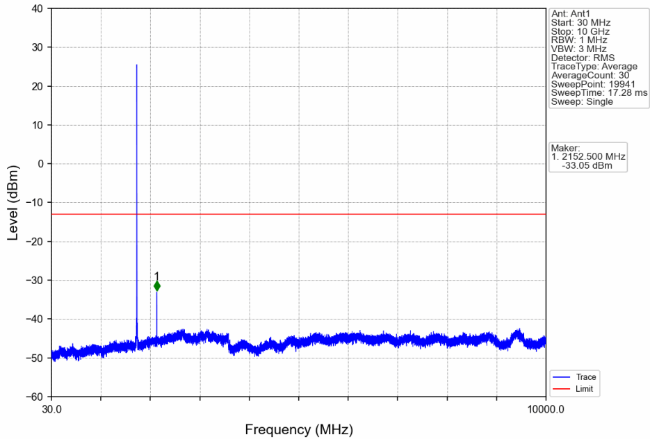
Band4_5MHz_QPSK_HCH_1752.5MHz_RB_1_0_NTNV
