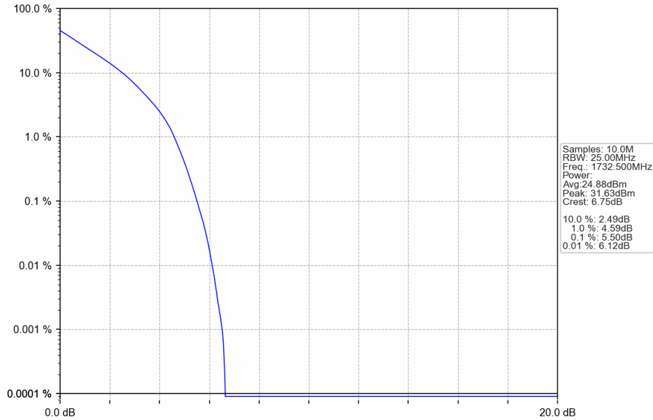
Band4_15MHz_QPSK_MCH_1732.5MHz_RB_75_0_NTNV
