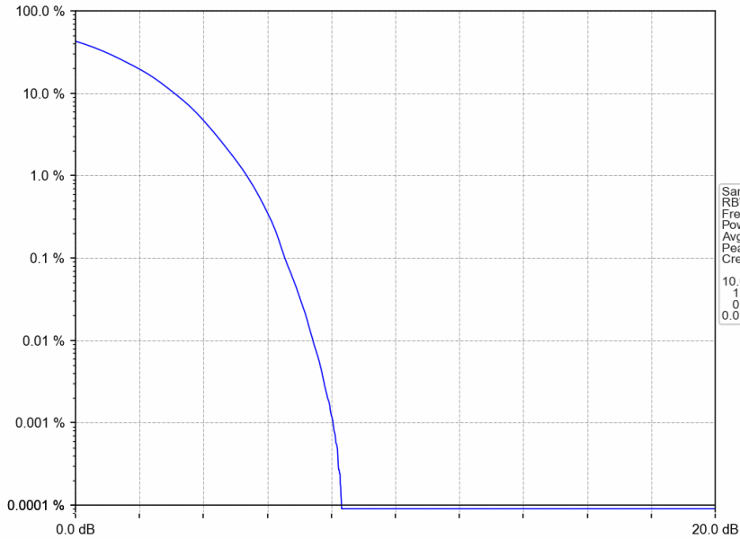
Band4_15MHz_64QAM_LCH_1717.5MHz_RB_75_0_NTNV
