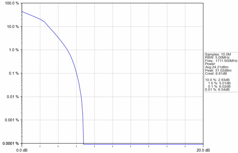
Band4_3MHz_16QAM_LCH_1711.5MHz_RB_15_0_NTNV
