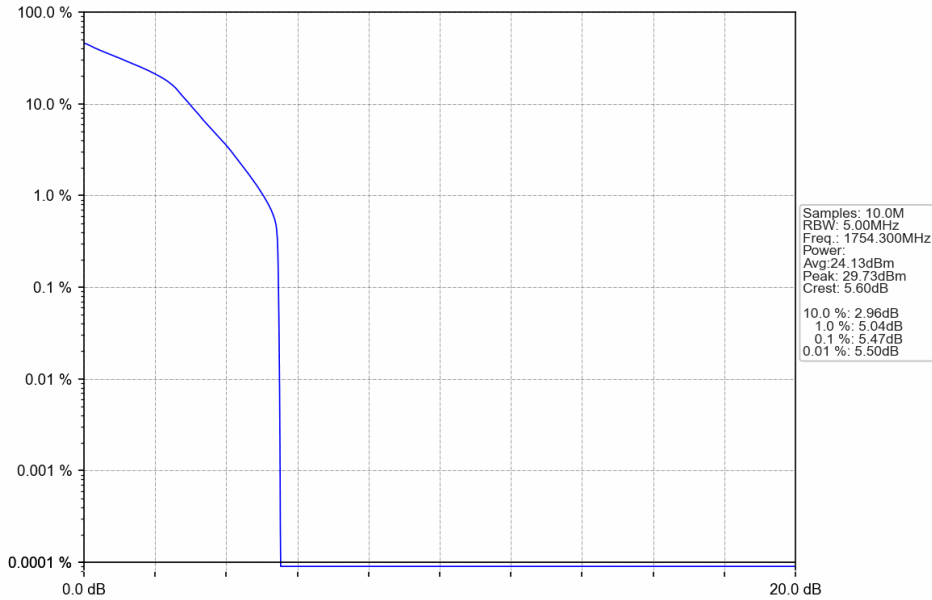
Band4_1.4MHz_16QAM_HCH_1754.3MHz_RB_6_0_NTNV
