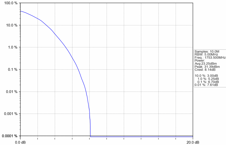
Band4_3MHz_64QAM_HCH_1753.5MHz_RB_15_0_NTNV
