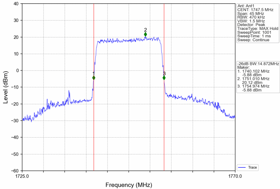
Band4_15MHz_64QAM_HCH_1747.5MHz_RB_75_0_NTNV
