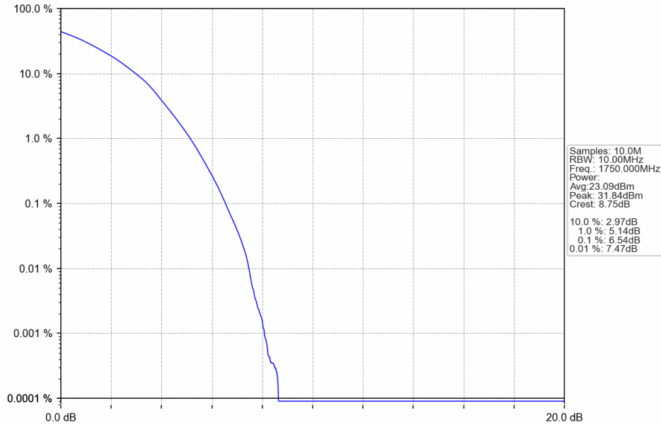
Band4_10MHz_64QAM_HCH_1750MHz_RB_50_0_NTNV
