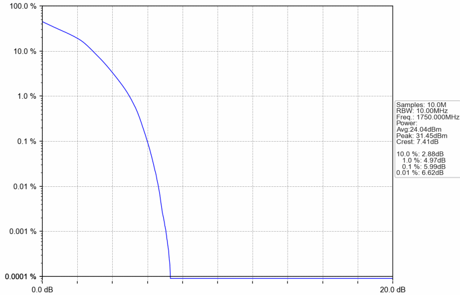
Band4_10MHz_16QAM_HCH_1750MHz_RB_50_0_NTNV
