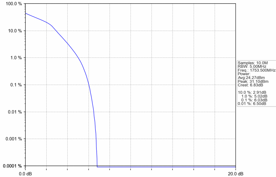
Band4_3MHz_16QAM_HCH_1753.5MHz_RB_15_0_NTNV
