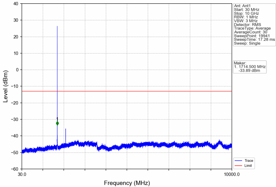
Band4_1.4MHz_QPSK_LCH_1710.7MHz_RB_1_0_NTNV
