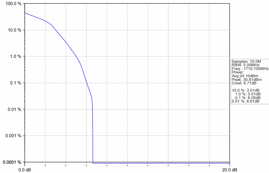
Band4_1.4MHz_16QAM_LCH_1710.7MHz_RB_6_0_NTNV
