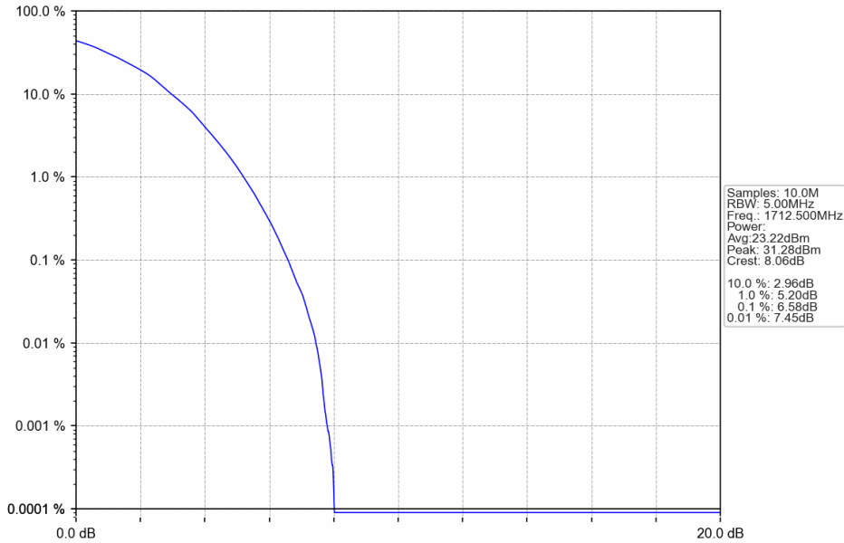
Band4_5MHz_64QAM_LCH_1712.5MHz_RB_25_0_NTNV
