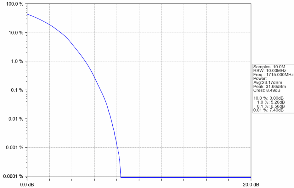
Band4_10MHz_64QAM_LCH_1715MHz_RB_50_0_NTNV
