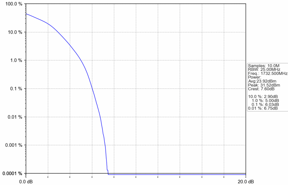
Band4_20MHz_16QAM_MCH_1732.5MHz_RB_100_0_NTNV
