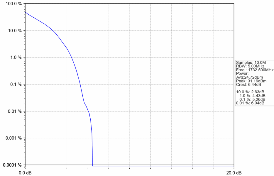
Band4_1.4MHz_QPSK_MCH_1732.5MHz_RB_6_0_NTNV
