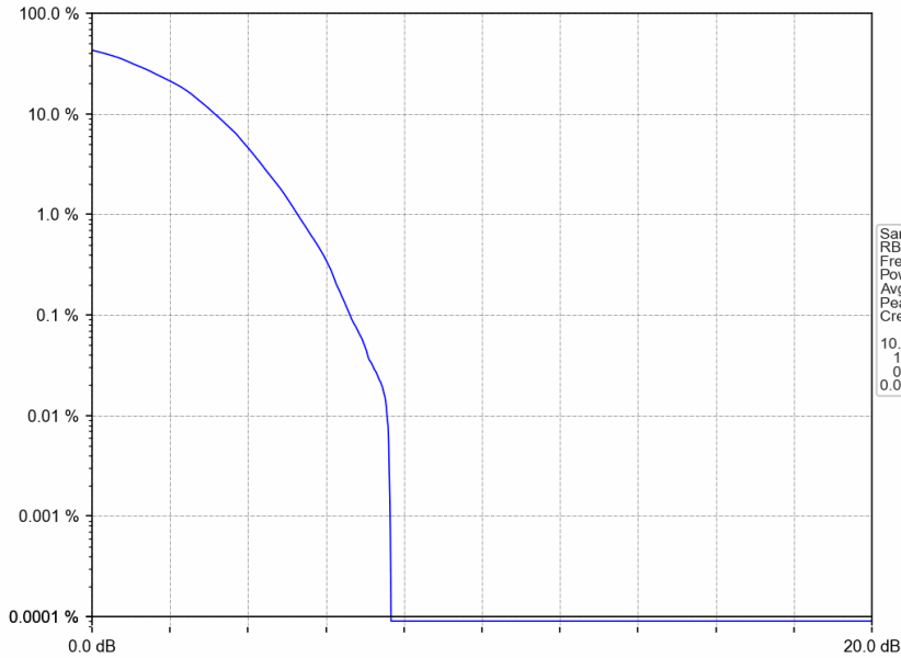
Band4_1.4MHz_64QAM_LCH_1710.7MHz_RB_6_0_NTNV
