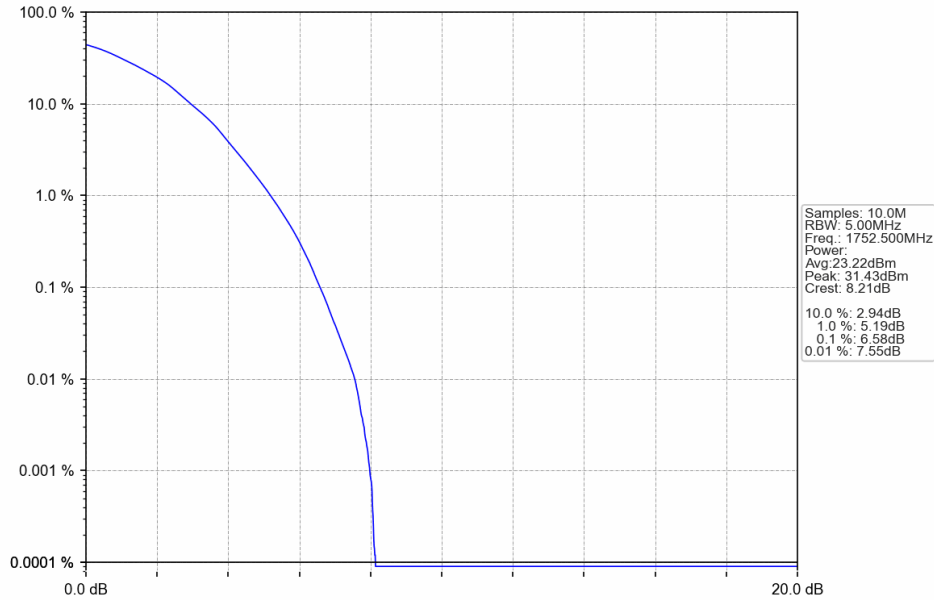
Band4_5MHz_64QAM_HCH_1752.5MHz_RB_25_0_NTNV
