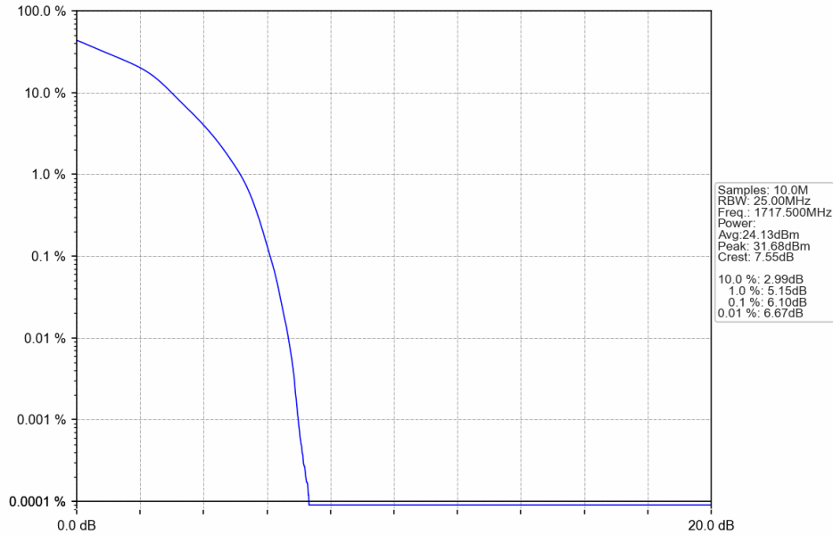
Band4_15MHz_16QAM_LCH_1717.5MHz_RB_75_0_NTNV
