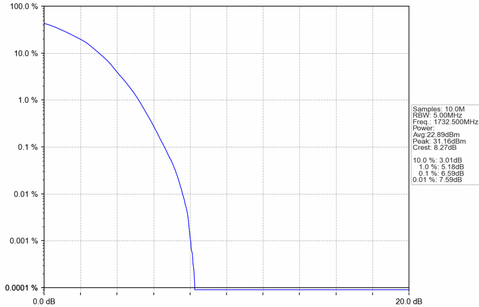
Band4_3MHz_64QAM_MCH_1732.5MHz_RB_15_0_NTNV
