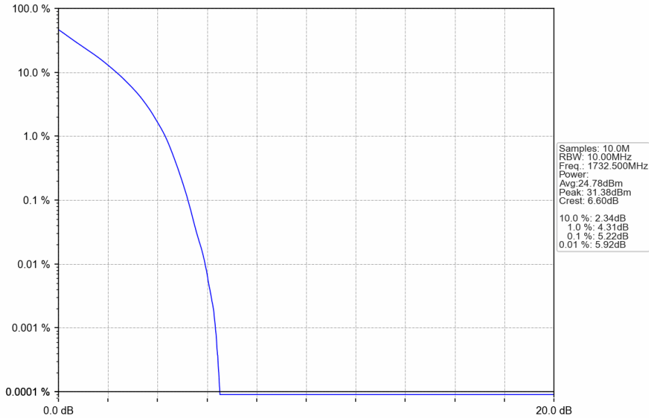
Band4_10MHz_QPSK_MCH_1732.5MHz_RB_50_0_NTNV
