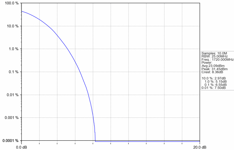
Band4_20MHz_64QAM_LCH_1720MHz_RB_100_0_NTNV
