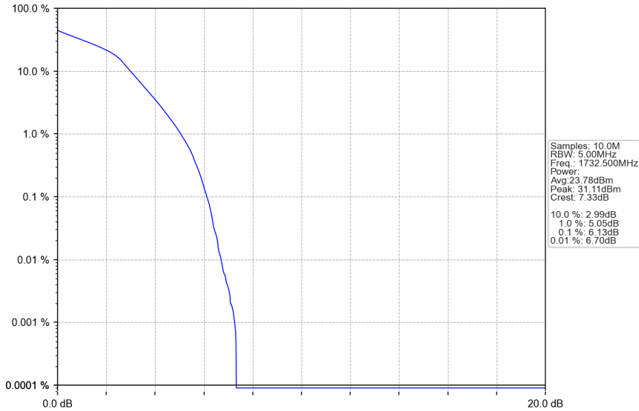
Band4_1.4MHz_16QAM_MCH_1732.5MHz_RB_6_0_NTNV
