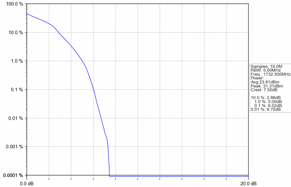
Band4_5MHz_16QAM_MCH_1732.5MHz_RB_25_0_NTNV
