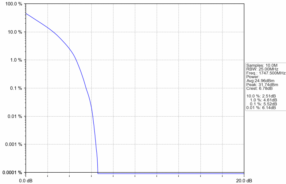
Band4_15MHz_QPSK_HCH_1747.5MHz_RB_75_0_NTNV
