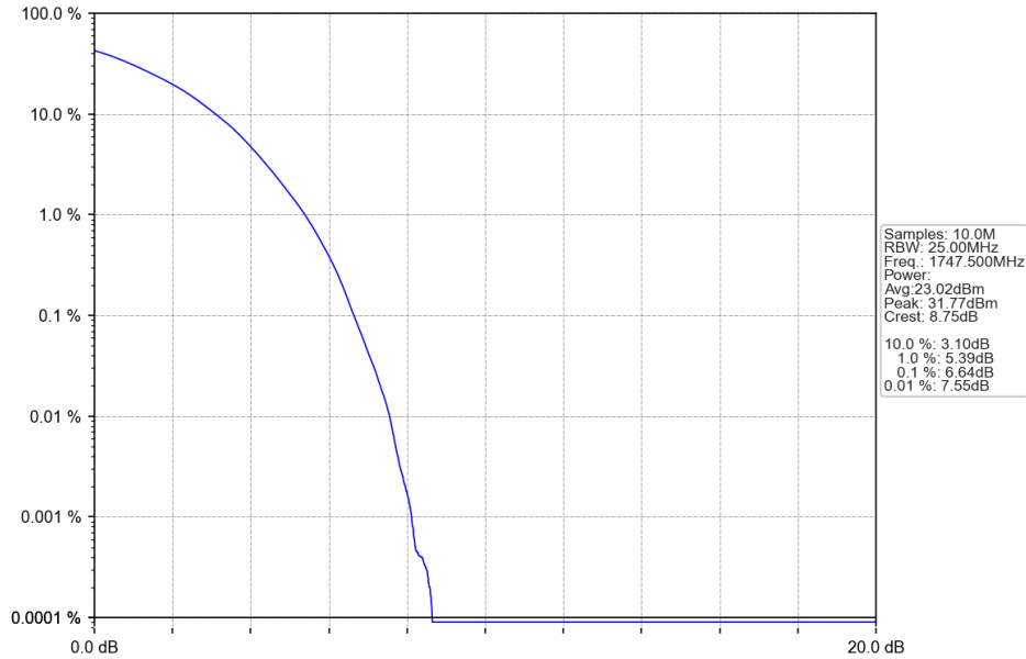
Band4_15MHz_64QAM_HCH_1747.5MHz_RB_75_0_NTNV
