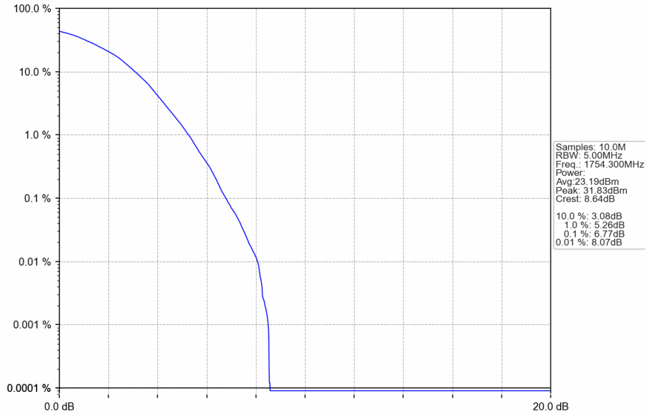
Band4_1.4MHz_64QAM_HCH_1754.3MHz_RB_6_0_NTNV
