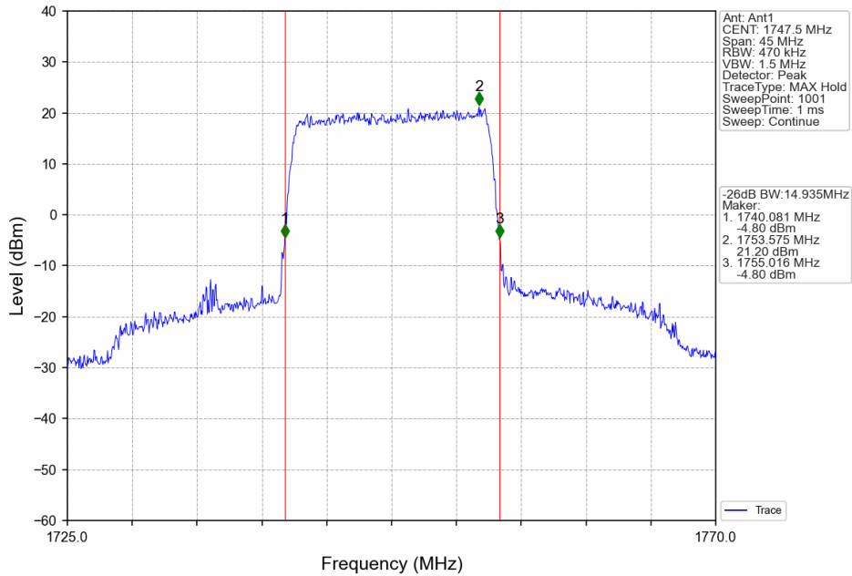
Band4_15MHz_16QAM_HCH_1747.5MHz_RB_75_0_NTNV
