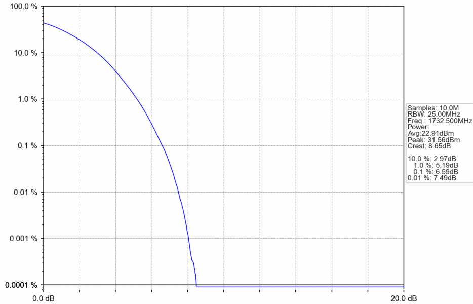
Band4_20MHz_64QAM_MCH_1732.5MHz_RB_100_0_NTNV
