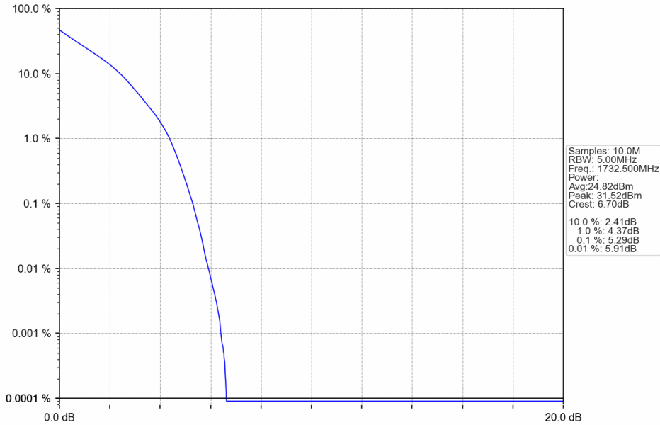
Band4_5MHz_QPSK_MCH_1732.5MHz_RB_25_0_NTNV
