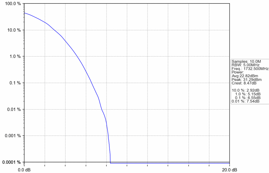
Band4_5MHz_64QAM_MCH_1732.5MHz_RB_25_0_NTNV
