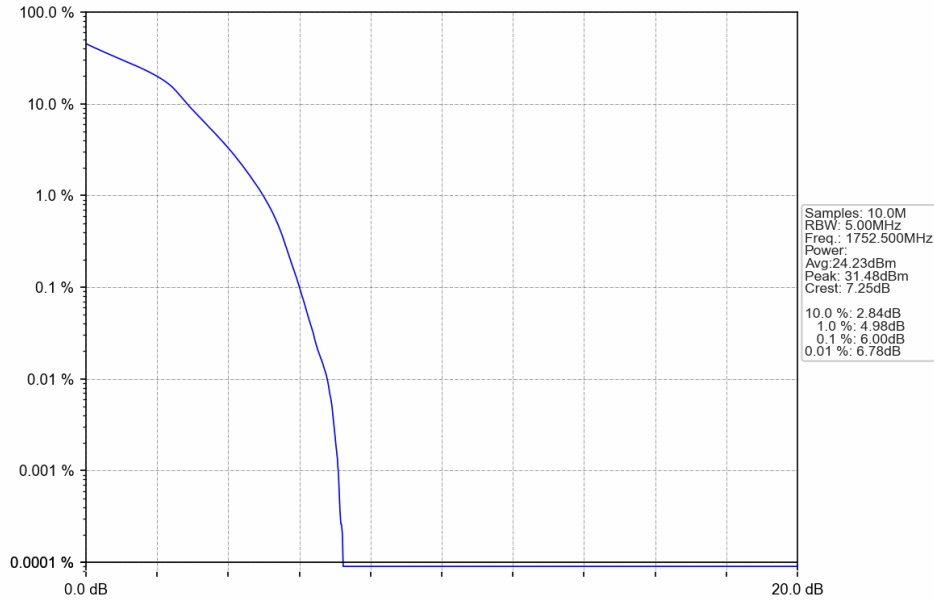
Band4_5MHz_16QAM_HCH_1752.5MHz_RB_25_0_NTNV
