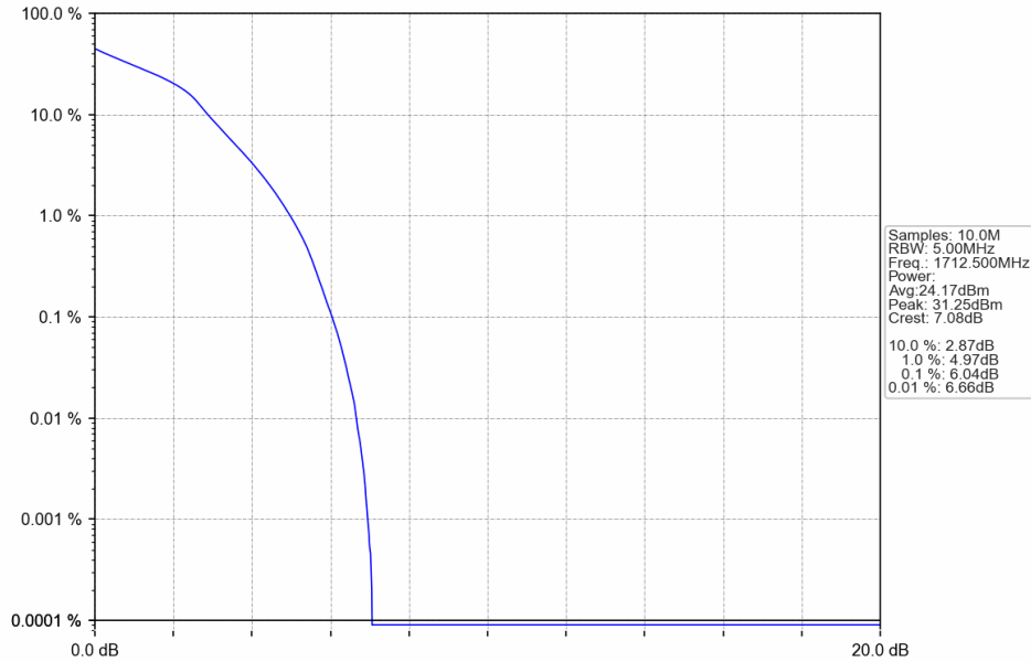
Band4_5MHz_16QAM_LCH_1712.5MHz_RB_25_0_NTNV
