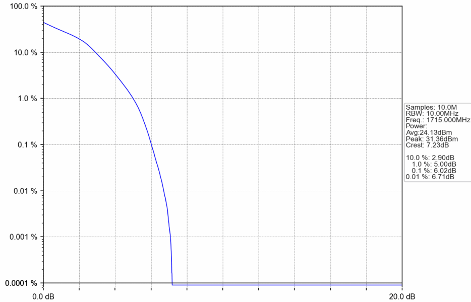
Band4_10MHz_16QAM_LCH_1715MHz_RB_50_0_NTNV
