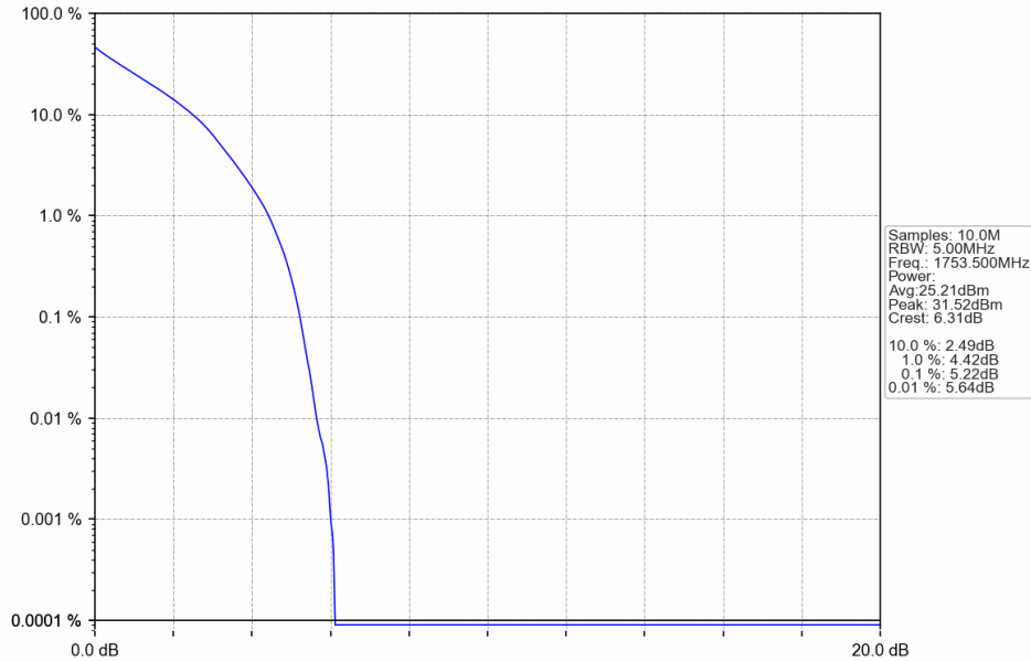
Band4_3MHz_QPSK_HCH_1753.5MHz_RB_15_0_NTNV
