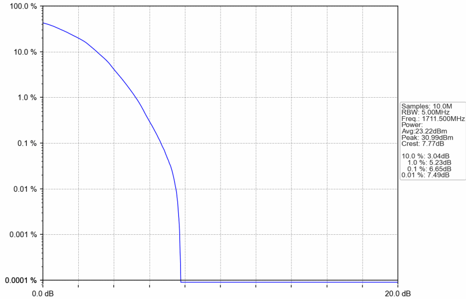
Band4_3MHz_64QAM_LCH_1711.5MHz_RB_15_0_NTNV
