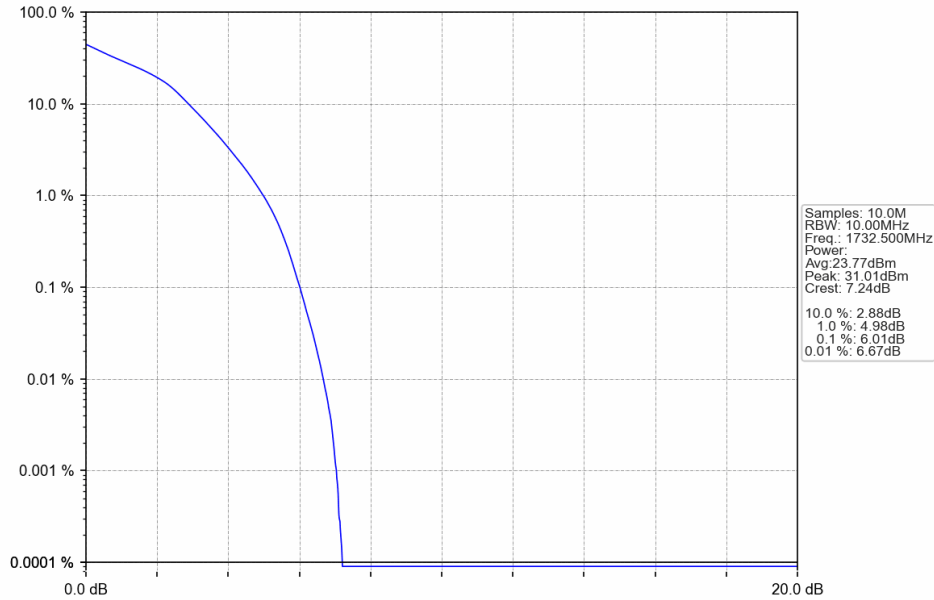
Band4_10MHz_16QAM_MCH_1732.5MHz_RB_50_0_NTNV
