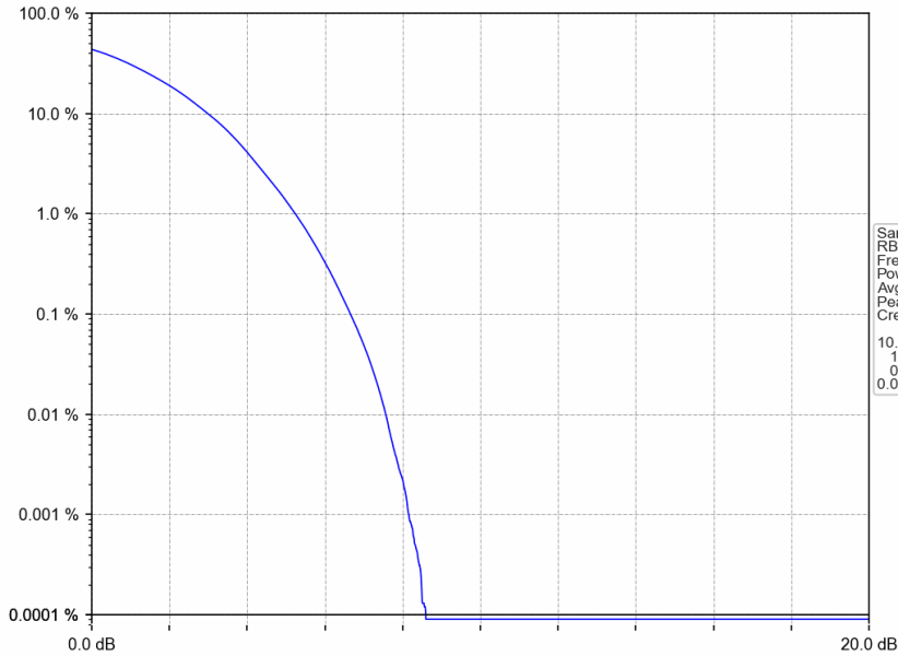
Band4_20MHz_64QAM_HCH_1745MHz_RB_100_0_NTNV
