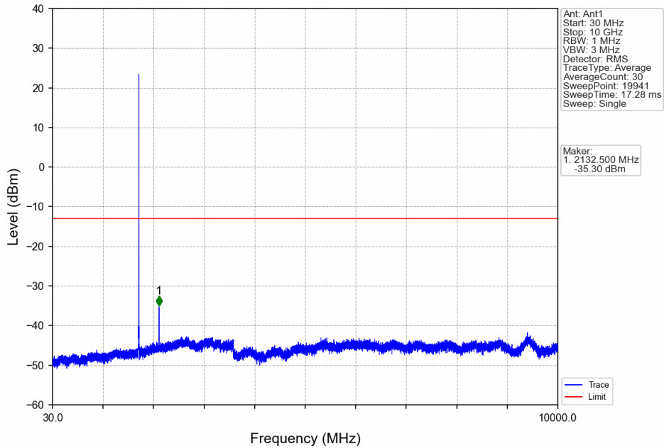
Band4_1.4MHz_16QAM_MCH_1732.5MHz_RB_1_0_NTNV
