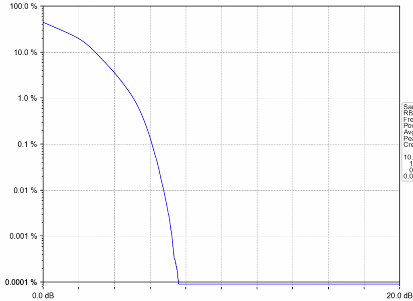
Band4_20MHz_16QAM_HCH_1745MHz_RB_100_0_NTNV
