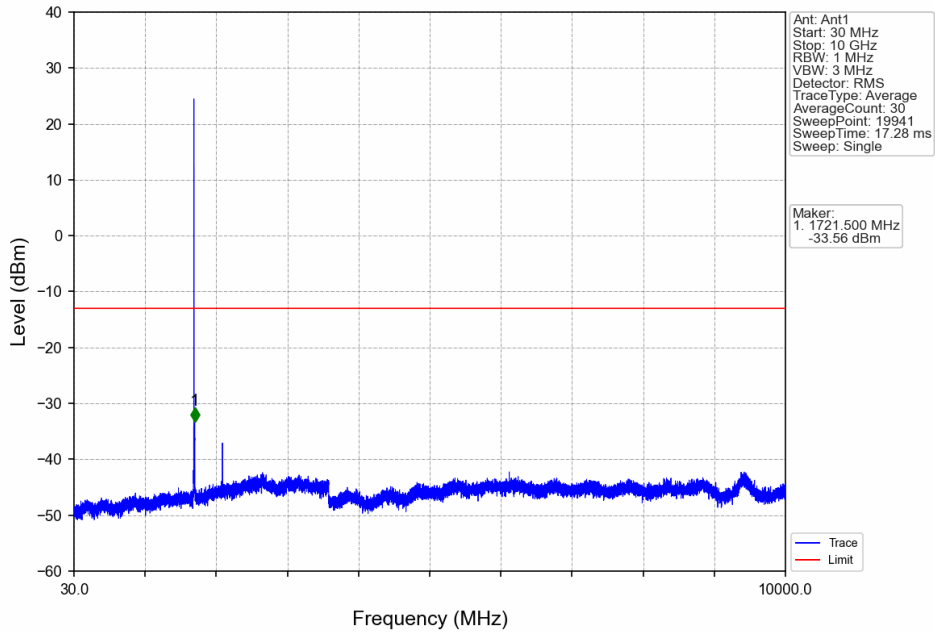
Band4_1.4MHz_16QAM_LCH_1710.7MHz_RB_1_0_NTNV
