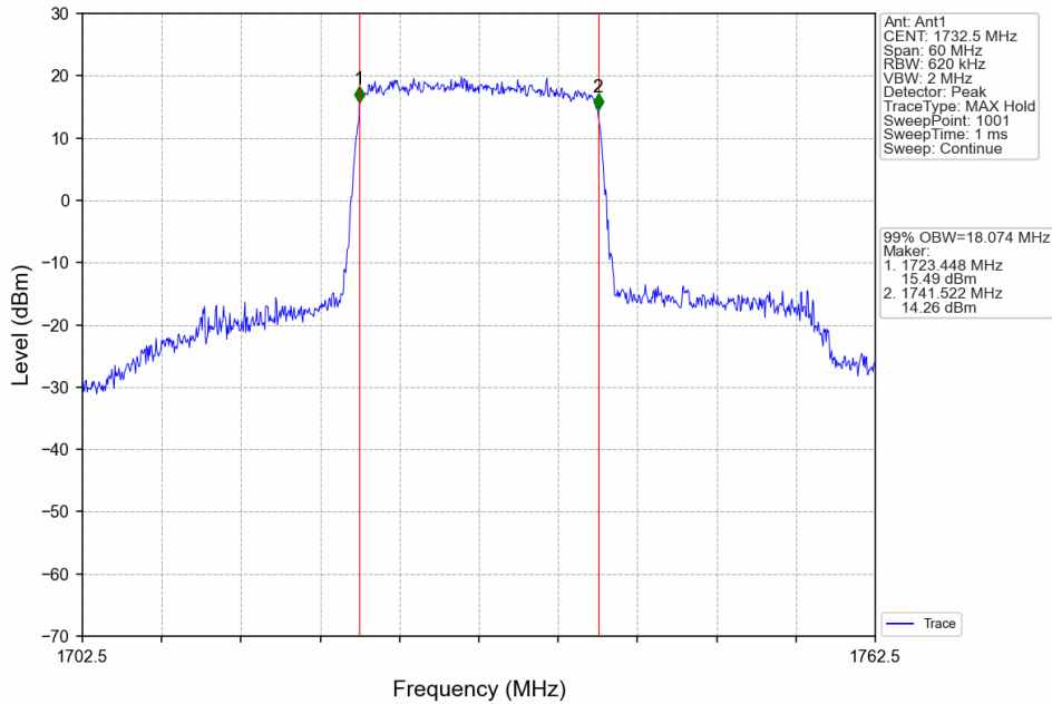
Band4_20MHz_64QAM_MCH_1732.5MHz_RB_100_0_NTNV
