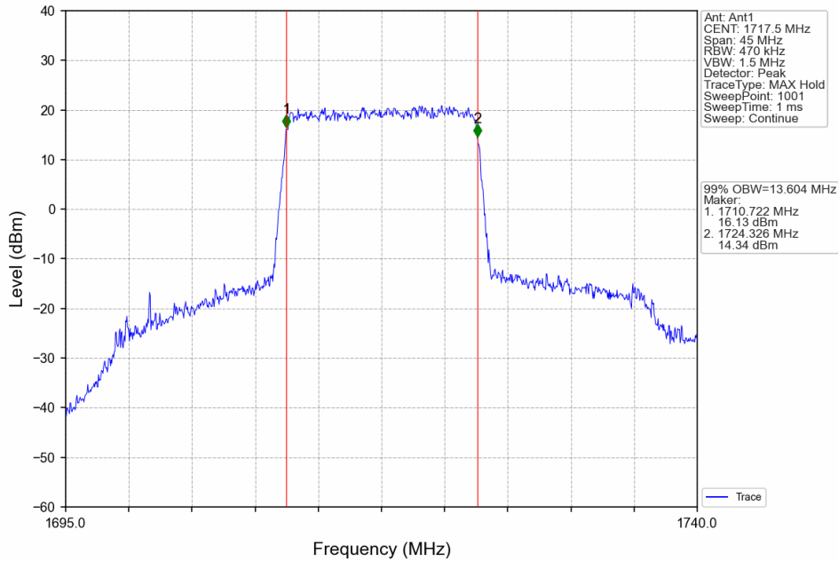
Band4_15MHz_16QAM_LCH_1717.5MHz_RB_75_0_NTNV
