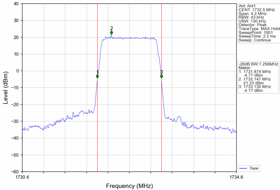
Band4_1.4MHz_16QAM_MCH_1732.5MHz_RB_6_0_NTNV
