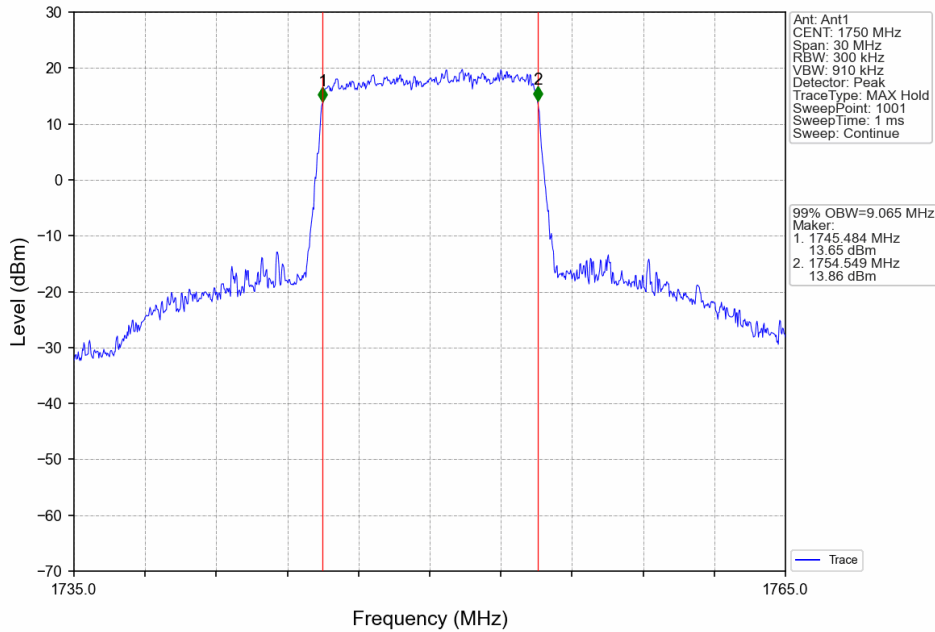
Band4_10MHz_64QAM_HCH_1750MHz_RB_50_0_NTNV
