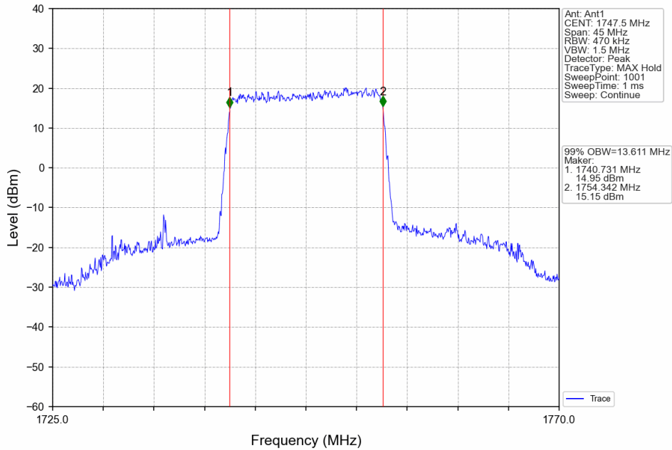
Band4_15MHz_64QAM_HCH_1747.5MHz_RB_75_0_NTNV
