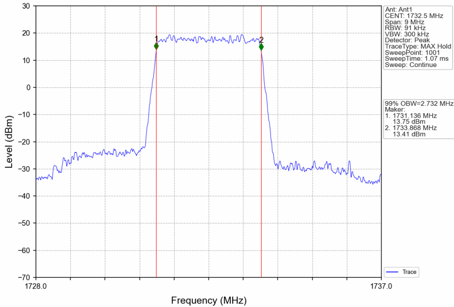
Band4_3MHz_64QAM_MCH_1732.5MHz_RB_15_0_NTNV
