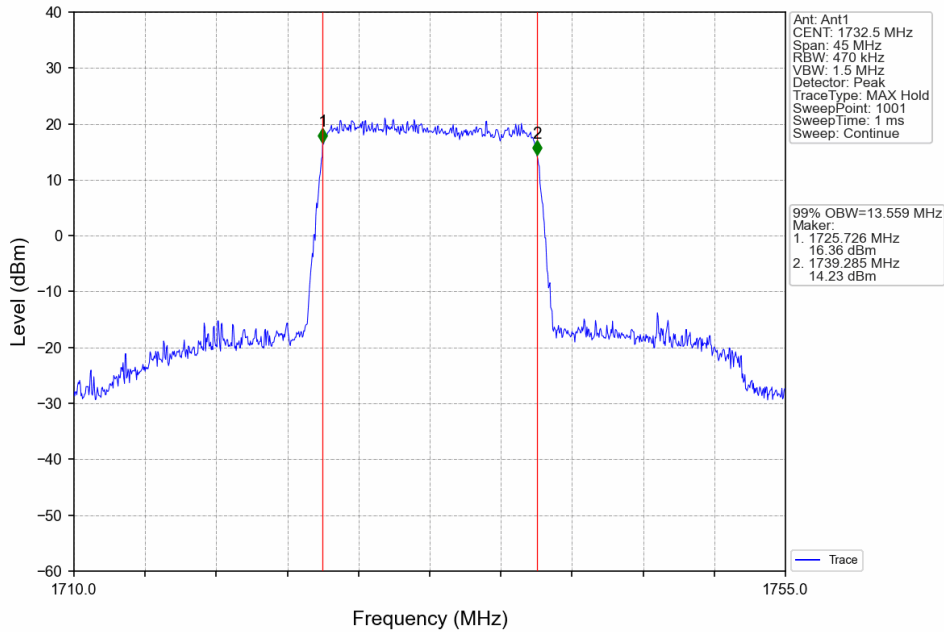
Band4_15MHz_16QAM_MCH_1732.5MHz_RB_75_0_NTNV
