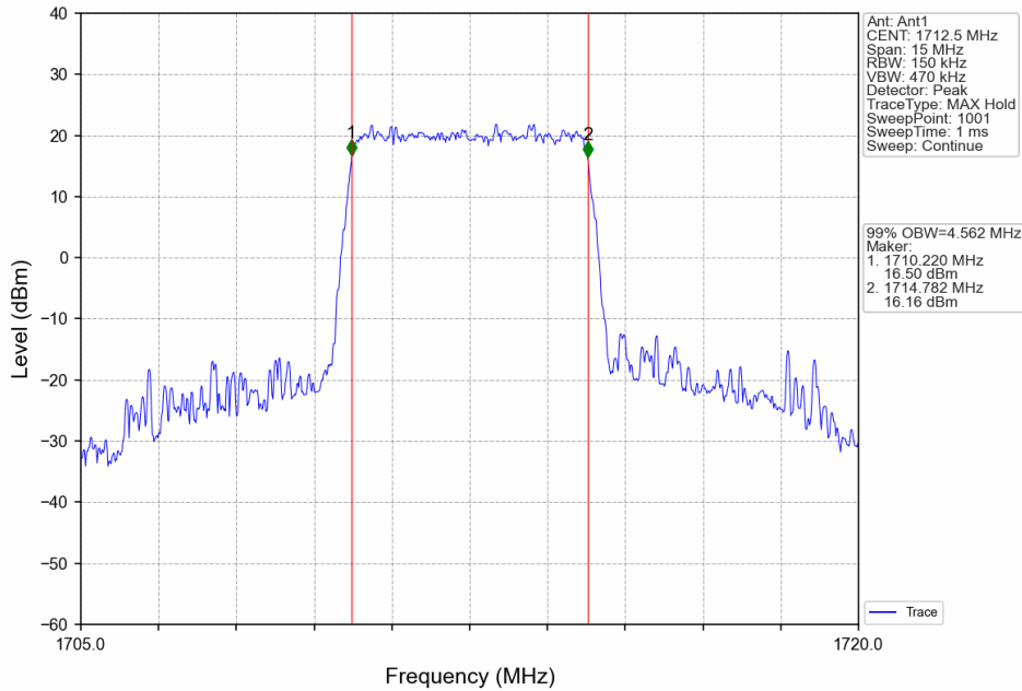
Band4_5MHz_QPSK_LCH_1712.5MHz_RB_25_0_NTNV
