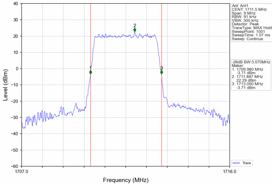
Band4_3MHz_QPSK_LCH_1711.5MHz_RB_15_0_NTNV
