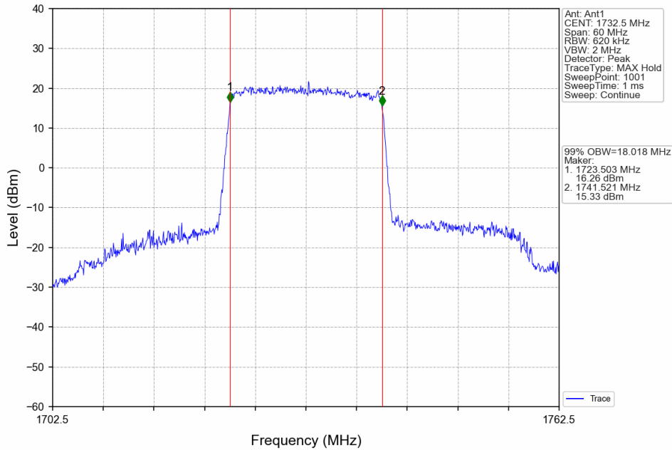
Band4_20MHz_16QAM_MCH_1732.5MHz_RB_100_0_NTNV
