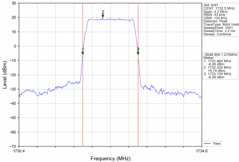
Band4_1.4MHz_64QAM_MCH_1732.5MHz_RB_6_0_NTNV
