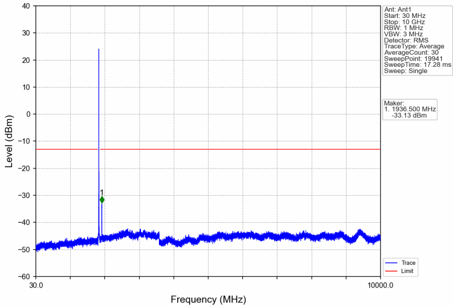
Band2_15MHz_64QAM_LCH_1857.5MHz_RB_1_0_NTNV
