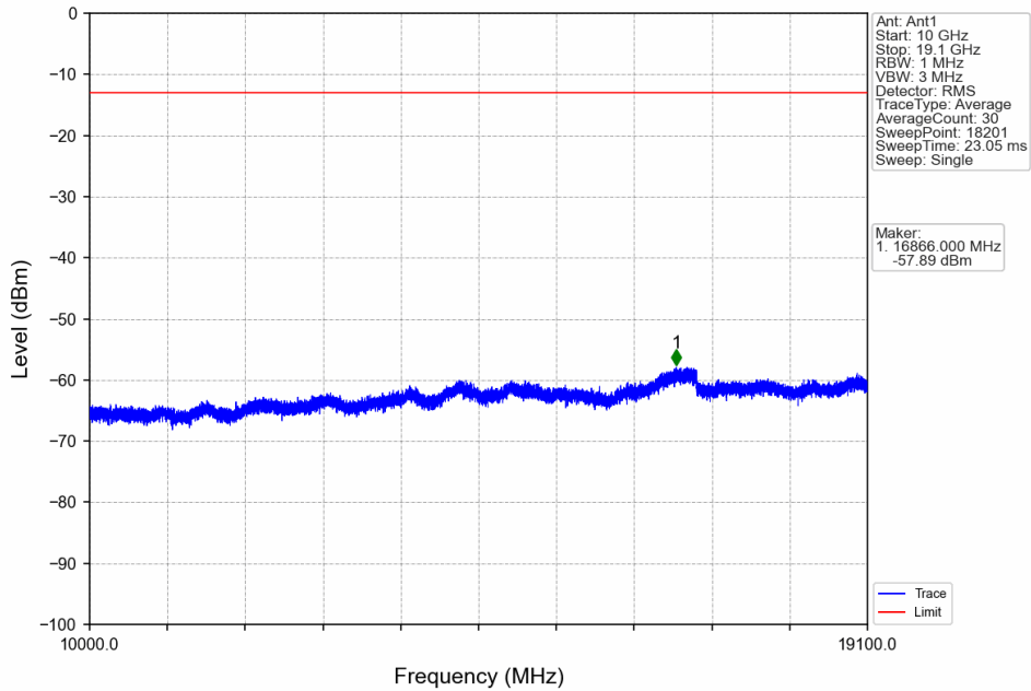
Band2_15MHz_64QAM_LCH_1857.5MHz_RB_1_0_NTNV
