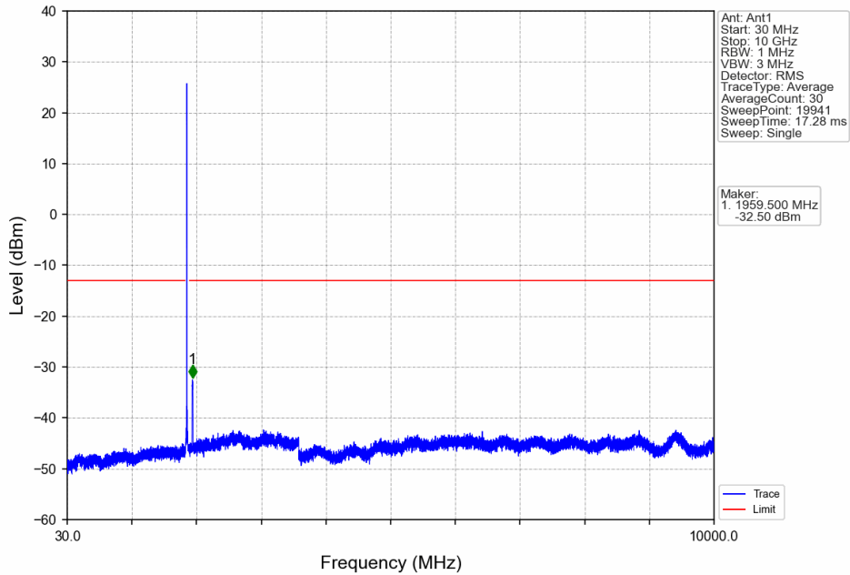
Band2_15MHz_16QAM_MCH_1880MHz_RB_1_0_NTNV
