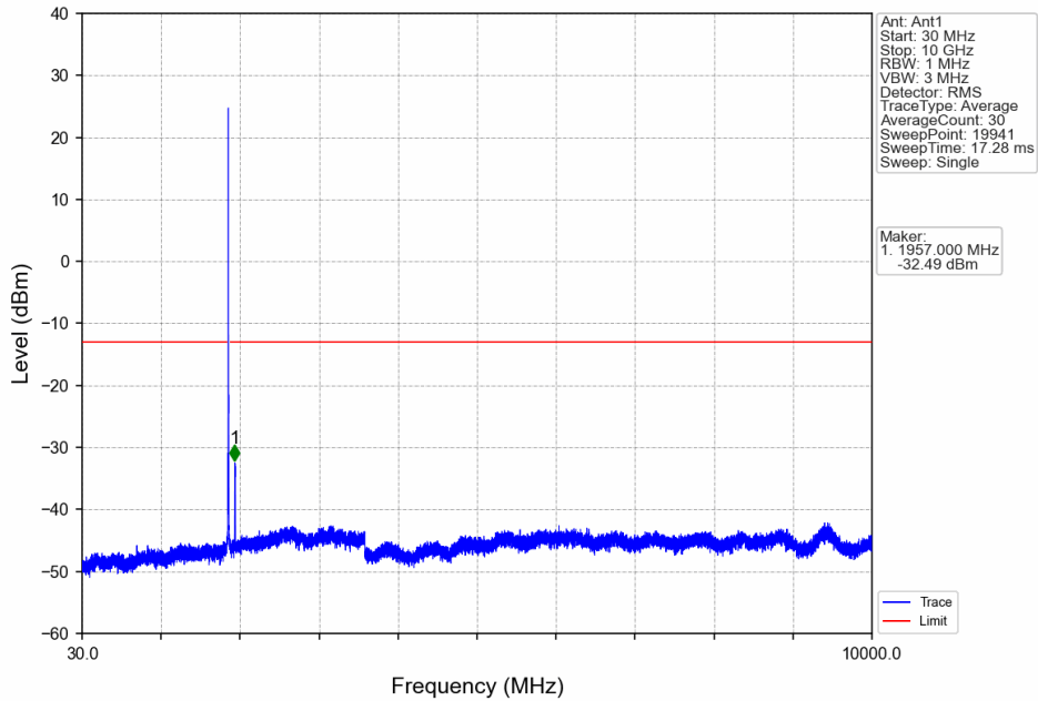
Band2_10MHz_64QAM_MCH_1880MHz_RB_1_0_NTNV
