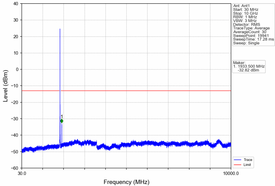
Band2_15MHz_16QAM_LCH_1857.5MHz_RB_1_0_NTNV
