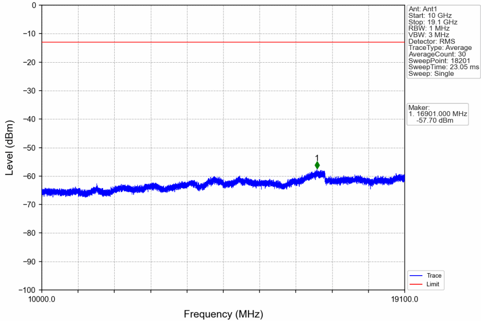
Band2_1.4MHz_64QAM_MCH_1880MHz_RB_1_0_NTNV
