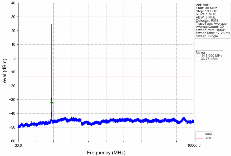
Band2_1.4MHz_64QAM_HCH_1909.3MHz_RB_1_0_NTNV
