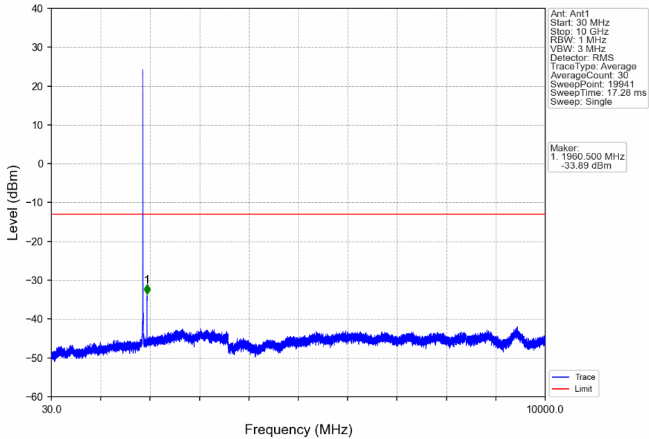
Band2_5MHz_16QAM_MCH_1880MHz_RB_1_0_NTNV
