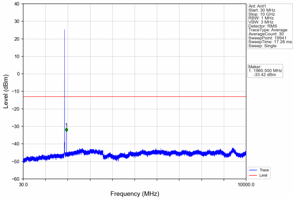
Band2_3MHz_64QAM_MCH_1880MHz_RB_1_0_NTNV
