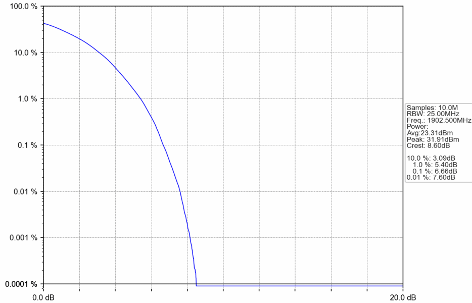
Band2_15MHz_64QAM_HCH_1902.5MHz_RB_75_0_NTNV
