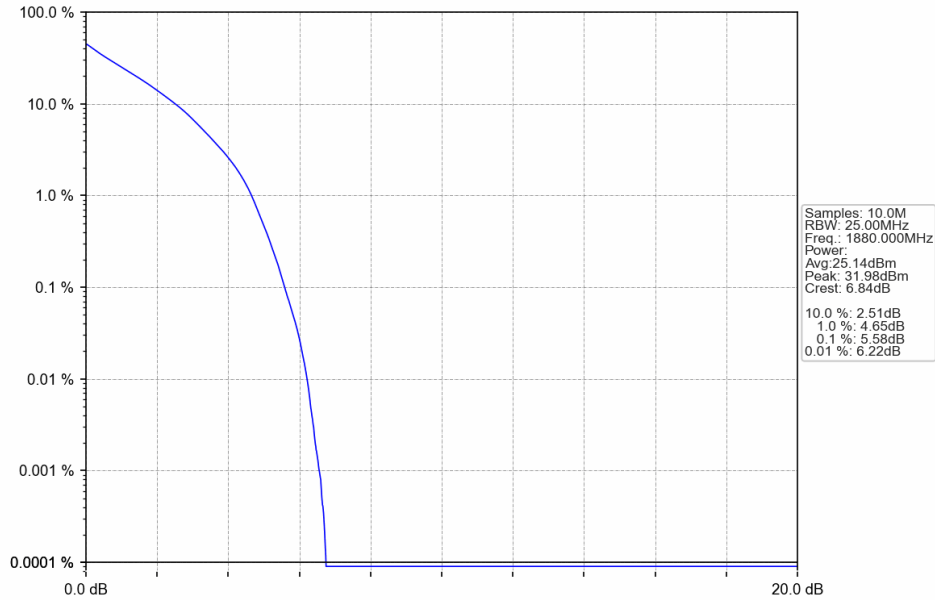
Band2_15MHz_QPSK_MCH_1880MHz_RB_75_0_NTNV
