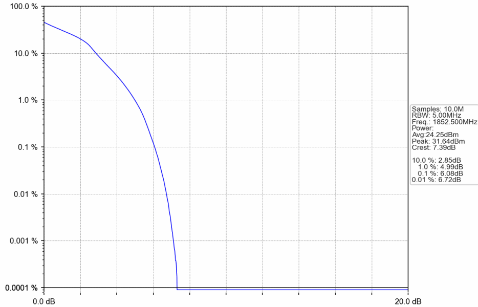
Band2_5MHz_16QAM_LCH_1852.5MHz_RB_25_0_NTNV
