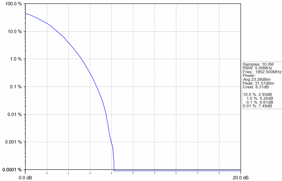
Band2_5MHz_64QAM_LCH_1852.5MHz_RB_25_0_NTNV
