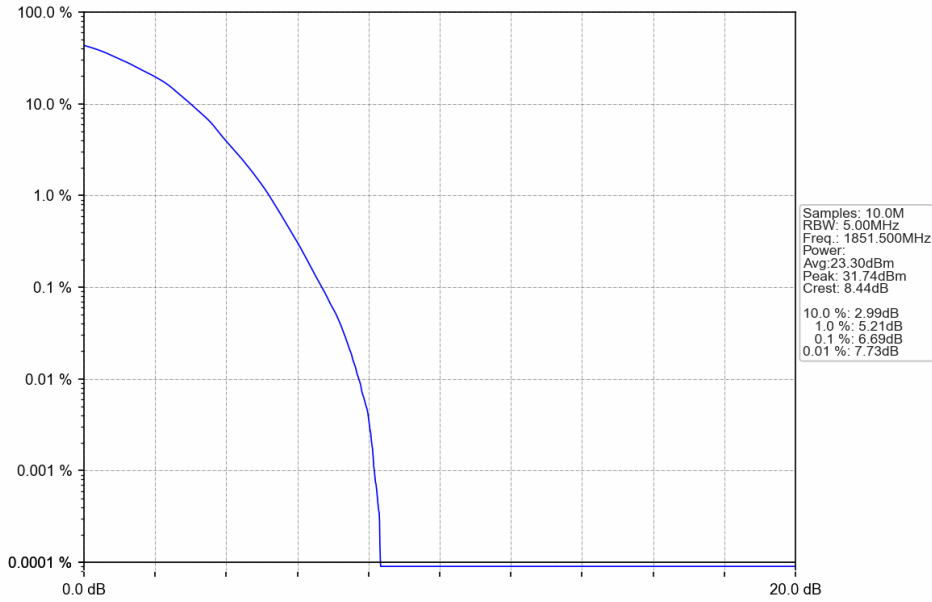
Band2_3MHz_64QAM_LCH_1851.5MHz_RB_15_0_NTNV
