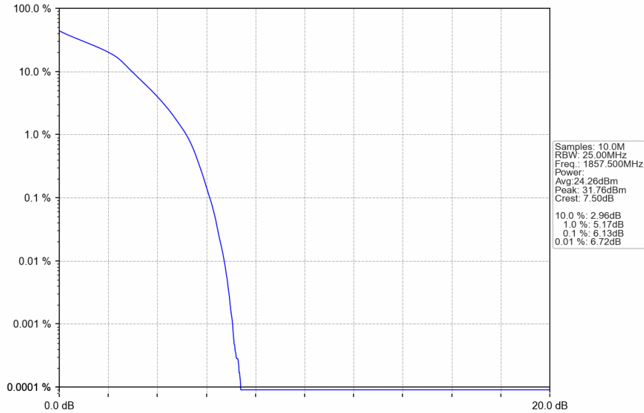
Band2_15MHz_16QAM_LCH_1857.5MHz_RB_75_0_NTNV
