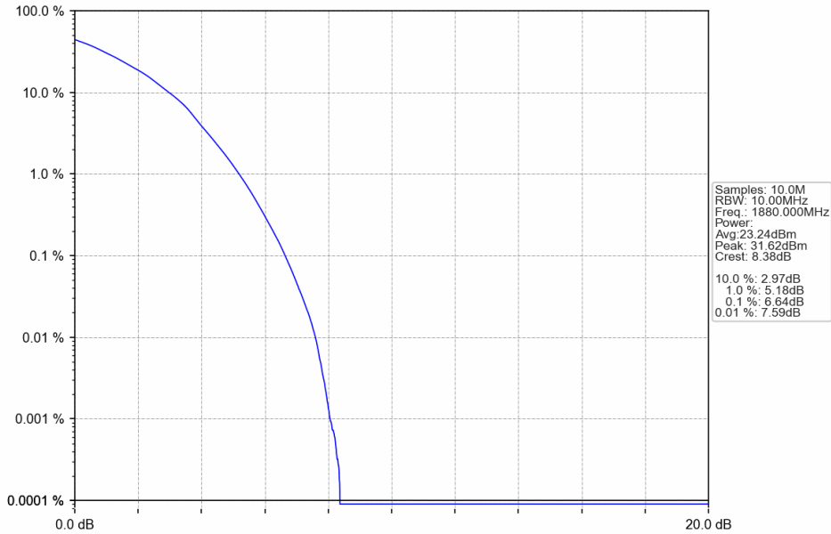
Band2_10MHz_64QAM_MCH_1880MHz_RB_50_0_NTNV
