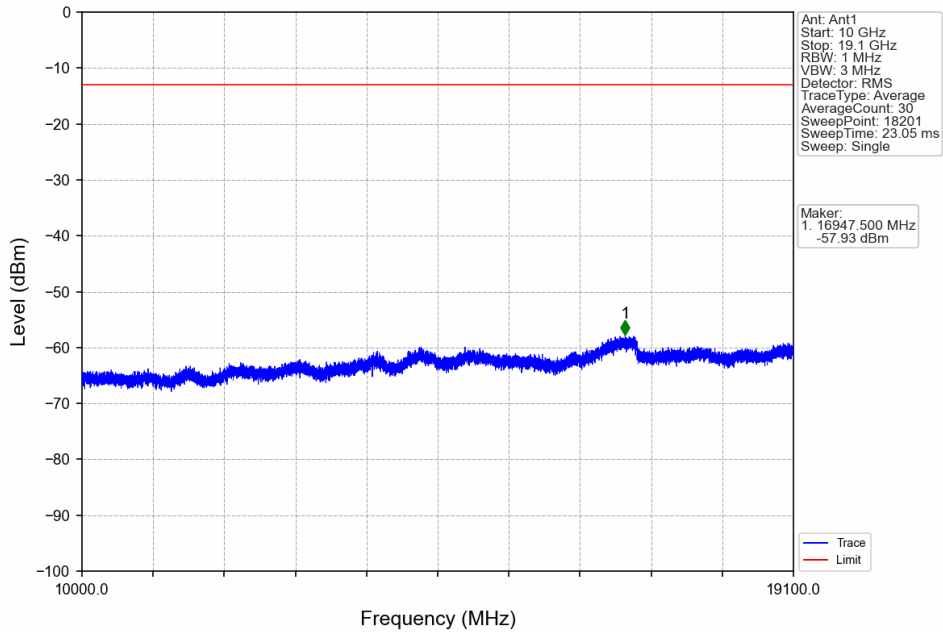
Band2_1.4MHz_16QAM_LCH_1850.7MHz_RB_1_0_NTNV
