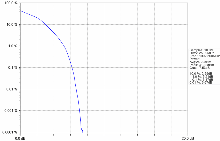
Band2_15MHz_16QAM_HCH_1902.5MHz_RB_75_0_NTNV
