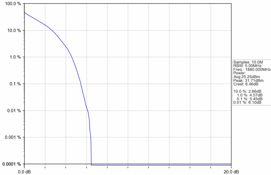
Band2_1.4MHz_QPSK_MCH_1880MHz_RB_6_0_NTNV
