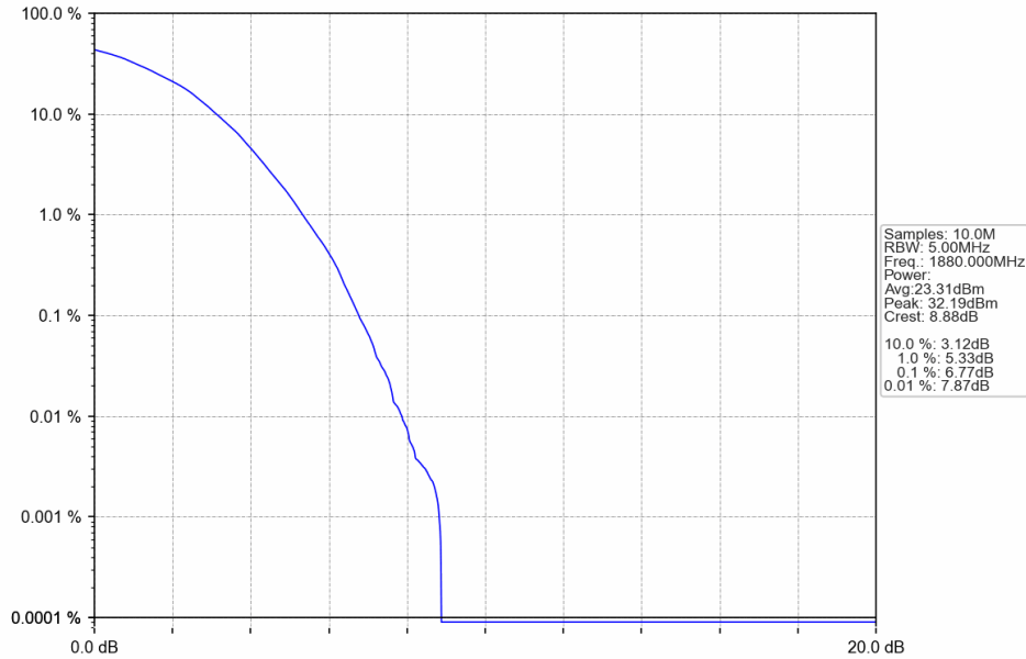
Band2_1.4MHz_64QAM_MCH_1880MHz_RB_6_0_NTNV
