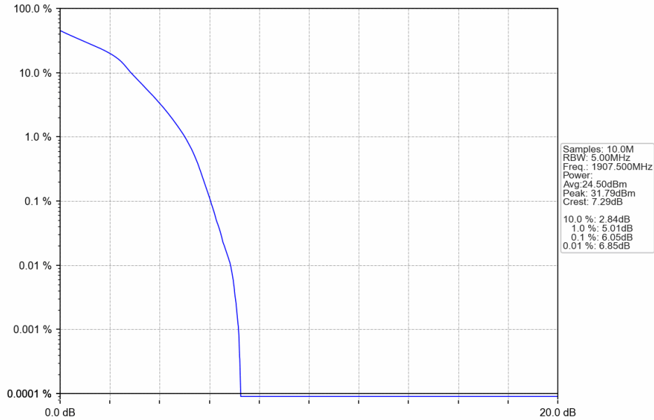
Band2_5MHz_16QAM_HCH_1907.5MHz_RB_25_0_NTNV
