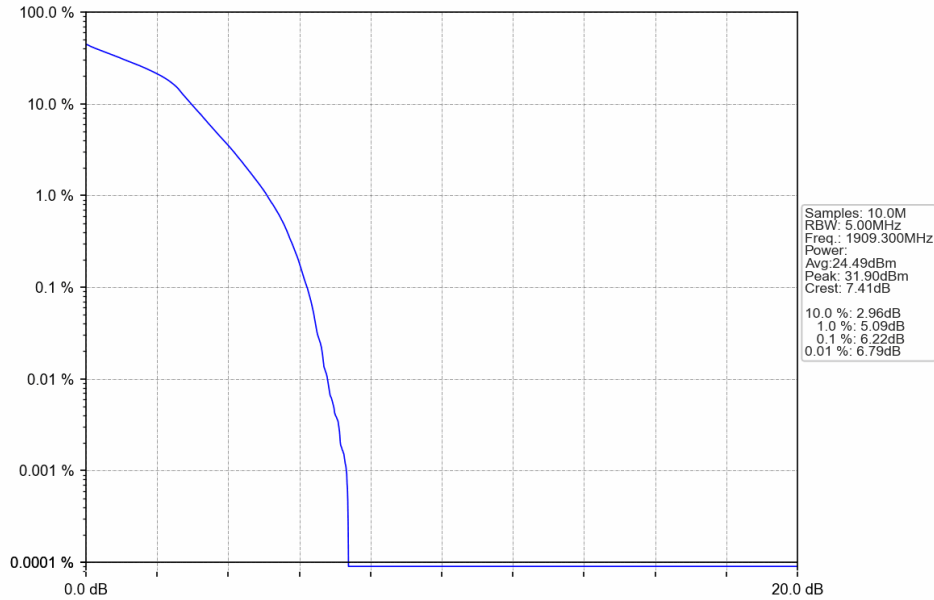
Band2_1.4MHz_16QAM_HCH_1909.3MHz_RB_6_0_NTNV
