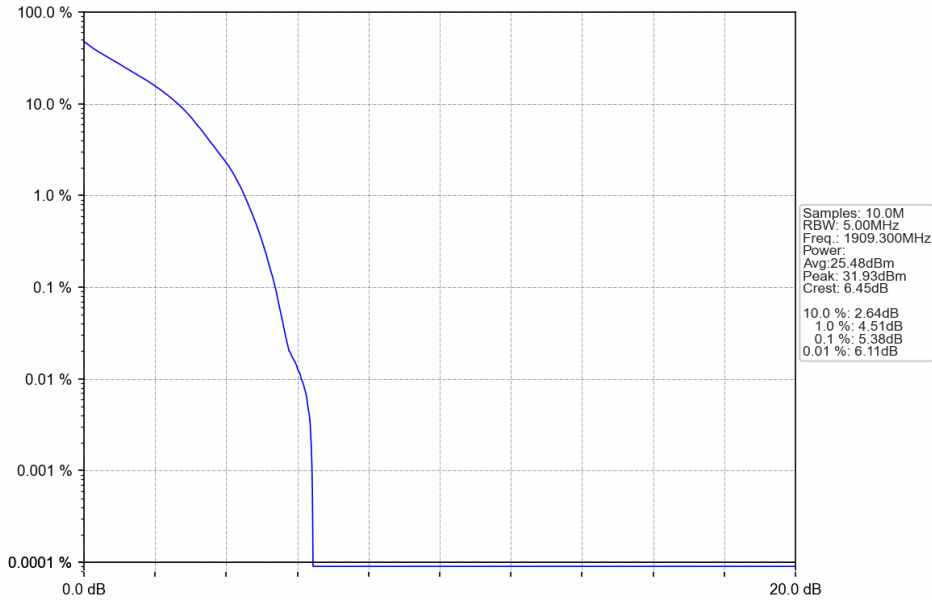
Band2_1.4MHz_QPSK_HCH_1909.3MHz_RB_6_0_NTNV
