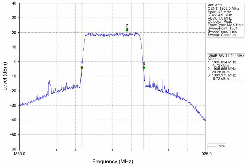
Band2_15MHz_64QAM_HCH_1902.5MHz_RB_75_0_NTNV
