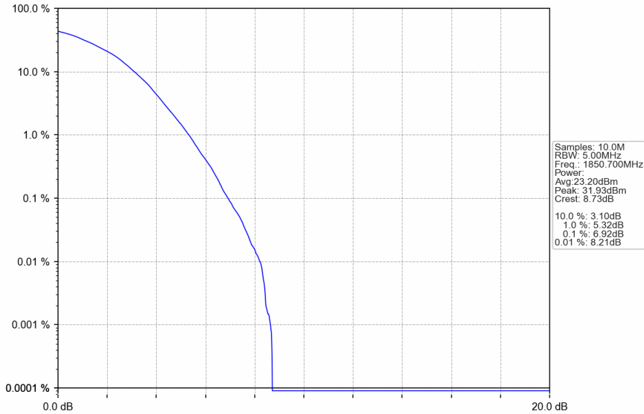
Band2_1.4MHz_64QAM_LCH_1850.7MHz_RB_6_0_NTNV
