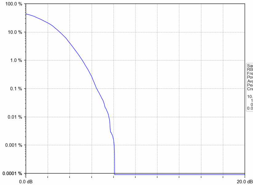
Band2_1.4MHz_64QAM_HCH_1909.3MHz_RB_6_0_NTNV
