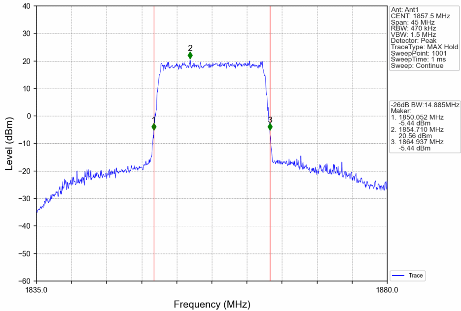
Band2_15MHz_64QAM_LCH_1857.5MHz_RB_75_0_NTNV
