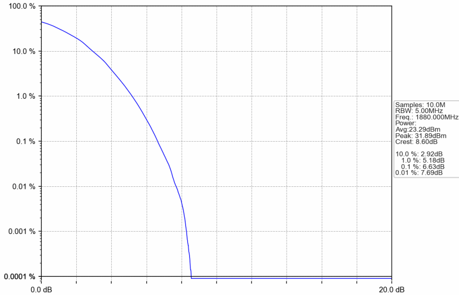
Band2_5MHz_64QAM_MCH_1880MHz_RB_25_0_NTNV
