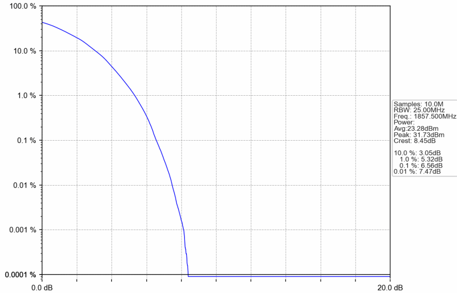
Band2_15MHz_64QAM_LCH_1857.5MHz_RB_75_0_NTNV
