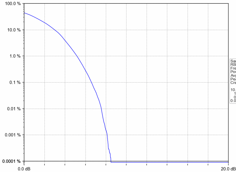
Band2_10MHz_64QAM_HCH_1905MHz_RB_50_0_NTNV
