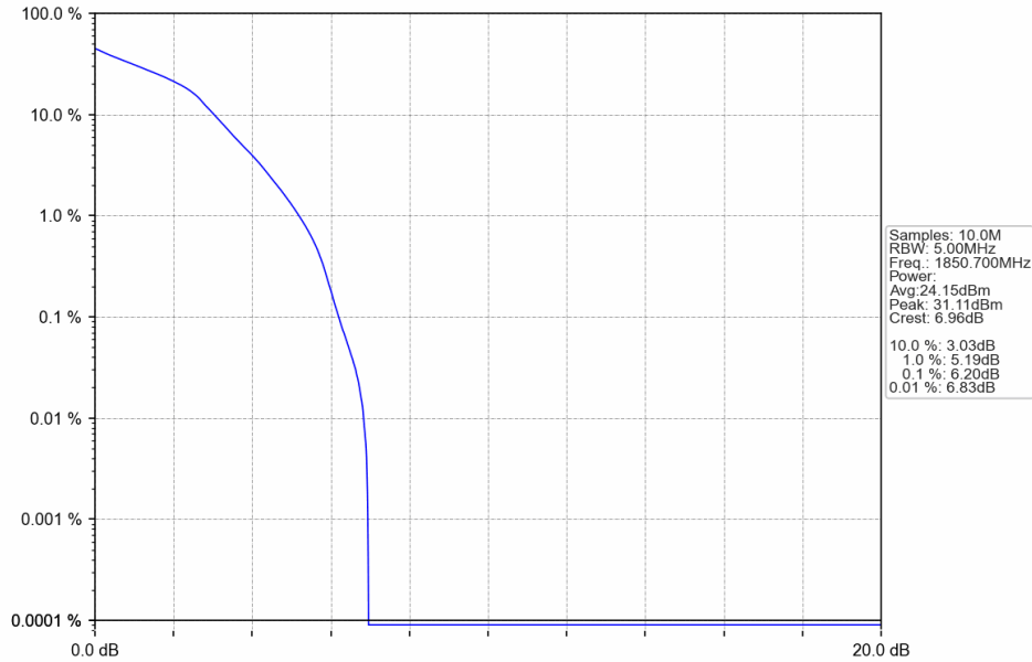
Band2_1.4MHz_16QAM_LCH_1850.7MHz_RB_6_0_NTNV
