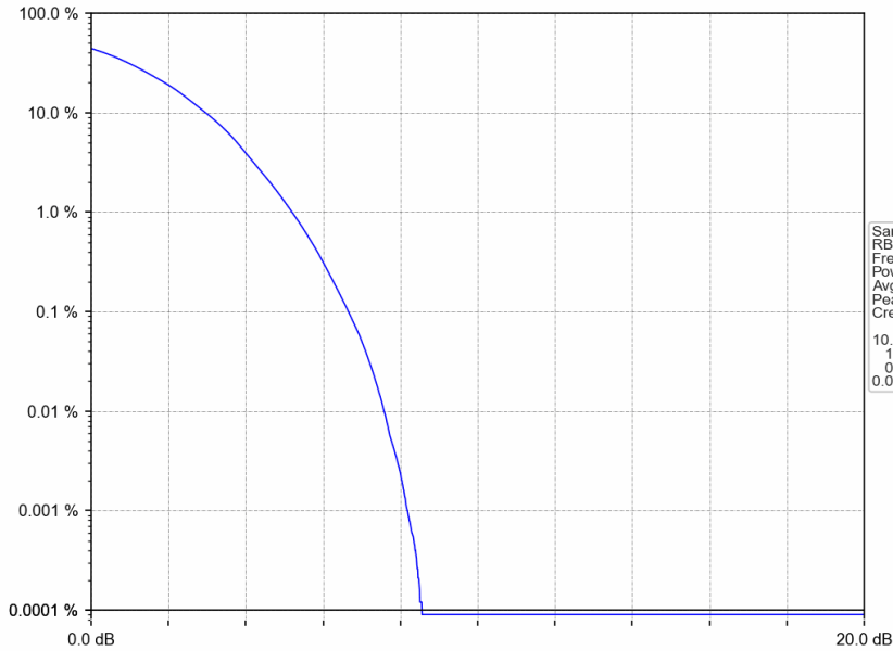
Band2_20MHz_64QAM_HCH_1900MHz_RB_100_0_NTNV
