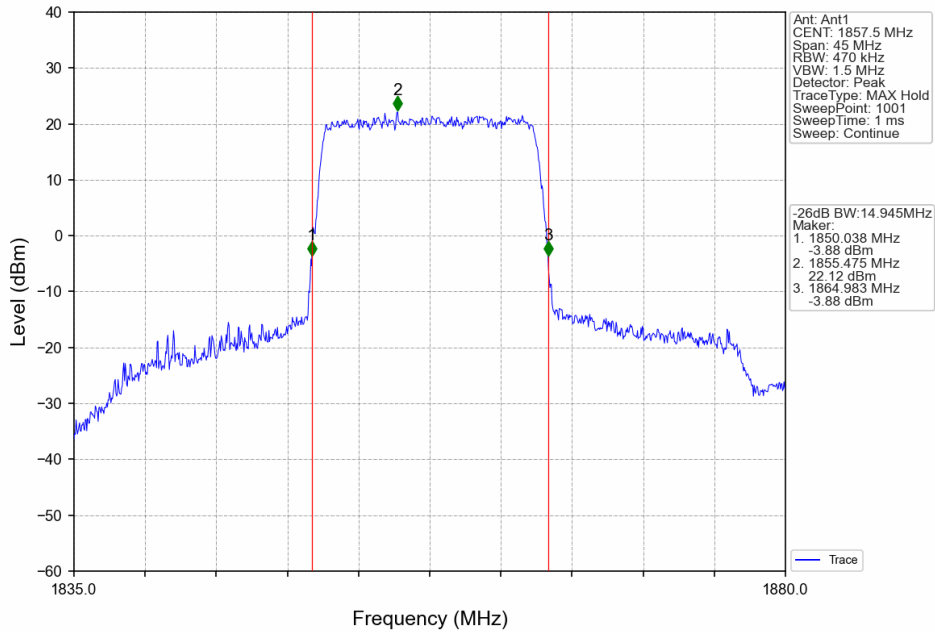
Band2_15MHz_QPSK_LCH_1857.5MHz_RB_75_0_NTNV
