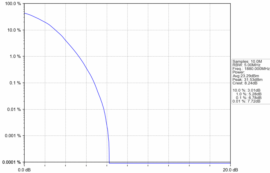
Band2_3MHz_64QAM_MCH_1880MHz_RB_15_0_NTNV
