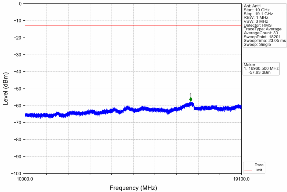
Band2_1.4MHz_16QAM_MCH_1880MHz_RB_1_0_NTNV
