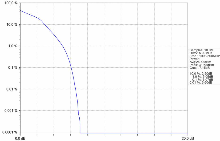
Band2_3MHz_16QAM_HCH_1908.5MHz_RB_15_0_NTNV
