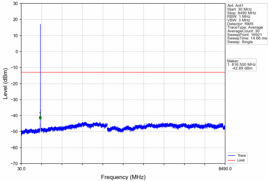
Band V_RMC_LCH_826.4MHz_12.2kbps RMC_NTNV
