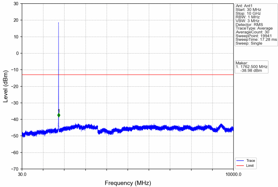
Band IV_RMC_HCH_1752.6MHz_12.2kbps RMC_NTNV
