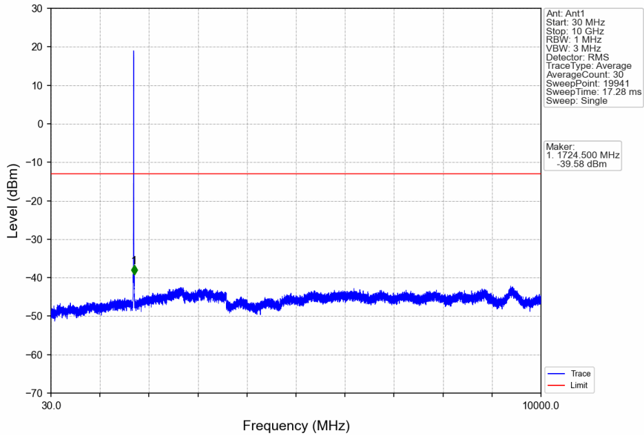
Band IV_RMC_LCH_1712.4MHz_12.2kbps RMC_NTNV
