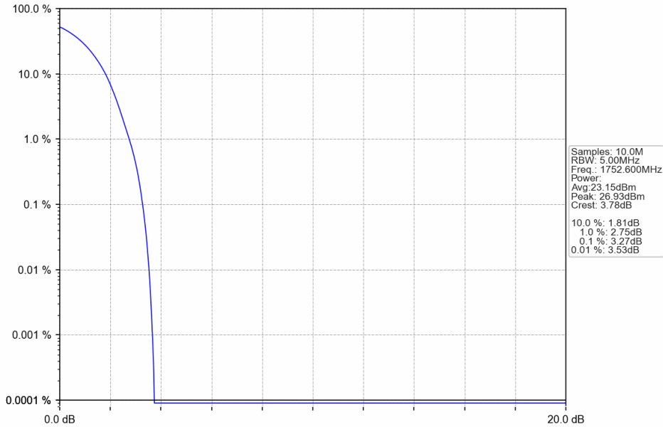
Band IV_RMC_HCH_1752.6MHz_12.2kbps RMC_NTNV
