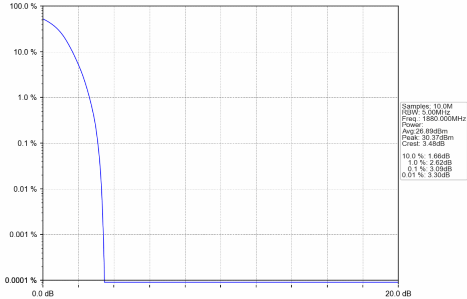
Band II_RMC_MCH_1880MHz_12.2kbps RMC_NTNV
