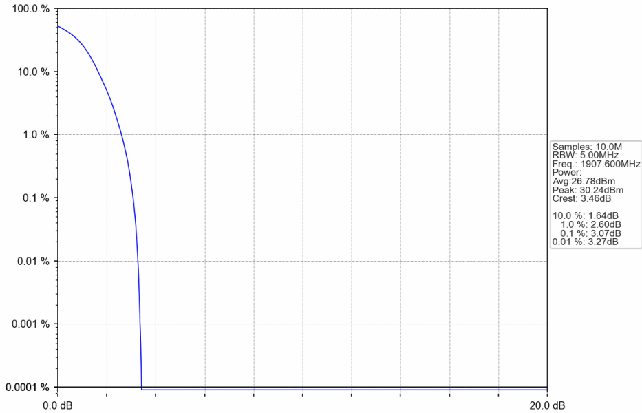
Band II_RMC_HCH_1907.6MHz_12.2kbps RMC_NTNV
