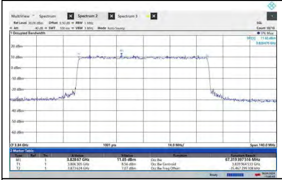
NTNV-N77-3700-3980-PC2-30-70-M-CP-QPSK-Outer Full-Ant2-PASS
