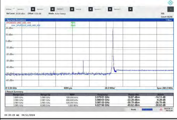
NTNV-N77-3700-3980-PC2-30-100-H-CP-QPSK-Edge 1RB Right-Ant1-PASS
