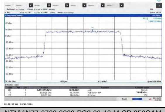
NTNV-N77-3700-3980-PC2-30-40-M-CP-256QAM-Outer Full-Ant2-PASS
