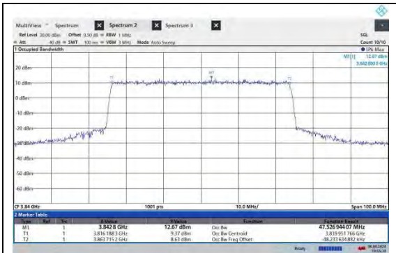
NTNV-N77-3700-3980-PC2-30-50-M-CP-64QAM-Outer Full-Ant2-PASS
