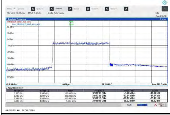
NTNV-N77-3700-3980-PC2-30-100-H-CP-QPSK-Outer Full-Ant1-PASS
