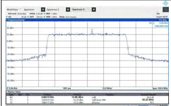
NTNV-N77-3700-3980-PC2-30-50-M-CP-64QAM-Outer_Full-Ant2-PASS
