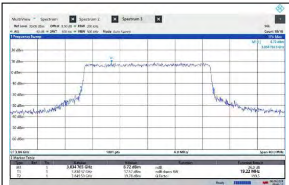
NTNV-N77-3700-3980-PC2-30-20-M-CP-QPSK-O
