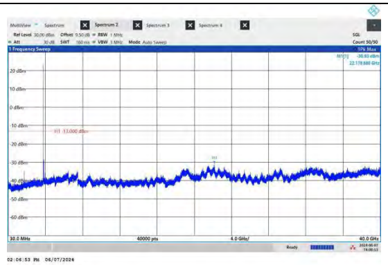
NTNV-N77-3700-3980-PC2-30-100-M-CP-QPSK-Edge_1RB_Left-Ant2-PASS
