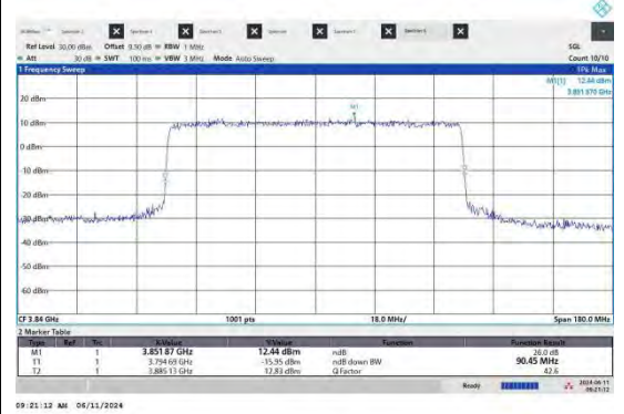
NTNV-N77-3700-3980-PC2-30-90-M-CP-16QAM-Outer Full-Ant2-PASS
