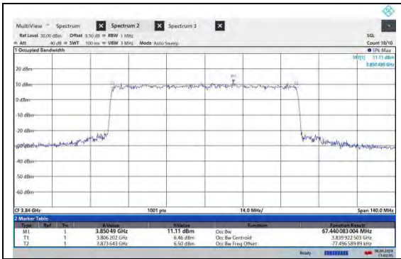
NTNV-N77-3700-3980-PC2-30-70-M-CP-64QAM-Outer_Full-Ant2-PASS
