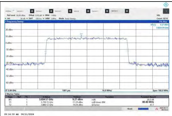
NTNV-N77-3700-3980-PC2-30-80-M-CP-256QAM-Outer Full-Ant2-PASS
