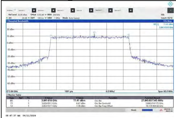
NTNV-N77-3700-3980-PC2-30-30-M-CP-64QAM-Outer Full-Ant2-PASS
