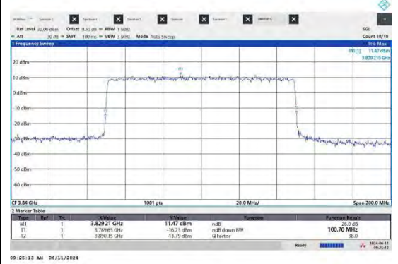
NTNV-N77-3700-3980-PC2-30-100-M-CP-16QAM-Outer Full-Ant2-PASS
