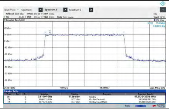
NTNV-N77-3700-3980-PC2-30-70-M-CP-16QAM-Outer Full-Ant2-PASS
