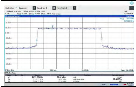
NTNV-N77-3700-3980-PC2-30-80-M-CP-64QAM-Outer_Full-Ant2-PASS
