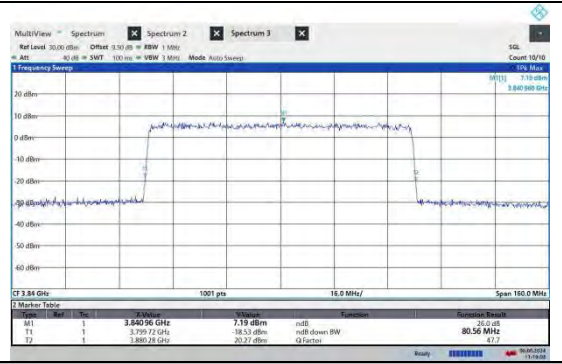
NTNV-N77-3700-3980-PC2-30-80-M-CP-256QAM-Outer_Full-Ant2-PASS
