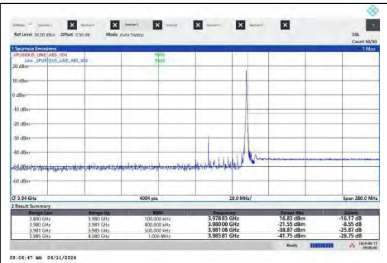
NTNV-N77-3700-3980-PC2-30-60-H-CP-QPSK-Edge 1RB Right-Ant1-PASS
