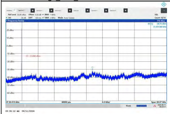
NTNV-N77-3700-3980-PC2-30-100-H-CP-QPSK-Edge_1RB_Left-Ant2-PASS
