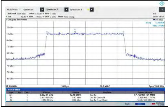
NTNV-N77-3700-3980-PC2-30-60-M-CP-QPSK-Outer Full-Ant2-PASS
