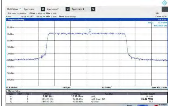
NTNV-N77-3700-3980-PC2-30-50-M-CP-QPSK-Outer_Full-Ant2-PASS
