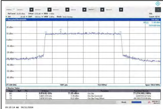
NTNV-N77-3700-3980-PC2-30-80-M-CP-64QAM-Outer Full-Ant2-PASS
