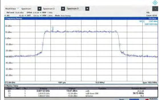
NTNV-N77-3700-3980-PC2-30-50-M-CP-16QAM-Outer_Full-Ant2-PASS
