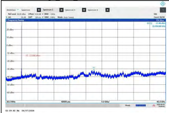
NTNV-N77-3700-3980-PC2-30-100-H-CP-QPSK-Edge_1RB_Left-Ant2-PASS
