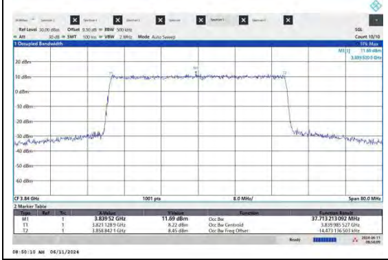
NTNV-N77-3700-3980-PC2-30-40-M-CP-QPSK-Outer Full-Ant2-PASS
