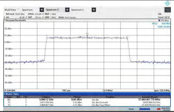
NTNV-N77-3700-3980-PC2-30-60-M-CP-256QAM-Outer Full-Ant2-PASS
