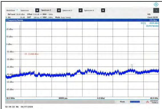
NTNV-N77-3700-3980-PC2-30-100-L-CP-QPSK-E_dge_1RB_Left-Ant2-PASS
