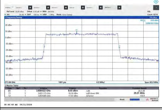
NTNV-N77-3700-3980-PC2-30-30-M-CP-256QAM-Outer Full-Ant2-PASS
