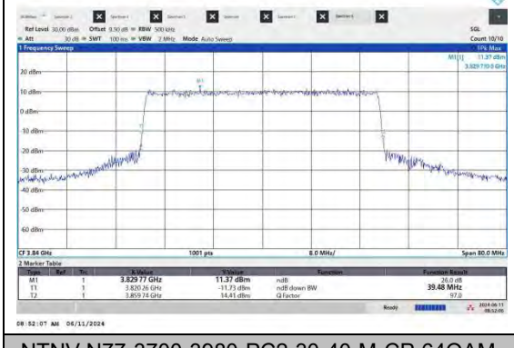
NTNV-N77-3700-3980-PC2-30-40-M-CP-64QAM-Outer Full-Ant2-PASS
