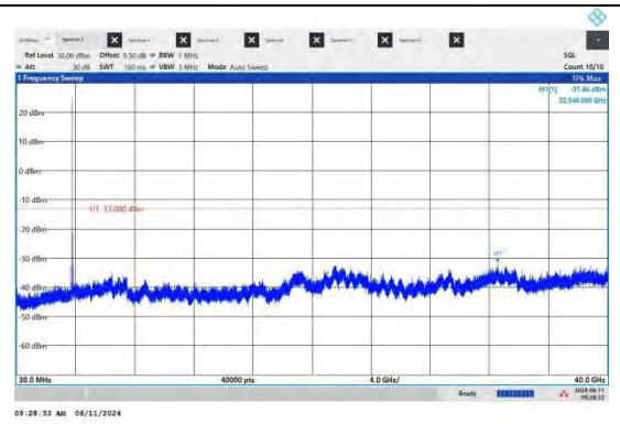
NTNV-N77-3700-3980-PC2-30-100-M-CP-QPSK-Edge_1RB_Left-Ant2-PASS
