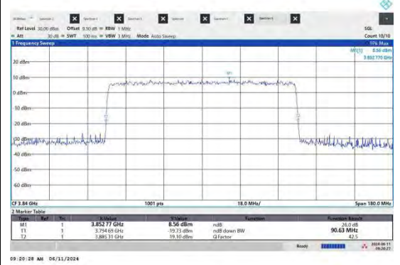
NTNV-N77-3700-3980-PC2-30-90-M-CP-256QAM-Outer Full-Ant2-PASS
