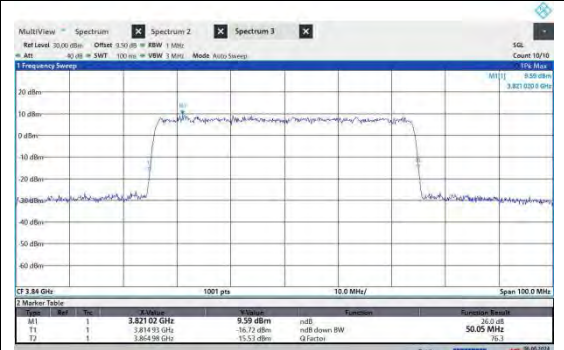
NTNV-N77-3700-3980-PC2-30-50-M-CP-256QAM-Outer_Full-Ant2-PASS
