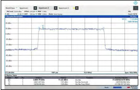
NTNV-N77-3700-3980-PC2-30-80-M-CP-QPSK-Outer_Full-Ant2-PASS
