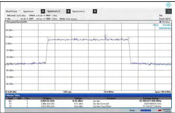
NTNV-N77-3700-3980-PC2-30-70-M-CP-256QAM-Outer_Full-Ant2-PASS
