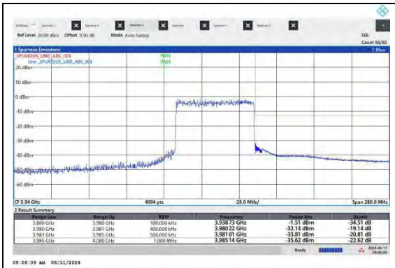
NTNV-N77-3700-3980-PC2-30-60-H-CP-QPSK-Outer Full-Ant1-PASS
