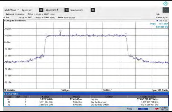
NTNV-N77-3700-3980-PC2-30-60-M-CP-16QAM-Outer Full-Ant2-PASS
