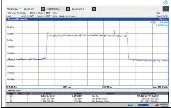
NTNV-N77-3700-3980-PC2-30-100-M-CP-64QAM-Outer_Full-Ant2-PASS
