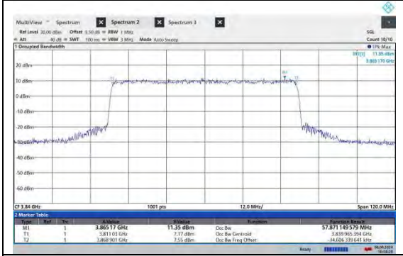
NTNV-N77-3700-3980-PC2-30-60-M-CP-64QAM-Outer Full-Ant2-PASS
