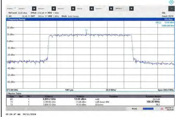
NTNV-N77-3700-3980-PC2-30-100-M-CP-QPSK-Outer Full-Ant2-PASS
