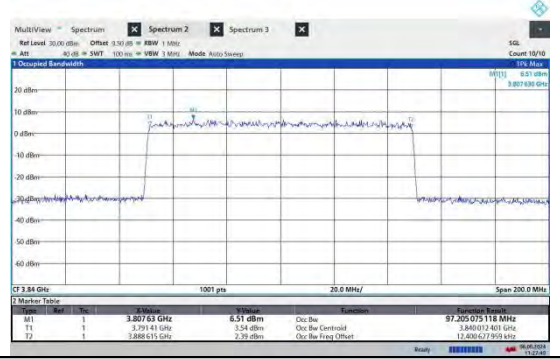
NTNV-N77-3700-3980-PC2-30-100-M-CP-256QAM-Outer_Full-Ant2-PASS
