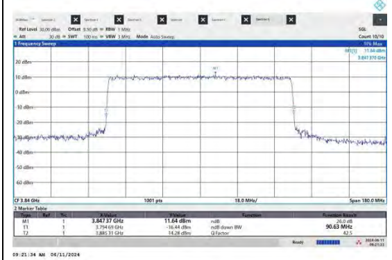
NTNV-N77-3700-3980-PC2-30-90-M-CP-QPSK-Outer Full-Ant2-PASS
