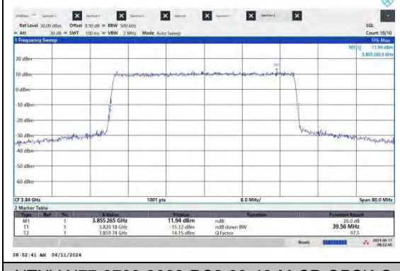
NTNV-N77-3700-3980-PC2-30-40-M-CP-QPSK-Outer Full-Ant2-PASS
