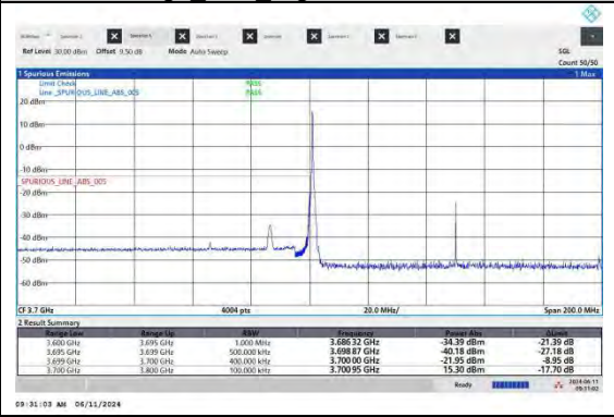
NTNV-N77-3700-3980-PC2-30-100-L-CP-QPSK-Edge 1RB Left-Ant1-PASS
