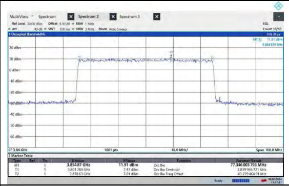
NTNV-N77-3700-3980-PC2-30-80-M-CP-16QAM-Outer_Full-Ant2-PASS
