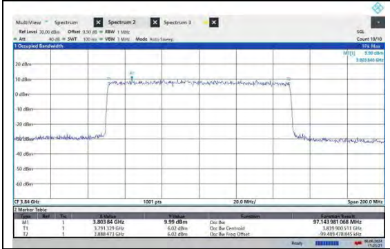
NTNV-N77-3700-3980-PC2-30-100-M-CP-QPSK-Outer_Full-Ant2-PASS
