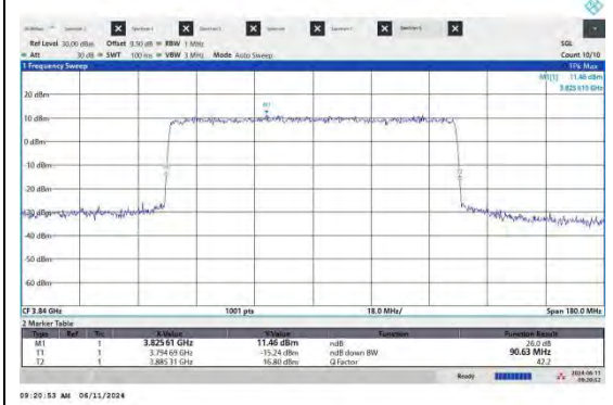
NTNV-N77-3700-3980-PC2-30-90-M-CP-64QAM-Outer Full-Ant2-PASS
