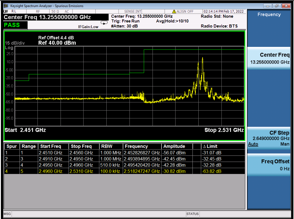
Band 41C 16QAM LCH 20M+15M RB FULL 0 NTN
