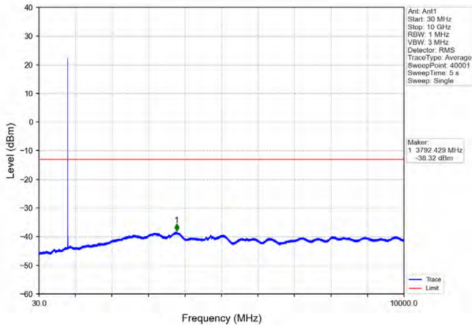
Band26_5MHz_64QAM_LCH_816.5MHz_RB_1_0_NTNV
