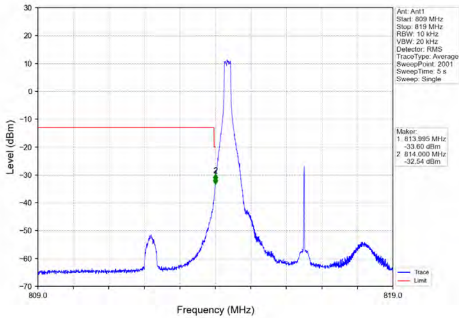
Band26_5MHz_64QAM_LCH_816.5MHz_RB_1_0_NTNV
