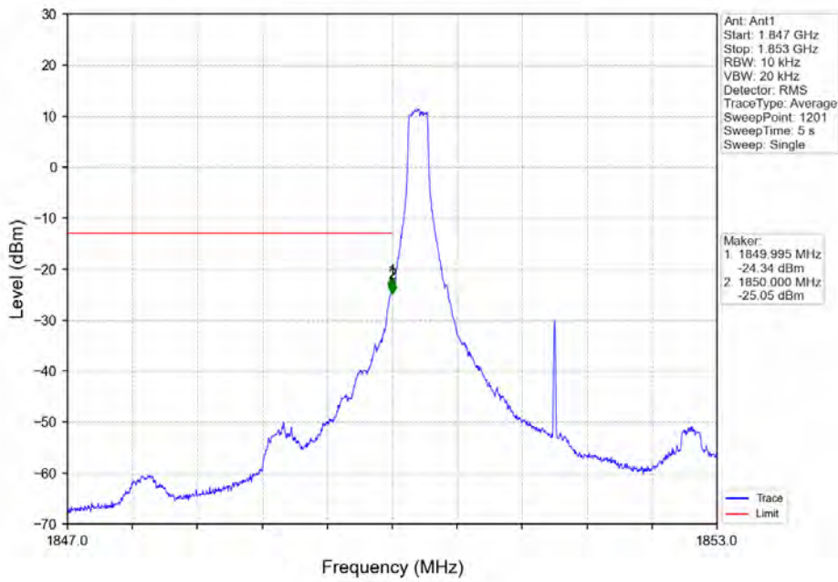
Band 2 3MHz QPSK LCH 1851.5MHz RB 1_0 NTV
