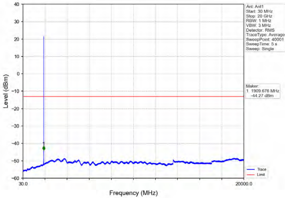
Band 25 1.4MHz 64QAM HCH 1914.3MHz RB 1 5 NTNV
