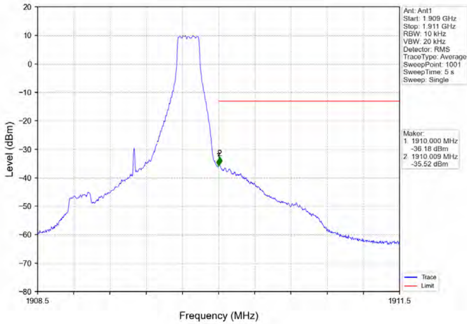
Band 2 1.4MHz 16QAM HCH 1909.3MHz RB 6 0 NTN
