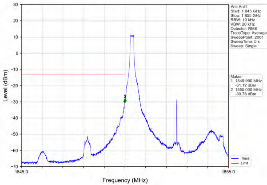
Band 2 5MHz QPSK LCH 1852.5MHz RB 1 0 NTV
