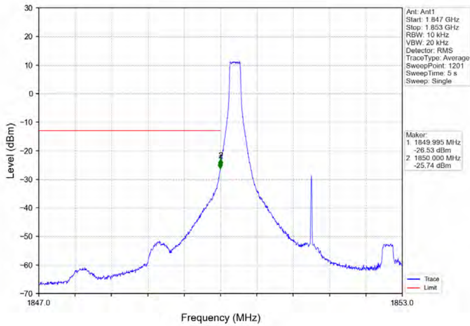
Band 25 3MHz 64QAM LCH 1851.5MHz RB 1 0 NTN
