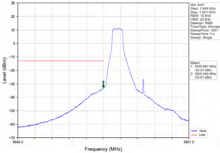
Band_25_1.4MHz_64QAM_LCH_1850.7MHz_RB_1_0_NTNV
