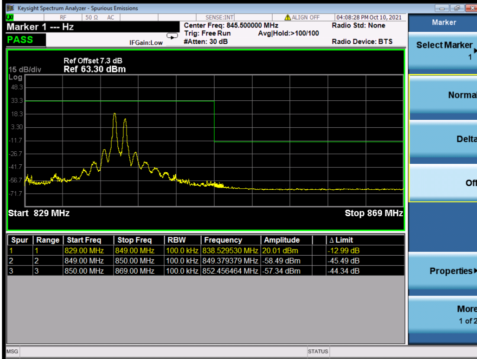
Band 5B 64QAM HCH 10M+10M RB FULL 0 NTN
