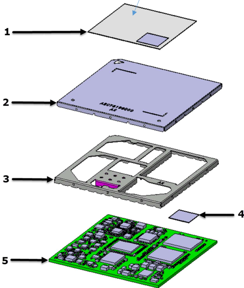
Figure 2: Module Exploded View
