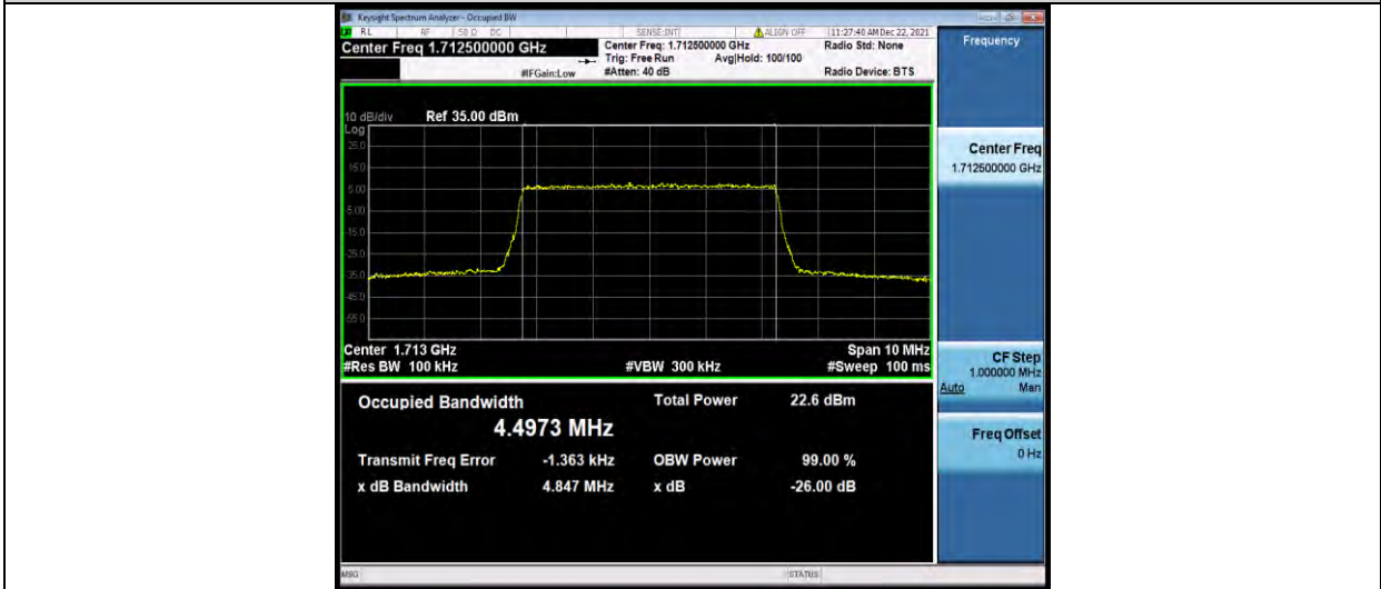
Band4-5MHz-16QAM-20175-25RB#0
