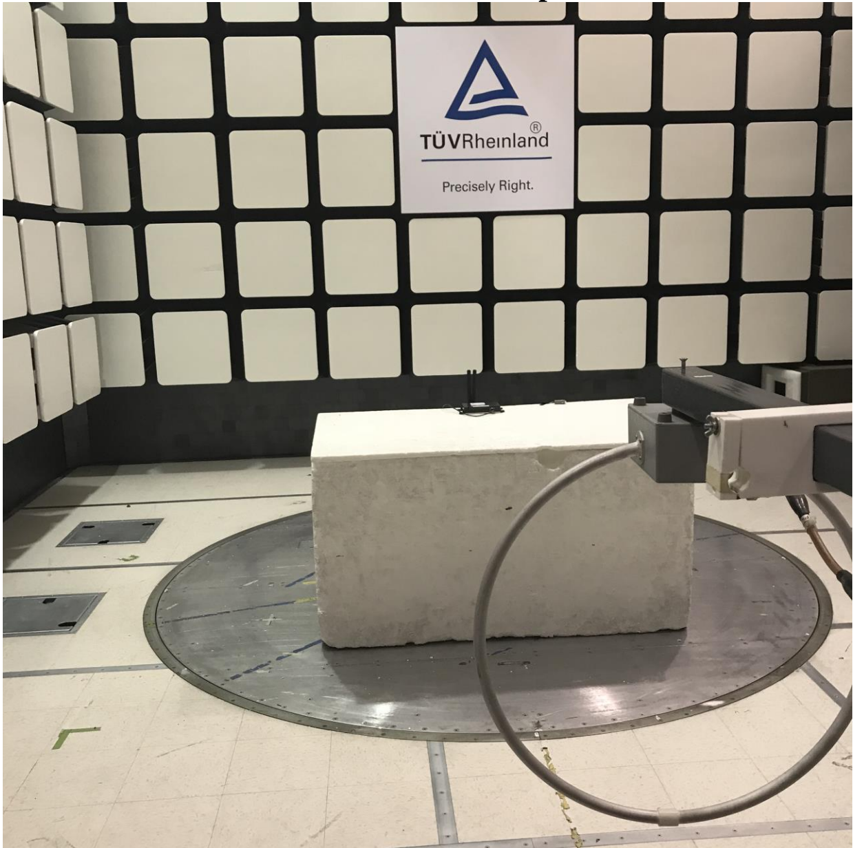
Figure 1: Test Setup for Radiated Emissions 9 kHz to 30 MHz - Front
