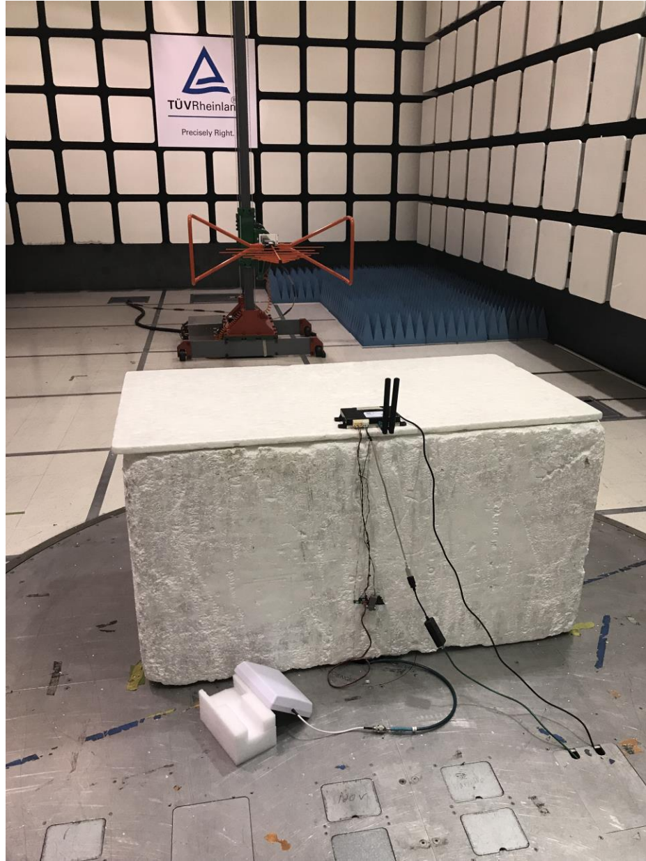
Figure 2: Test Setup for Radiated Emissions 30 MHz to 1000 MHz - Rear
