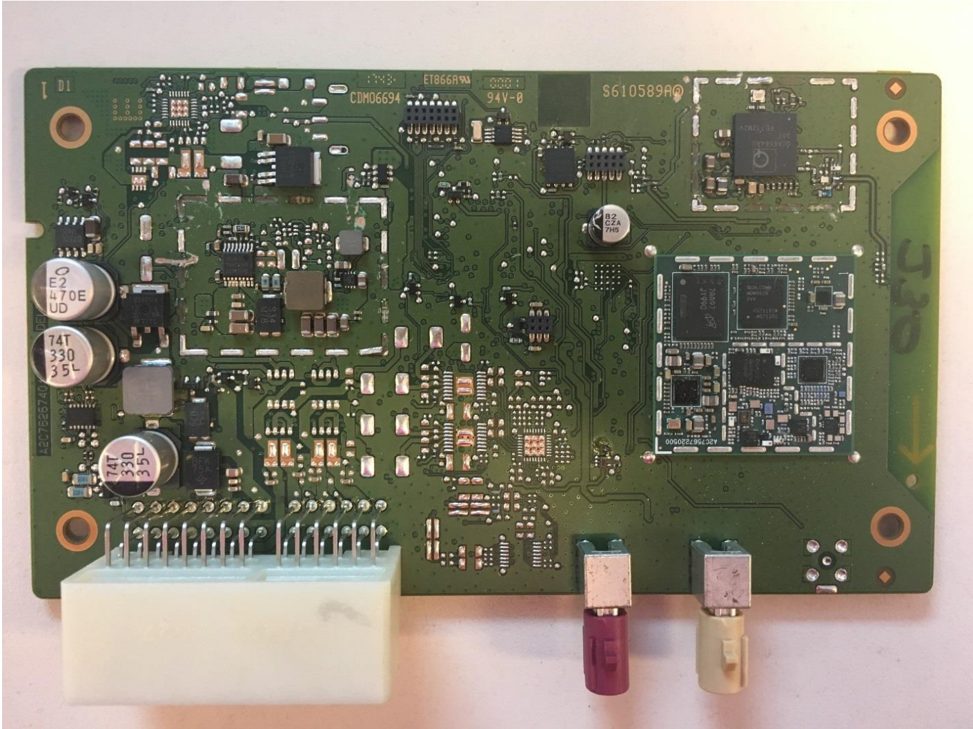
Fig. 4. FB40-ND1 Main pcb side 2 without shields.
