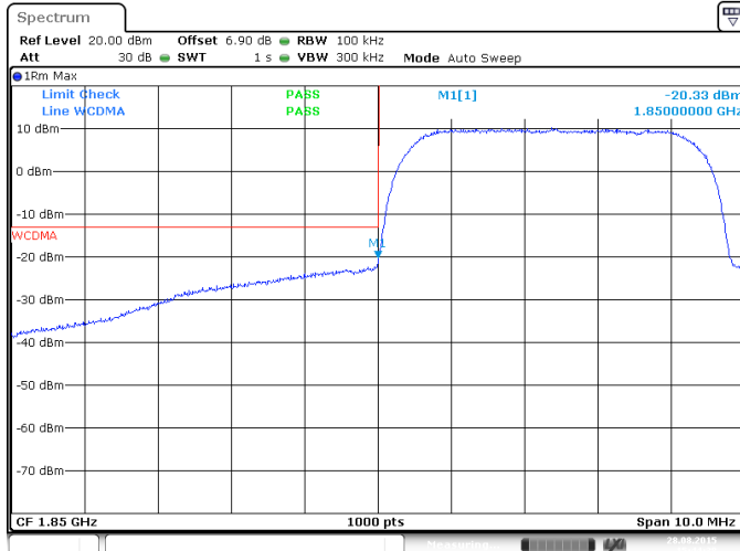
Lower Band Edge (Channel 9262, 1852.4 MHz)
