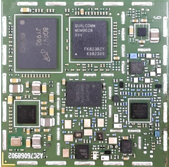
Fig. 3. BL28RW-001 module top view with the shield and shield frame removed.
