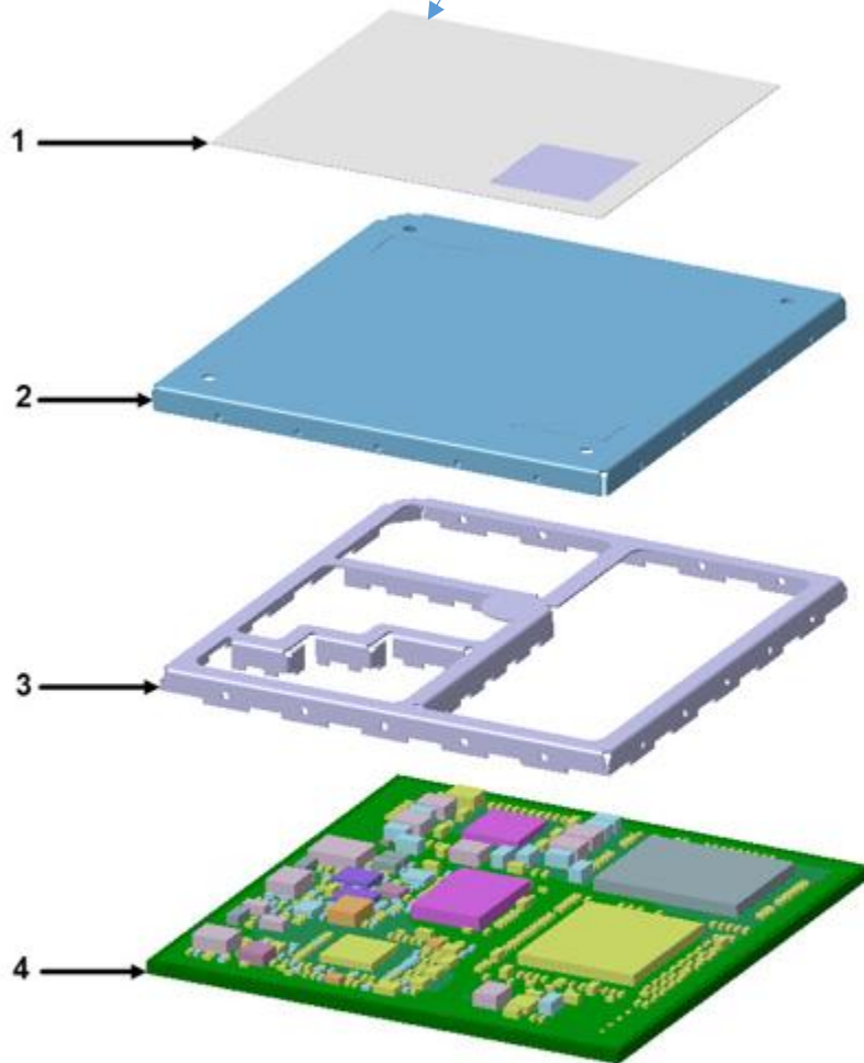
Figure 2} Module Exploded View
