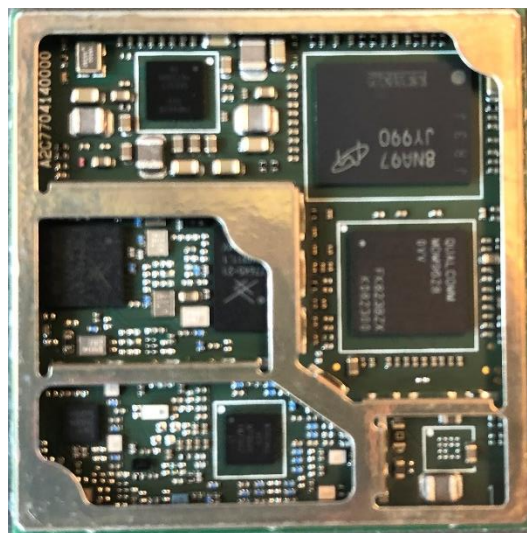
Fig. 2. BL28NA-RD1 top view with the shield removed.
