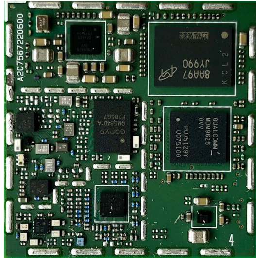
Fig. 3. BL28NA-003 module top view with the shield and shield frame removed.
