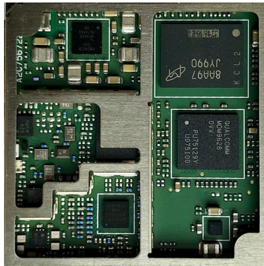
Fig. 2. BL28NA-003 top view with the shield removed.
