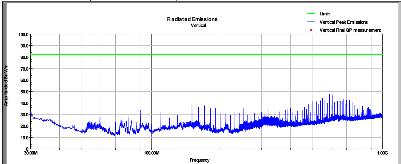
Band II, Low Channel (Vertical, 30-1000MHz)
