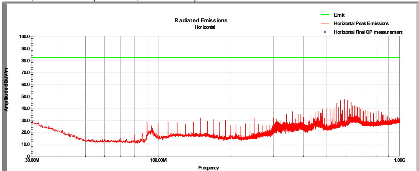
Band II, Low Channel (Horizontal, 30-1000MHz)
